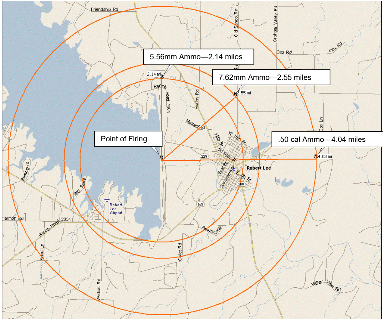
Figure 6-1 Maximum Ammunition Ranges for NATO Standard Ammunition for a Hypothetical Facility (Ball Type)
