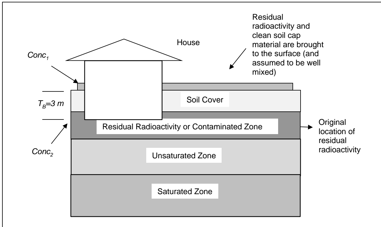
Figure J.4 Conceptual Model of Human Disturbance into Buried Residual Radioactivity (showing some of the Waste Mixed with Clean Soil on the Surface [ Conc_1 ] and some Waste Remaining at Depth [ Conc_2 ])
