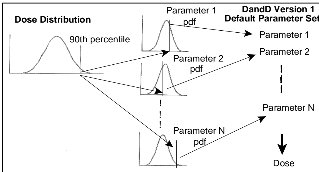
Figure I.10 Treatment of Parameter Uncertainty in DandD Version 1
