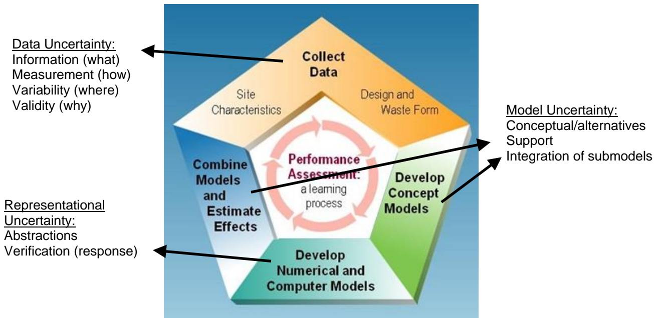
Figure Q.2 Uncertainty Types Associated with Performance Assessment
