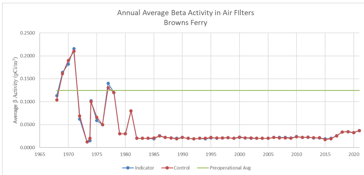
Figure H-1 - Average Beta Activity in Air Filters
