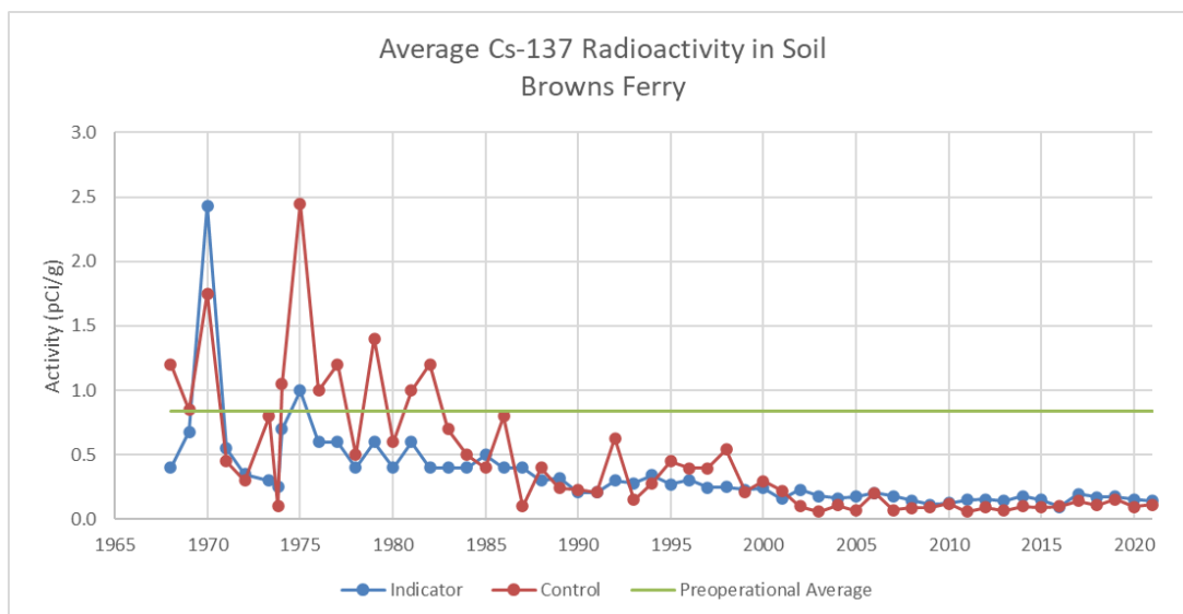
Figure H-2 - Average Cs-137 Radioactivity in Soil
