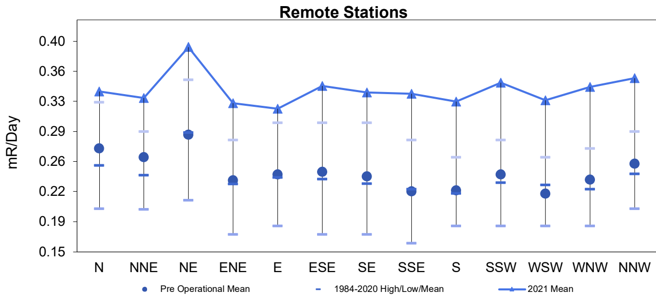
Figure 5-3 Remote Stations Quarterly TLDs 1984-2020 Hi/Low/Mean and 2021 Dosimeter Mean by Sector
