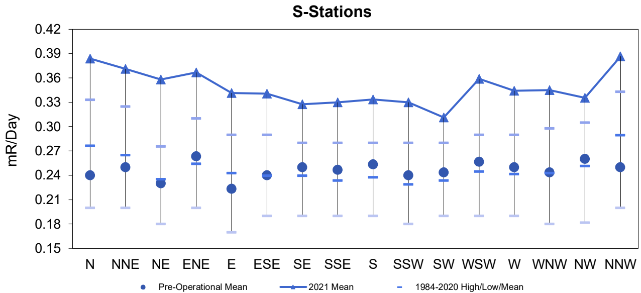
Figure 5-1 "S" Stations Quarterly TLDs 1984-2020 Hi/Low/Mean and 2021 Dosimeter Mean by Sector
