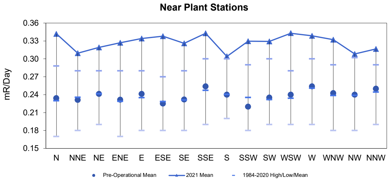
Figure 5-2 Near Plant Stations Quarterly TLDs 1984-2020 Hi/Low/Mean and 2021 Dosimeter Mean by Sector
