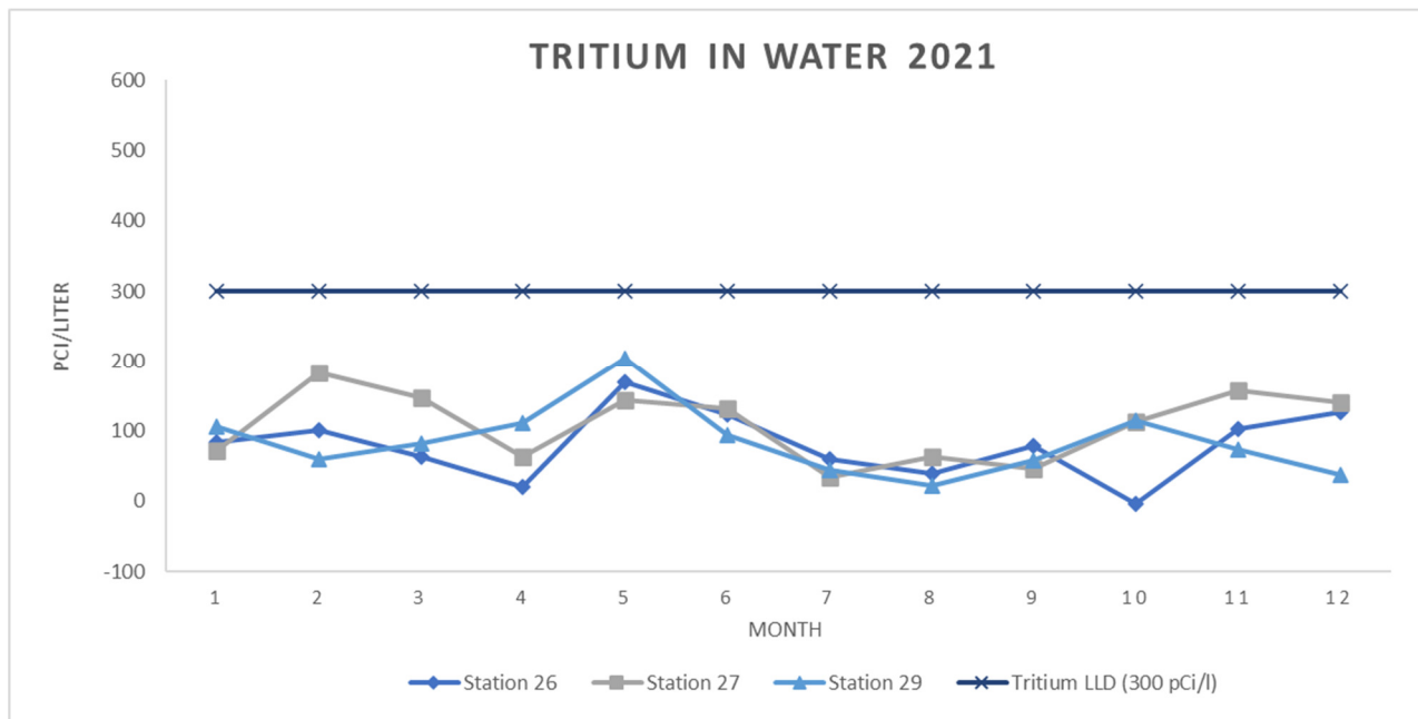
Figure 5-7 Tritium in River/Drinking (Stations 26 & 29) and Plant Discharge Water (Station 27) for 2021
