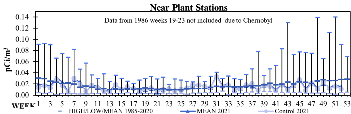
Figure 5-4 1985-2020 Weekly Hi/Low/Mean and 2021 Weekly Mean Gross Beta in Air - Near Plant Stations
