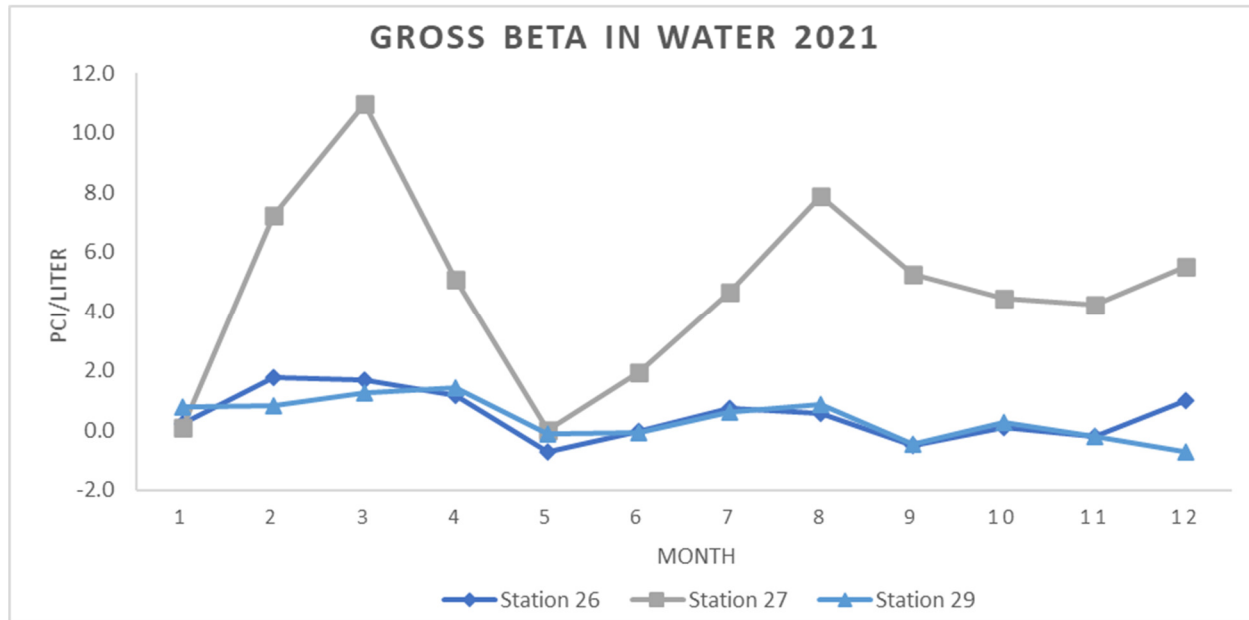
Figure 5-6 Gross Beta in River/Drinking (Stations 26 & 29) and Plant Discharge Water (Station 27) for 2021
