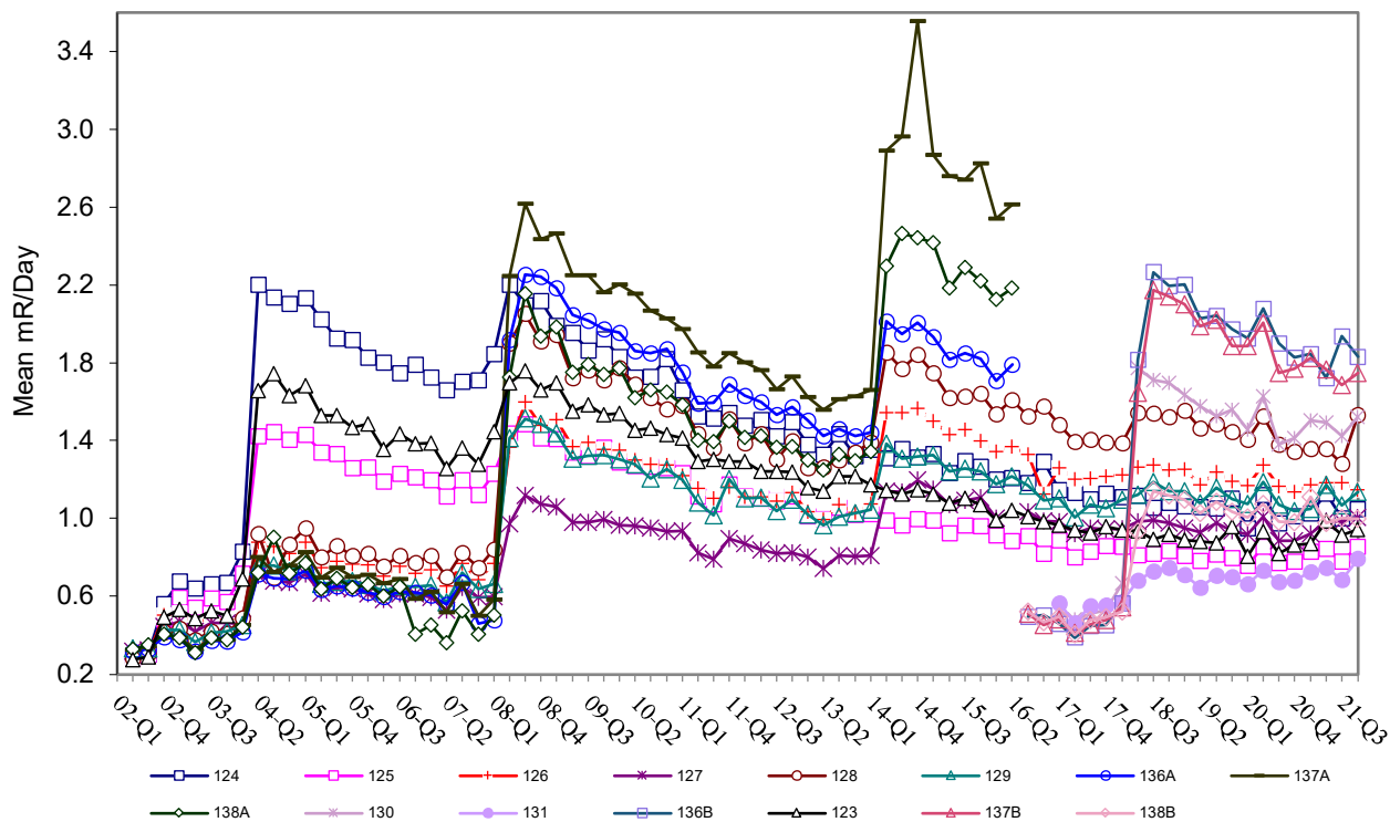
Trend of Exposure Rates at ISFSI Fence Line
