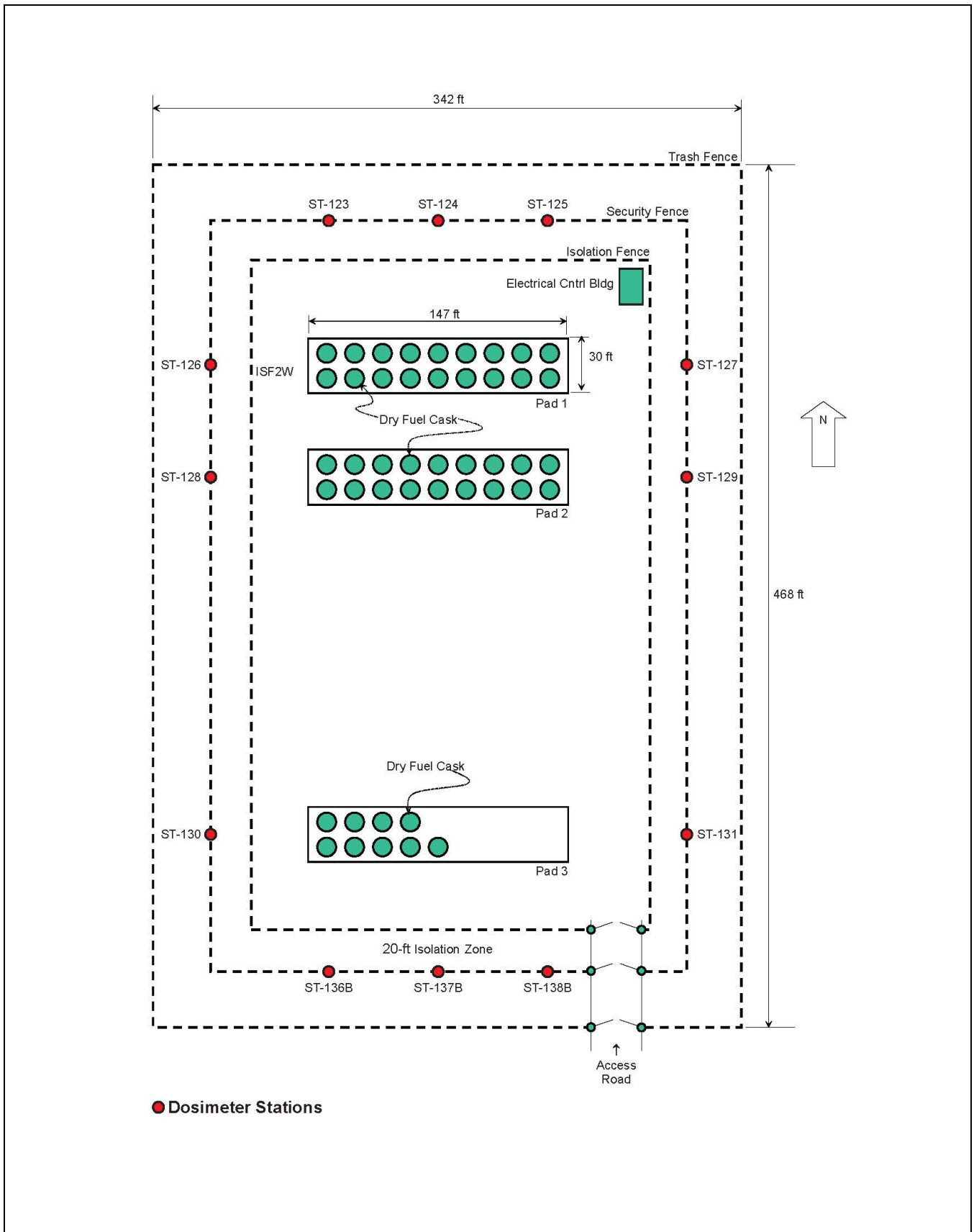
FIGURE 4-4 ISFSI DOSIMETER STATION LAYOUT
