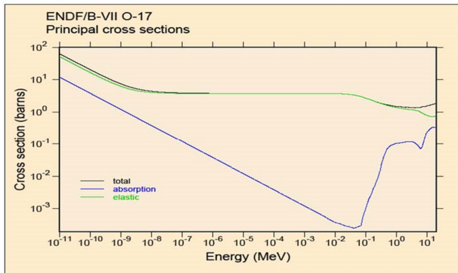
Figure 3: ENDF/B VII Cross Sections for ^{17}\text{O}
