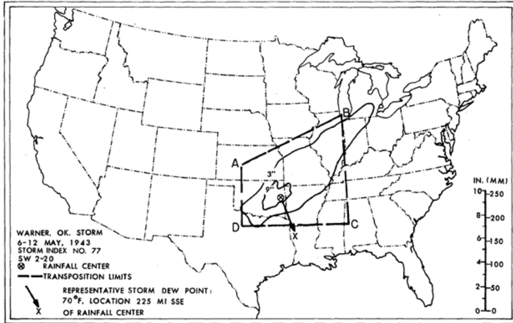
Figure 4-1 HMR transposition limit map for a May 1943 Warner, OK, storm (from HMR No. 51)
