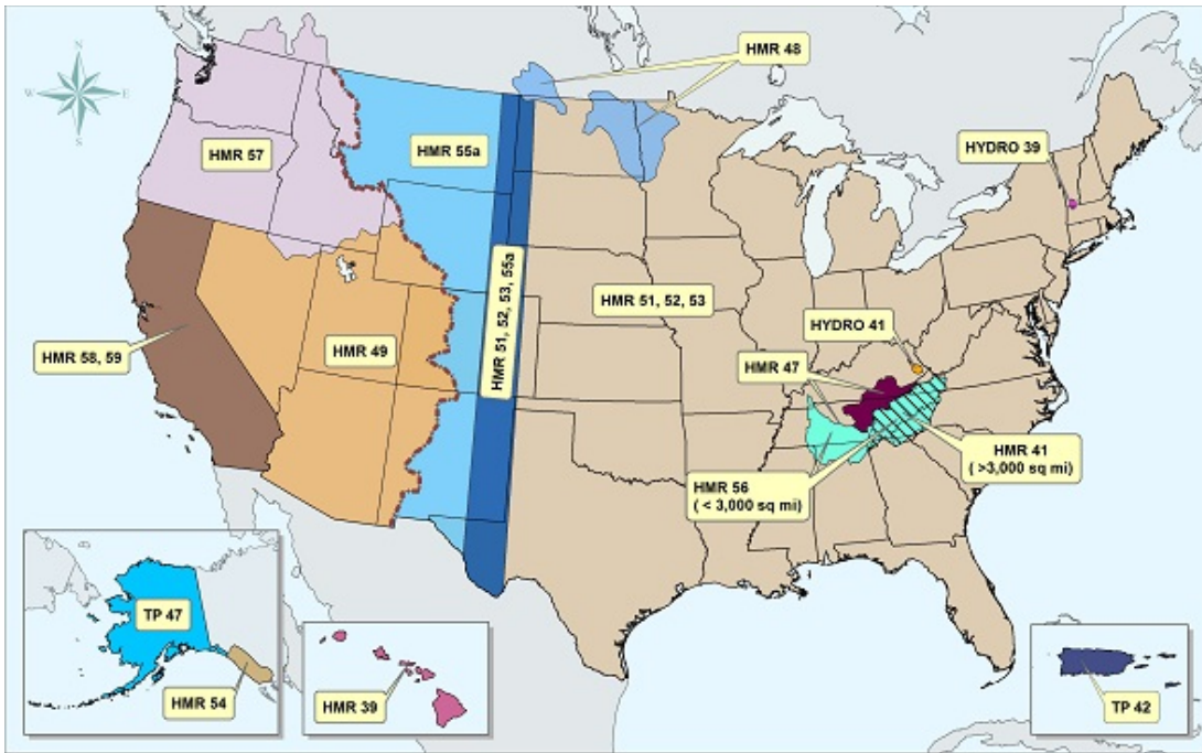
Figure 1-1 Map of regions covered by NOAA PMP documents (as of 2015) https://www.nws.noaa.gov/oh/hdsc/studies/images/pmp_figure.jpg
