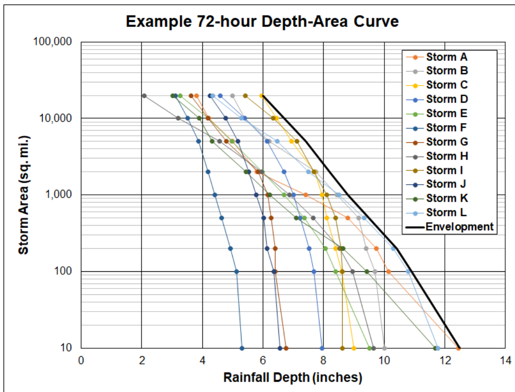
Figure 8-1 Example DAD curves (including envelopment) for a 72-h PMP (Note: Values do not represent actual storms or PMPs)
