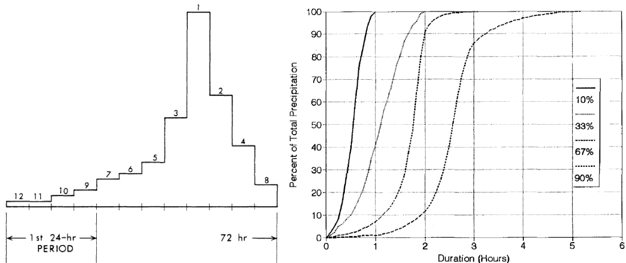
Figure 9-2 Example temporal distribution for a watershed-scale 72-h PMP event provided in HMR No. 52 (left) and example temporal distributions for middle-loaded, local-scale storms provided in HMR No. 57 (right)
