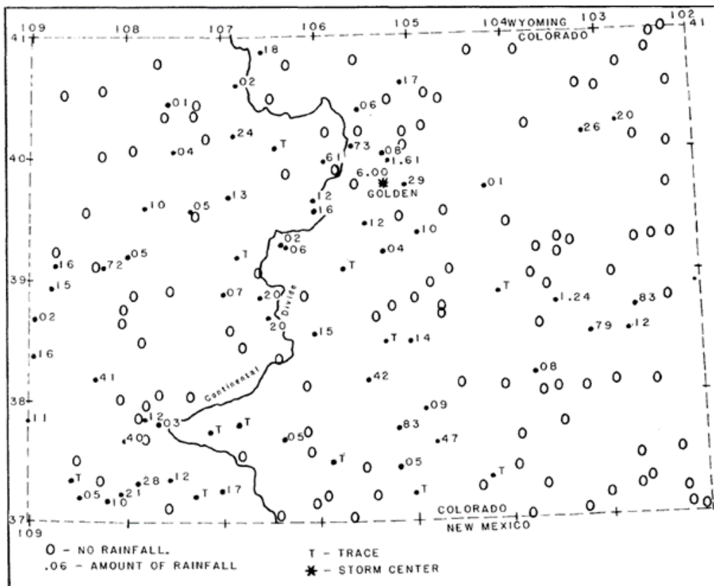
Figure 3-1 Map of precipitation gauge data for a June 1948 Golden, CO, storm (from HMR No. 55A)
