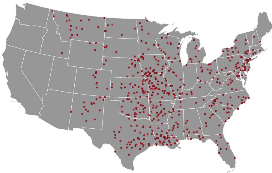
Figure 2-1 Map of USACE Black Book storm locations (data from USACE 1973)
