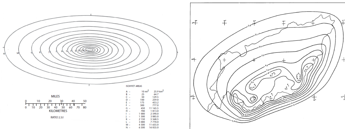
Figure 9-1 Standard isohyetal spatial distribution pattern recommended in HMR No. 52 (left; as included in WMO 2009) and example probable maximum March isohyets provided in HMR No. 41 (right)
