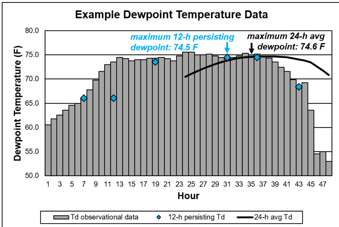
Figure 5-2 Example dewpoint temperature data with the maximum 24-h average dewpoint and maximum 12-h persisting dewpoint values identified
