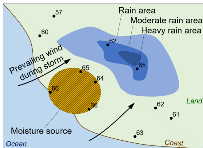
Figure 5-1 Example weather map showing moisture inflow and dewpoint observations (adapted from WMO 2009)
