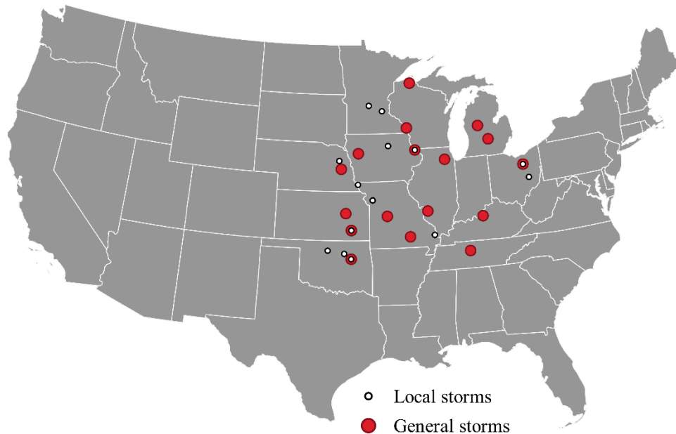
Figure 5-4 Map of storms used to evaluate alternative storm representative dewpoint conversion factors
