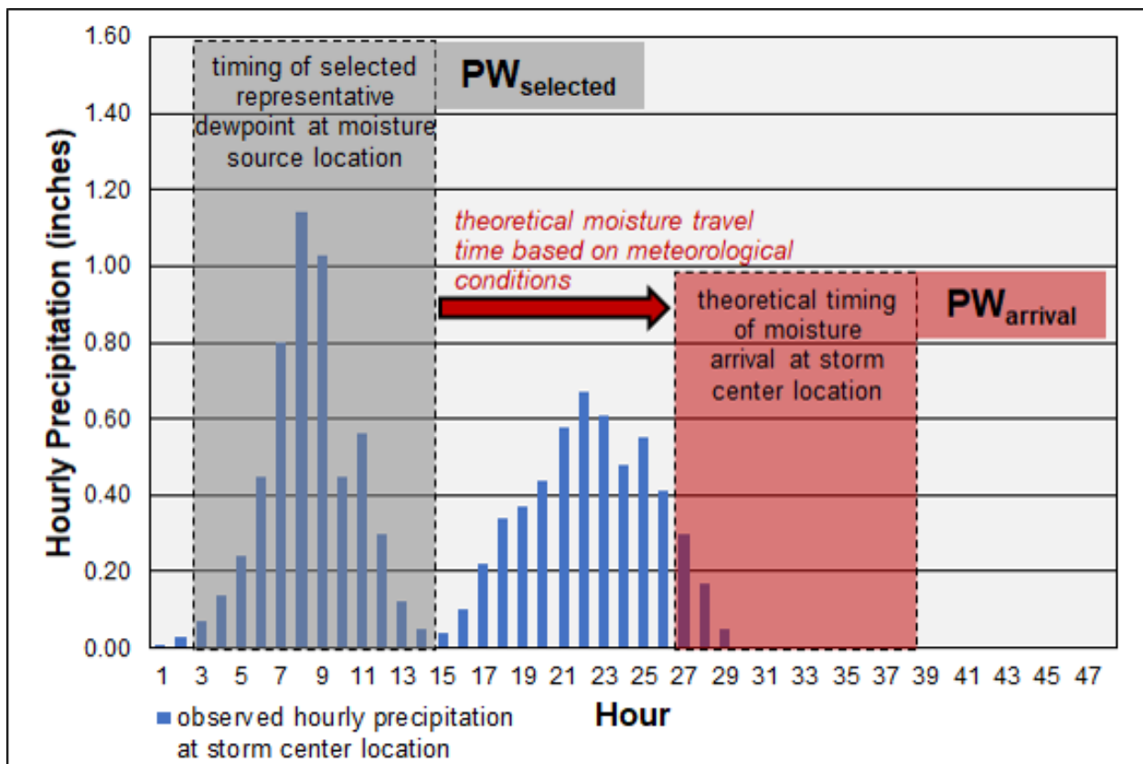
Figure 5-3 Example of improper representative dewpoint timing selection based on theoretical moisture travel time for precipitation event
