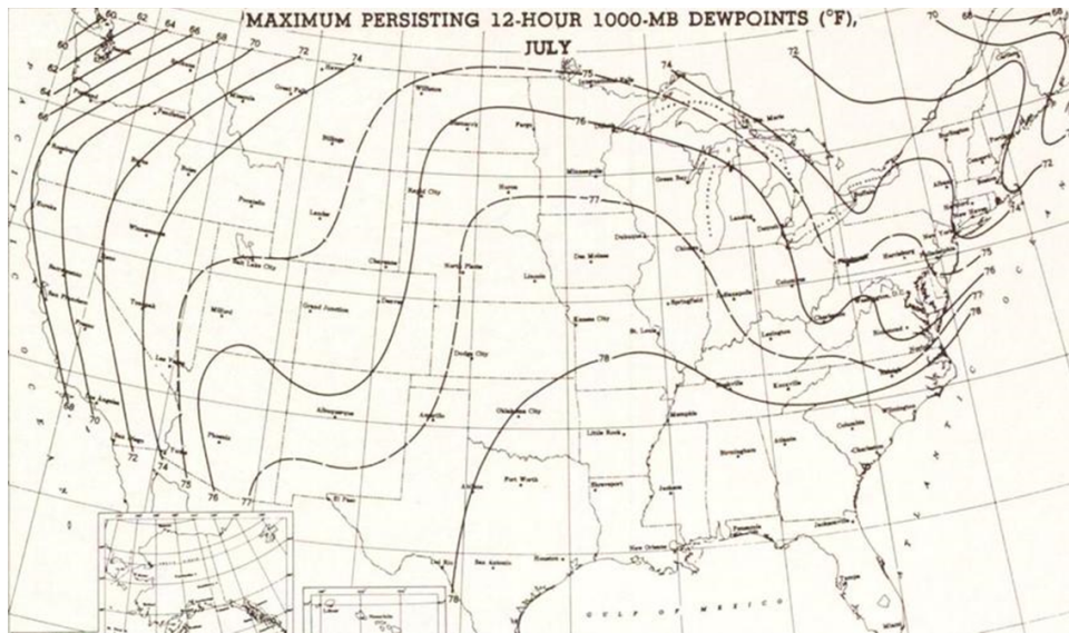
Figure 6-1 Example maximum 12-h persisting dewpoint map for July (EDS 1968)
