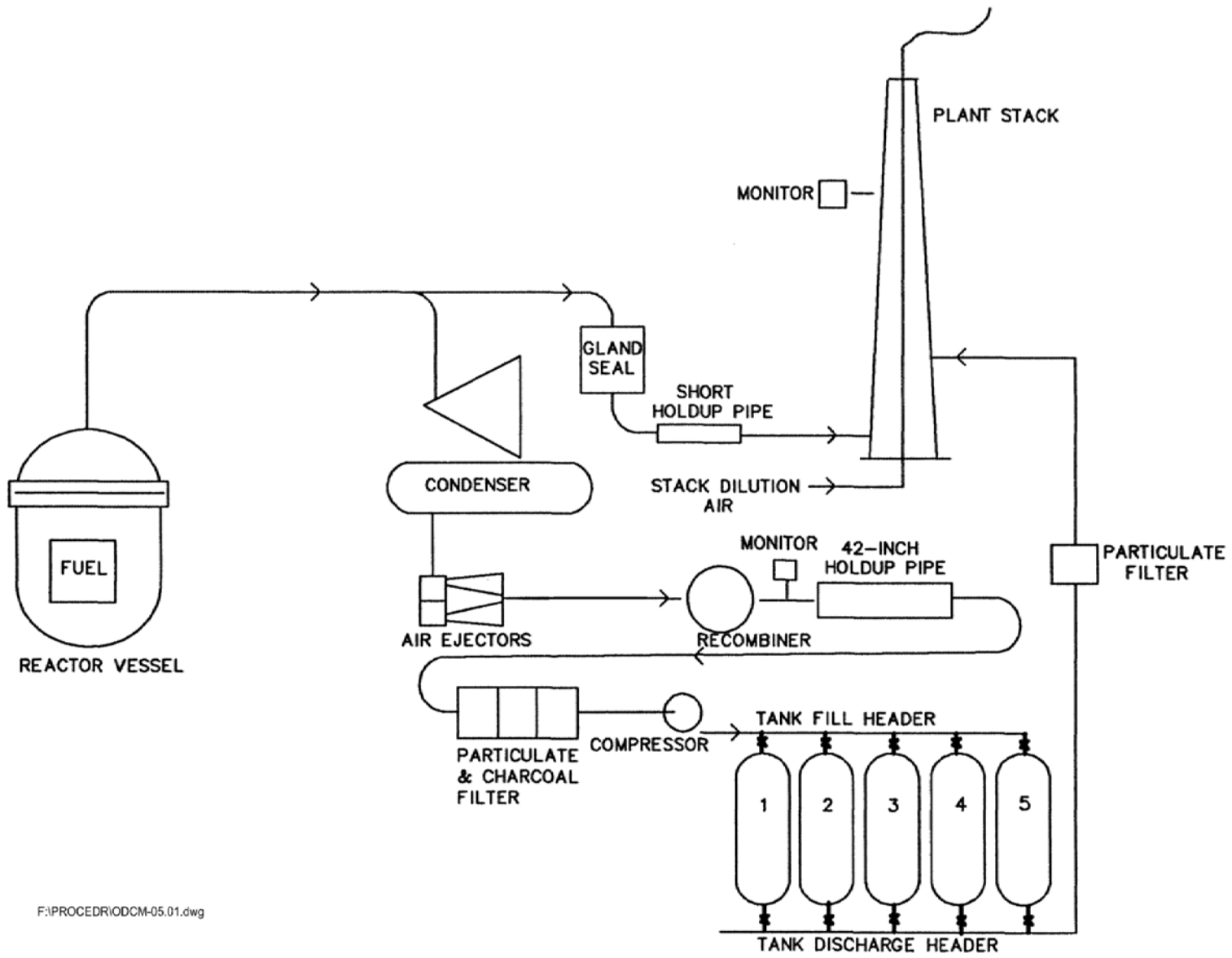
Figure 1 Gaseous Radwaste
