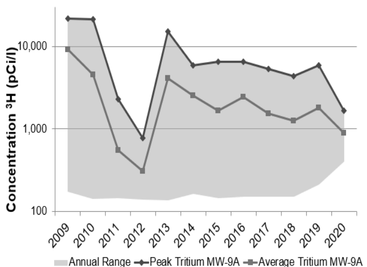
FIGURE 6: ANNUAL TRITIUM ACTIVITY TRENDS MW-9A FROM 2009-2020.
