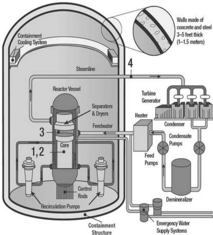
FIGURE 1: TYPICAL BOILING WATER REACTOR (BWR) DESIGN. (US NRC, REF. [10])
