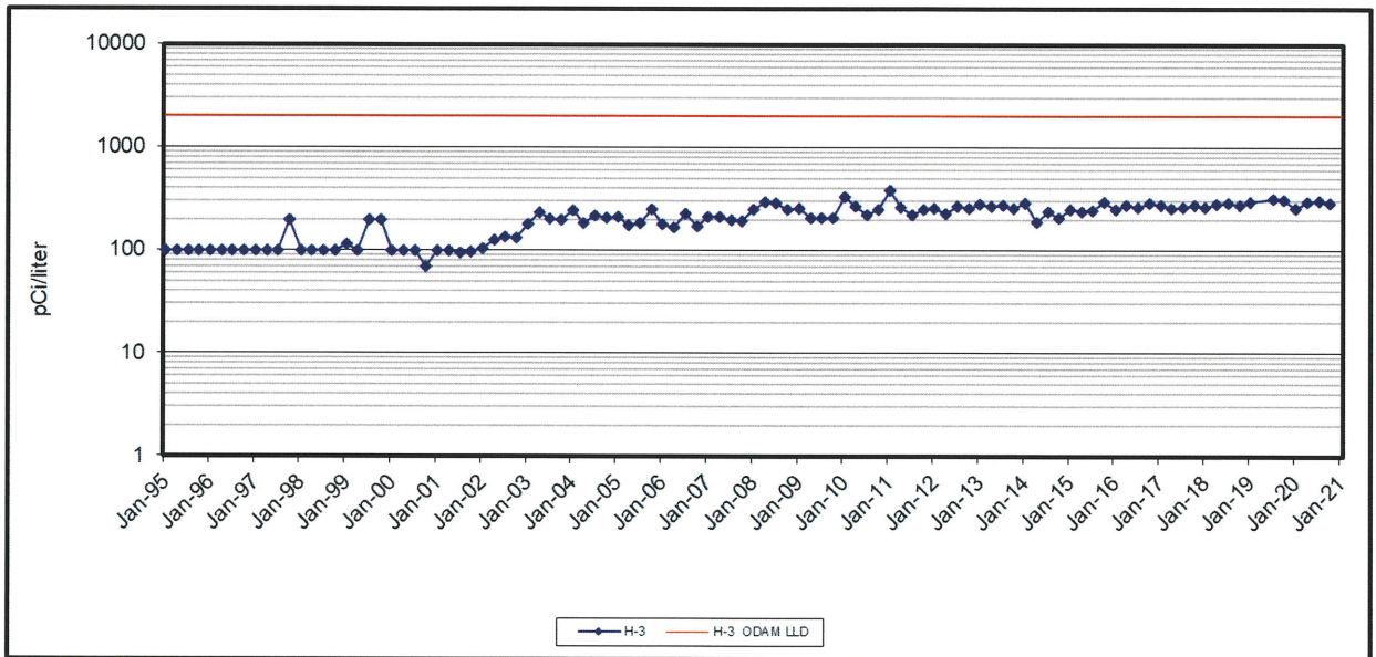
TRENDING GRAPH 6 TRITIUM IN RIVER WATER QUARTERLY AVERAGE – ALL LOCATIONS
