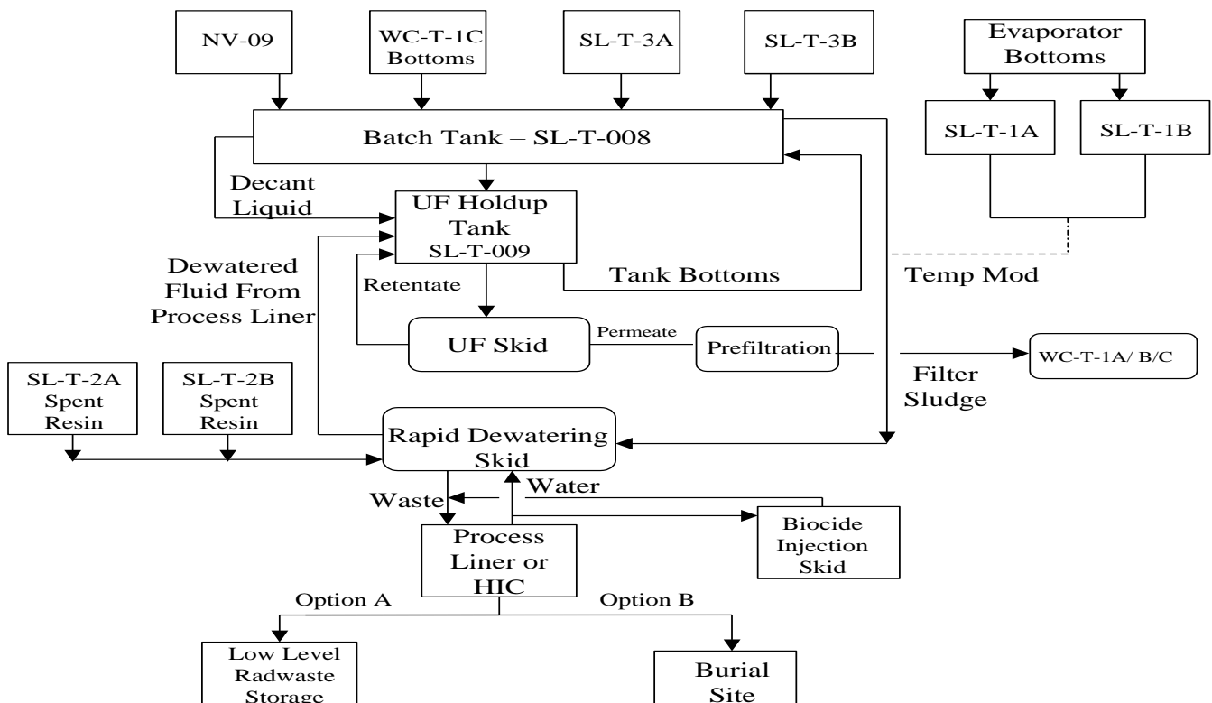
FIGURE D-1-2: SOLID RADWASTE PROCESSING SYSTEM
