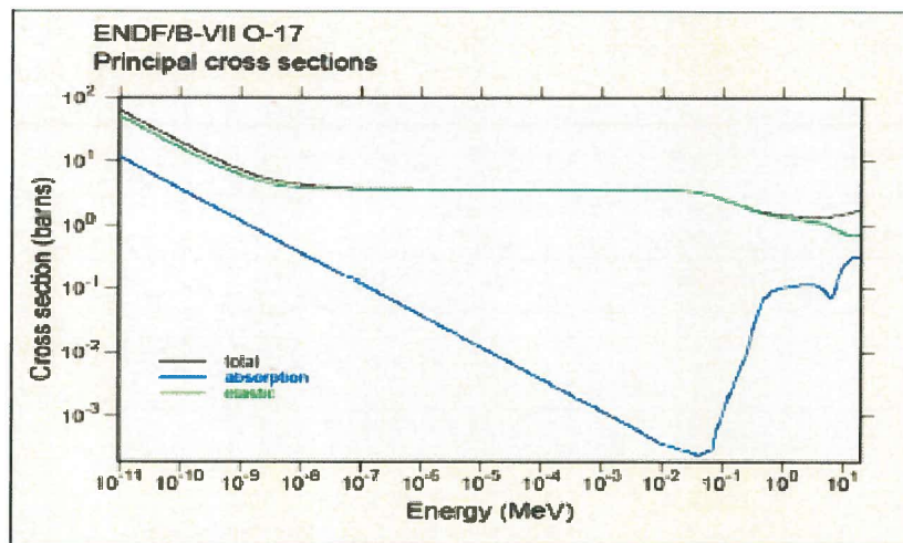
Figure 3: ENDF/B VII Cross Sections for ^{17}\text{O}
