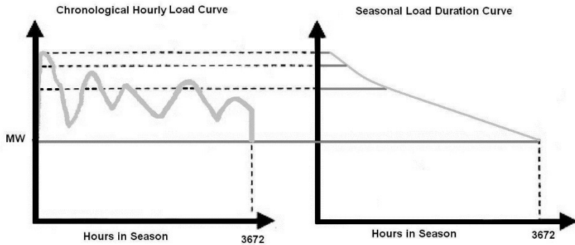
3 4 Figure A-1 Hypothetical Chronological Hourly Load Curve and Seasonal Load Duration 5 Curve
