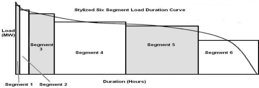
26 27 Figure A-2 Stylized Depiction of a Six Segment Load Duration Curve Used in EPA 28 Platform v6 (EPA, 2019)
