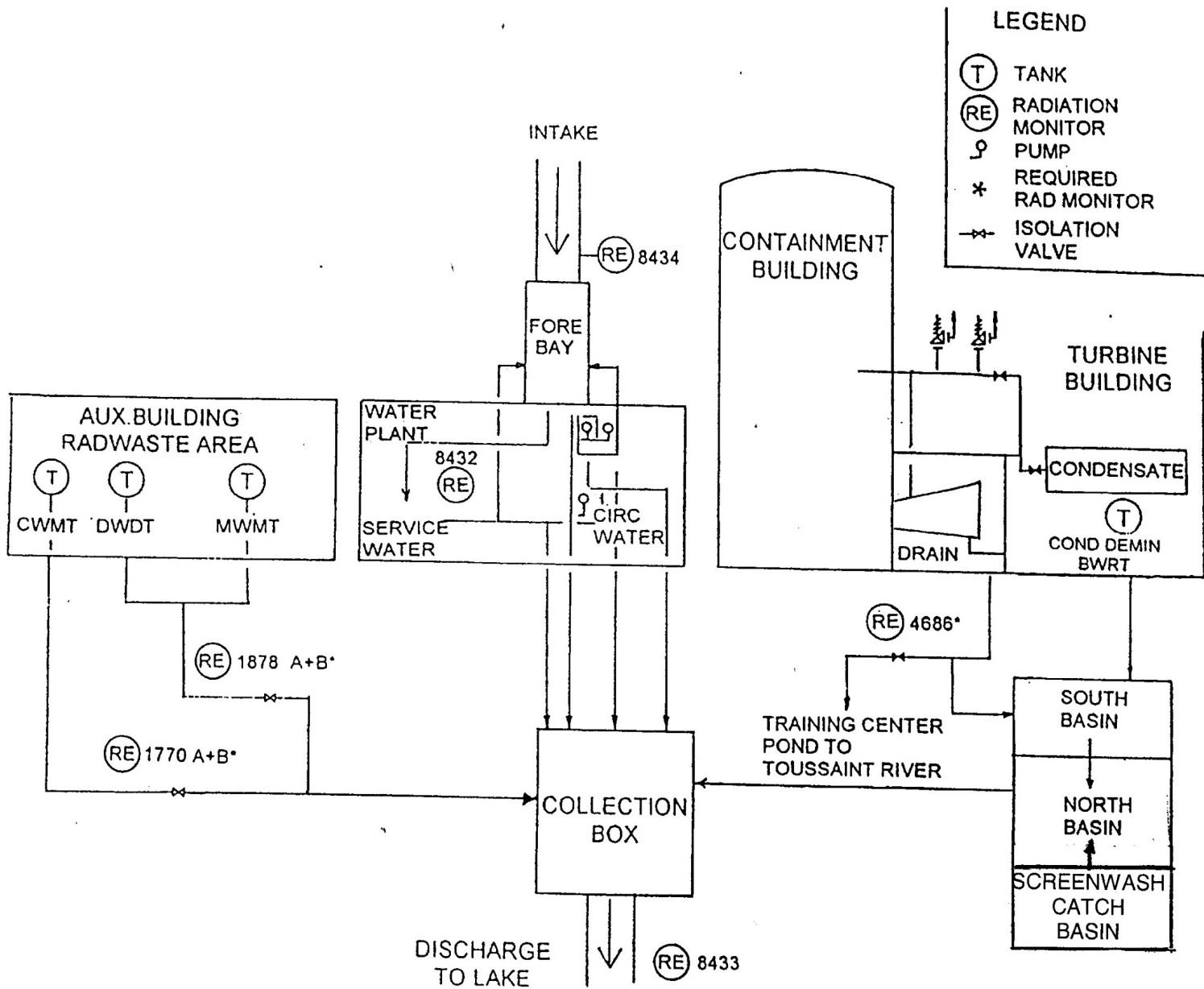
Liquid Radioactive Effluent Monitoring and Processing Diagram
