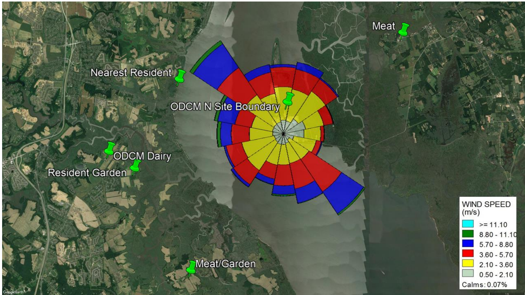
Figure 7 Locations of Dose Calculation Receptors with 2019 Wind Rose Overlay
