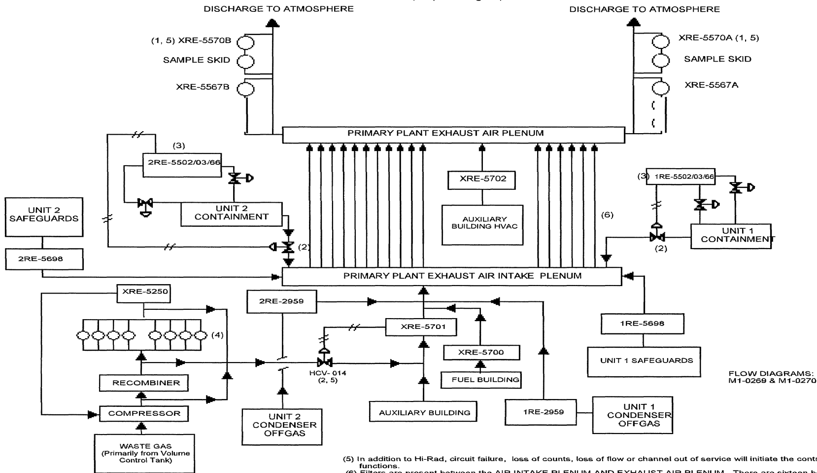
FIGURE 2.1 (Simplified diagram)
