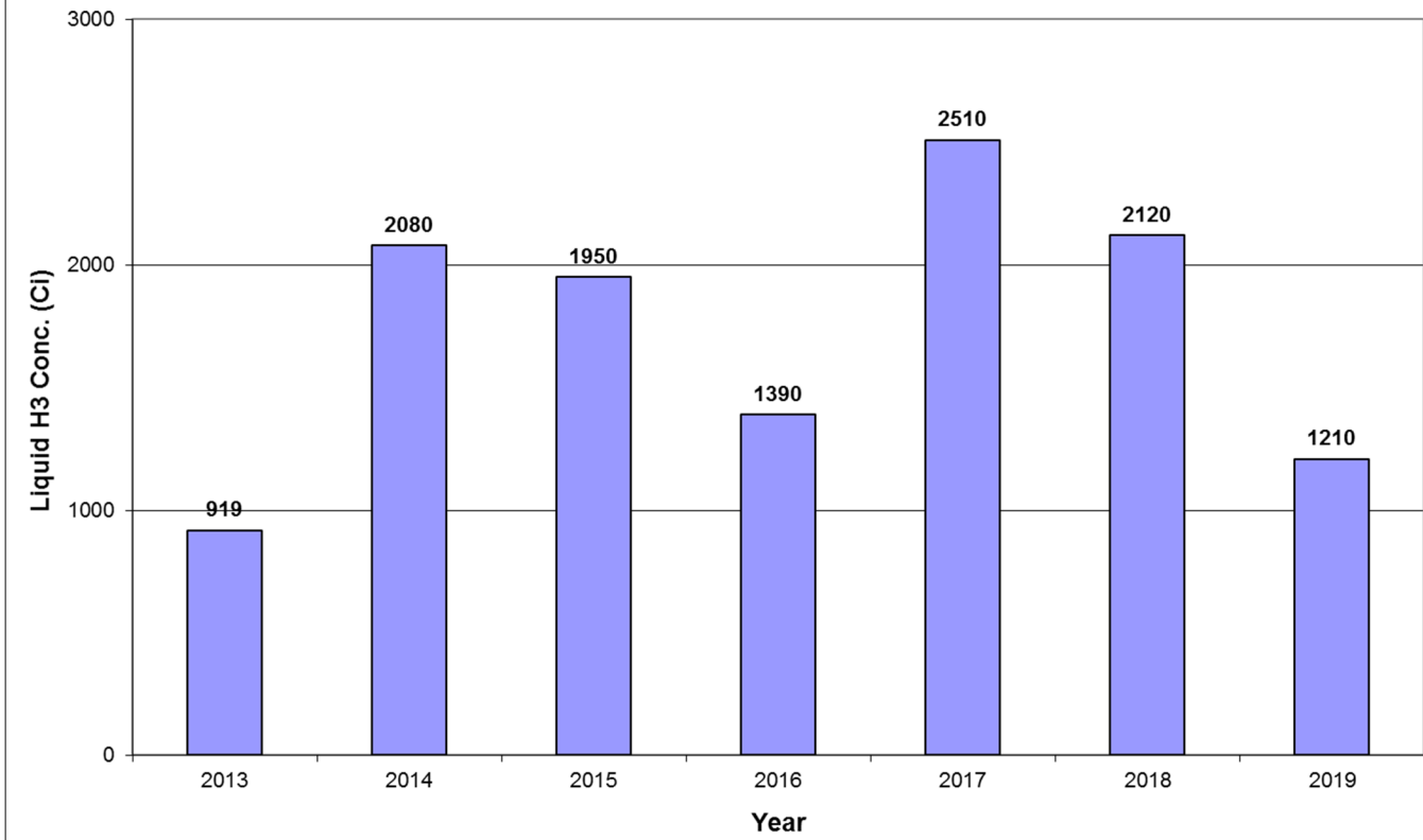
Total Curies of Tritium Released in Liquid Effluents
