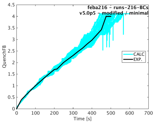
Figure 5-1 Simulation of Feba-216 – Effects of Uncertainty on Boundary Conditions
