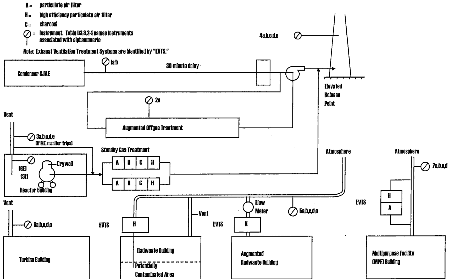
Figure 3-1 Caseous Effluent Streams, Treatment and Monitoring Equipment, and Discharge Points.
