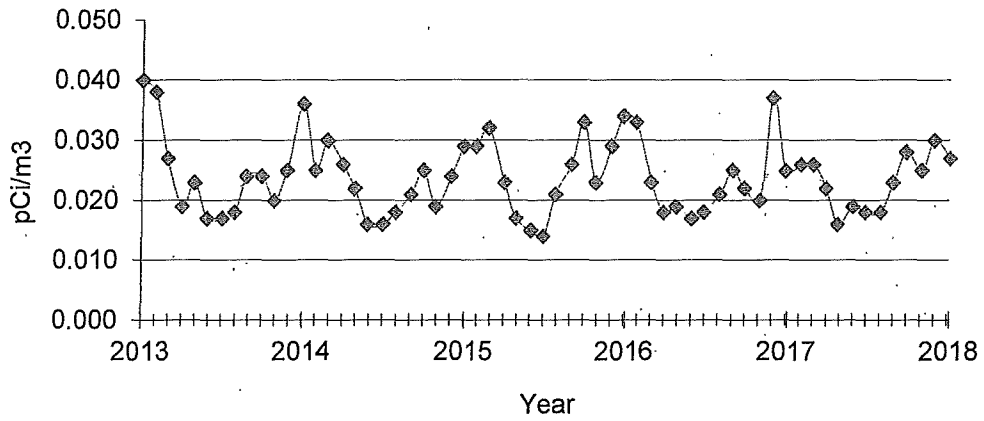
Location E-20, monthly averages 2013-2017
