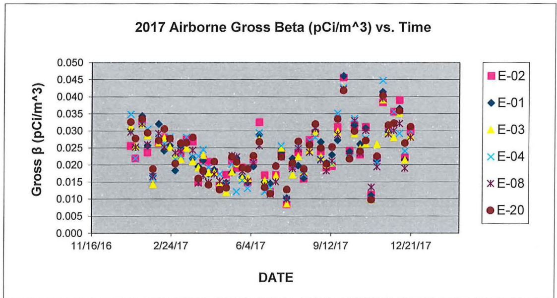
Figure 11-5 2017 Airborne Gross Beta
