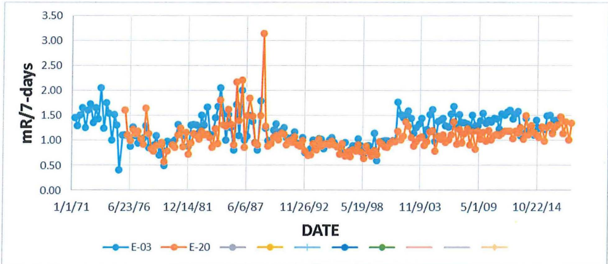
Figure 11-8 Comparison of E-03 and E-20 Results 1971 – 2017
