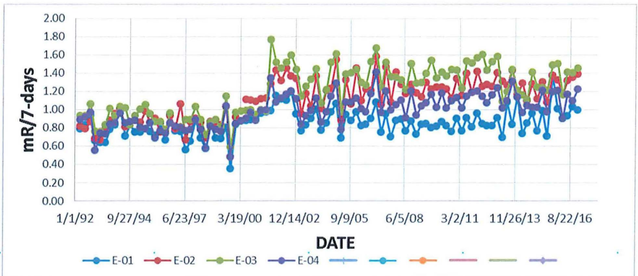
Figure 11-9 Comparison of E-01, E-02, E-03 and E-04 (1992 –2017)
