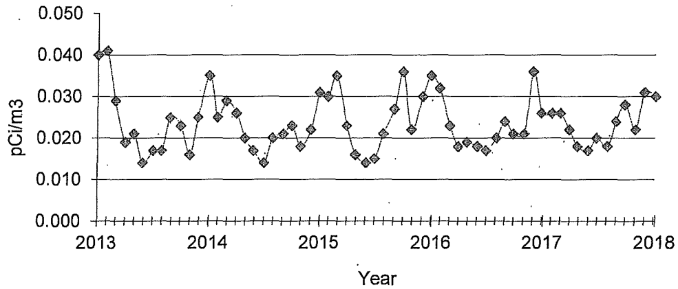
Location E-4, monthly averages 2013-2017
