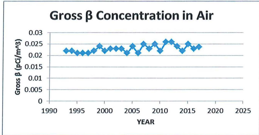
Figure 11-4 Annual Average Air Gross \beta (1993 – 2017)
