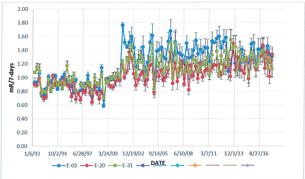
Figure 11-10 E-03, E-31, and Background Site E-20 Results 1992 to 2017
