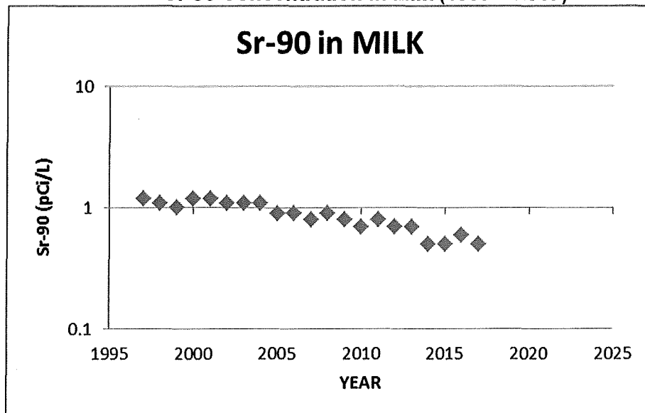
Figure 11-3 Sr-90 Concentration in Milk (1997 – 2017)
