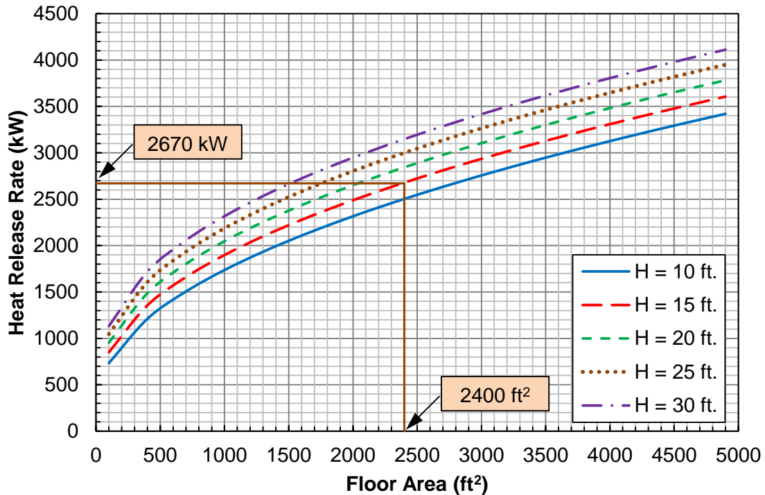
Figure 5.2.7 – Minimum HRR Required Creating a Damaging HGL for TS Targets in a Compartment with a Floor Area of 2400 ft 2 and Ceiling Height of 15 ft.
