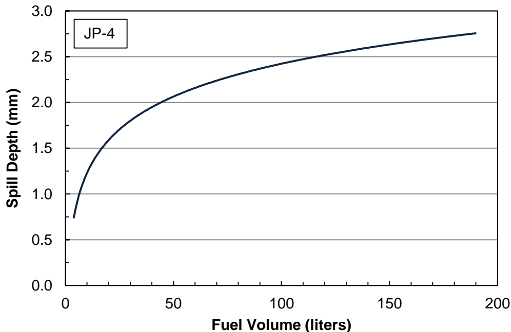
Figure 6.2.1 – Spill Depth as a Function of Fuel Volume for Unconfined JP-4 Spills. (Source: Figure 2-15.1 in Reference 28)
