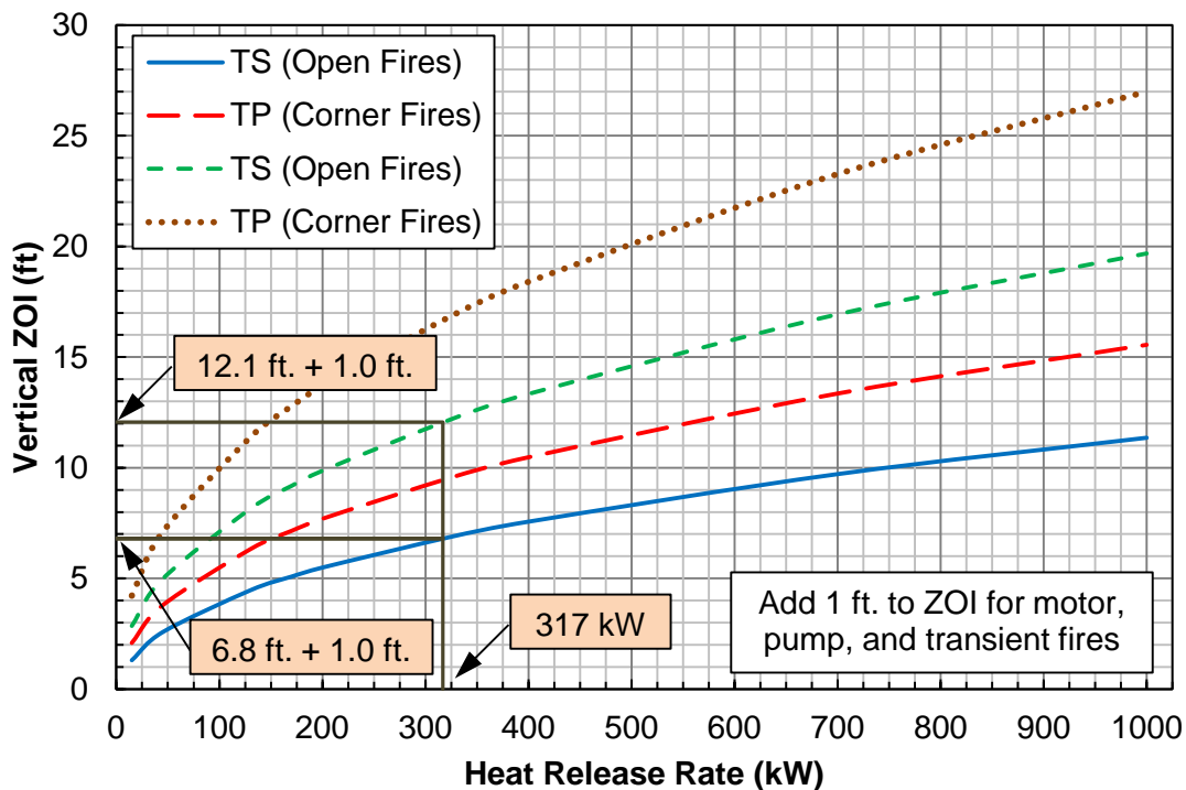
Figure 5.2.3 – Finding the Vertical ZOI for a Transient and TS Cable Target from Plots.
