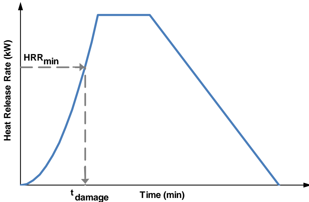
Figure 6.2.4 – Damage Time Determination for FDS1 Scenarios.
