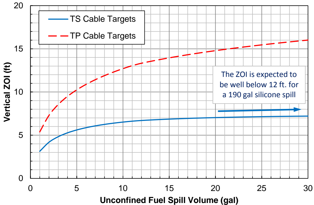
Figure 5.2.6 – Vertical ZOI for an Unconfined Silicone Liquid Spill Fire and a TS Target.
