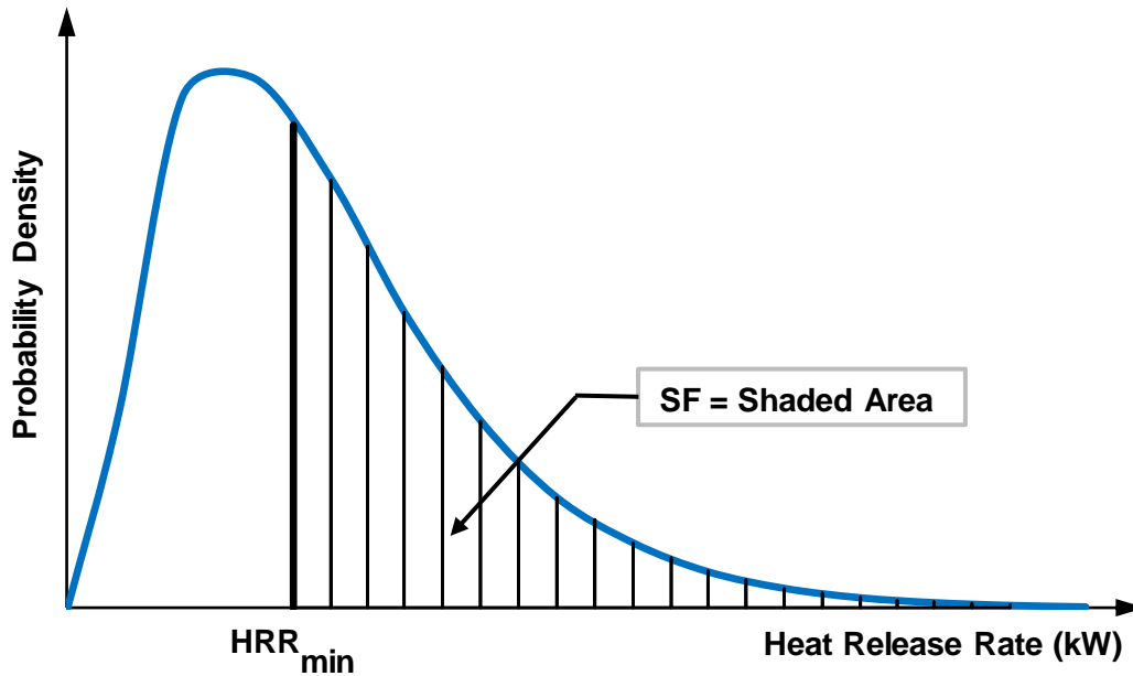
Figure 6.2.3 – Determination of the Severity Factor.
