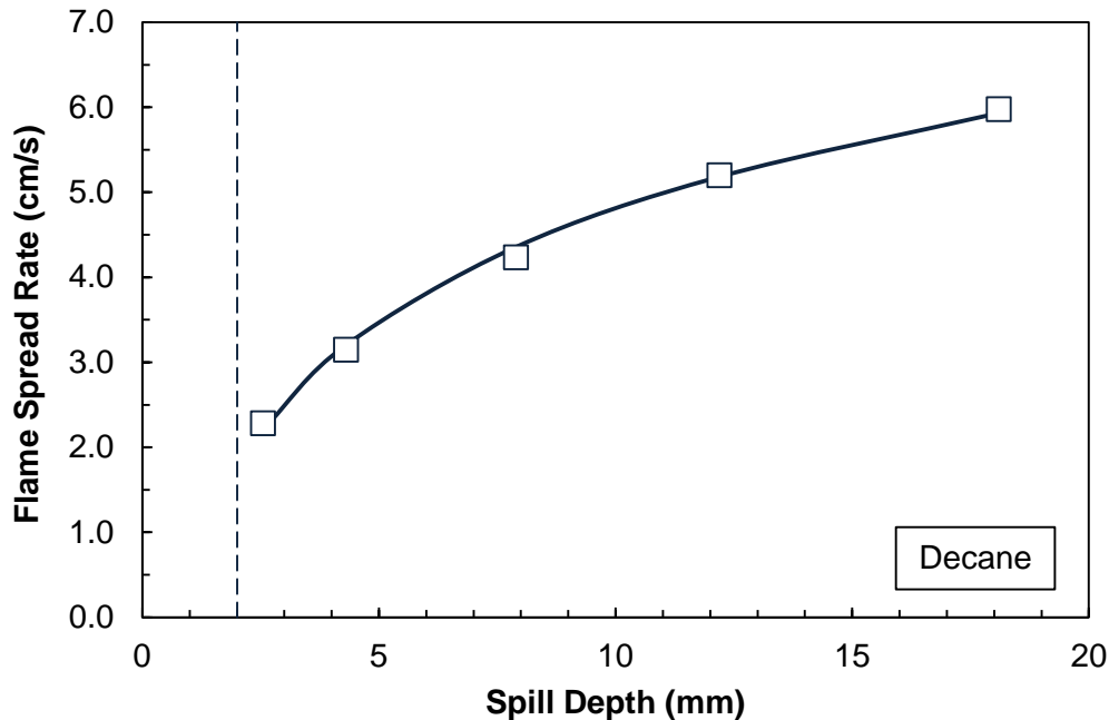
Figure 6.2.2 – Flame Spread Rate versus Spill Depth for an Unconfined Decane Spill. (Source: Figure 2-15.7 in Reference 28)
