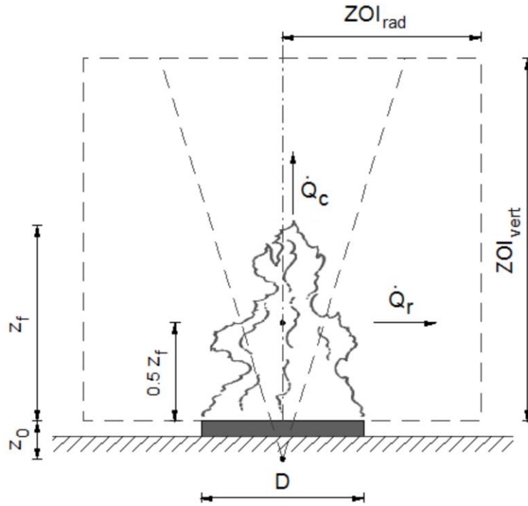
Figure 6.2.5 – Schematic of the Vertical and Radial ZOI.
