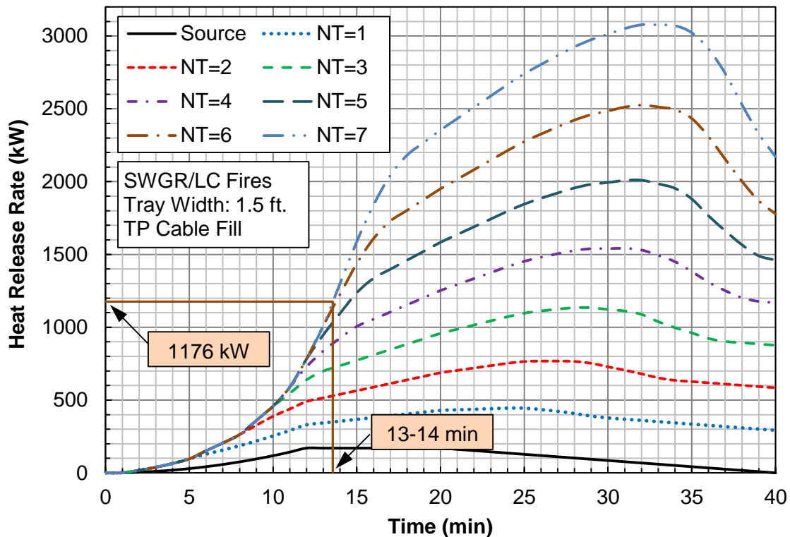
Figure 5.2.9 – HRR of a Switchgear Fire Involving a Vertical Stack 1.5 ft. Wide Horizontal Cable Trays Filled with TP Cables.
