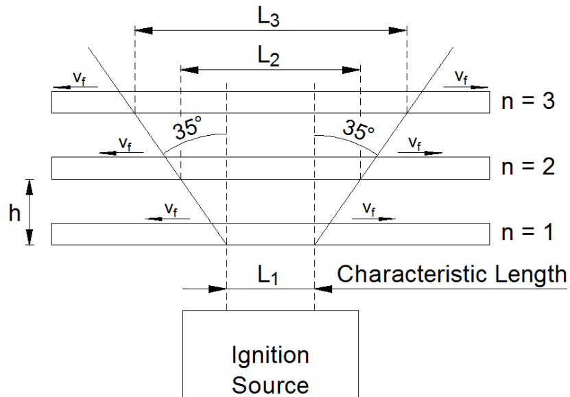
Figure 6.2.7. Configuration for Modeling of Fire Propagation in a Stack of Cable Trays.
