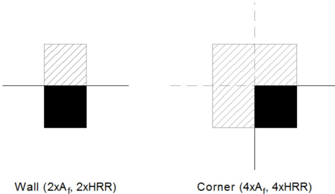
Figure 6.2.6. Schematic of the “Image” Method for Wall and Corner Fires.
