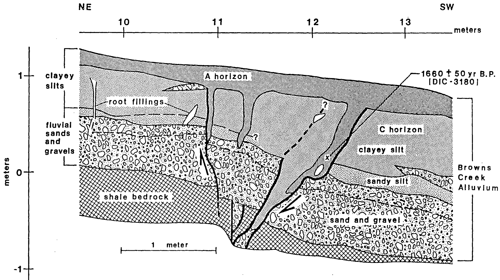
Figure 5. Part of the trench 1 log, showing stratigraphic relations near the main fault and location of 14 C age sample. Heavy lines are faults and edges of cracks that could be recognized by abrupt changes in the stratigraphy, dashed where inferred; arrows show general sense of displacement across the main fault zone. Fine lines are stratigraphic contacts, dashed where subtle.
