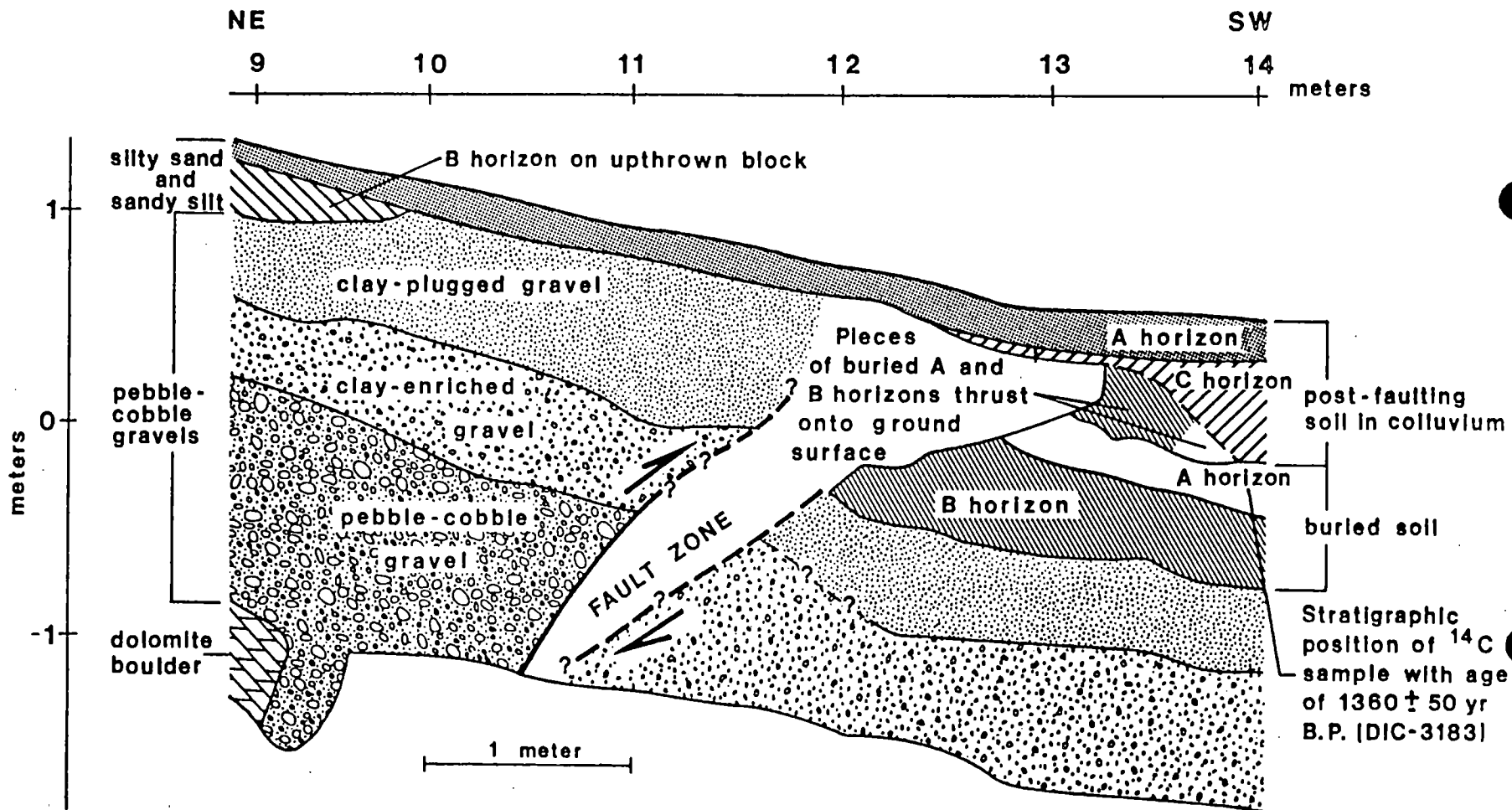
Figure 6. Part of trench 2 log, showing stratigraphic relations near the main fault zone. Heavy lines are faults that could be recognized by abrupt changes in the stratigraphy (dashed where inferred); arrows show general sense of displacement across the main fault zone. Fine lines are stratigraphic contacts (dashed where subtle).
