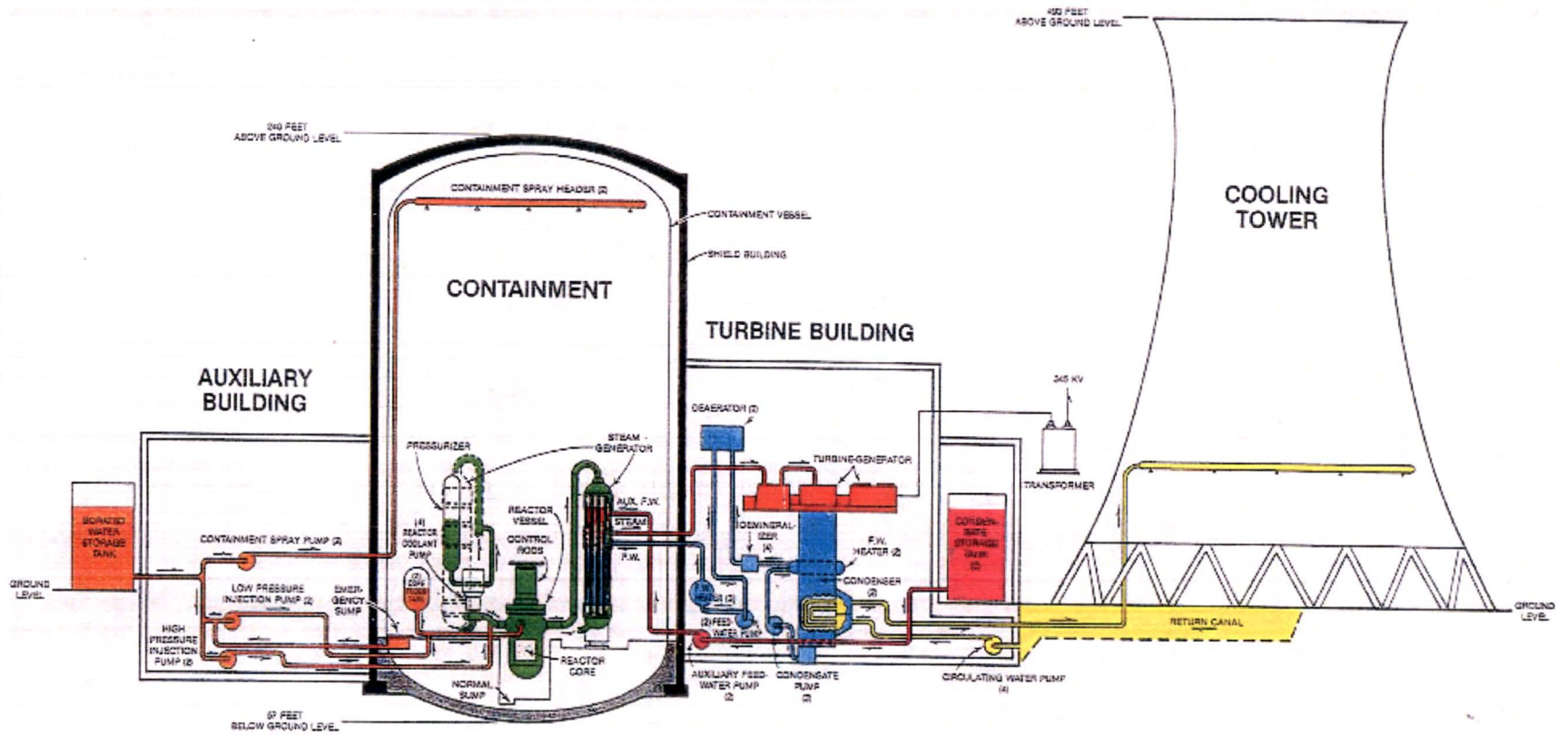
Figure 7: Station Systems
