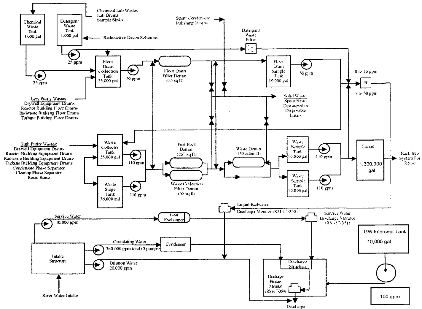
Figure 9.1: Radioactive Liquid Effluent Streams, Radiation Monitors, and Radwaste Treatment System at Vermont Yankee*
