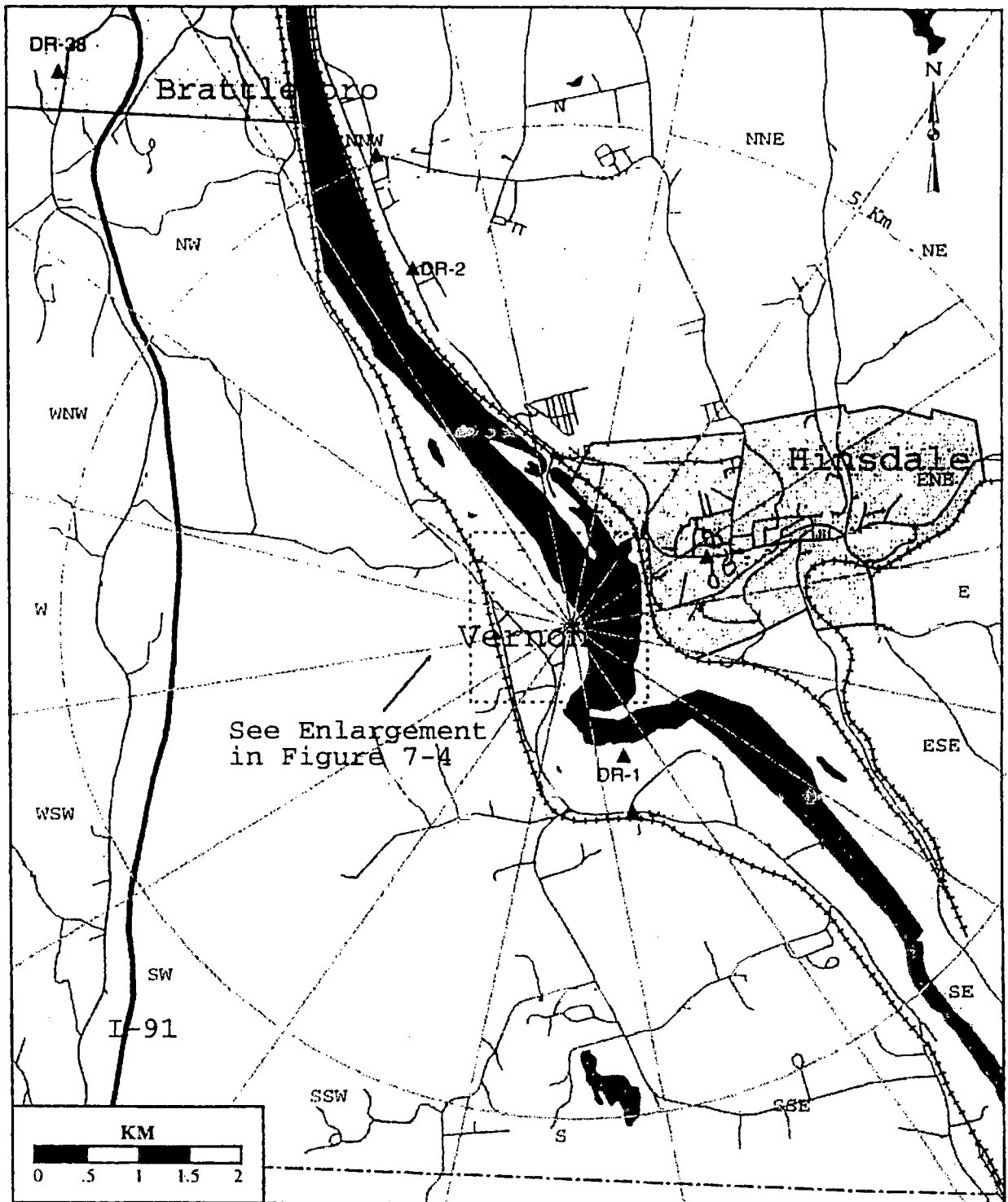
Figure 7-5 TLD Locations Within 5 Km of Plant
