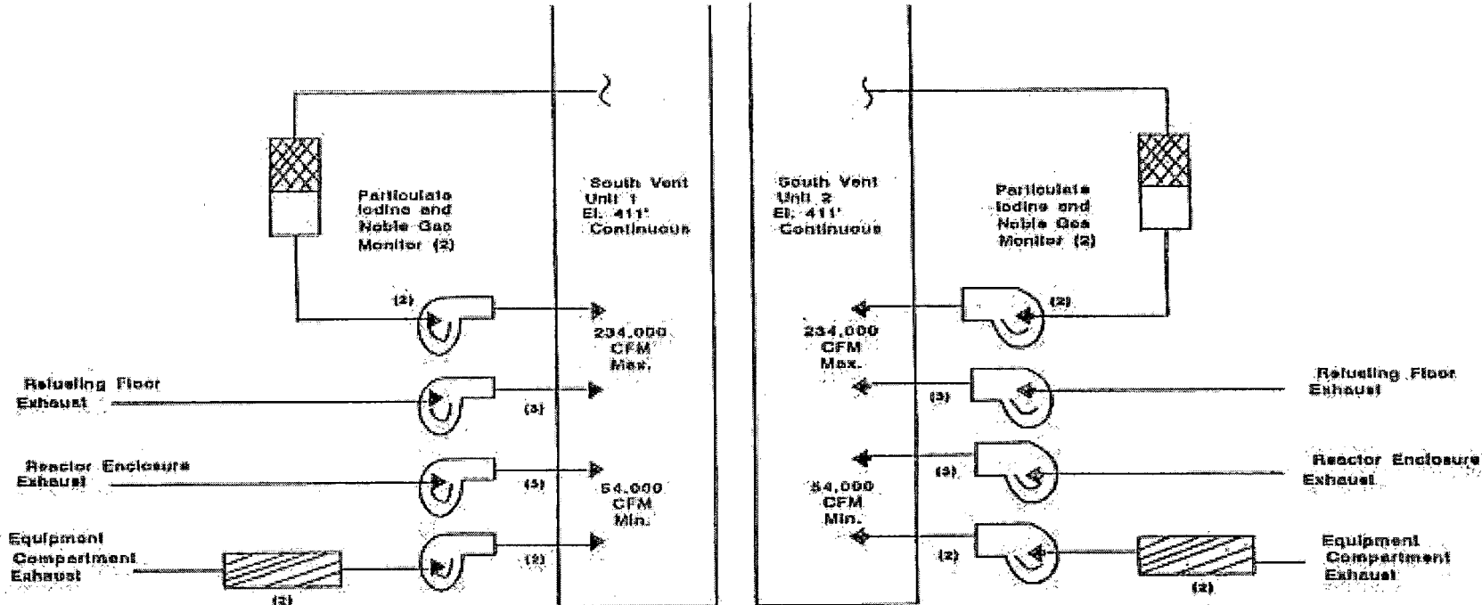
Limerick Generating Station Units 1 & 2 Gasous Effluent Flow Diagram South Stack
