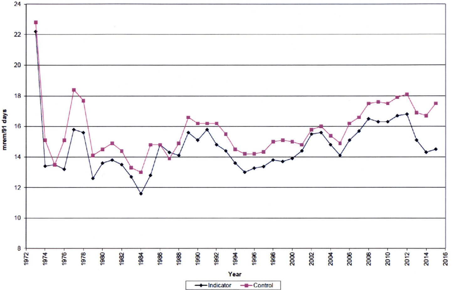
Gamma Dose for Environmental TLDs 1973-2015
