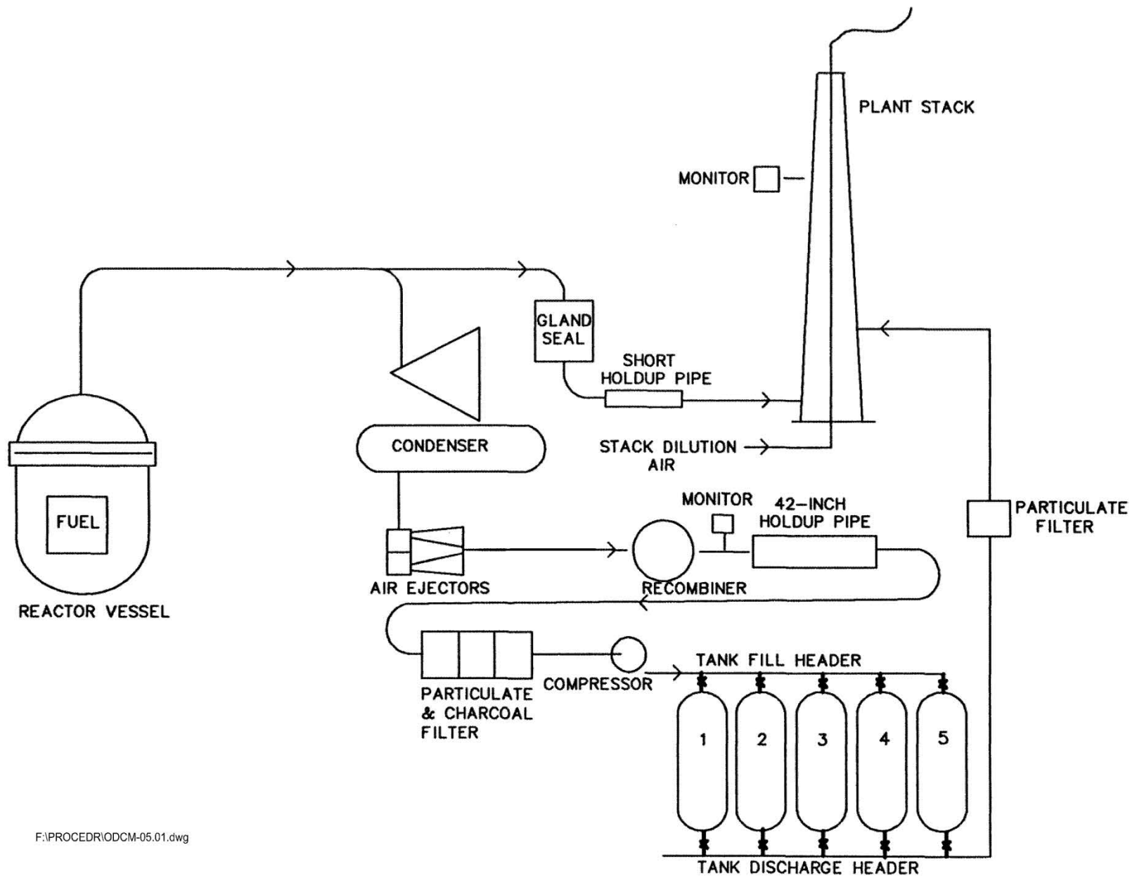
Figure 1 Gaseous Radwaste
