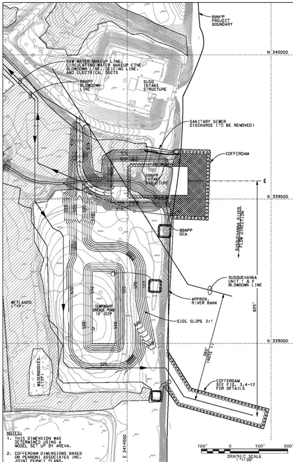
Figure 3-4. Location of BBNPP Intake and Discharge Structures Relative to SSES Intake and Discharge Structures (PPL Bell Bend 2013-TN3377)
