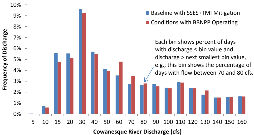
Figure 5-1. Effect of Operations of the Proposed BBNPP Unit on the Distribution of Daily Flows in the Cowanesque River below Cowanesque Dam
