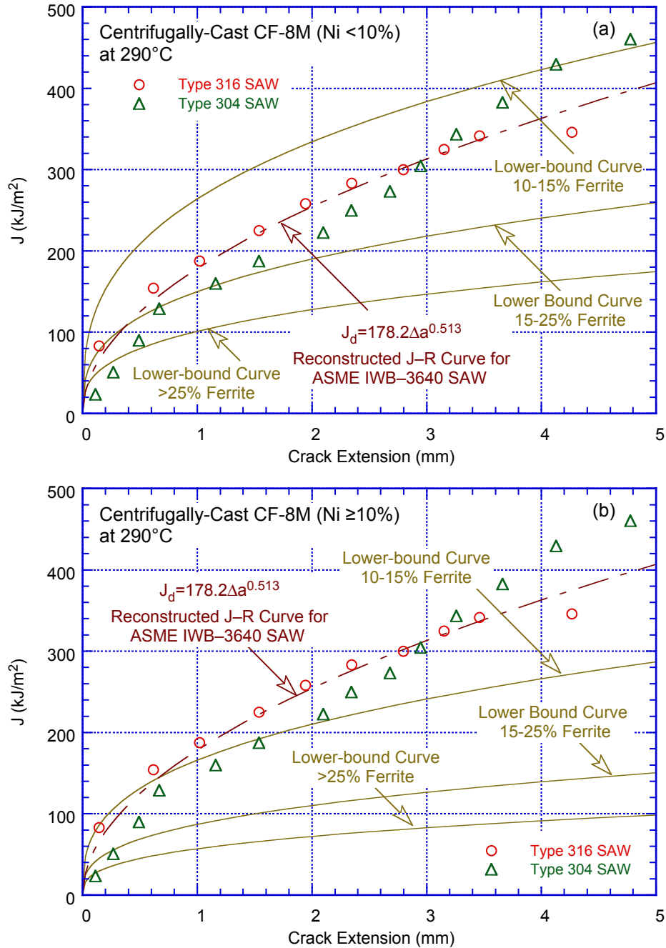
Figure 26. Comparison of the lower-bound fracture toughness J-R curve for thermally aged centrifugally-cast CF-8M steels containing (a) <10% Ni and (b) ≥10% Ni at 290°C estimated using the updated expressions presented in this report, with the fracture toughness of SA welds used to develop ASME Section XI Subsection IWB-3640 evaluations.
