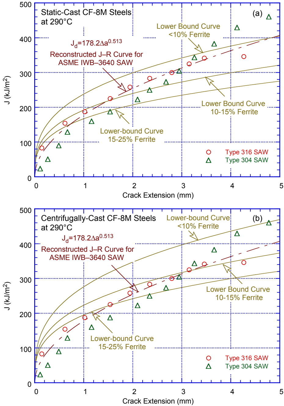
Figure 24. Comparison of the lower-bound fracture toughness J-R curve for thermally aged (a) static-cast and (b) centrifugally-cast CF-8M steels at 290^\circ\text{C} estimated using the NUREG/CR-4513, Rev. 1 expressions, with the fracture toughness of SA welds used to develop ASME Section XI Subsection IWB-3640 evaluations.
