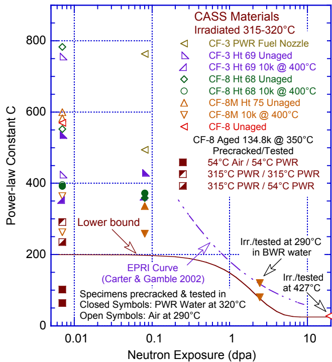
Figure 63. Plots of constant C of the power-law J-R curve as a function of neutron dose for (a) austenitic SS welds, (b) CASS materials, and (c) austenitic SS HAZ. The solid line represents the lower-bound C values proposed in NUREG/CR-7027. The data points plotted at 0.007 dpa are for nonirradiated materials.
