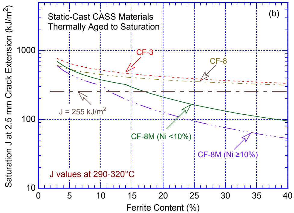
Figure 30. The change in saturation J at 2.5 mm crack extension determined at (a) RT and (b) 290-320°C as a function of ferrite content for static-cast CF-3, CF-8, and CF-8M CASS materials.
