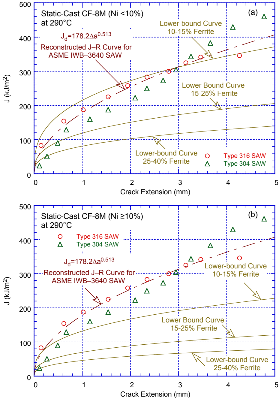
Figure 25. Comparison of the lower-bound fracture toughness J-R curve for thermally aged static-cast CF-8M steels containing (a) <10% Ni and (b) ≥10% Ni at 290°C estimated using the updated expressions presented in this report, with the fracture toughness of SA welds used to develop ASME Section XI Subsection IWB-3640 evaluations.
