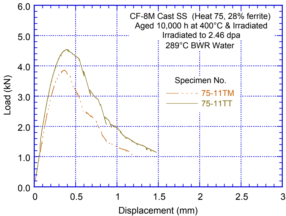
Figure 58. Fracture toughness J-R curves and load vs. loadline displacement curves for thermally aged and irradiated CF-8M steel (Ref. 21).
