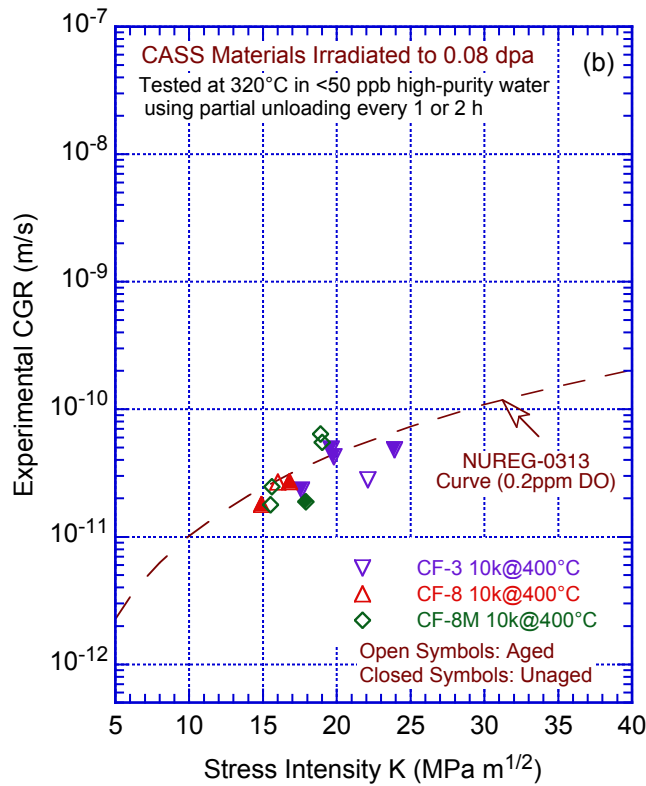
Figure 48. SCC growth rates for aged and unaged (a) Type 316L welds and (b) CASS materials in irradiated or nonirradiated conditions and tested at 289 or 320°C in high-purity water with 300–2,000 or <50 ppb DO (Refs. 20, 88, 105, 135, 136).
