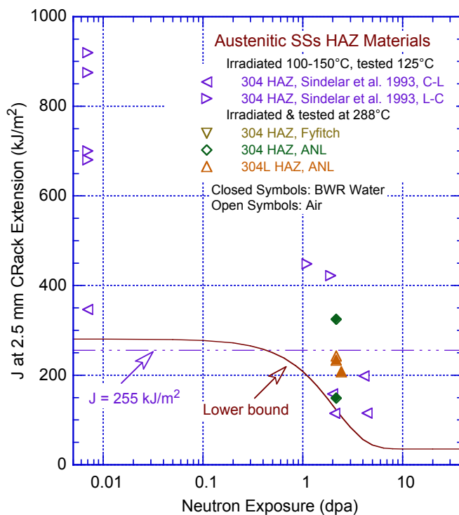
Figure 65. Plots of fracture toughness J_{2.5} values as a function of neutron dose for (a) austenitic SS welds, (b) CASS materials, and (c) austenitic SS HAZ. Solid line represents the lower-bound J_{2.5} values proposed in NUREG/CR-7027. The data points plotted at 0.007 dpa are for nonirradiated materials.
