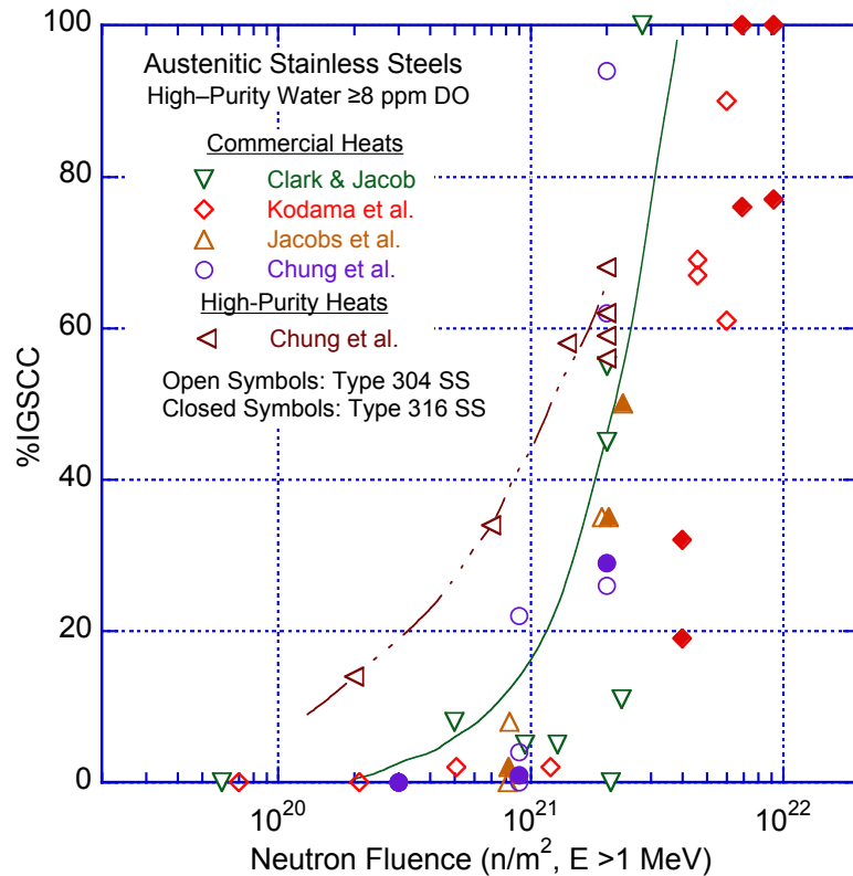
Figure 42. Susceptibility of irradiated austenitic SSs to IGSC as a function of fluence in high-DO water.
