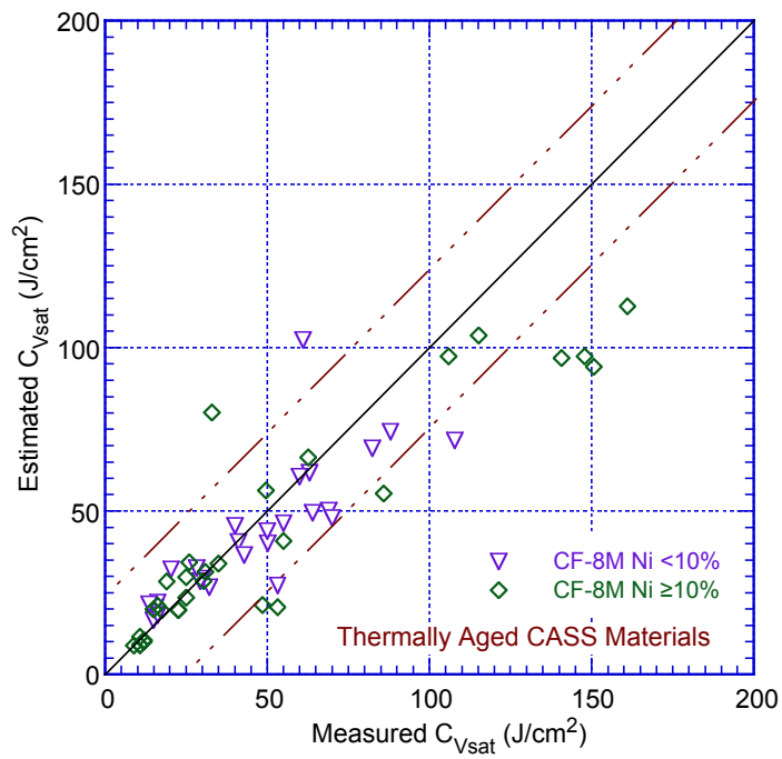
Figure 12. Measured and estimated values of saturation RT Charpy-impact energy for CF-3, CF-8, and CF-8M CASS materials.
