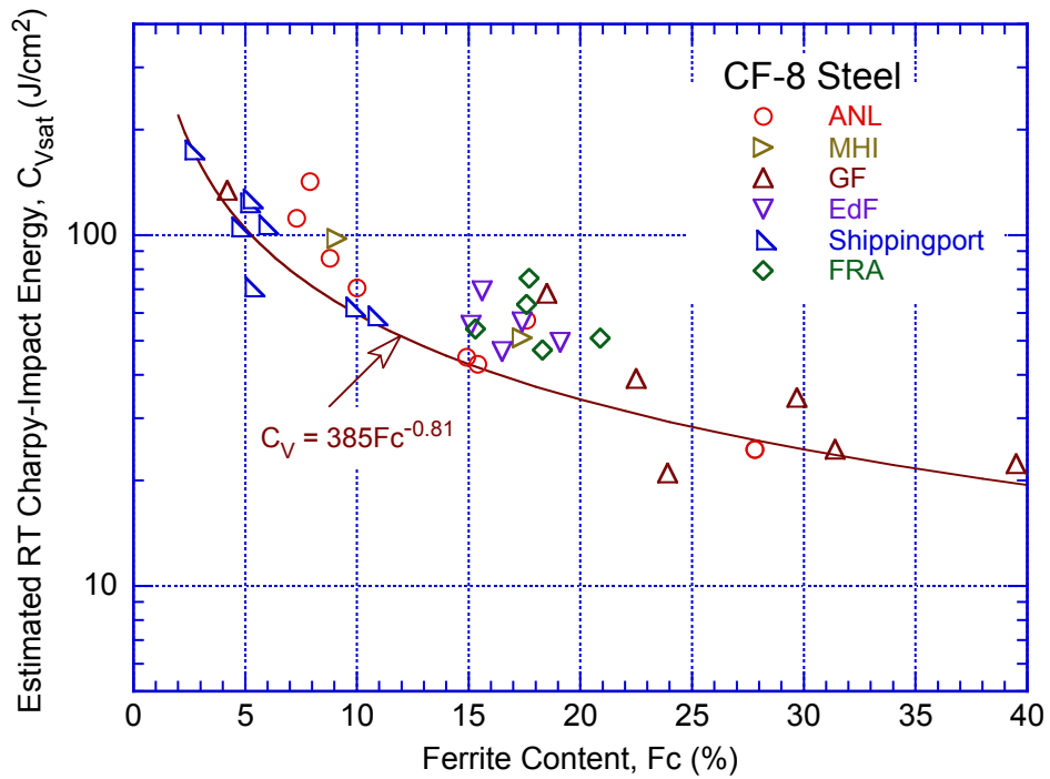
Figure 21. Correlation between saturation RT Charpy-impact energy and ferrite content for CF-3, CF-8, and CF-8M CASS materials.
