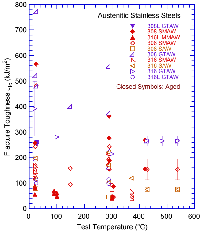
Figure 36. Fracture toughness J_{1c} for unaged and aged stainless steel welds.
