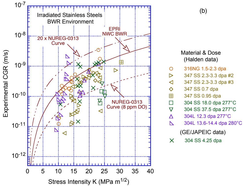
Figure 44. SCC growth rates in NWC BWR environment on austenitic SSs irradiated to 0.75–37.5 dpa (Refs. 20, 26, 128–133).
