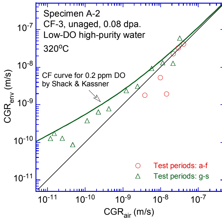
Figure 20. Cyclic CGRs of specimen A-2.
