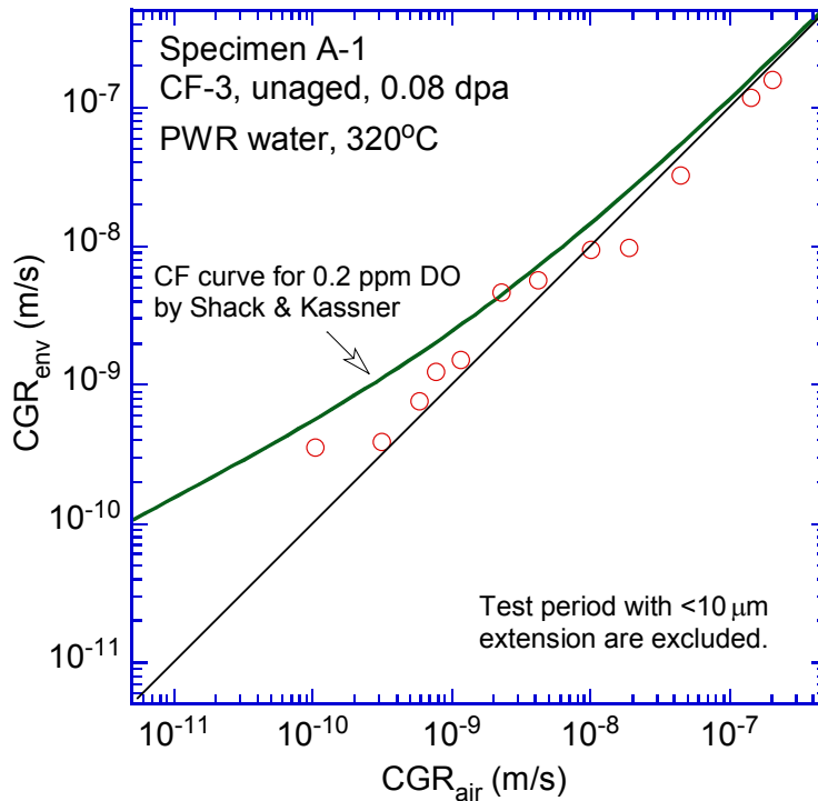
Figure 14. Cyclic CGRs of specimen A-1.
