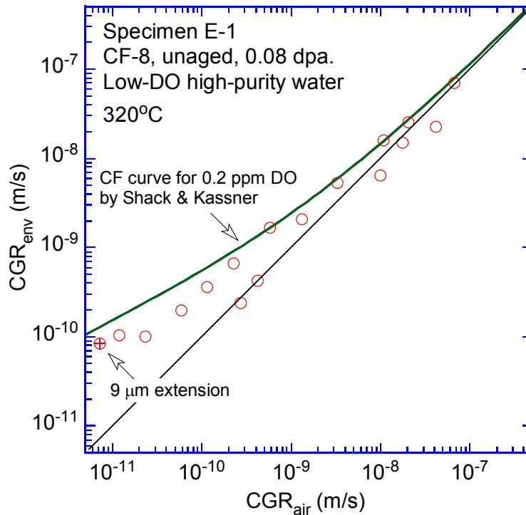
Figure 52. Cyclic CGRs of specimen E-1.
