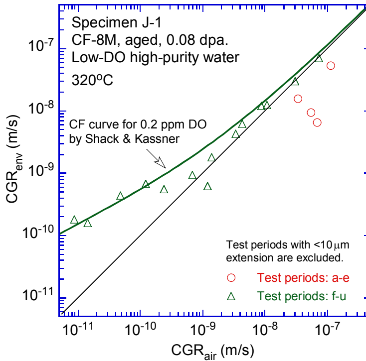
Figure 86. Cyclic CGRs of specimen J-1.
