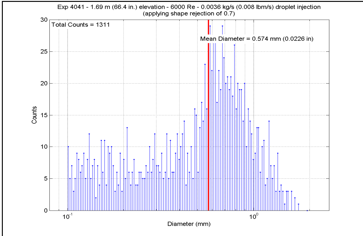
Figure A-610: Droplet Measurements at 1.687 m (66.4 in.) Elevation for Experiment 4041I
