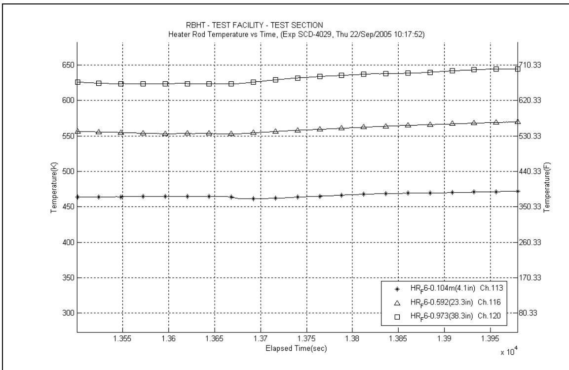
Figure A-107: Heater Rod F6 Temperatures for Experiment 4029F
