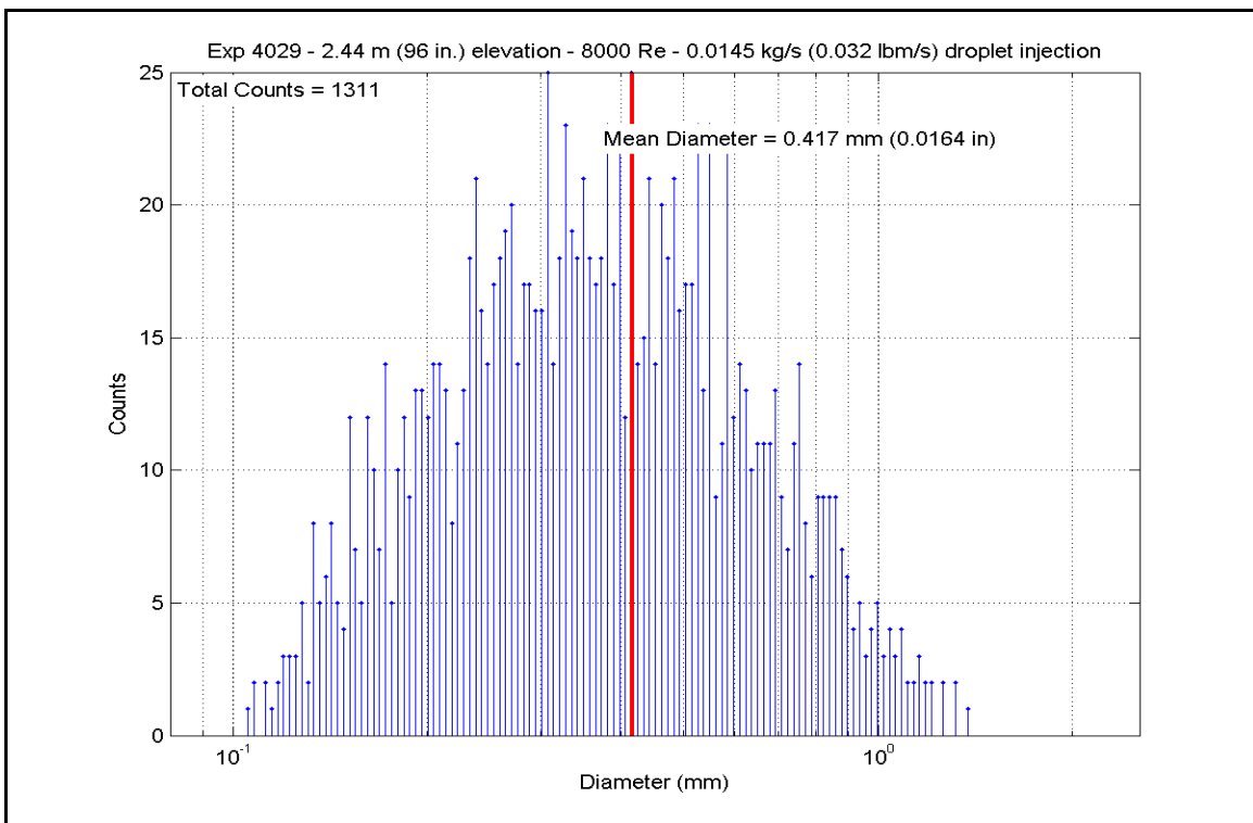
Figure A-95: Droplet Measurements at 2.438 m (96 in.) Elevation for Experiment 4029D
