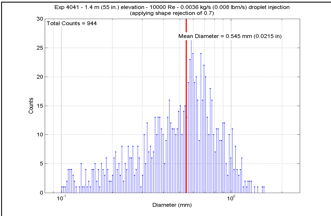
Figure A-448: Droplet Measurements at 1.397 m (55 in.) Elevation for Experiment 4041A
