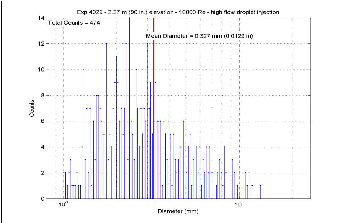
Figure A-35: Droplet Measurements at 2.286 m (90 in.) Elevation for Experiment 4029A
