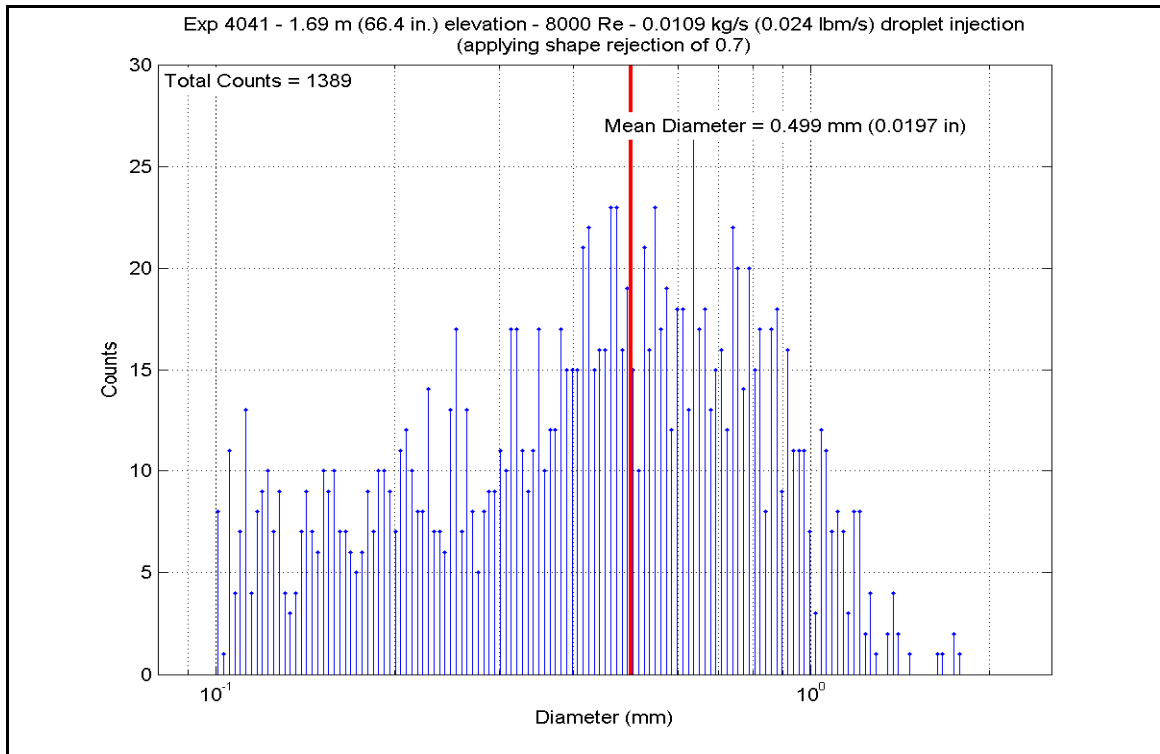
Figure A-572: Droplet Measurements at 1.687 m (66.4 in.) Elevation for Experiment 4041G
