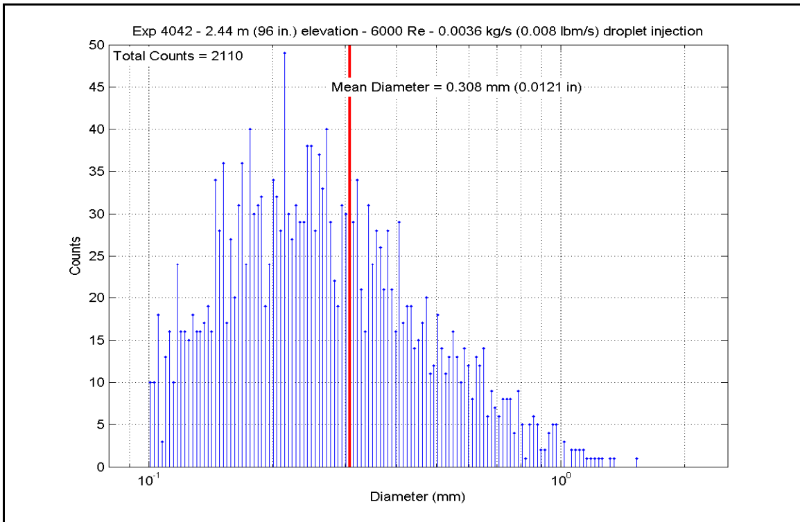
Figure A-672: Droplet Measurements at 2.438 m (96 in.) Elevation for Experiment 4042A
