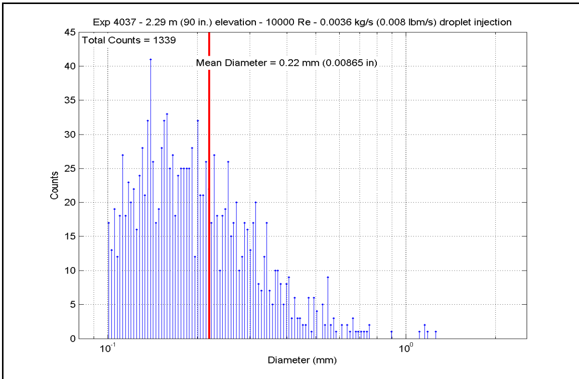
Figure A-324: Droplet Measurements at 2.286 m (90 in.) Elevation for Experiment 4037A
