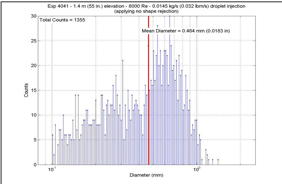
Figure A-589: Droplet Measurements at 1.397 m (55 in.) Elevation for Experiment 4041H
