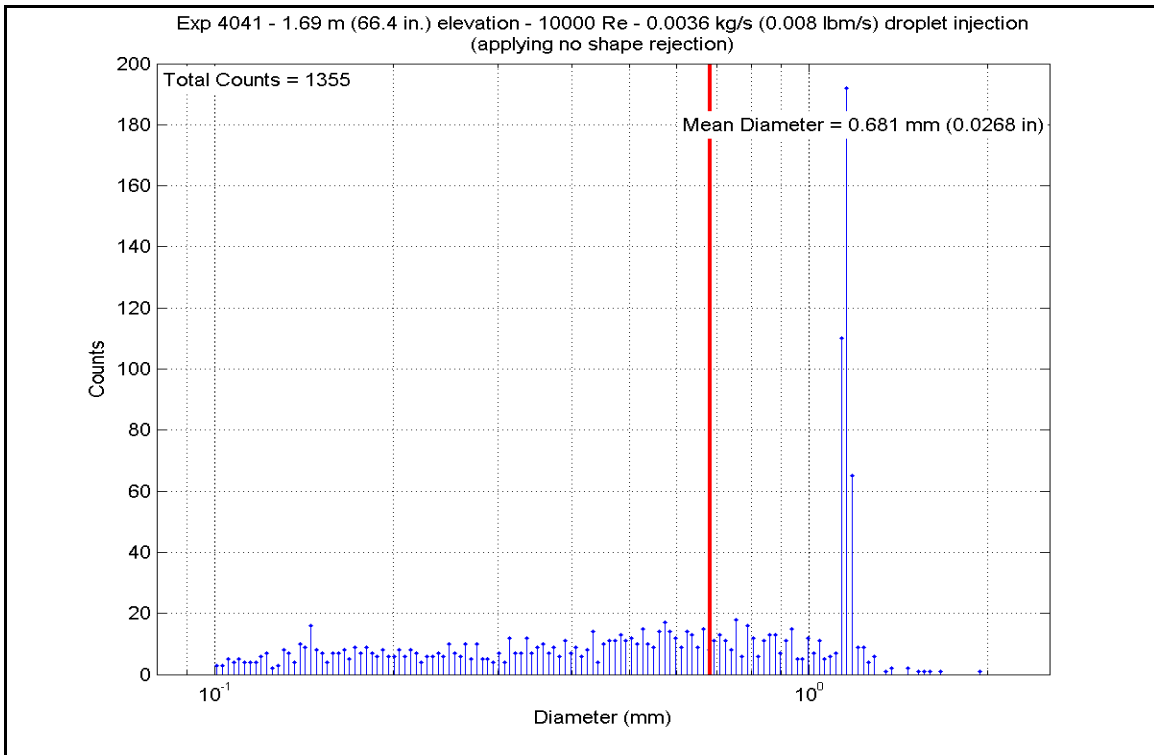
FFigure A-457: Droplet Measurements at 1.687 m (66.4 in.) Elevation for Experiment 4041A
