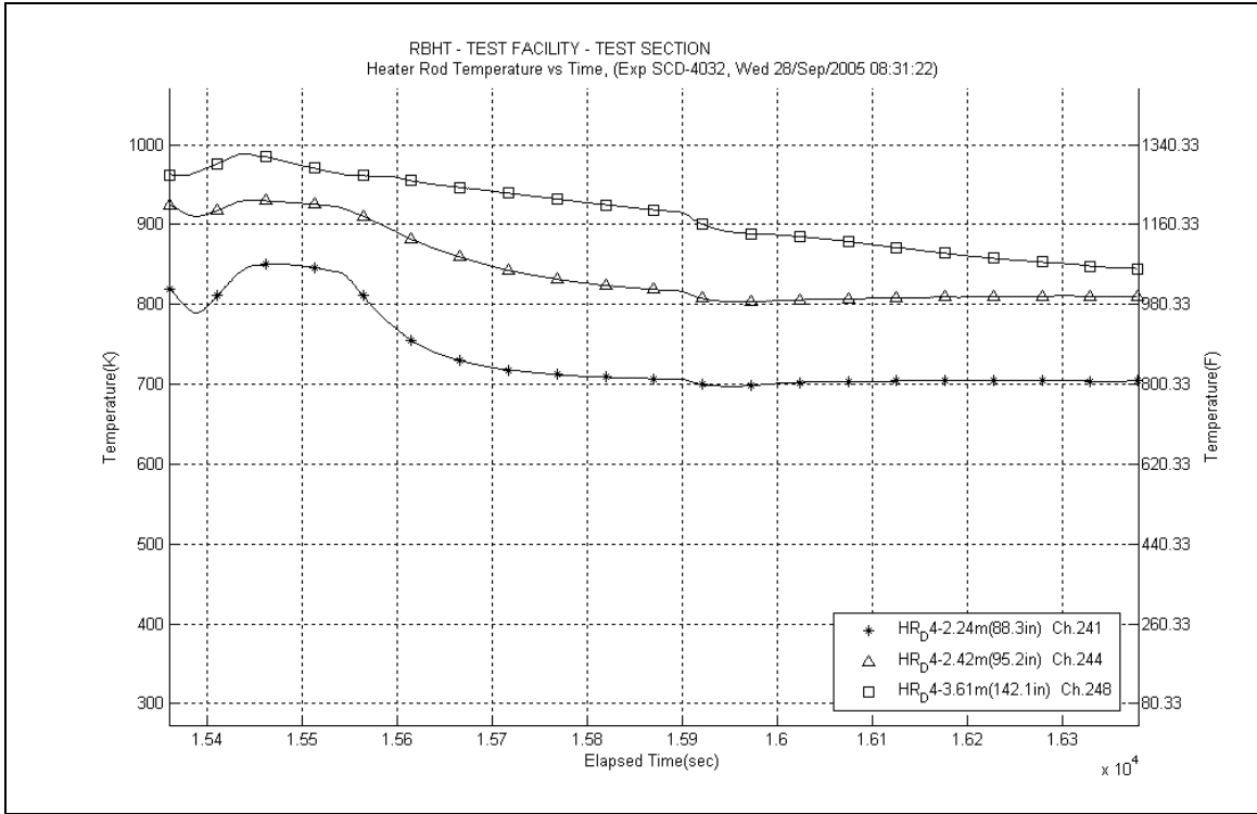
Figure A-192: Heater Rod D4 Temperatures for Experiment 4032F
