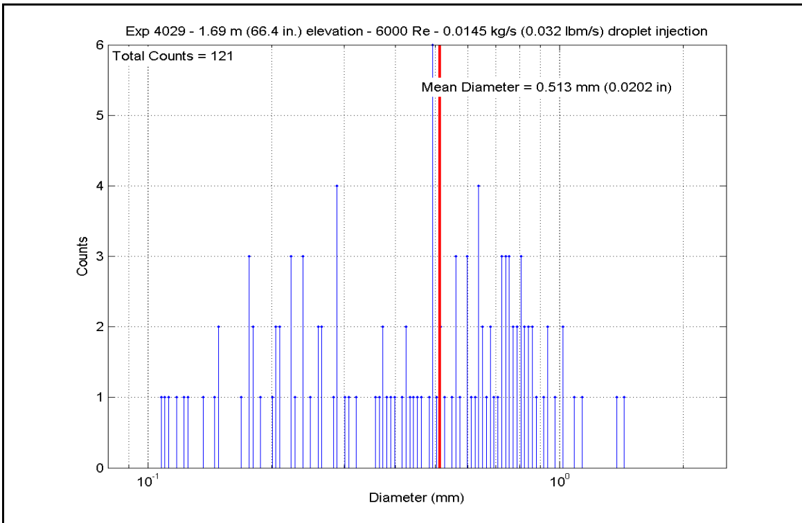
Figure A-109: Droplet Measurements at 1.687 m (66.4 in.) Elevation for Experiment 4029F
