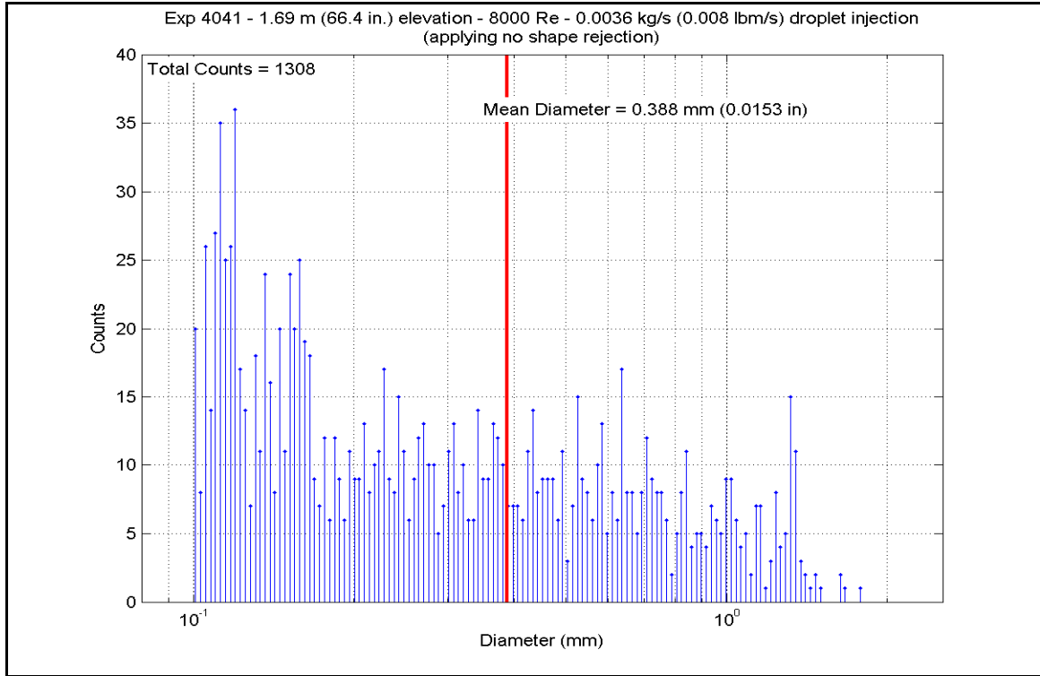
Figure A-533: Droplet Measurements at 1.687 m (66.4 in.) Elevation for Experiment 4041E
