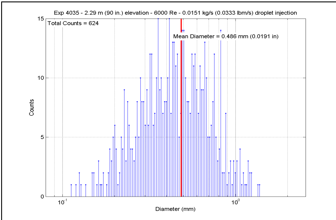
Figure A-306: Droplet Measurements at 2.286 m (90 in.) Elevation for Experiment 4035F
