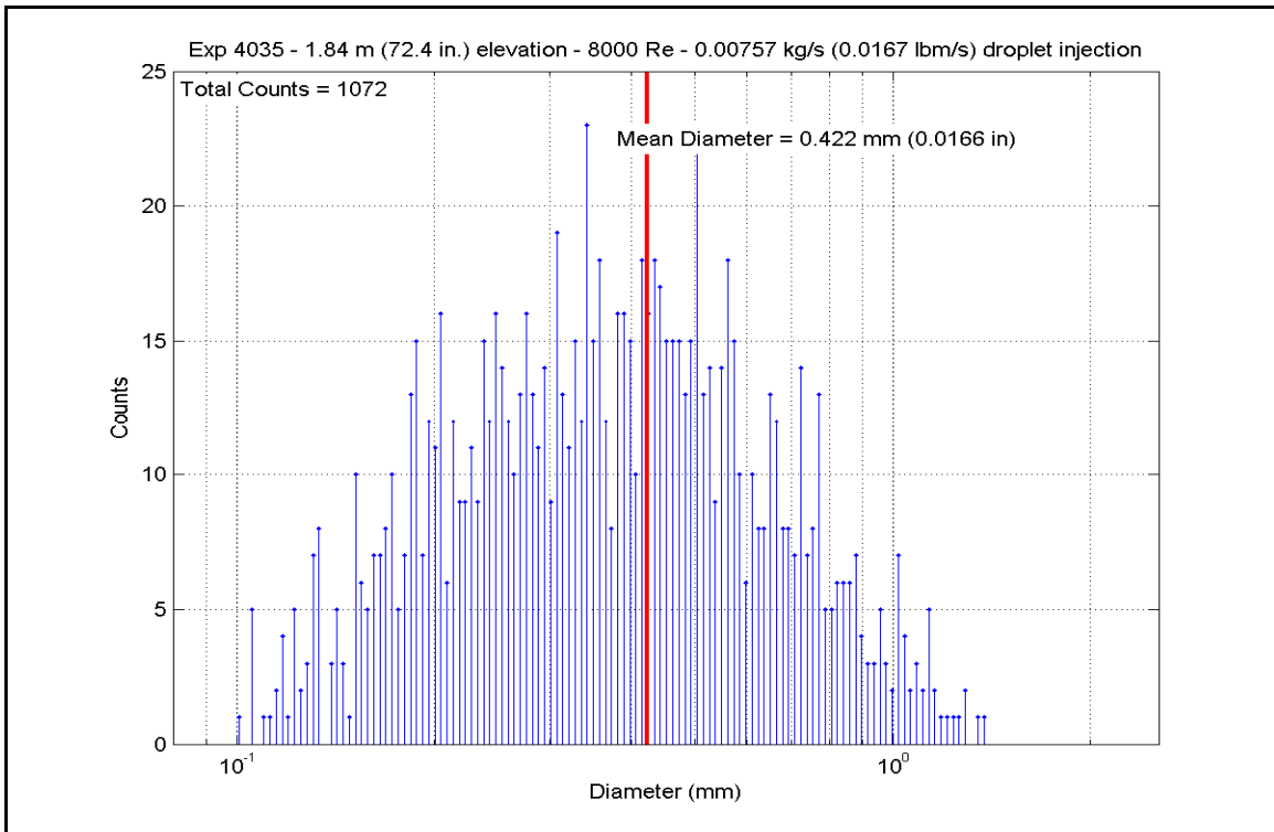
Figure A-251: Droplet Measurements at 1.839 m (72.4 in.) Elevation for Experiment 4035C
