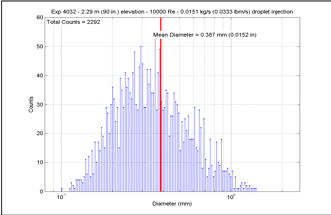
Figure A-145: Droplet Measurements at 2.286 m (90 in.) Elevation for Experiment 4032B
