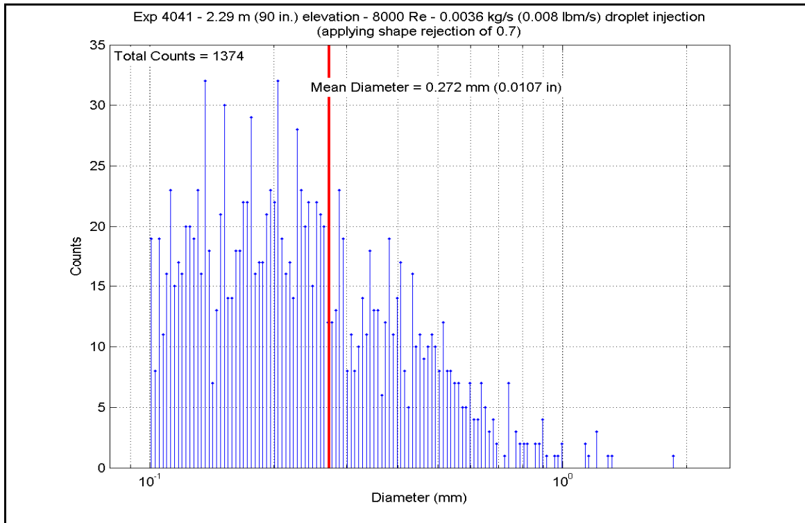
Figure A-536: Droplet Measurements at 2.286 m (90 in.) Elevation for Experiment 4041E
