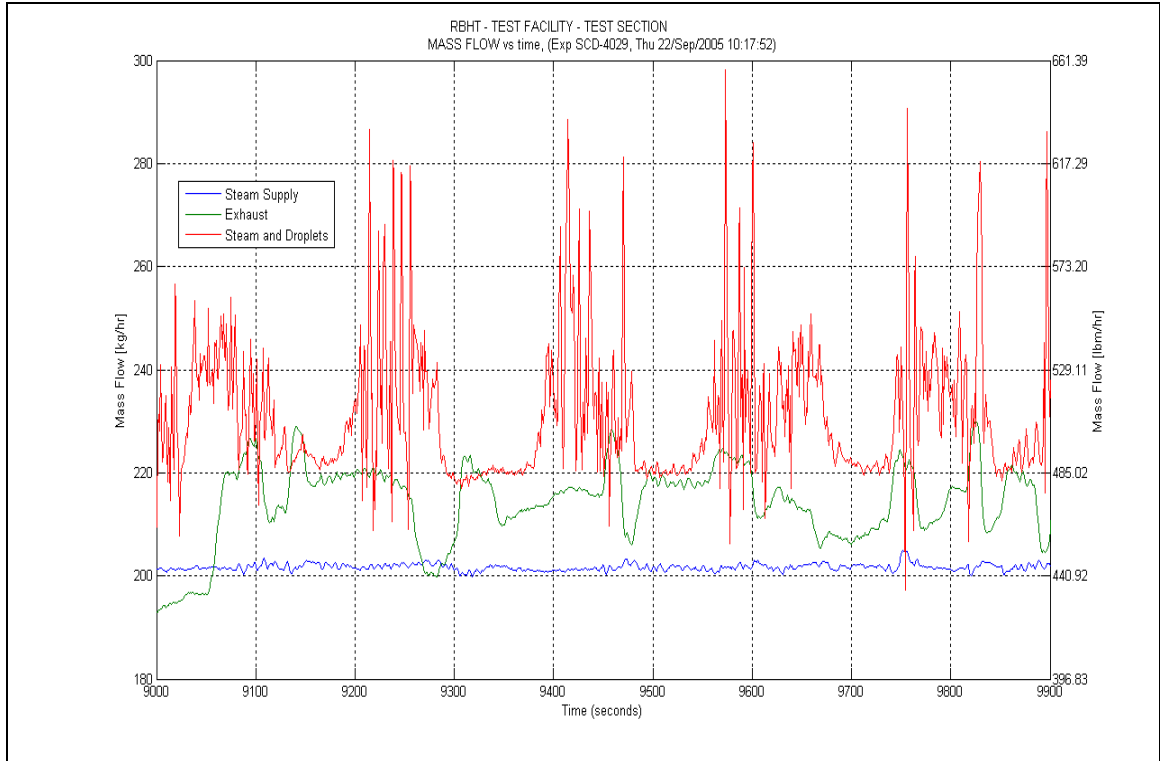
Figure A-27: Mass Flow for Experiment 4029A
