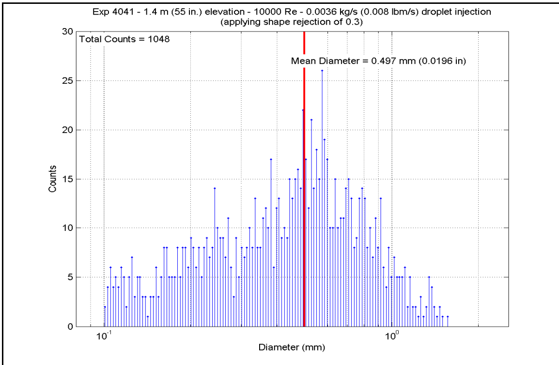
Figure A-452: Droplet Measurements at 1.397 m (55 in.) Elevation for Experiment 4041A
