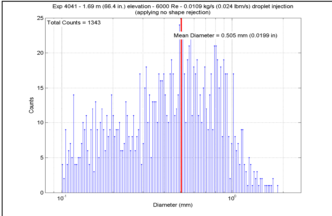
Figure A-648: Droplet Measurements at 1.687 m (66.4 in.) Elevation for Experiment 4041K
