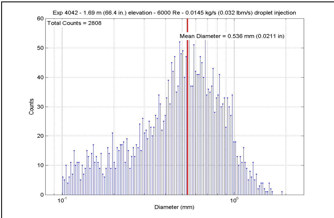
Figure A-723: Droplet Measurements at 1.687 m (66.4 in.) Elevation for Experiment 4042D
