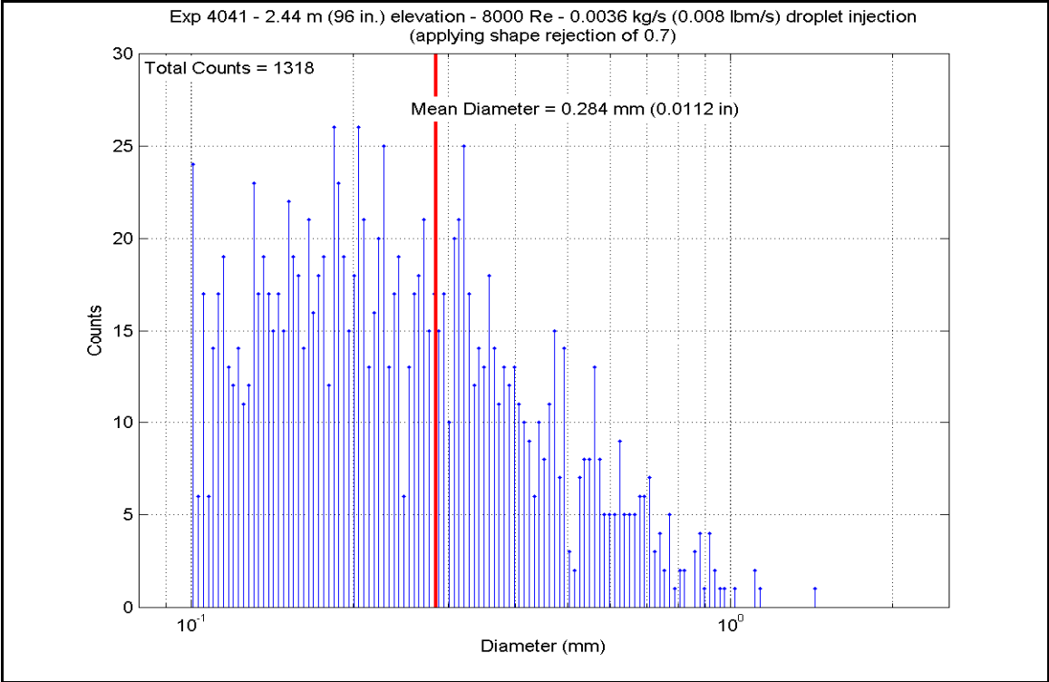
Figure A-537: Droplet Measurements at 2.438 m (96 in.) Elevation for Experiment 4041E
