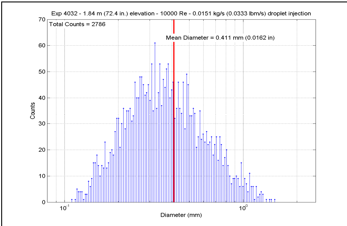
Figure A-144: Droplet Measurements at 1.839 m (72.4 in.) Elevation for Experiment 4032B
