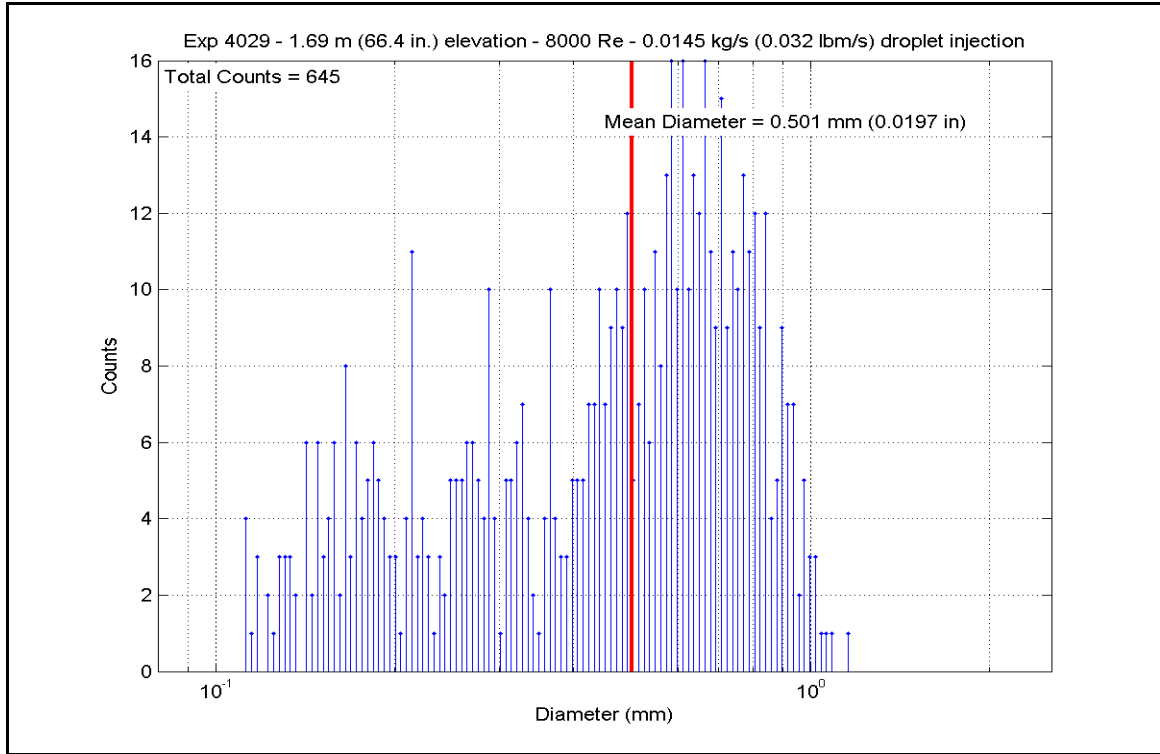
Figure A-92: Droplet Measurements at 1.687 m (66.4 in.) Elevation for Experiment 4029D
