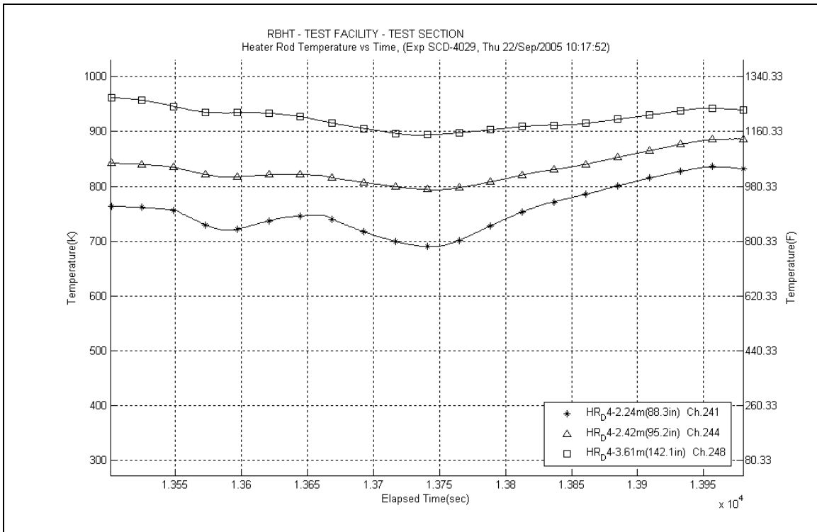
Figure A-106 Heater Rod D4 Temperatures for Experiment 4029F
