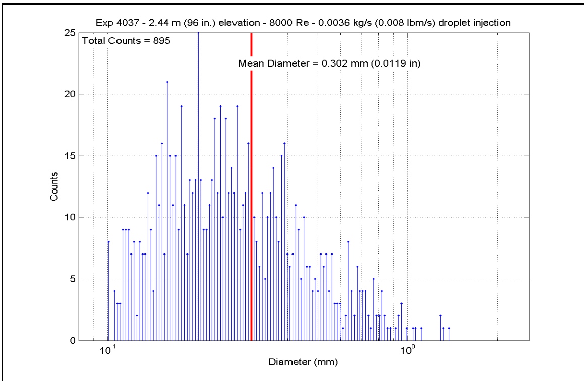
Figure A-380: Droplet Measurements at 2.438 m (96 in.) Elevation for Experiment 4037D
