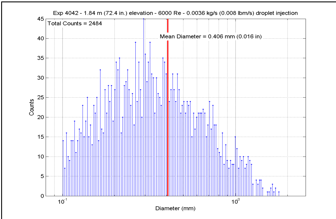
Figure A-670: Droplet Measurements at 1.839 m (72.4 in.) Elevation for Experiment 4042A
