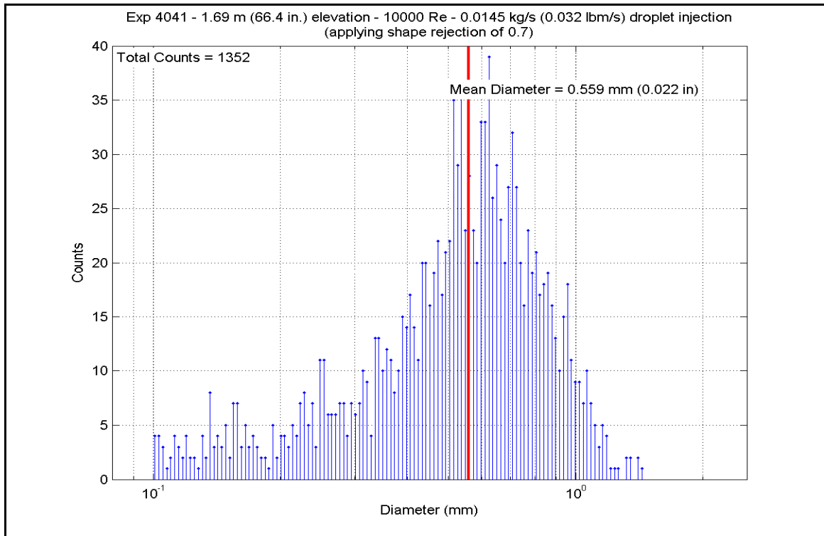
Figure A-515: Droplet Measurements at 1.687 m (66.4 in.) Elevation for Experiment 4041D
