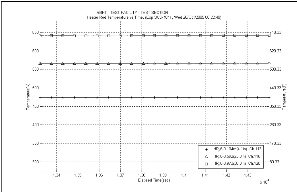
Figure A-446: Heater Rod F6 Temperatures for Experiment 401A
