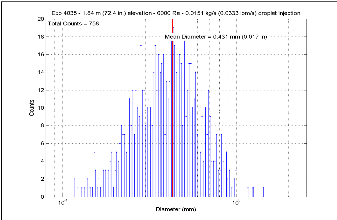
Figure A-305: Droplet Measurements at 1.839 m (72.4 in.) Elevation for Experiment 4035F
