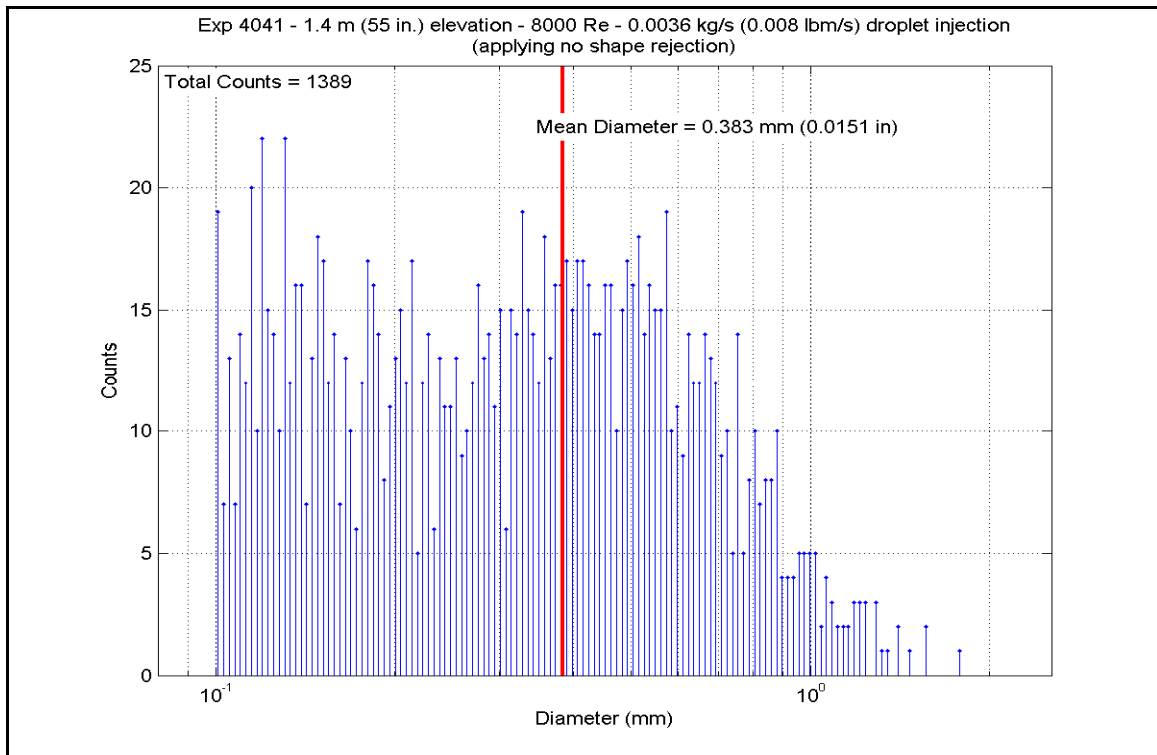
Figure A-532: Droplet Measurements at 1.397 m (55 in.) Elevation for Experiment 4041E
