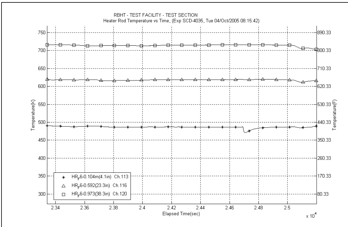
Figure A-301: Heater Rod F6 Temperatures for Experiment 4035F
