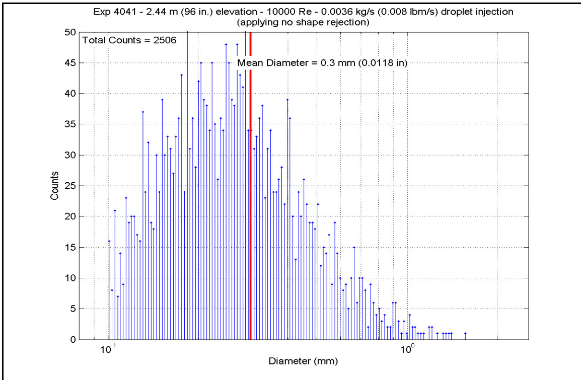
Figure A-455: Droplet Measurements at 2.438 m (96 in.) Elevation for Experiment 4041A
