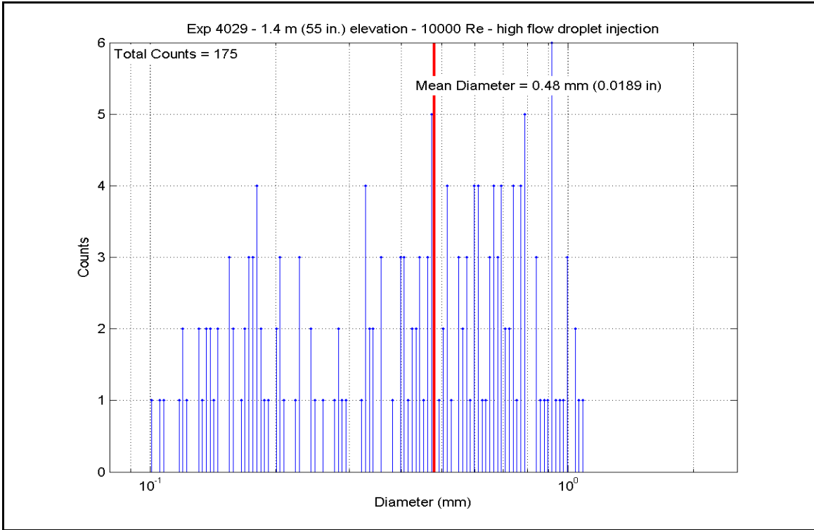
Figure A-37: Droplet Measurements at 1.397 m (55 in.) Elevation for Experiment 4029A
