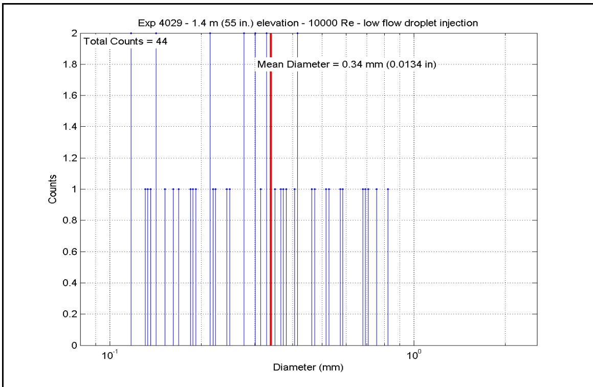
Figure A-28: Droplet Measurements at 1.397 m (55 in.) Elevation for Experiment 4029A
