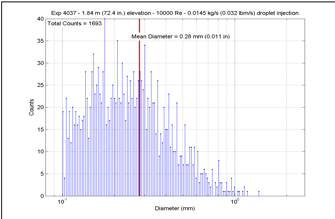
Figure A-359: Droplet Measurements at 1.839 m (72.4 in.) Elevation for Experiment 4037C
