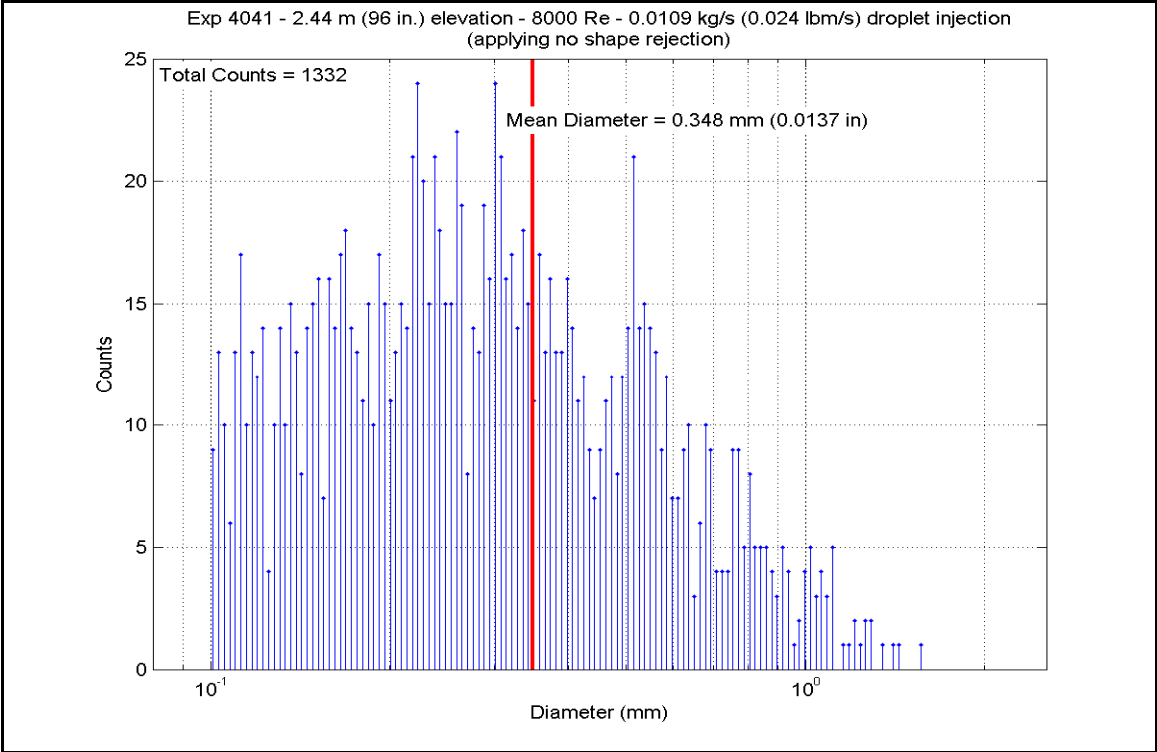
Figure A-575: Droplet Measurements at 2.438 m (96 in.) Elevation for Experiment 4041G
