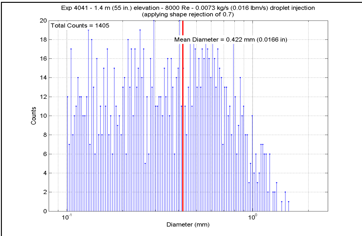
Figure A-551: Droplet Measurements at 1.397 m (55 in.) Elevation for Experiment 4041F
