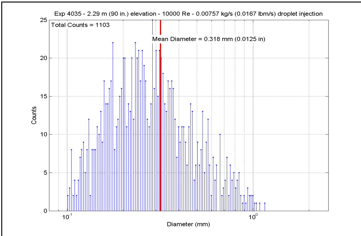
Figure A-216: Droplet Measurements at 2.286 m (90 in.) Elevation for Experiment 4035A
