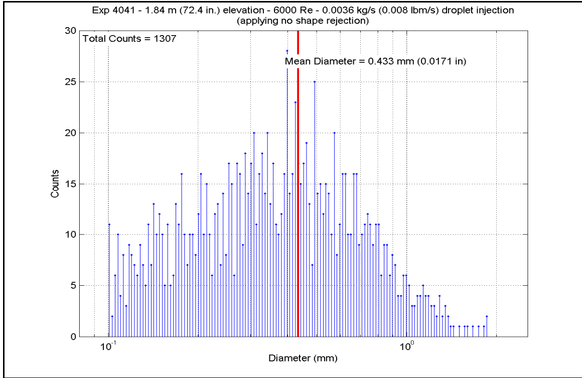
Figure A-611: Droplet Measurements at 1.839 m (72.4 in.) Elevation for Experiment 4041
