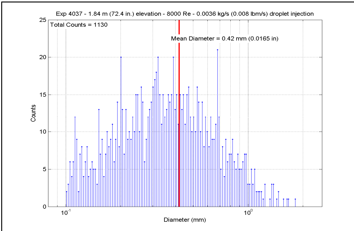
Figure A-378: Droplet Measurements at 1.839 m (72.4 in.) Elevation for Experiment 4037D
