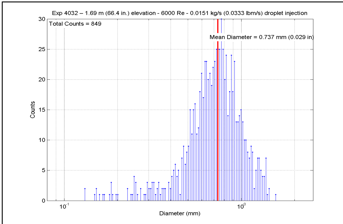
Figure A-196: Droplet Measurements at 1.687 m (66.4 in.) Elevation for Experiment 4032F
