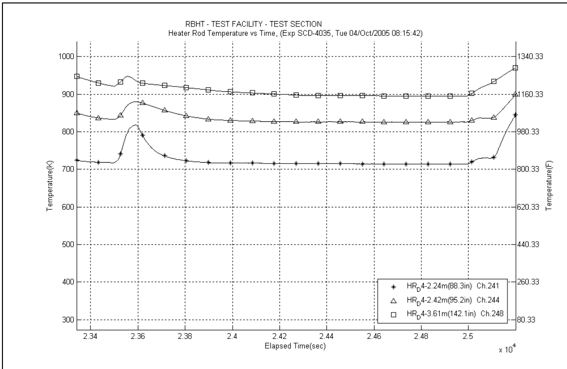
Figure A-300: Heater Rod D4 Temperatures for Experiment 4035F
