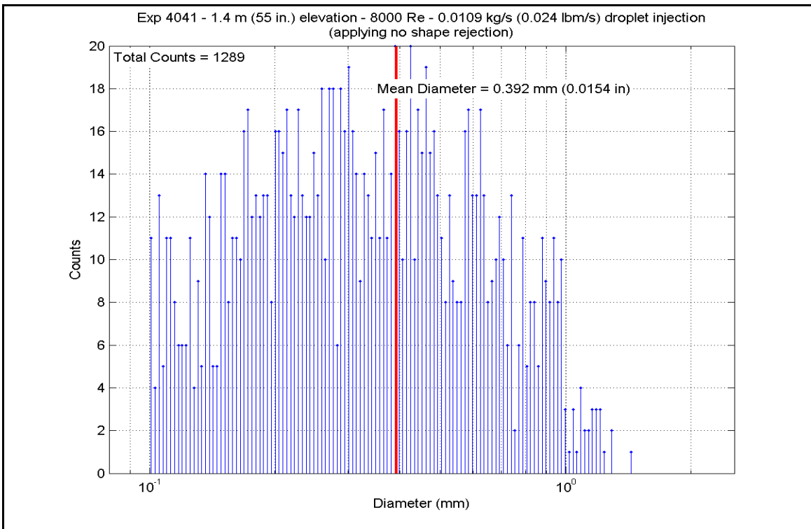
Figure A-570: Droplet Measurements at 1.397 m (55 in.) Elevation for Experiment 4041G
