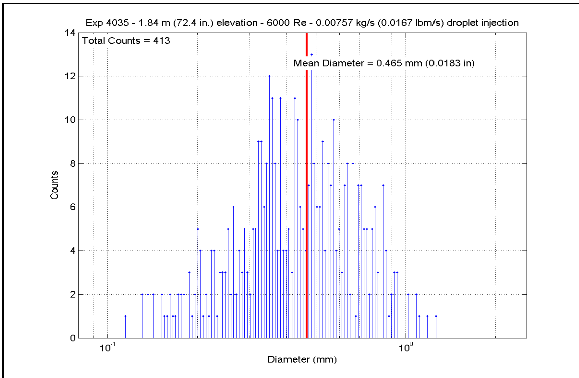
Figure A-287: Droplet Measurements at 1.839 m (72.4 in.) Elevation for Experiment 4035E
