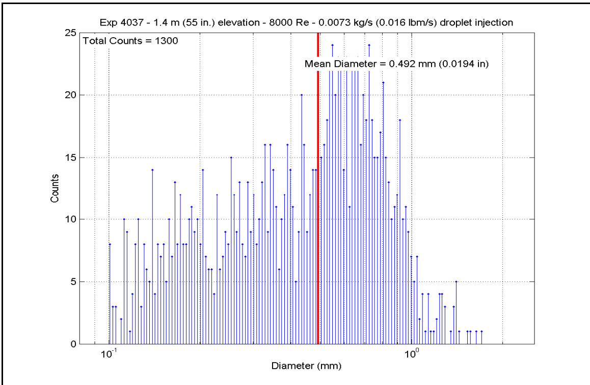
Figure A-394: Droplet Measurements at 1.397 m (55 in.) Elevation for Experiment 4037E
