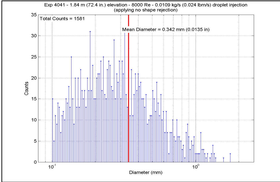
Figure A-573: Droplet Measurements at 1.839 m (72.4 in.) Elevation for Experiment 4041G
