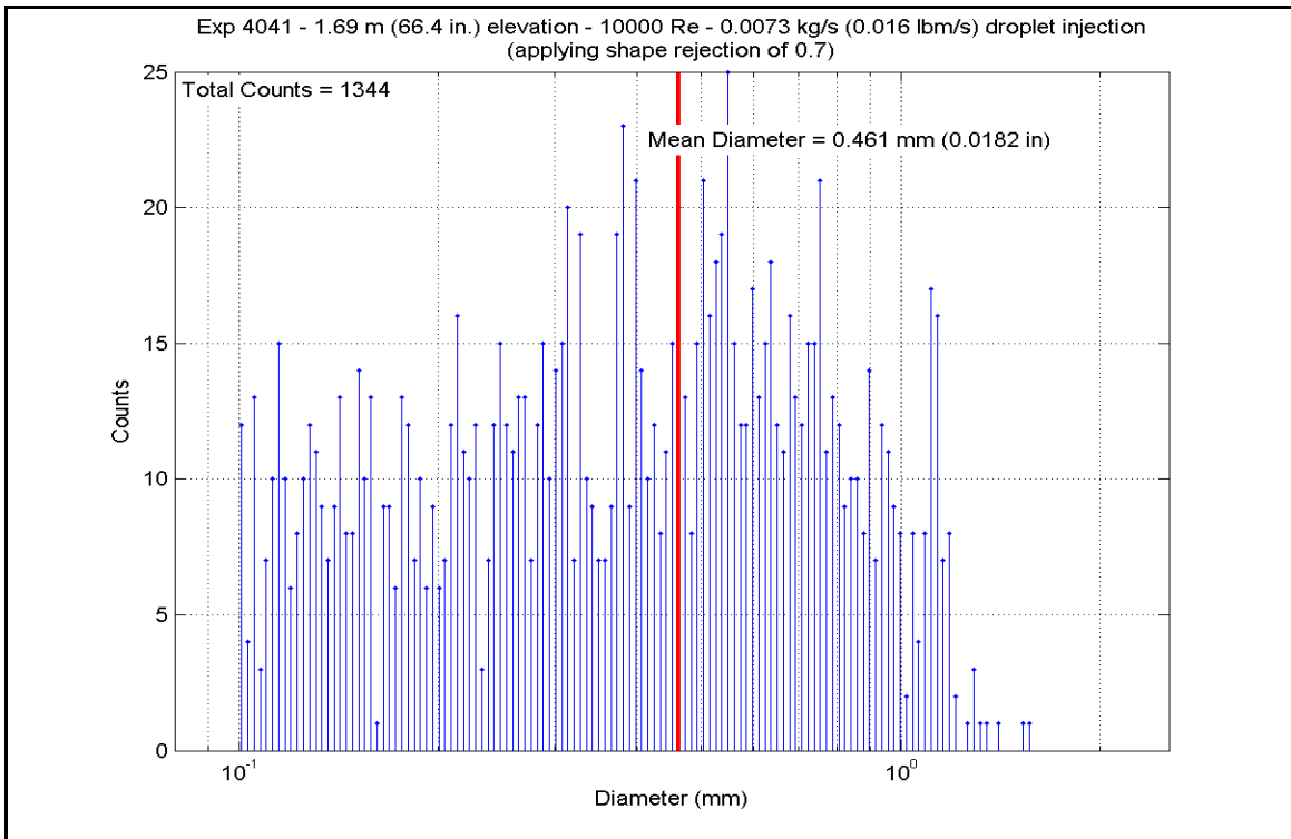
Figure A-477: Droplet Measurements at 1.687 m (66.4 in.) Elevation for Experiment 4041B
