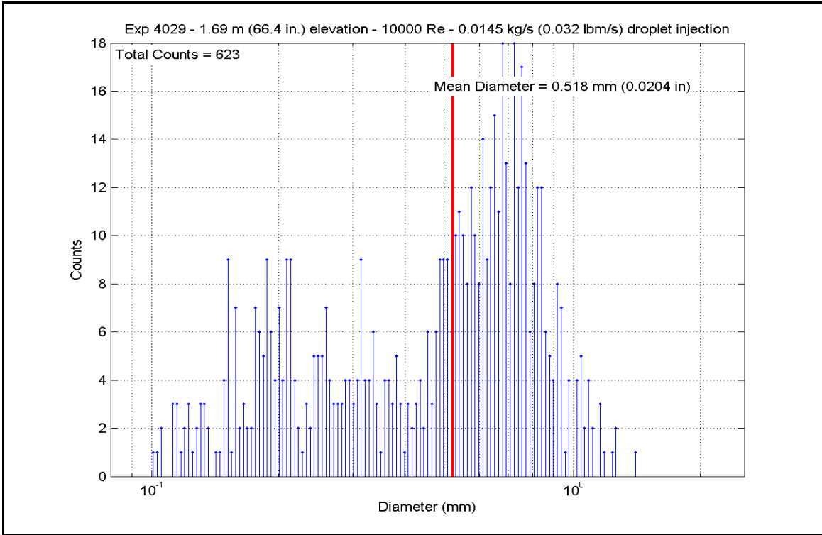
Figure A-56: Droplet Measurements at 1.687 m (66.4 in.) Elevation for Experiment 4029B
