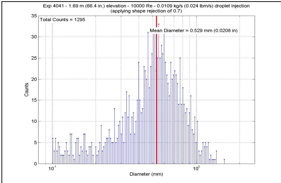
Figure A-496: Droplet Measurements at 1.687 m (66.4 in.) Elevation for Experiment 4041C
