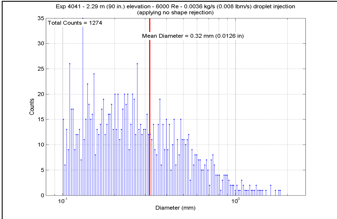
Figure A-612: Droplet Measurements at 2.286 m (90 in.) Elevation for Experiment 4041
