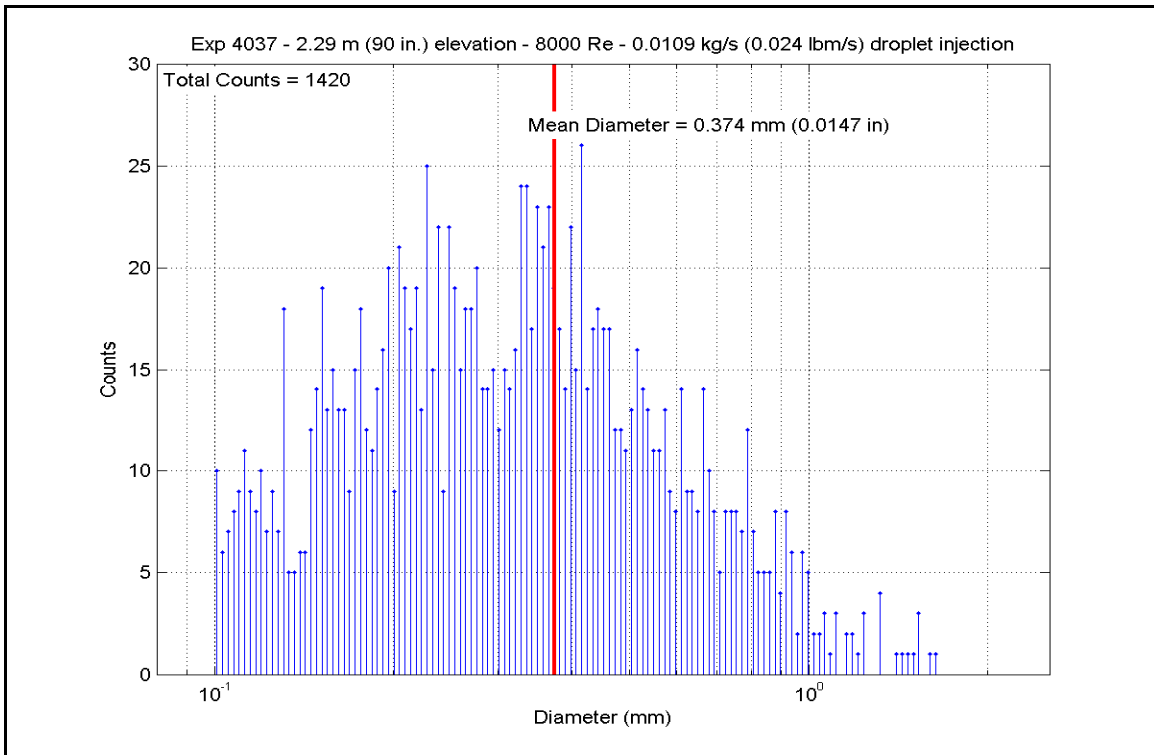
Figure A-415: Droplet Measurements at 2.286 m (90 in.) Elevation for Experiment 4037F
