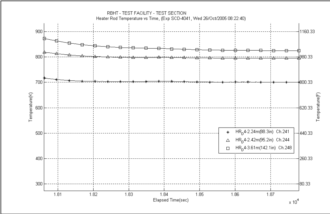
Figure A-491: Heater Rod D4 Temperatures for Experiment 401C
