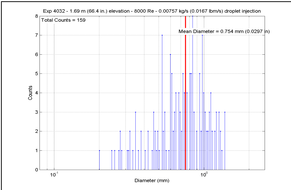
Figure A-161: Droplet Measurements at 1.687 m (66.4 in.) Elevation for Experiment 4032C
