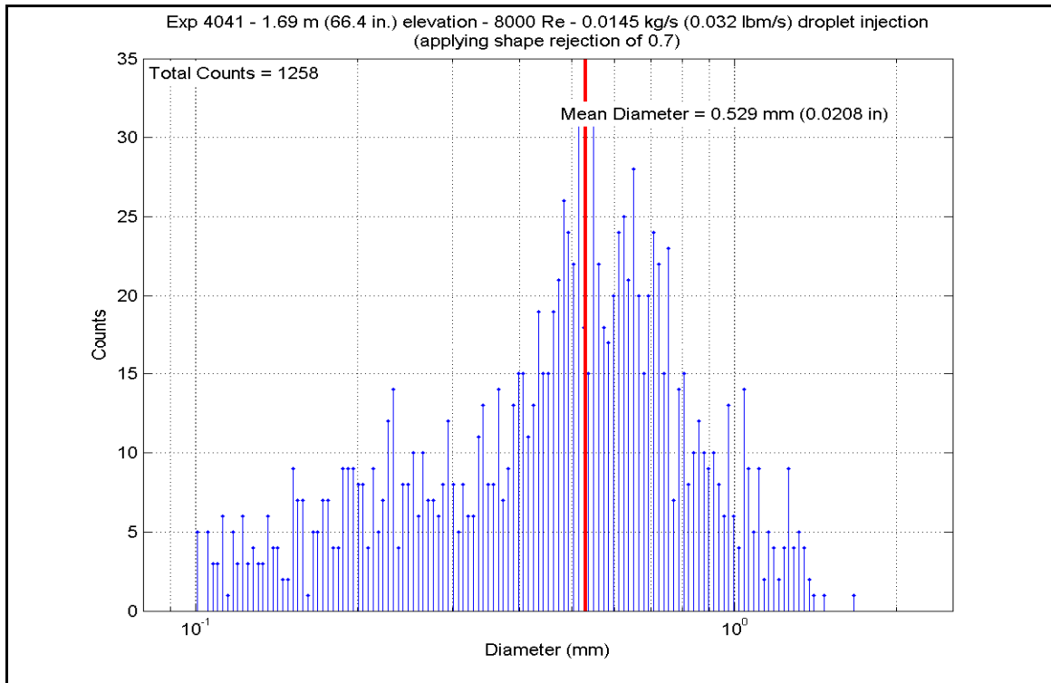
Figure A-591: Droplet Measurements at 1.687 m (66.4 in.) Elevation for Experiment 4041H
