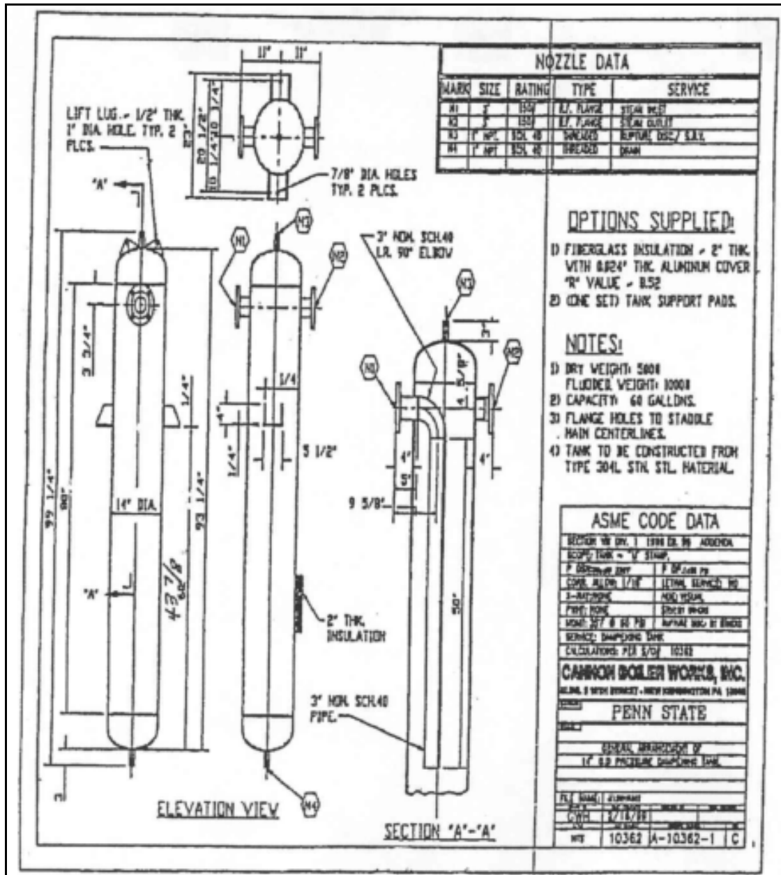
Figure 2-19: Pressure Oscillation Damping Tank
