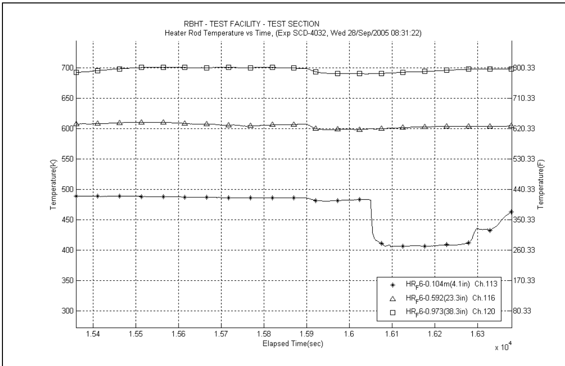
Figure A-193: Heater Rod F6 Temperatures for Experiment 4032F
