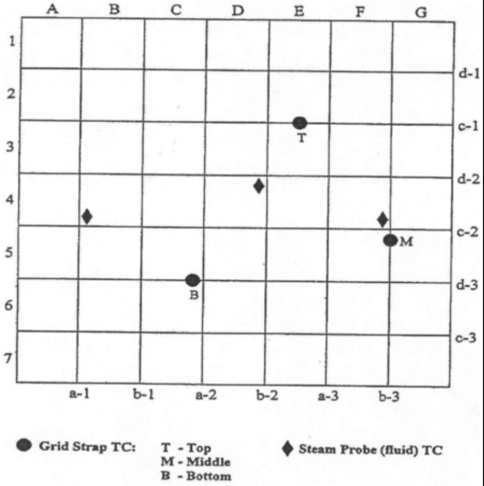
Figure 2-34: Grid No. 6 Instrumentation
