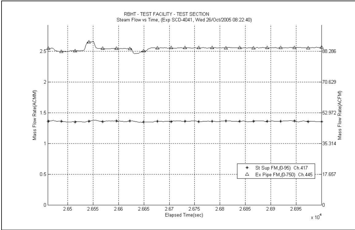
Figure A-595: Inlet and Exhaust Steam Flow Rates for Experiment 40411
