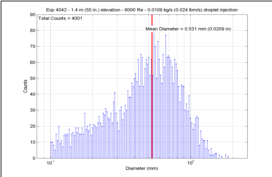
Figure A-704: Droplet Measurements at 1.397 m (55 in.) Elevation for Experiment 4042C
