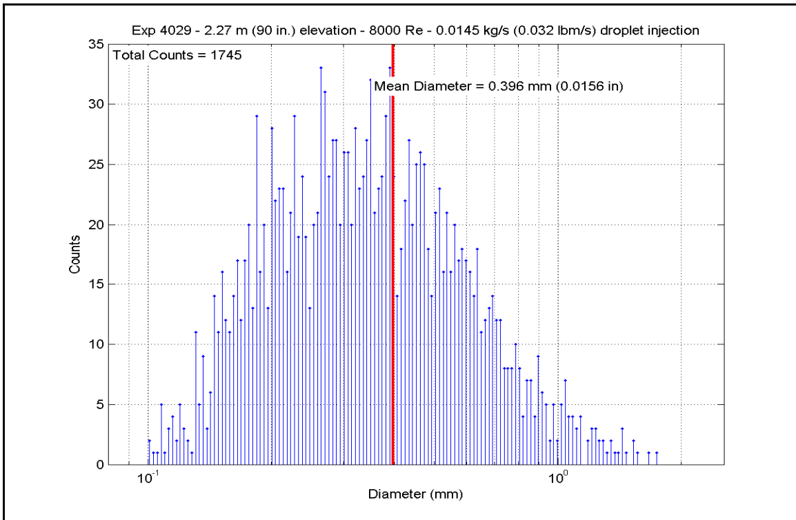
Figure A-94: Droplet Measurements at 2.286 m (90 in.) Elevation for Experiment 4029D
