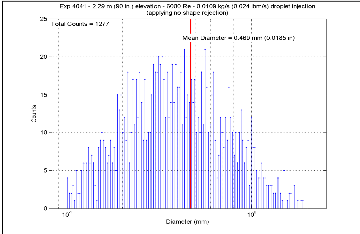
Figure A-651: Droplet Measurements at 2.286 m (90 in.) Elevation for Experiment 4041K
