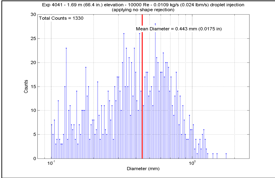
Figure A-495: Droplet Measurements at 1.687 m (66.4 in.) Elevation for Experiment 4041C
