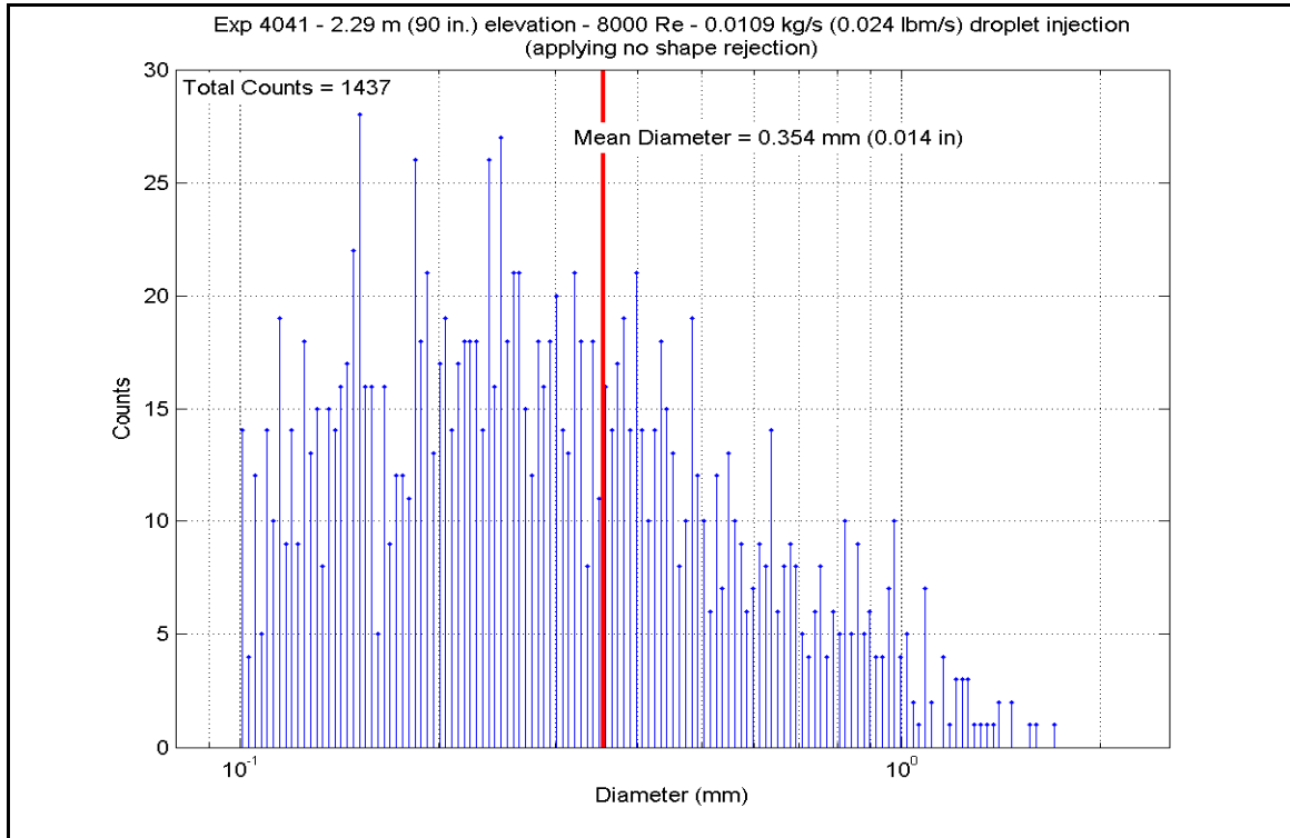
Figure A-574: Droplet Measurements at 2.286 m (90 in.) Elevation for Experiment 4041G
