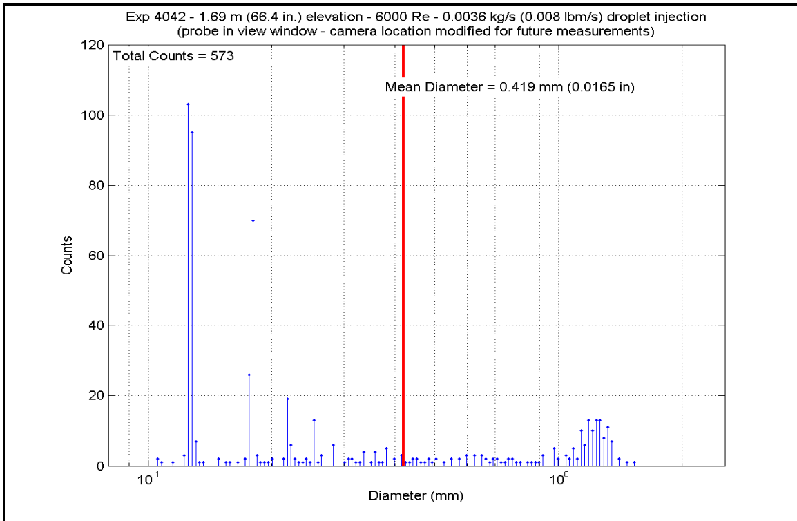
Figure A-668: Droplet Measurements at 1.687 m (66.4 in.) Elevation for Experiment 4042A
