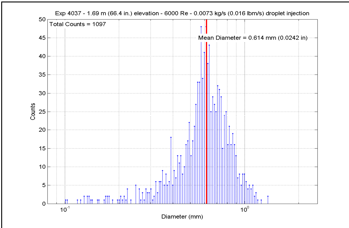
Figure A-431: Droplet Measurements at 1.687 m (66.4 in.) Elevation for Experiment 4037H
