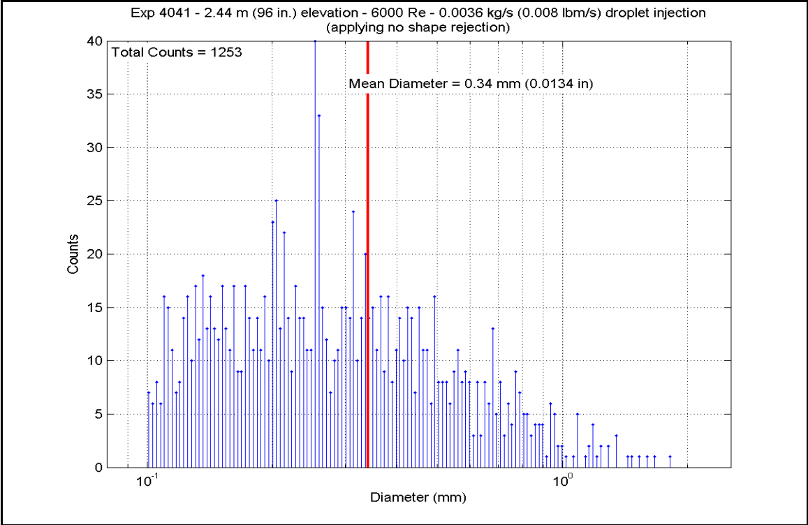
Figure A-613: Droplet Measurements at 2.438 m (96 in.) Elevation for Experiment 40411
