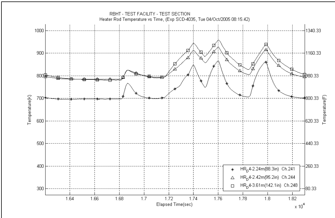
Figure A-228: Heater Rod D4 Temperatures for Experiment 4035B
