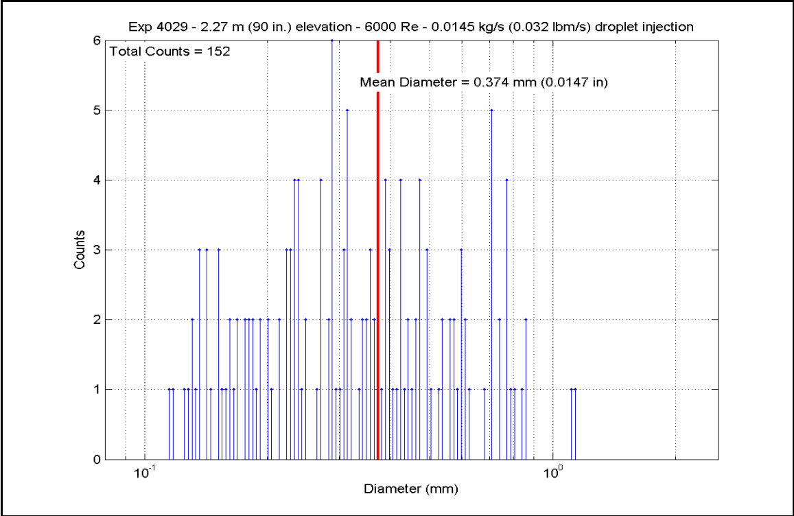
Figure A-110: Droplet Measurements at 2.286 m (90 in.) Elevation for Experiment 4029F
