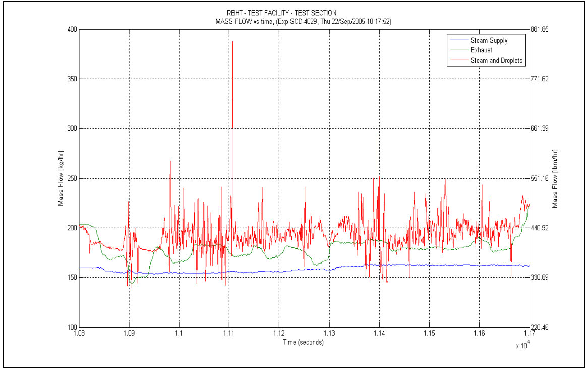
Figure A-72: Mass Flow for Experiment 4029C
