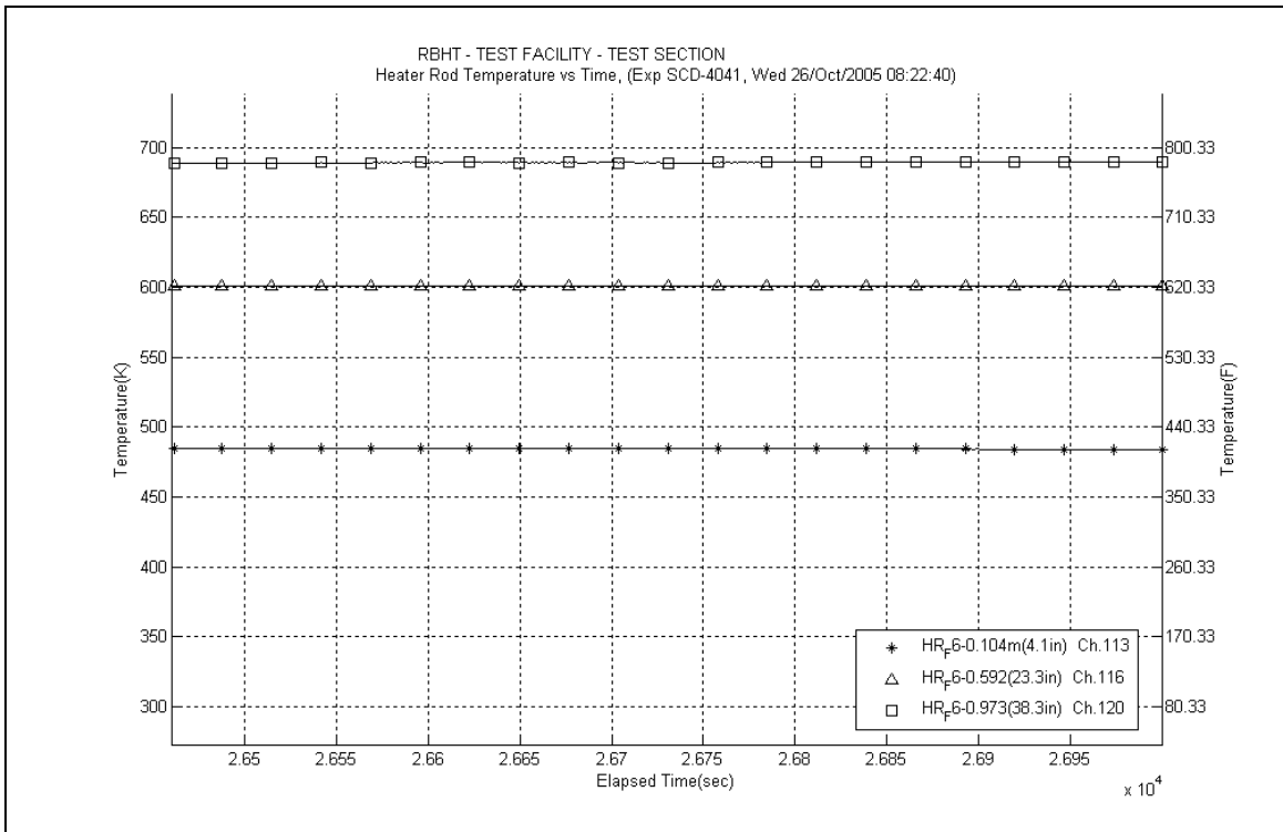
Figure A-606: Heater Rod F6 Temperatures for Experiment 40411
