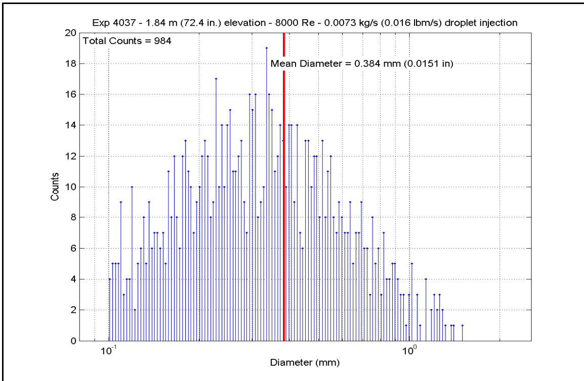
Figure A-396: Droplet Measurements at 1.839 m (72.4 in.) Elevation for Experiment 4037E
