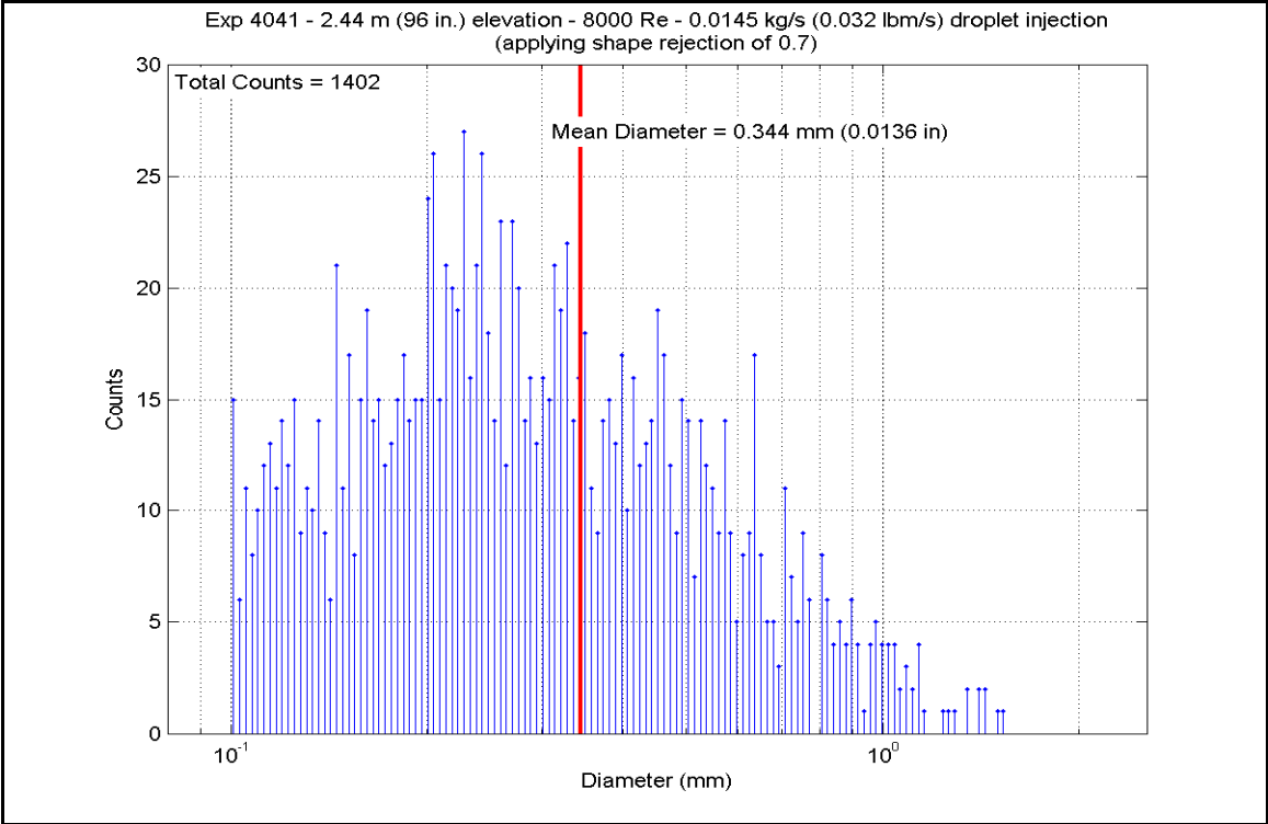
Figure A-594: Droplet Measurements at 2.438 m (96 in.) Elevation for Experiment 4041H
