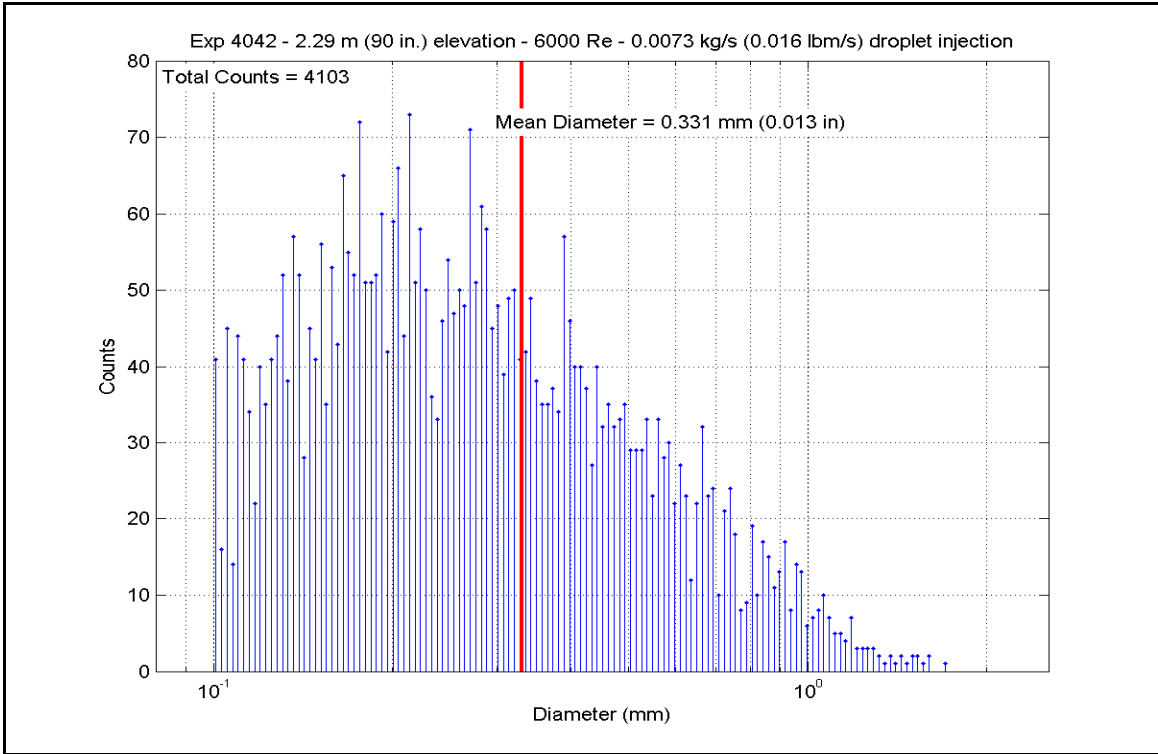
Figure A-689: Droplet Measurements at 2.286 m (90 in.) Elevation for Experiment 4042B
