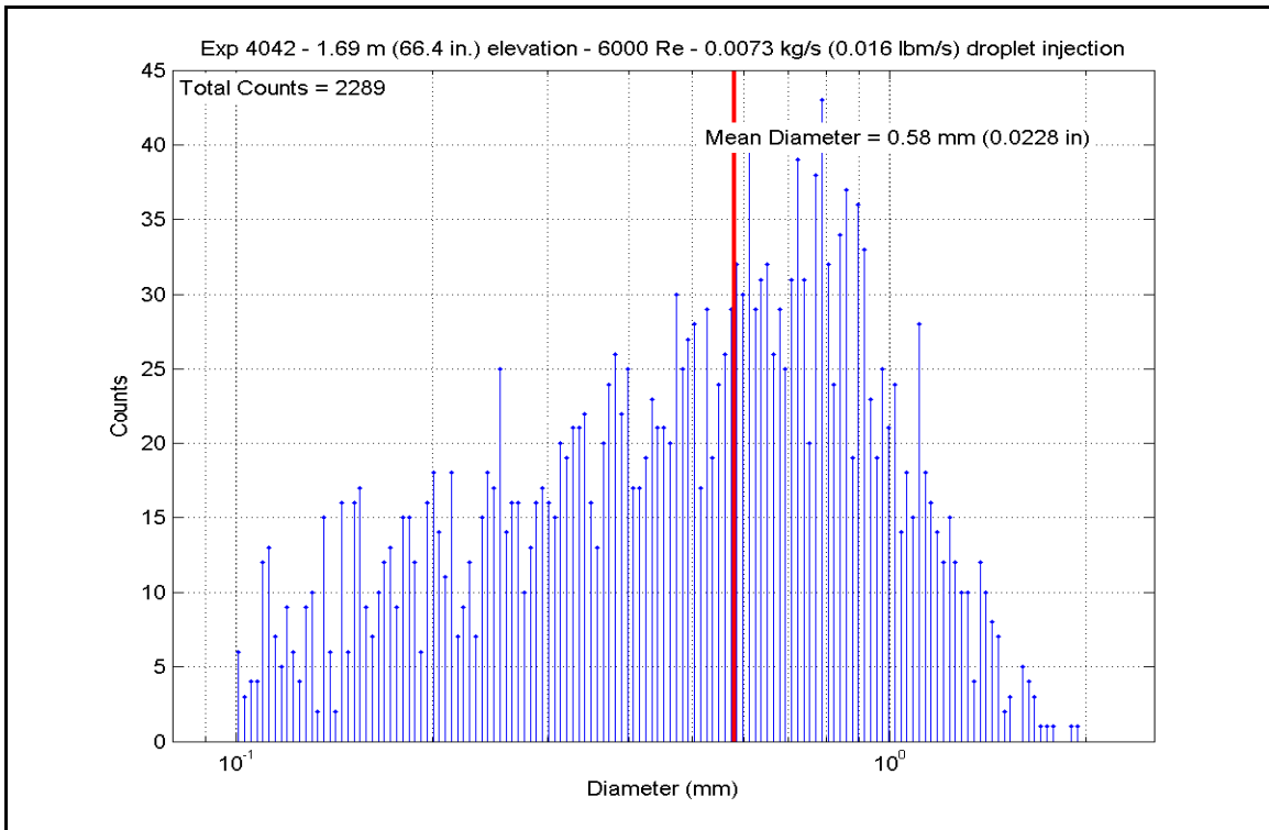
Figure A-687: Droplet Measurements at 1.687 m (66.4 in.) Elevation for Experiment 4042B
