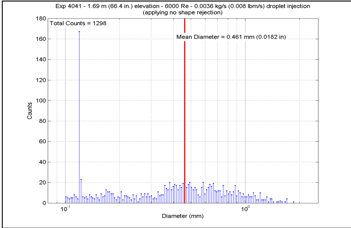
Figure A-609: Droplet Measurements at 1.687 m (66.4 in.) Elevation for Experiment 4041I
