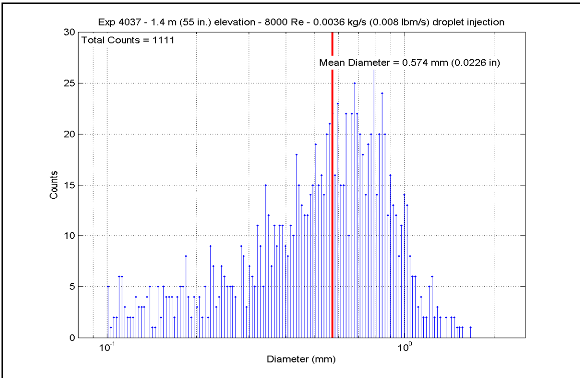
Figure A-376: Droplet Measurements at 1.397 m (55 in.) Elevation for Experiment 4037D
