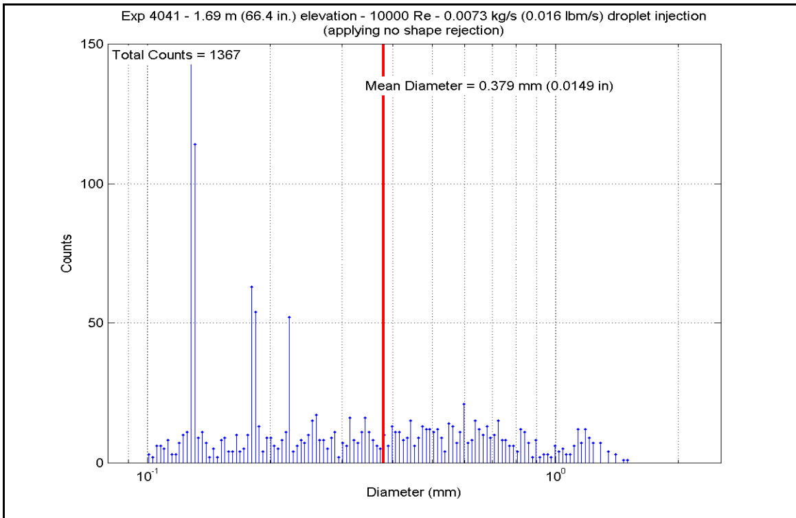
Figure A-476: Droplet Measurements at 1.687 m (66.4 in.) Elevation for Experiment 4041B
