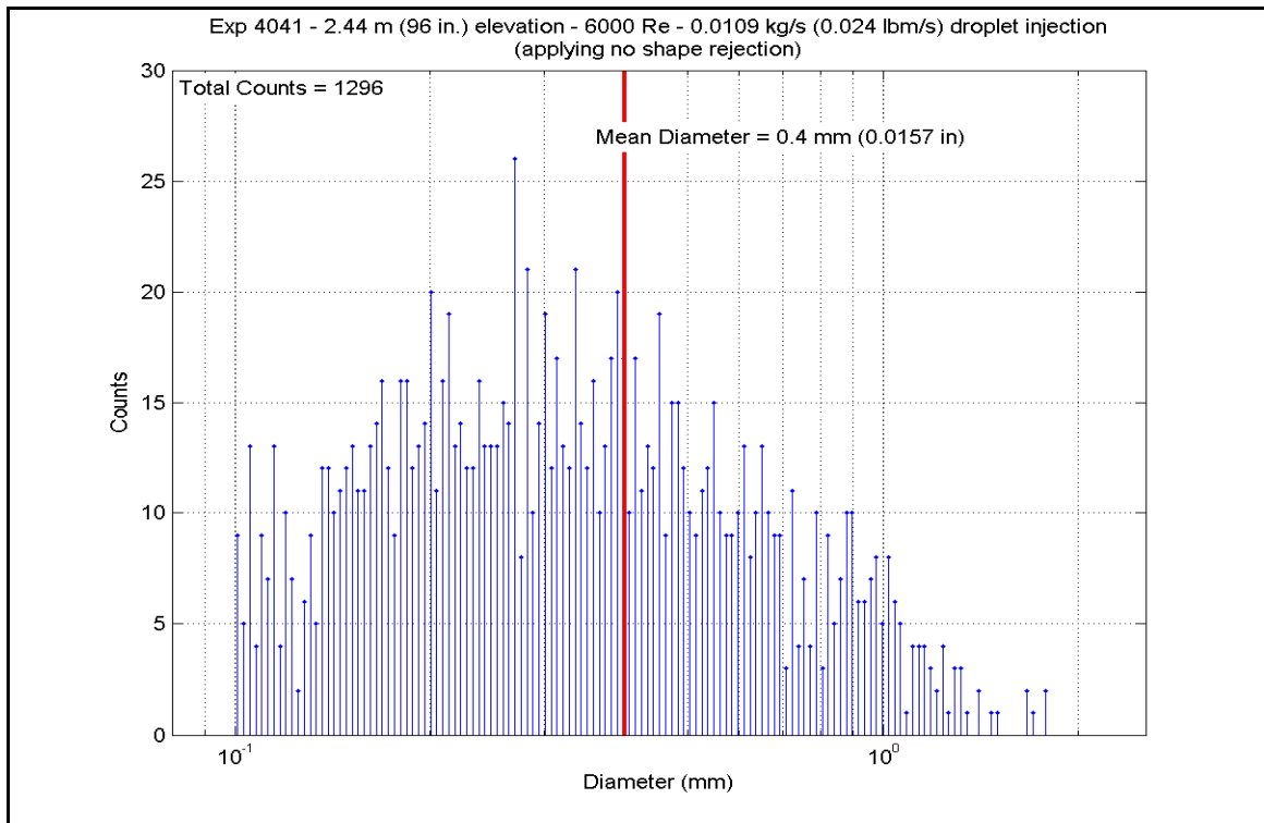
Figure A-652: Droplet Measurements at 2.438 m (96 in.) Elevation for Experiment 4041K
