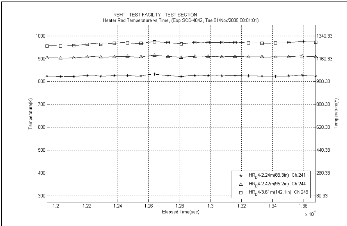
Figure A-663: Heater Rod D4 Temperatures for Experiment 4042A
