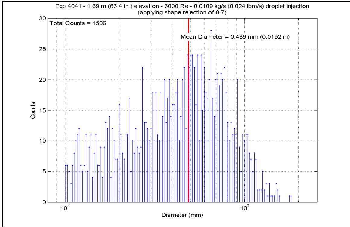
Figure A-649: Droplet Measurements at 1.687 m (66.4 in.) Elevation for Experiment 4041K
