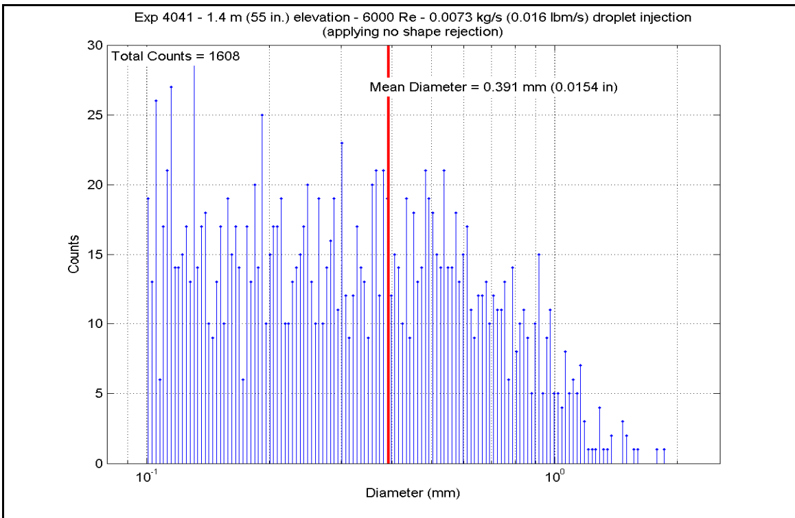
Figure A-627: Droplet Measurements at 1.397 m (55 in.) Elevation for Experiment 4041J
