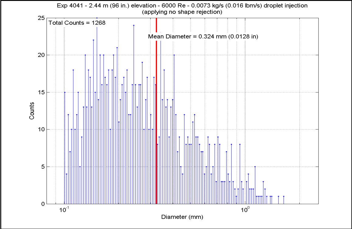
Figure A-632: Droplet Measurements at 2.438 m (96 in.) Elevation for Experiment 4041J
