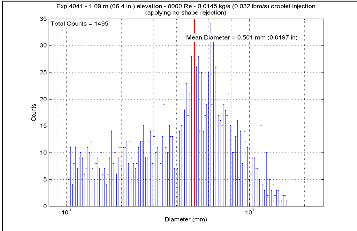
Figure A-590: Droplet Measurements at 1.687 m (66.4 in.) Elevation for Experiment 4041H
