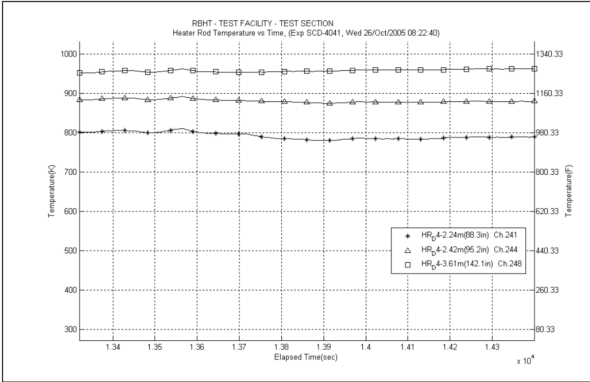
Figure A-445: Heater Rod D4 Temperatures for Experiment 401A
