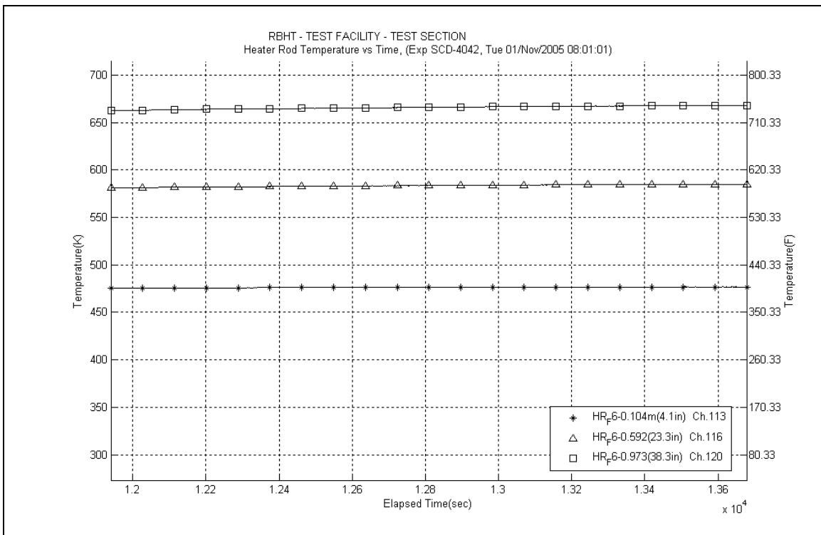
Figure A-664: Heater Rod F6 Temperatures for Experiment 4042A
