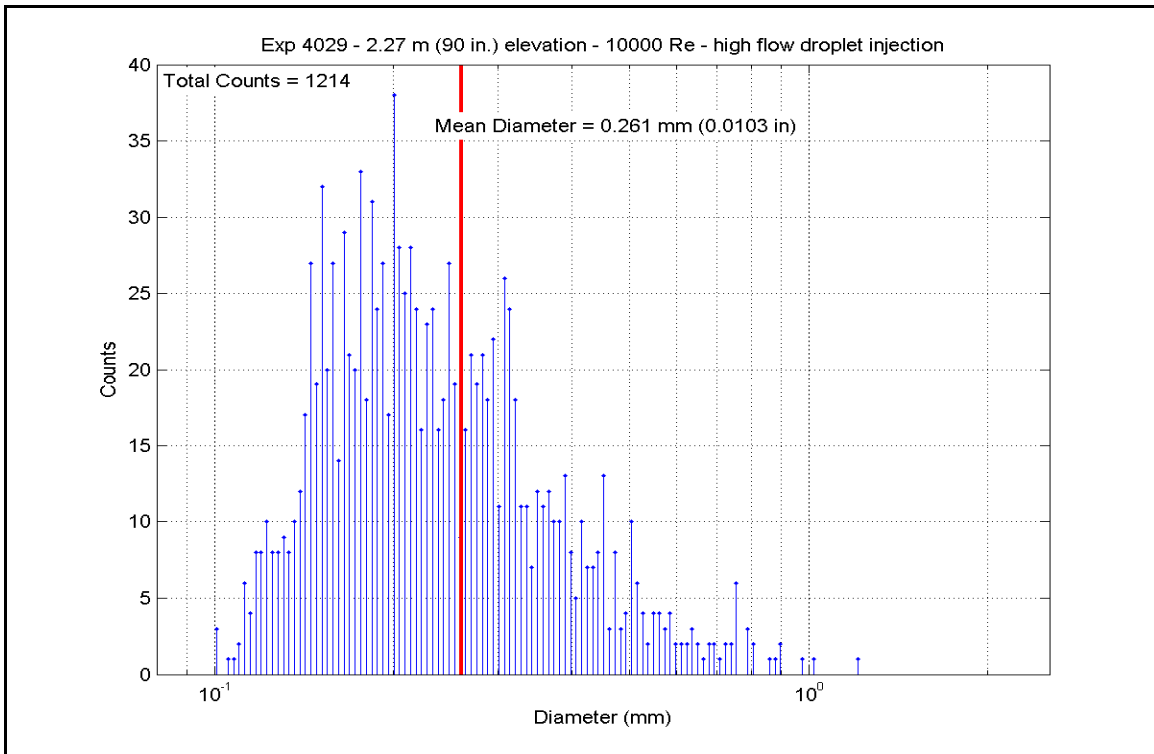
Figure A-40: Droplet Measurements at 2.286 m (90 in.) Elevation for Experiment 4029A
