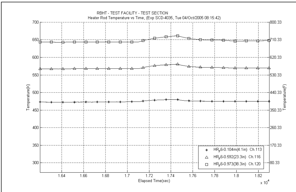
Figure A-229: Heater Rod F6 Temperatures for Experiment 4035B
