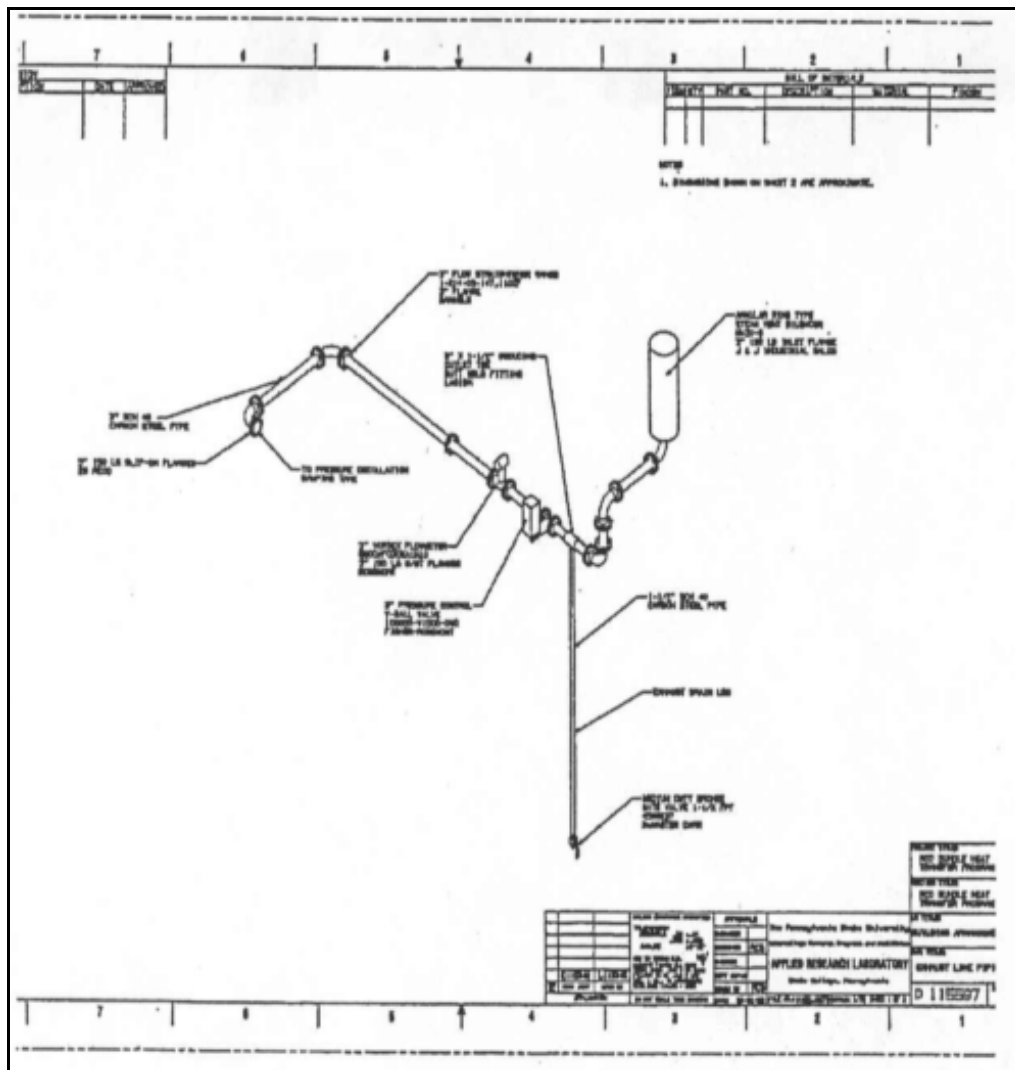
Figure 2-20: Exhaust Piping
