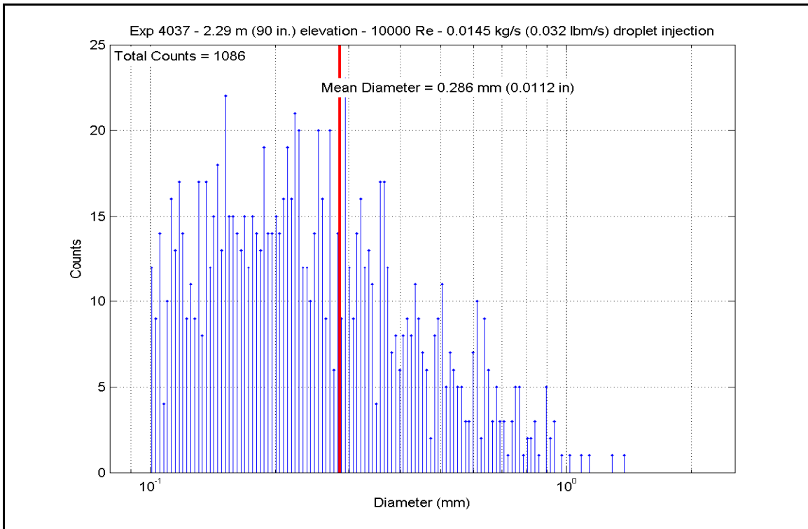
Figure A-360: Droplet Measurements at 2.286 m (90 in.) Elevation for Experiment 4037C
