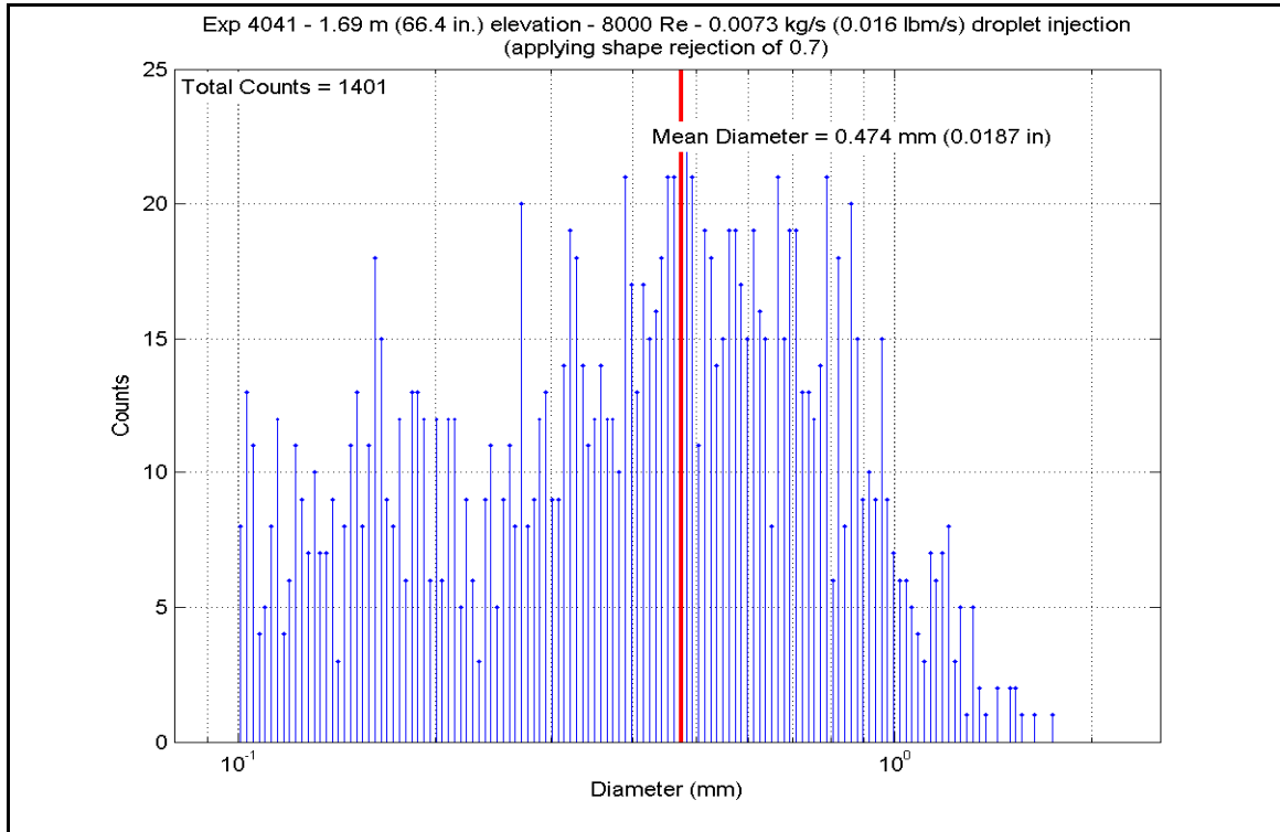
Figure A-553: Droplet Measurements at 1.687 m (66.4 in.) Elevation for Experiment 4041F
