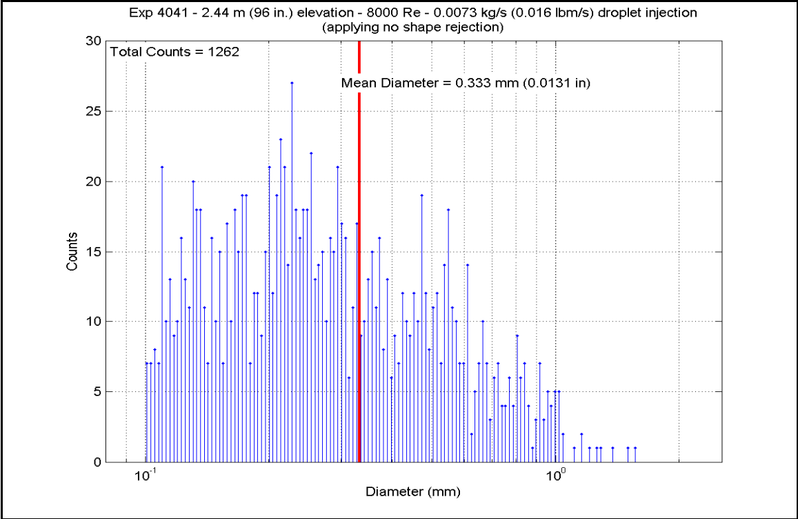
Figure A-556: Droplet Measurements at 2.438 m (96 in.) Elevation for Experiment 4041F
