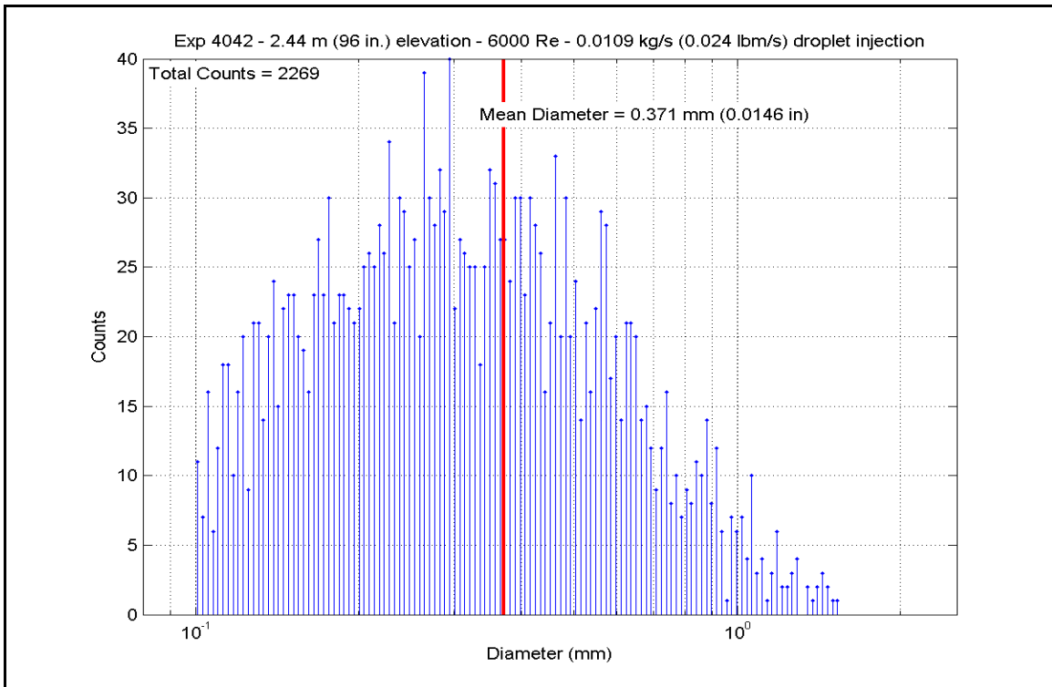
Figure A-708: Droplet Measurements at 2.438 m (96 in.) Elevation for Experiment 4042C
