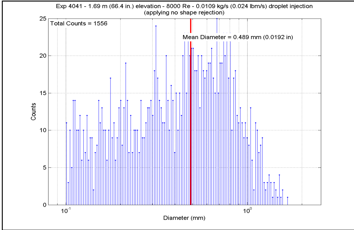
Figure A-571: Droplet Measurements at 1.687 m (66.4 in.) Elevation for Experiment 4041G
