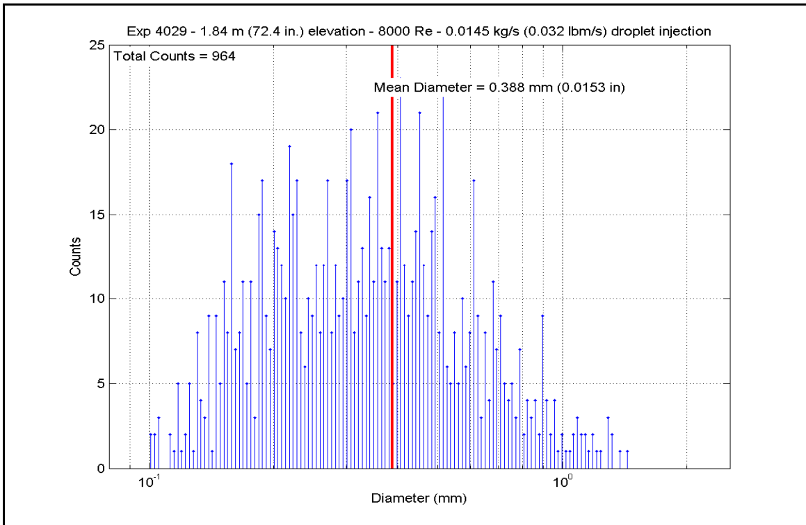
Figure A-93: Droplet Measurements at 1.839 m (72.4 in.) Elevation for Experiment 4029D
