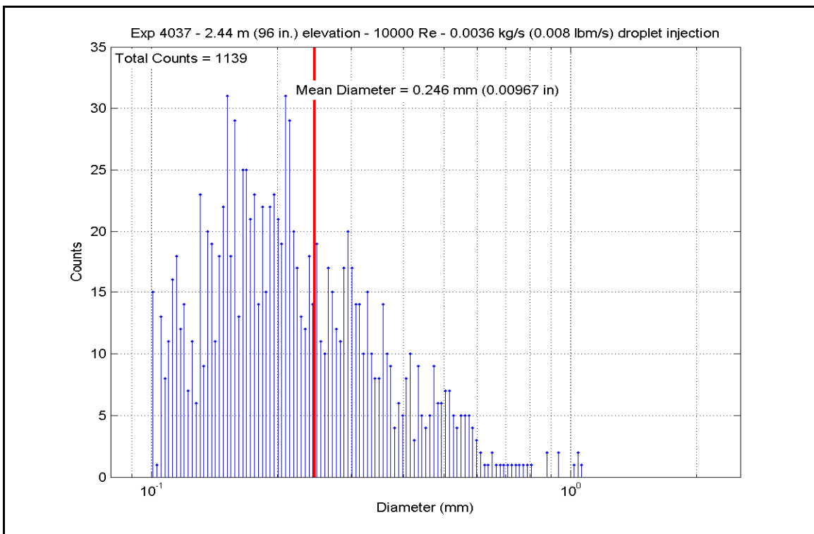
Figure A-325: Droplet Measurements at 2.438 m (96 in.) Elevation for Experiment 4037A
