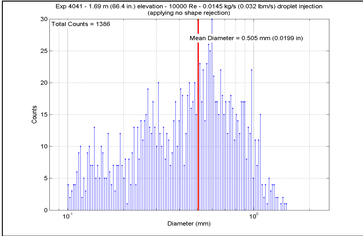
Figure A-514: Droplet Measurements at 1.687 m (66.4 in.) Elevation for Experiment 4041D
