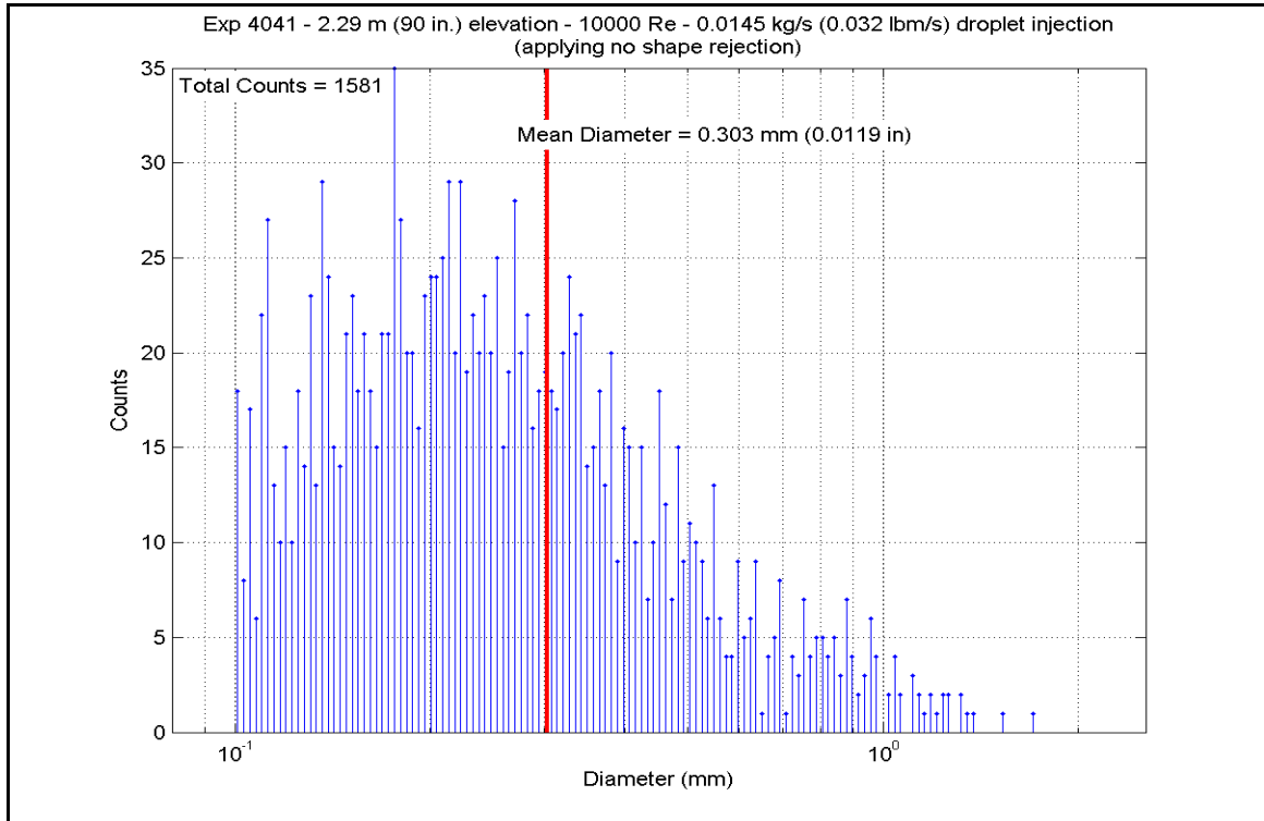
Figure A-517: Droplet Measurements at 2.286 m (90 in.) Elevation for Experiment 4041D
