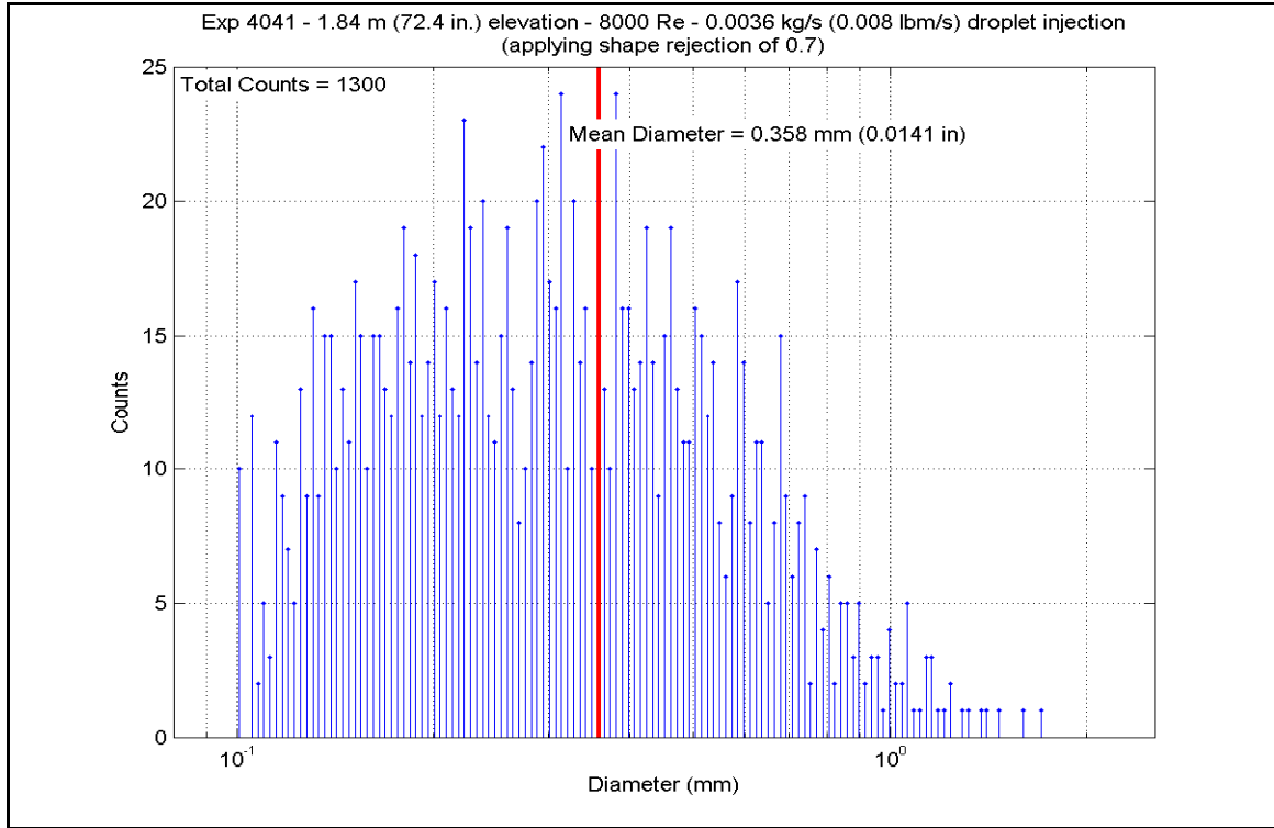
Figure A-535: Droplet Measurements at 1.839 m (72.4 in.) Elevation for Experiment 4041E
