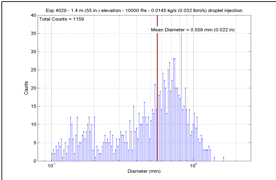
Figure A-55: Droplet Measurements at 1.397 m (55 in.) Elevation for Experiment 4029B
