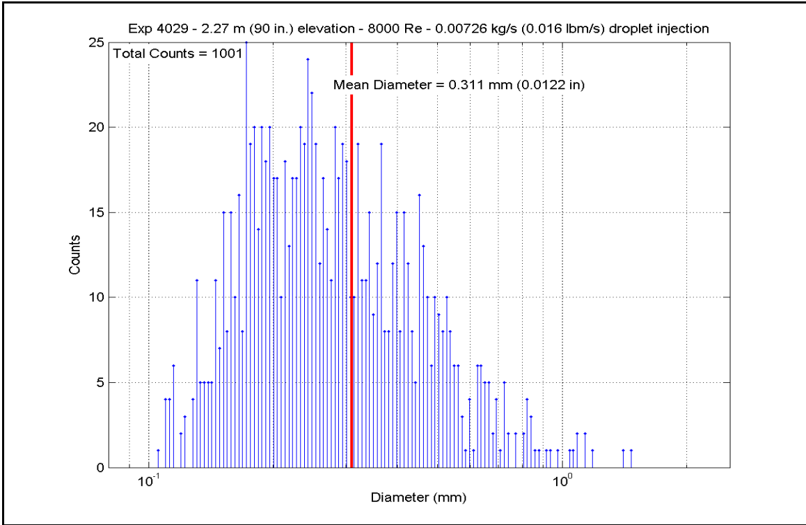
Figure A-76: Droplet Measurements at 2.286 m (90 in.) Elevation for Experiment 4029C
