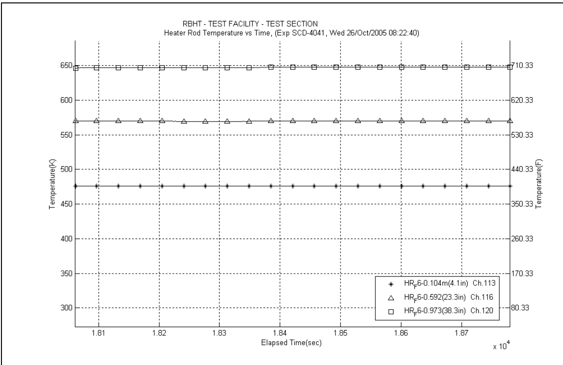
Figure A-492: Heater Rod F6 Temperatures for Experiment 401C
