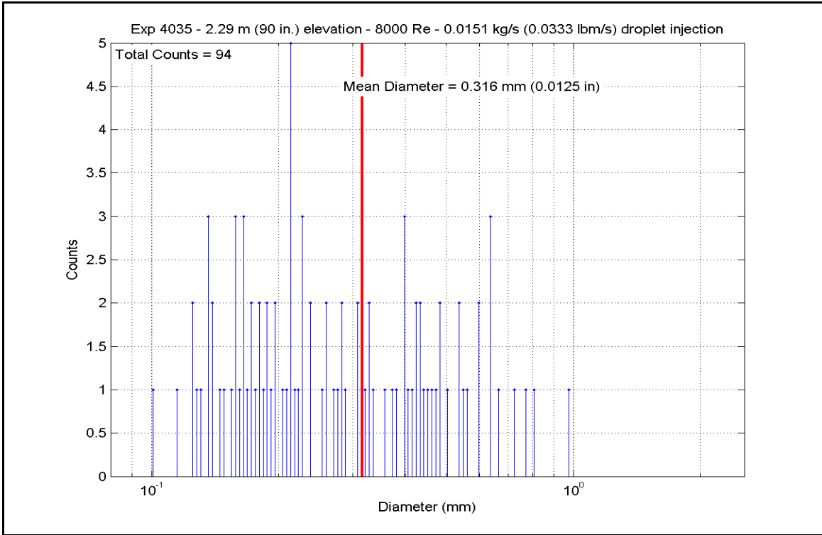
Figure A-270: Droplet Measurements at 2.286 m (90 in.) Elevation for Experiment 4035D
