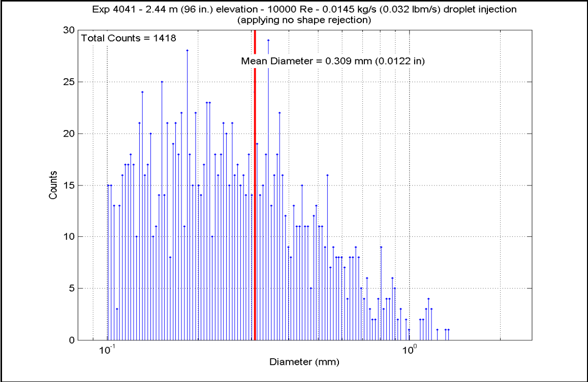
Figure A-518: Droplet Measurements at 2.438 m (96 in.) Elevation for Experiment 4041D
