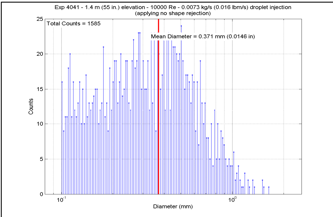
Figure A-475: Droplet Measurements at 1.397 m (55 in.) Elevation for Experiment 4041B
