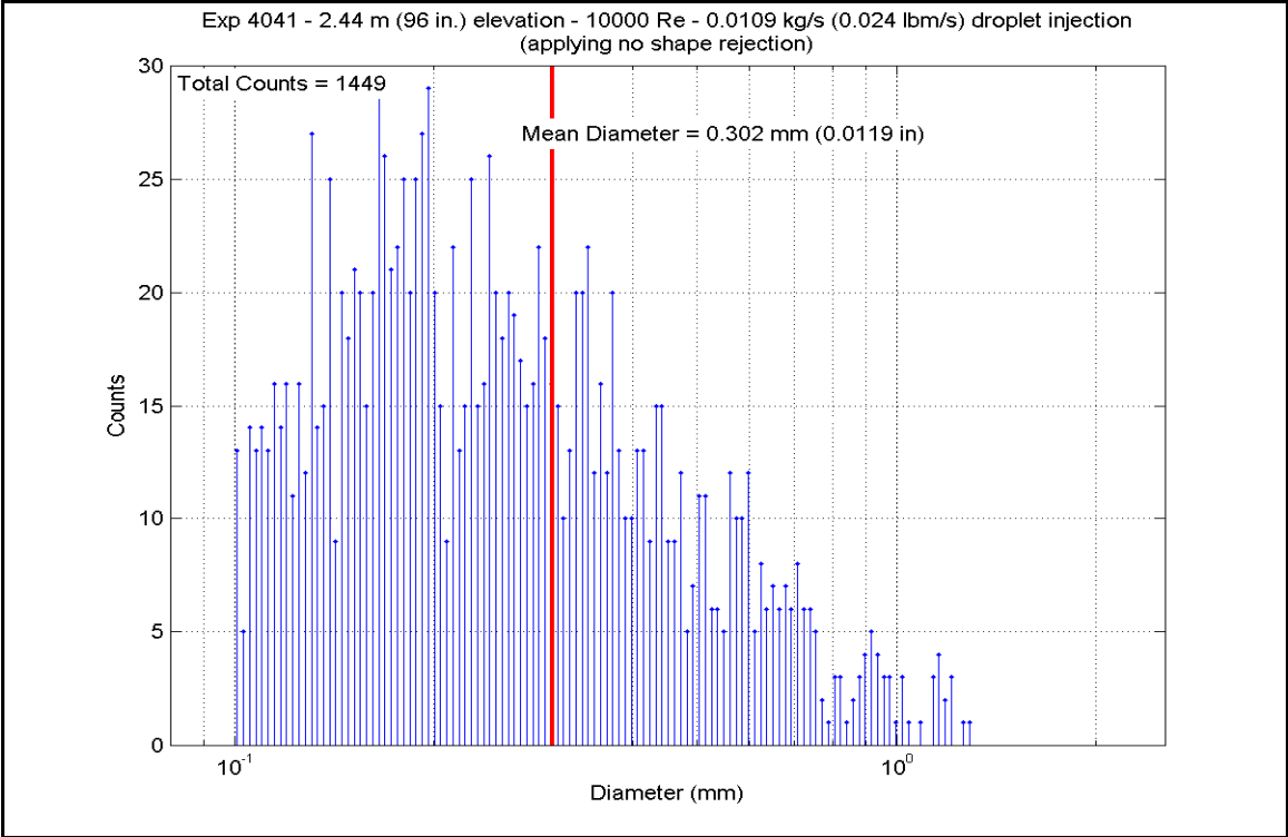
Figure A-499: Droplet Measurements at 2.438 m (96 in.) Elevation for Experiment 4041C
