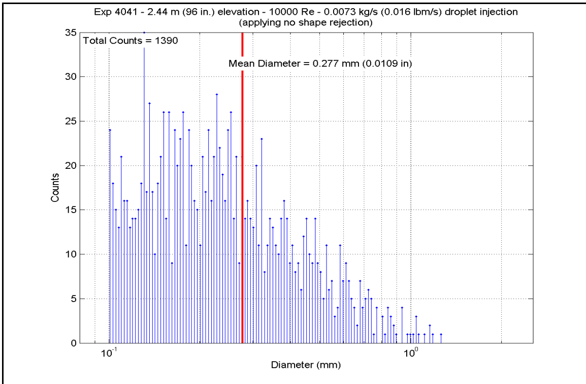
Figure A-480: Droplet Measurements at 2.438 m (96 in.) Elevation for Experiment 4041B
