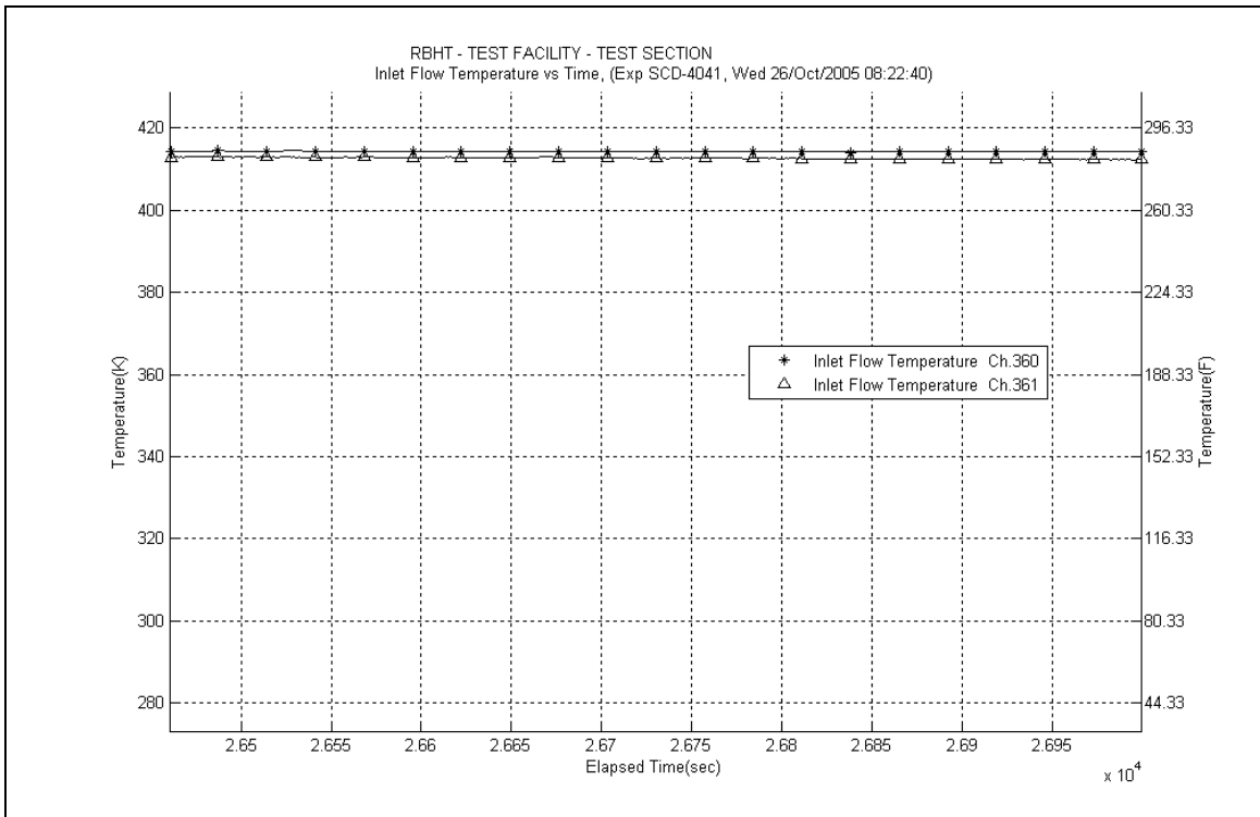
Figure A-596: Inlet Steam Temperature for Experiment 40411
