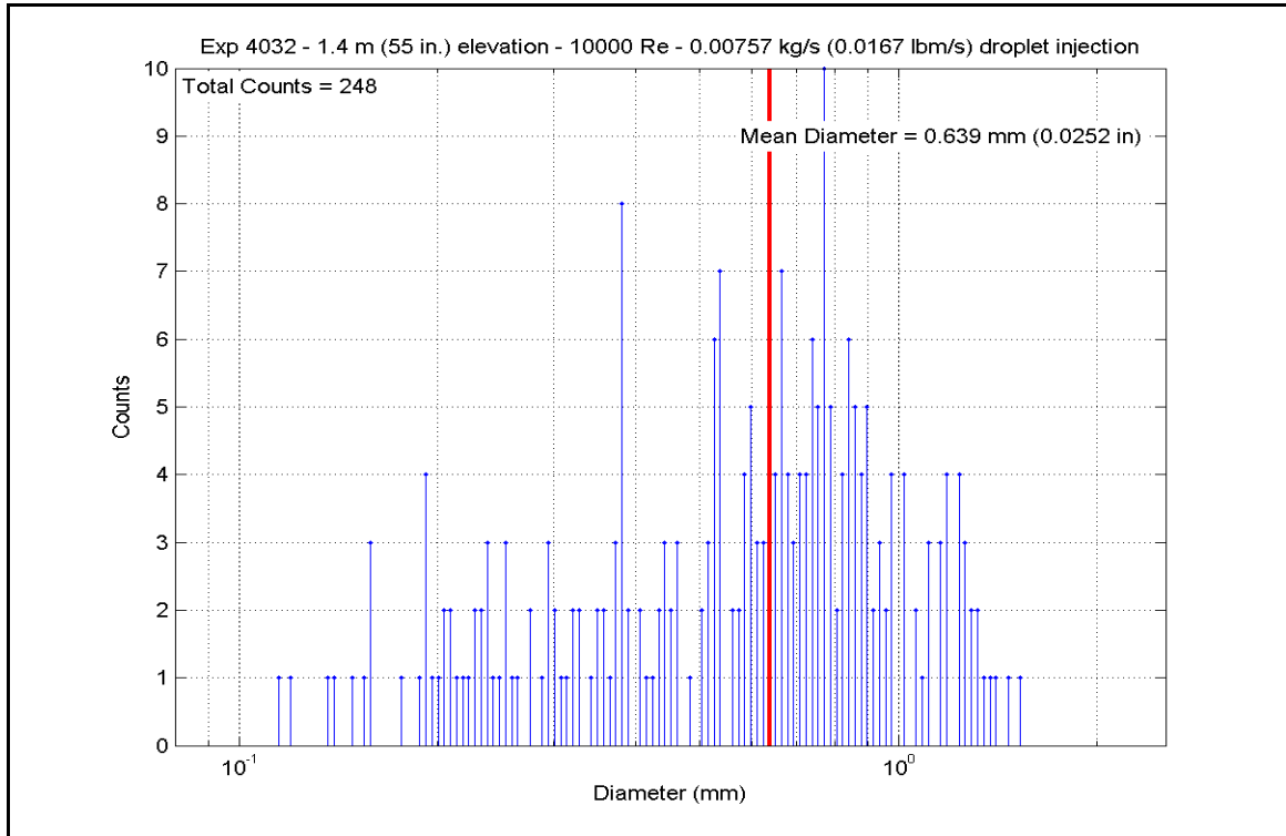
Figure A-124: Droplet Measurements at 1.397 m (55 in.) Elevation for Experiment 4032A
