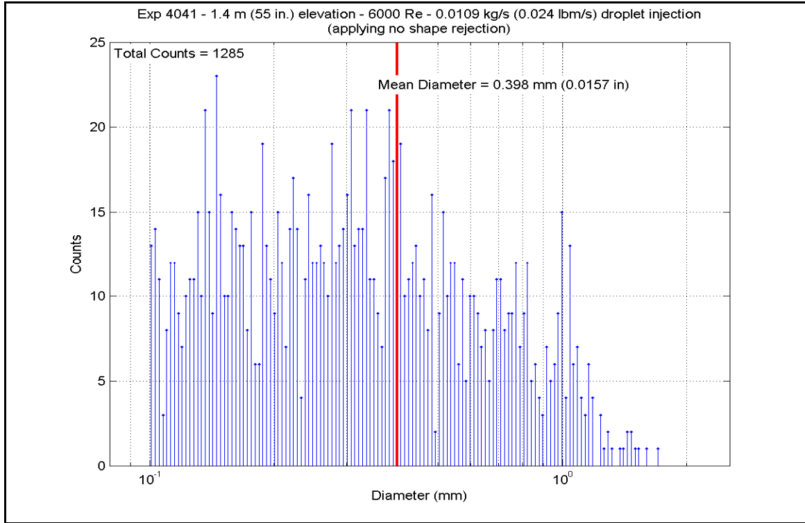
Figure A-647: Droplet Measurements at 1.397 m (55 in.) Elevation for Experiment 4041K
