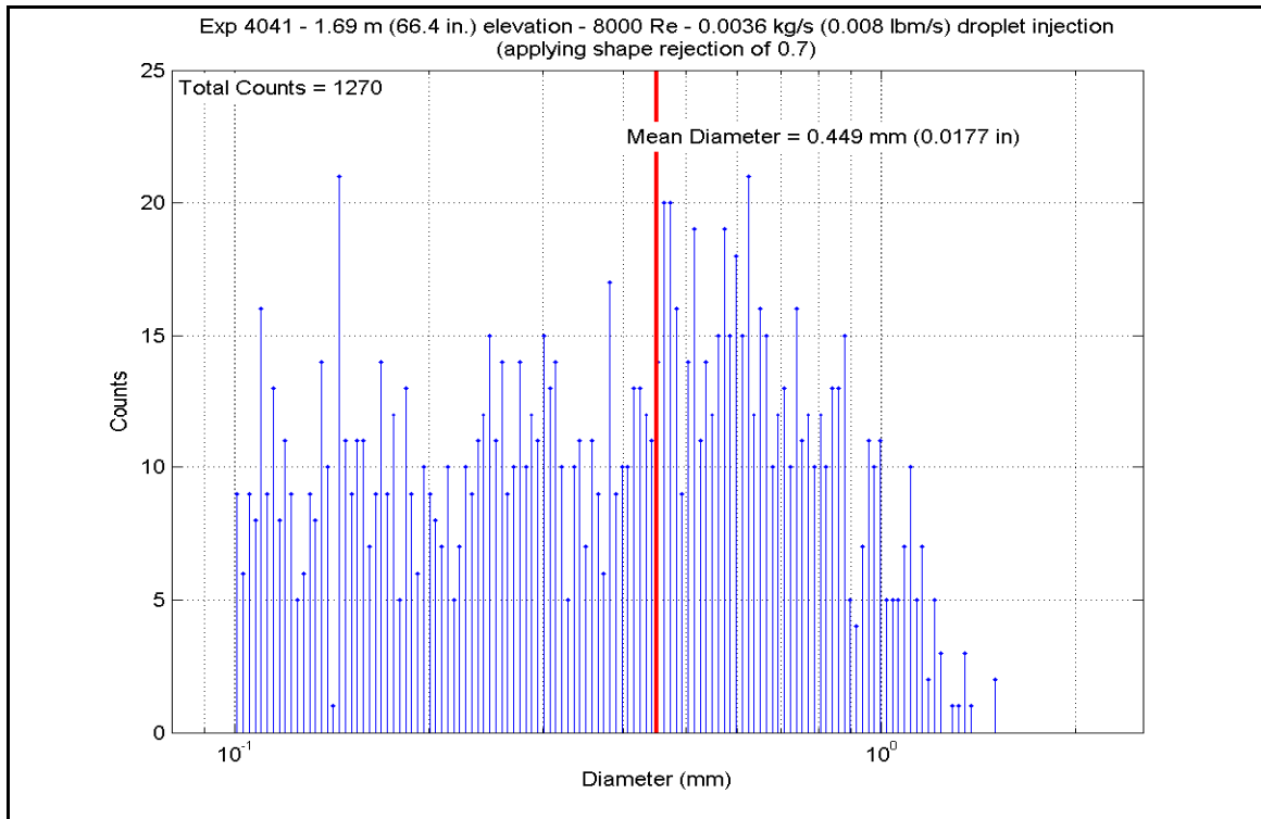
Figure A-534: Droplet Measurements at 1.687 m (66.4 in.) Elevation for Experiment 4041E
