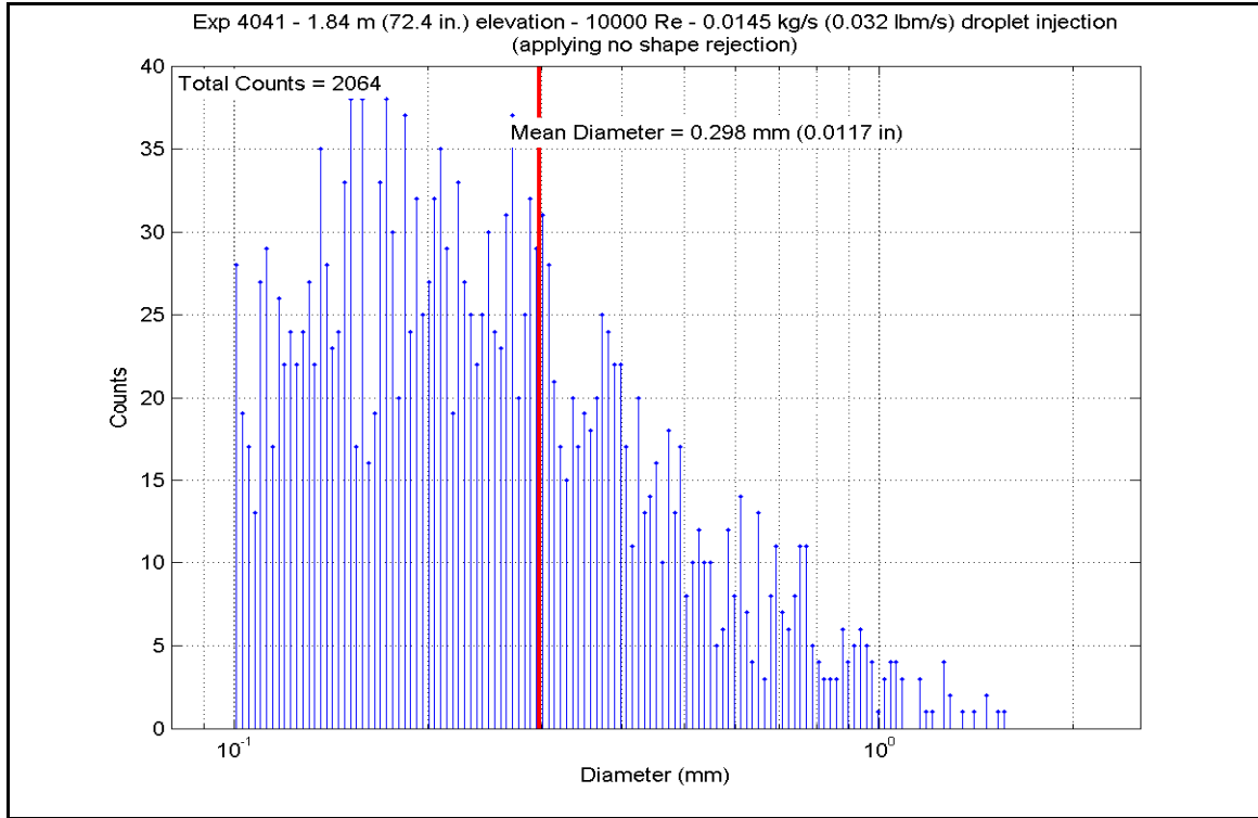
Figure A-516: Droplet Measurements at 1.839 m (72.4 in.) Elevation for Experiment 4041D
