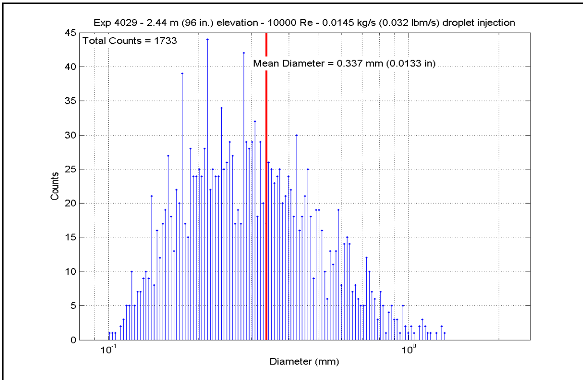
Figure A-59: Droplet Measurements at 2.438 m (96 in.) Elevation for Experiment 4029B
