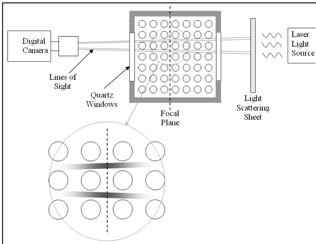
Figure 2-40: General Schematic of the Imaging System
