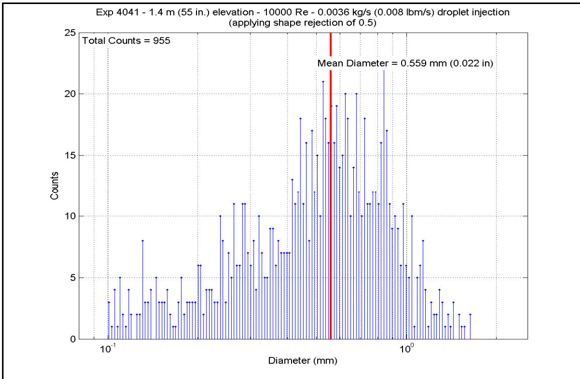
Figure A-450: Droplet Measurements at 1.397 m (55 in.) Elevation for Experiment 4041A
