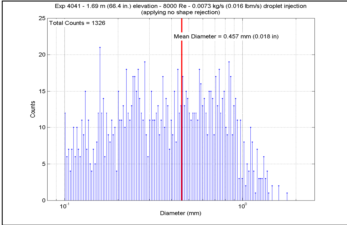
Figure A-552: Droplet Measurements at 1.687 m (66.4 in.) Elevation for Experiment 4041F
