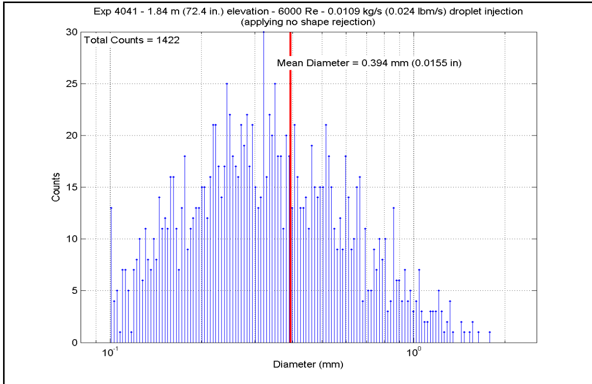
Figure A-650: Droplet Measurements at 1.839 m (72.4 in.) Elevation for Experiment 4041K
