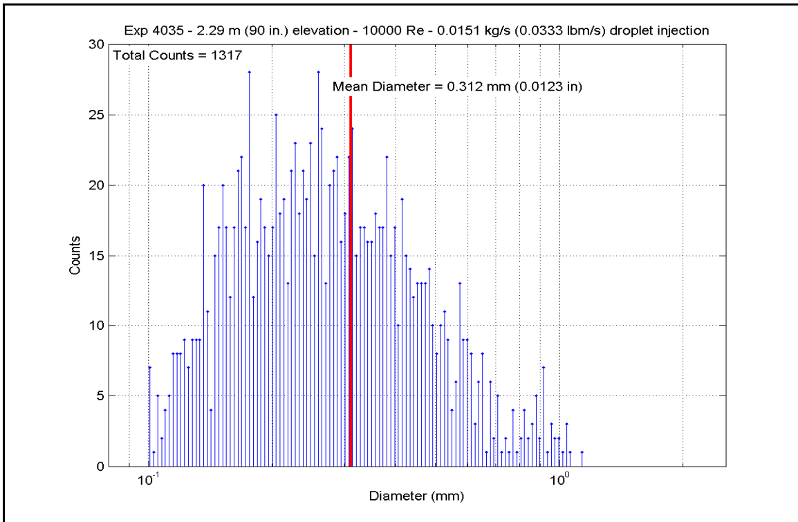
Figure A-234: Droplet Measurements at 2.286 m (90 in.) Elevation for Experiment 4035B
