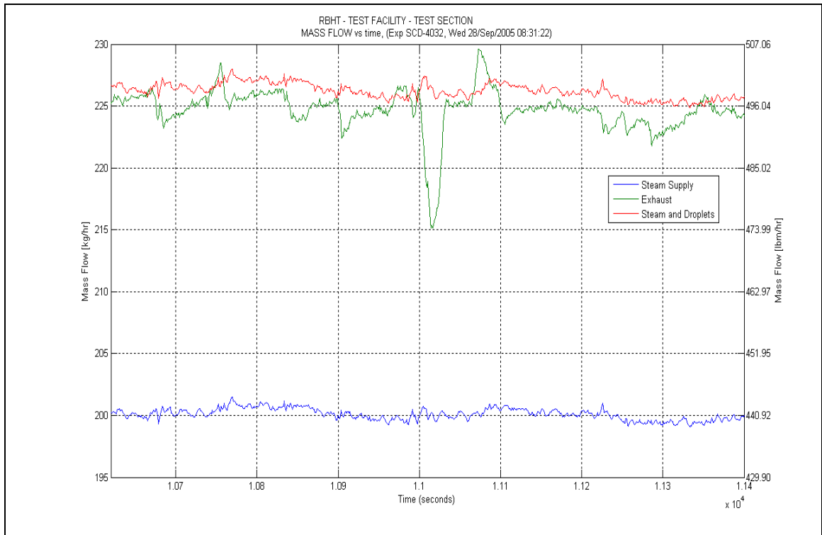
Figure A-123: Mass Flow for Experiment 4032A
