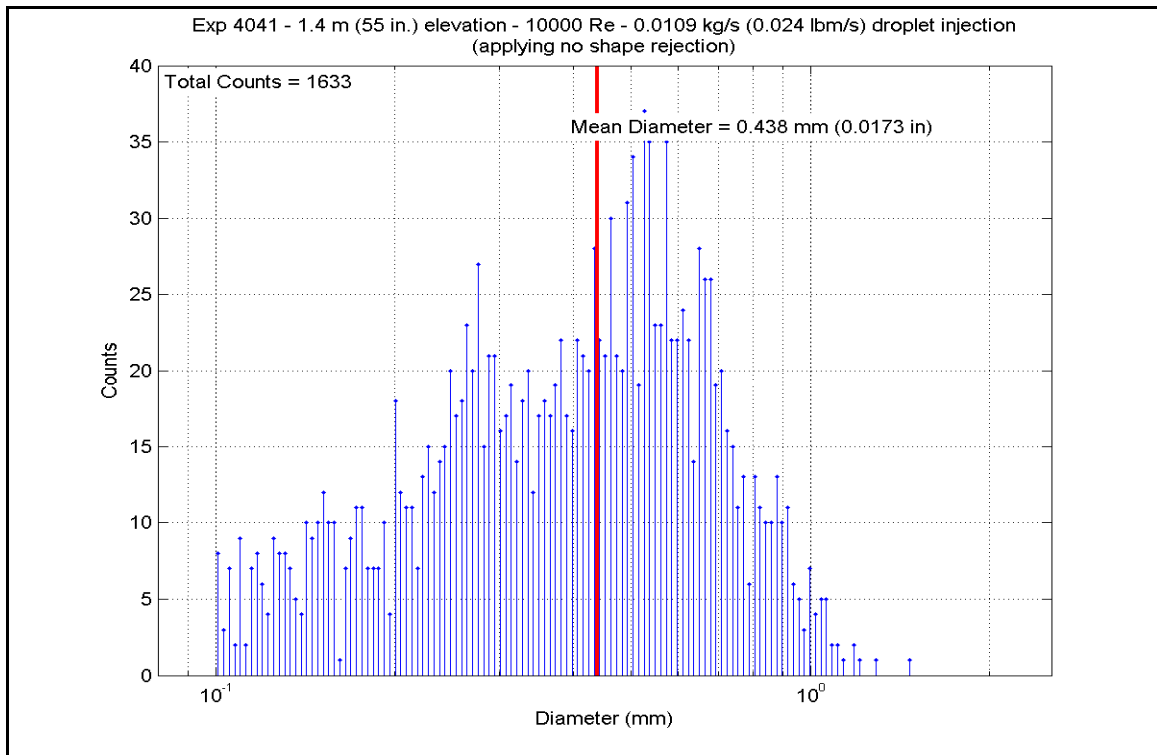
Figure A-494: Droplet Measurements at 1.397 m (55 in.) Elevation for Experiment 4041C
