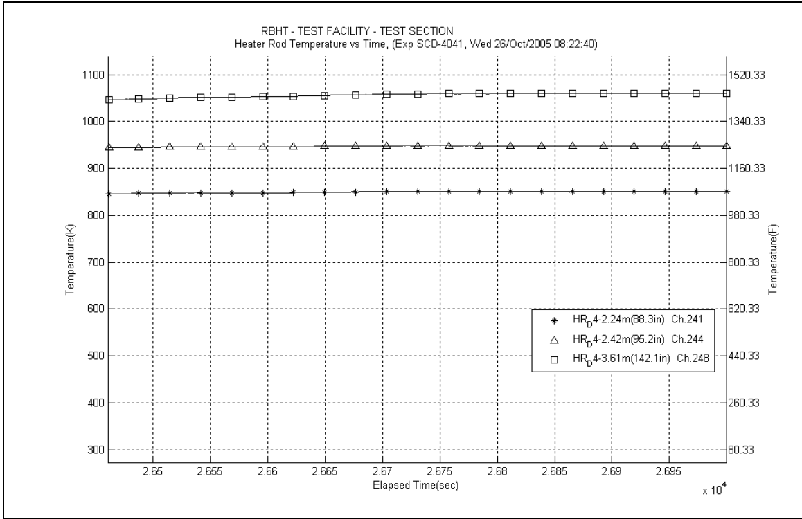
Figure A-605: Heater Rod D4 Temperatures for Experiment 40411
