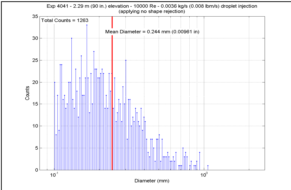
Figure A-460: Droplet Measurements at 2.286 m (90 in.) Elevation for Experiment 4041A
