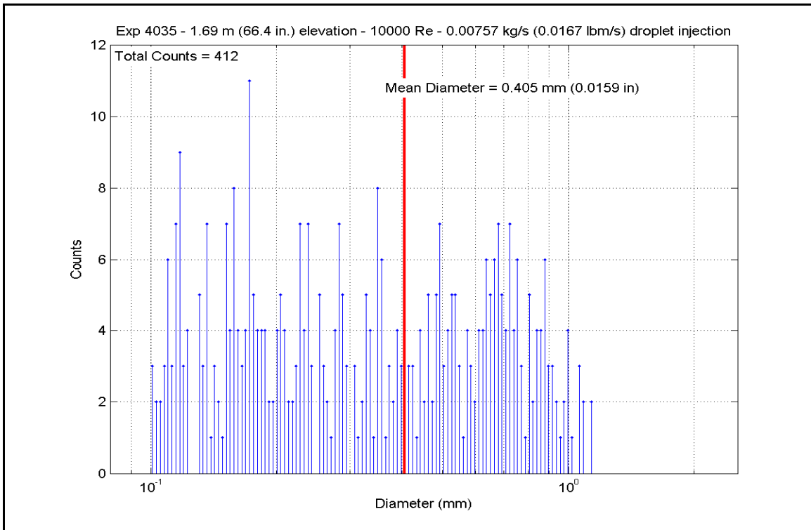
Figure A-214: Droplet Measurements at 1.687 m (66.4 in.) Elevation for Experiment 4035A
