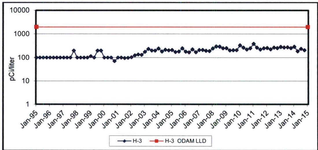
TRENDING GRAPH 7 TRITIUM IN RIVER WATER QUARTERLY AVERAGE – ALL LOCATIONS
