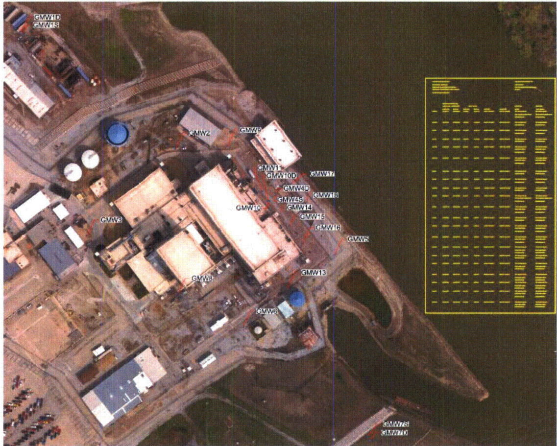
Routine Well Water Sample Locations for the Radiological Groundwater Protection Program, Nebraska Public Power District, Cooper Nuclear Station, 2014
