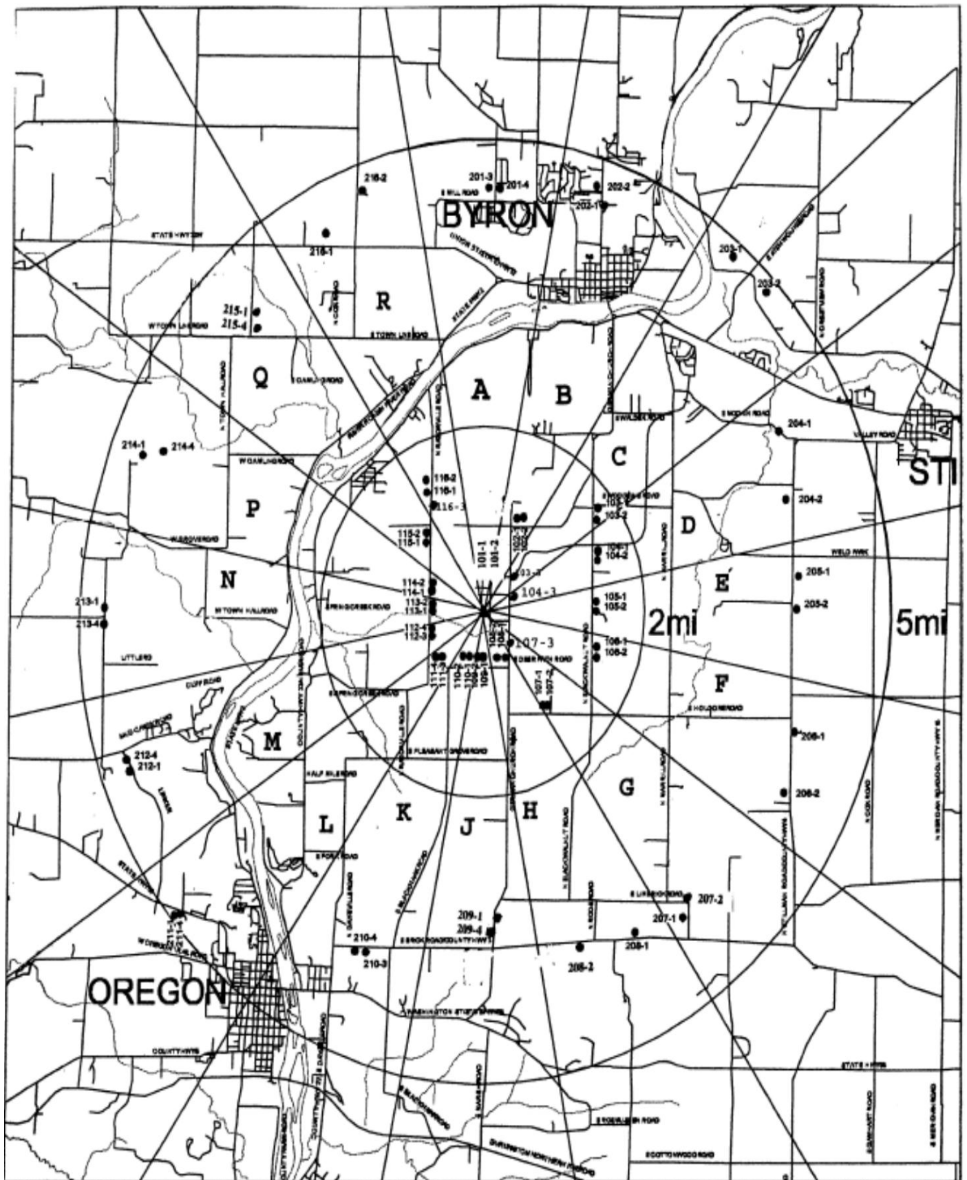
Figure B-1 Inner and Outer Ring OSRD Locations of the Byron Nuclear Generating Station, 2014
