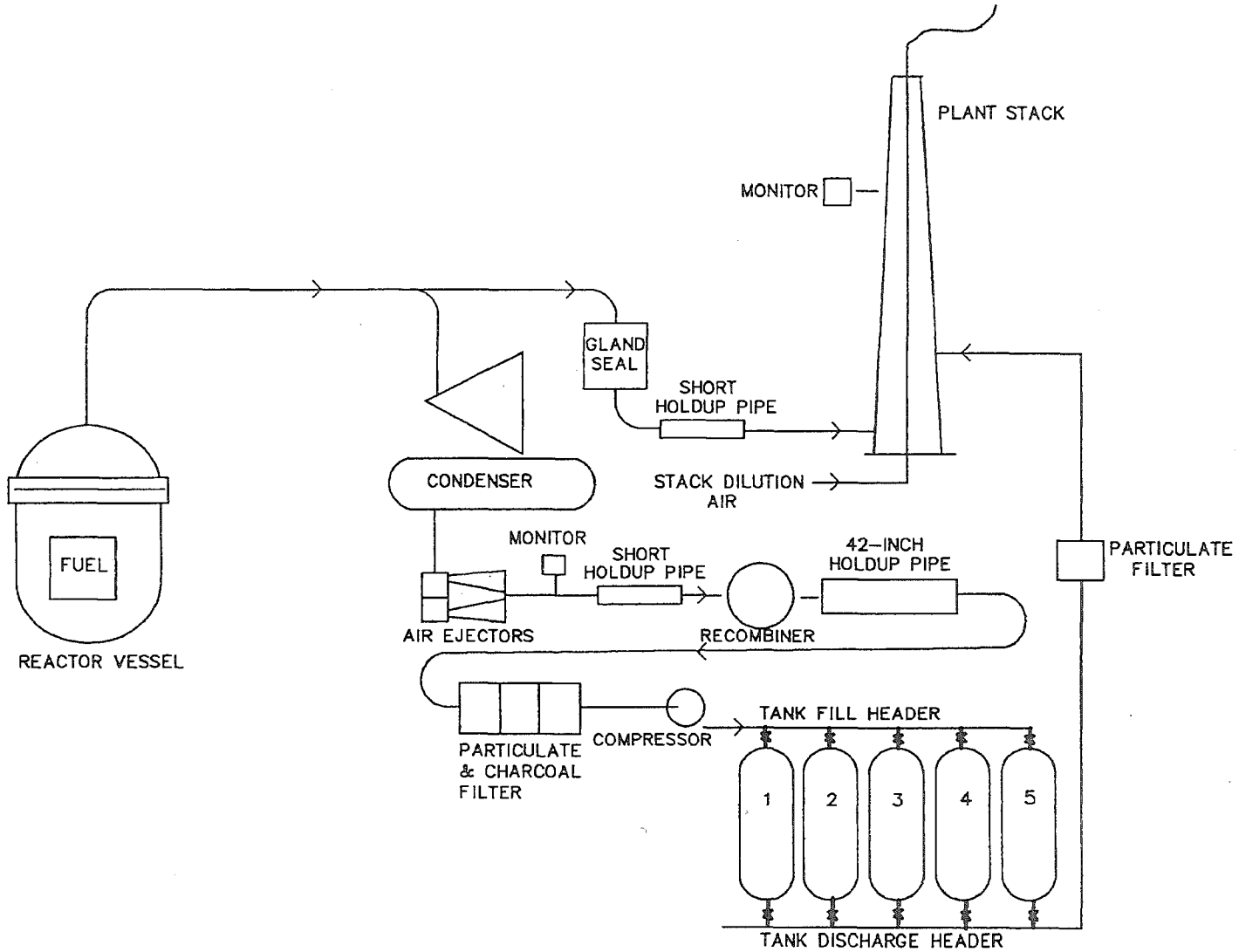
Figure 1 Gaseous Radwaste
