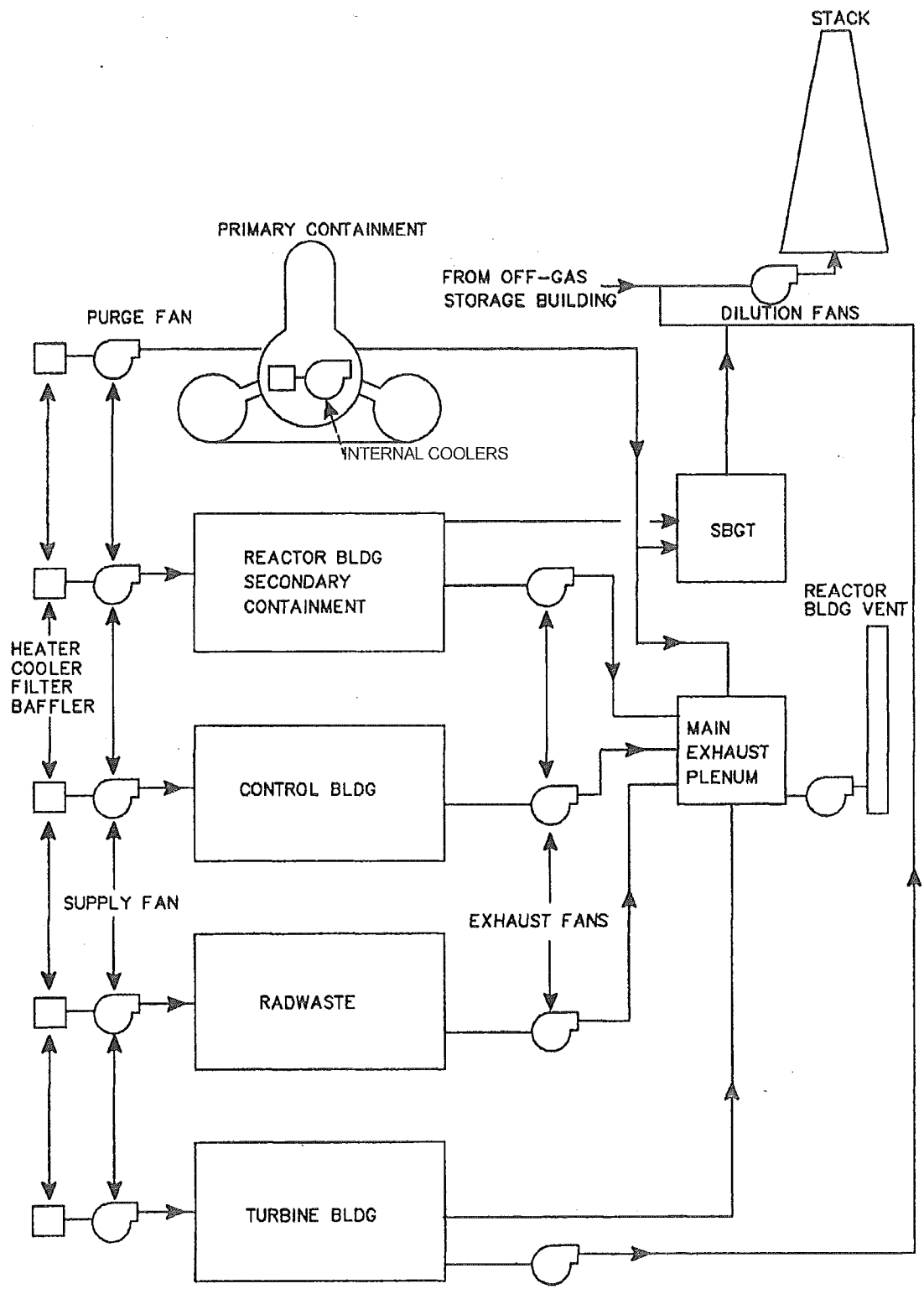
Figure 2 Ventilation System
