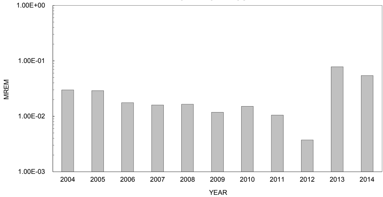
UNIT 1 GASEOUS EFFLUENTS TOTAL BODY DOSE
