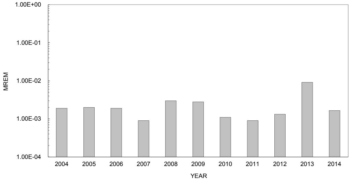
UNIT 2 LIQUID EFFLUENTS CRITICAL ORGAN DOSE
