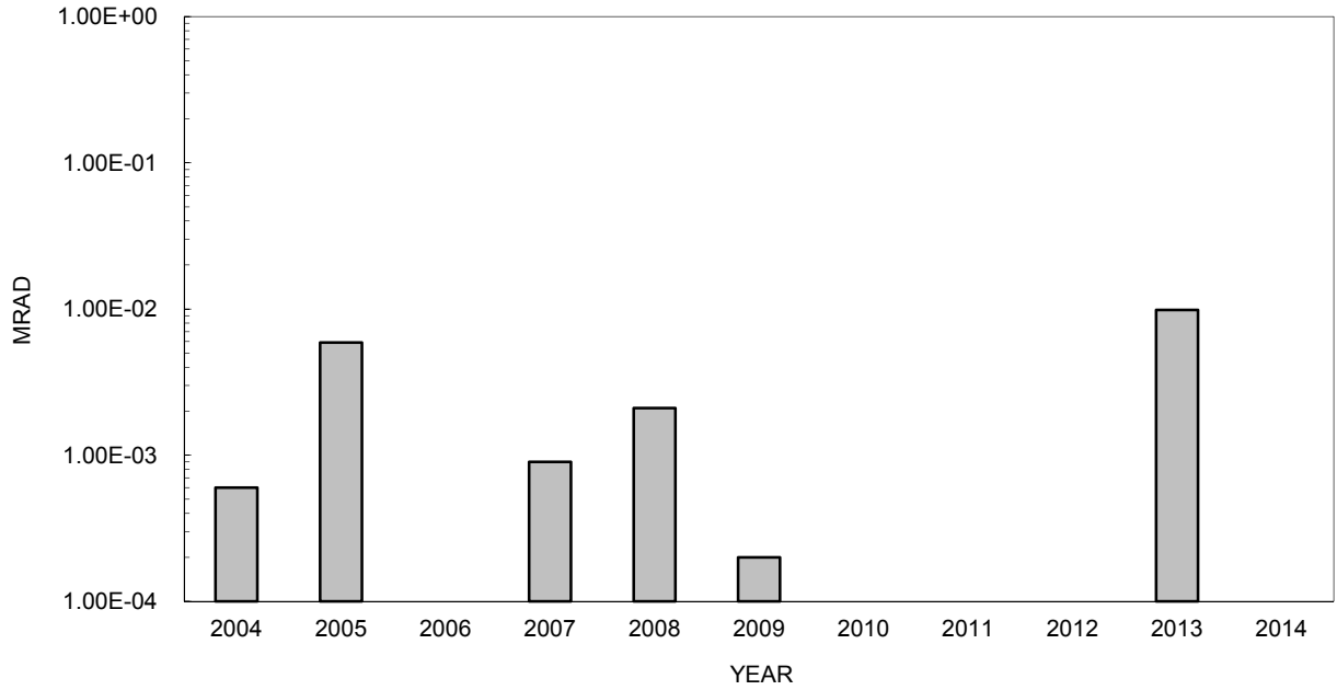
UNIT 1 GASEOUS EFFLUENTS BETA DOSE
