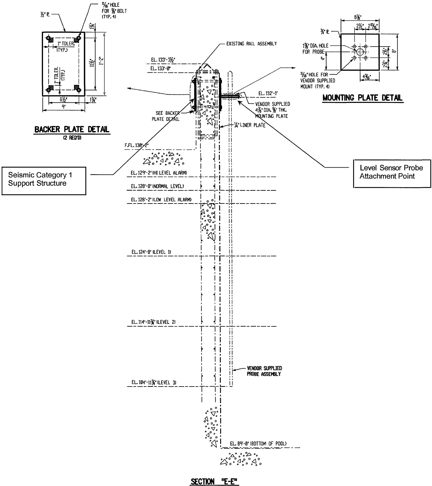
Figure 1 - Typical Mounting Sketch (Not to scale) Ref: PSEG Drawing 606366
