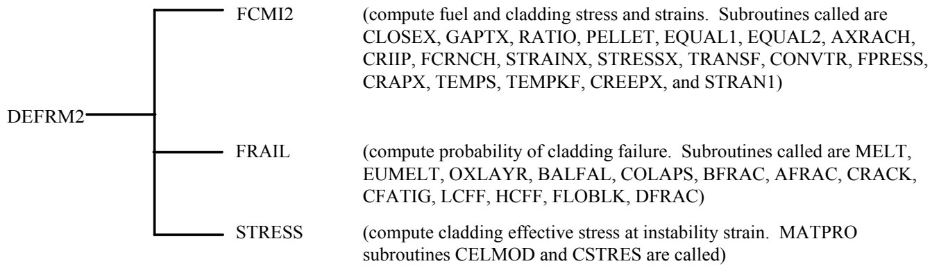
Figure F.9 Subroutine calls from subroutine DEFRM2
