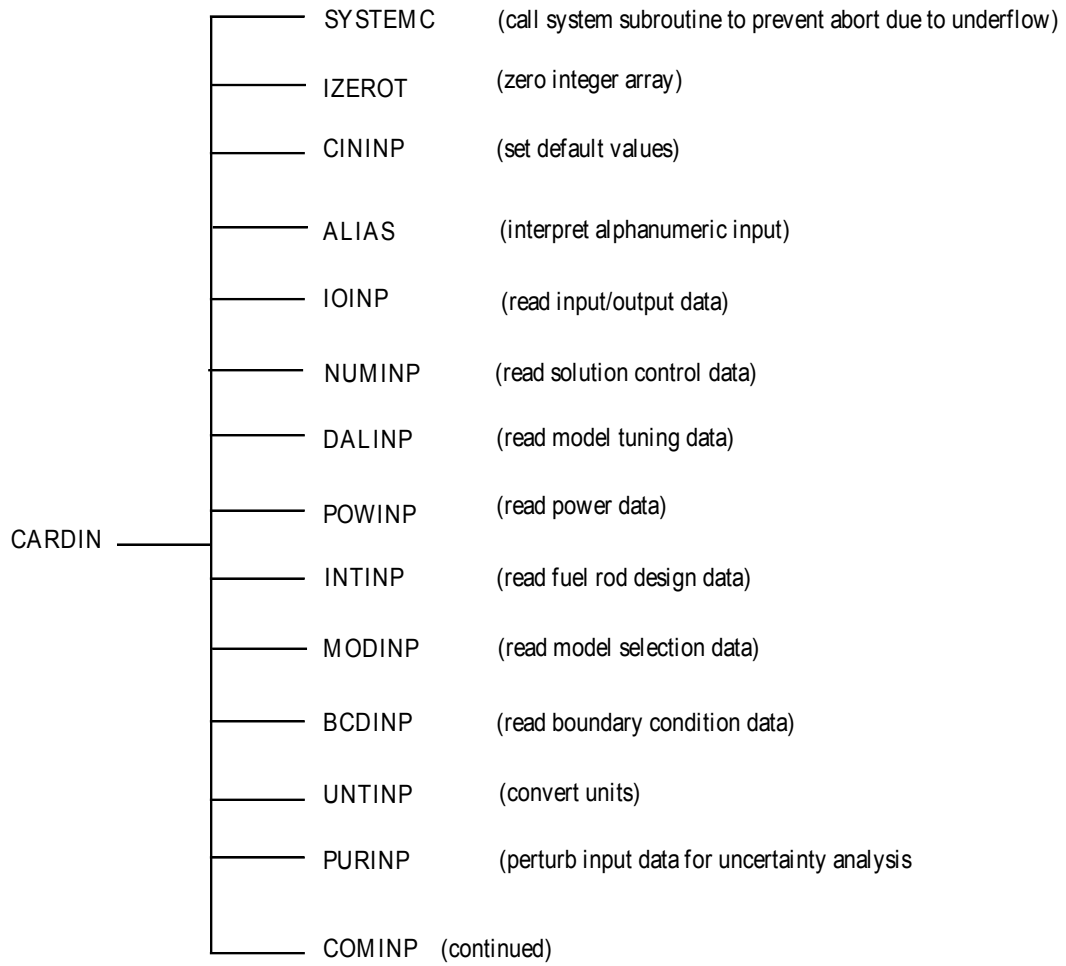
Figure F.3 Subroutine calls from subroutine CARDIN
