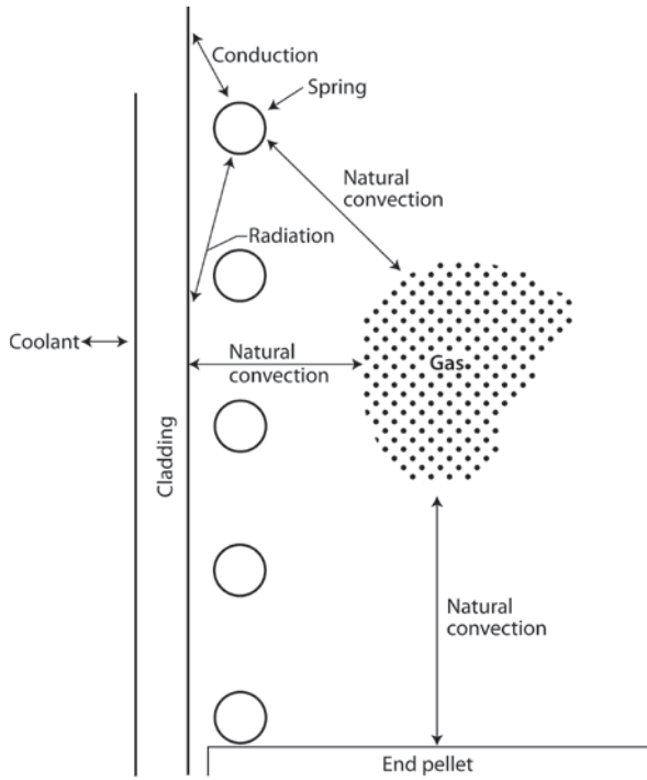
Figure 2.6 Energy flow in plenum model – energy exchange mechanisms
