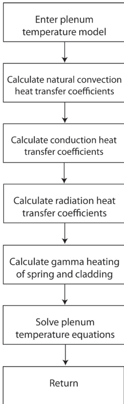
Figure 2.7 Flowchart of plenum temperature calculation
