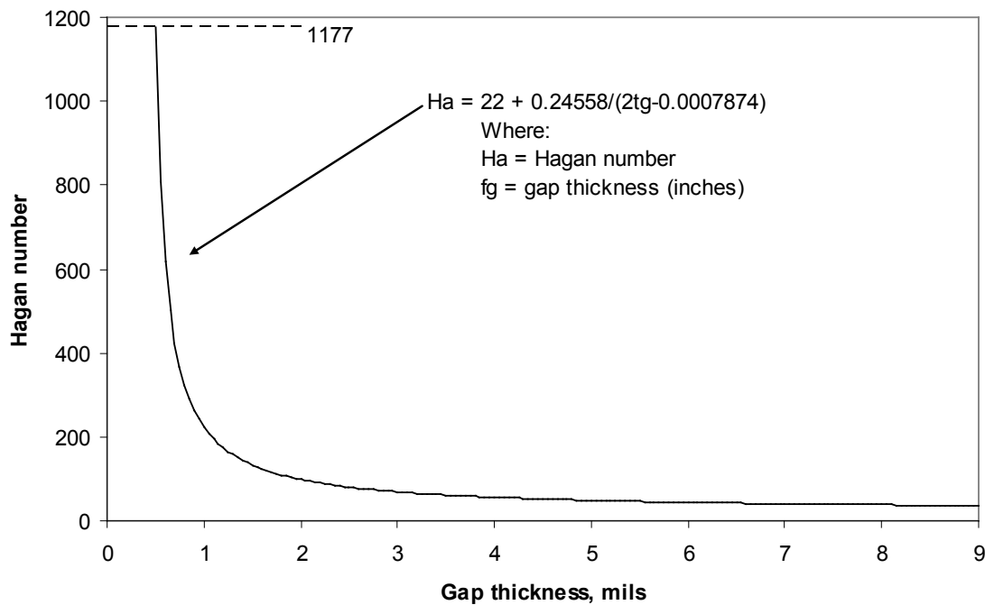
Figure 2.24 Hagan number versus width of fuel-cladding gap
