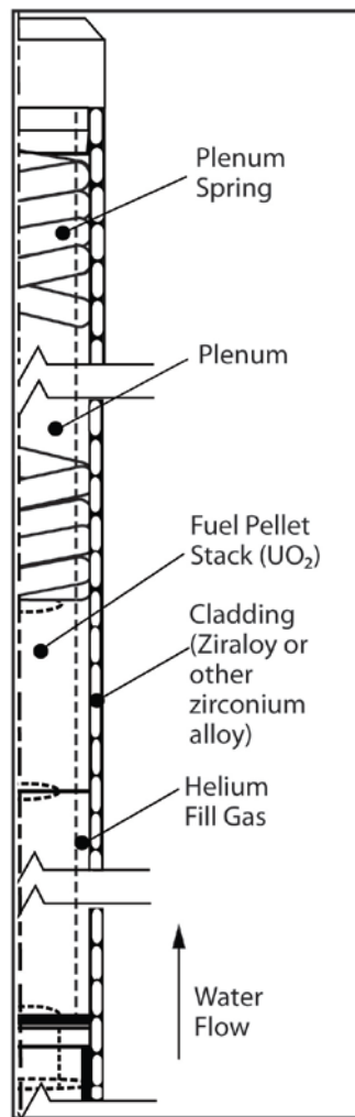
Figure 1.1 Schematic of typical LWR fuel rod
