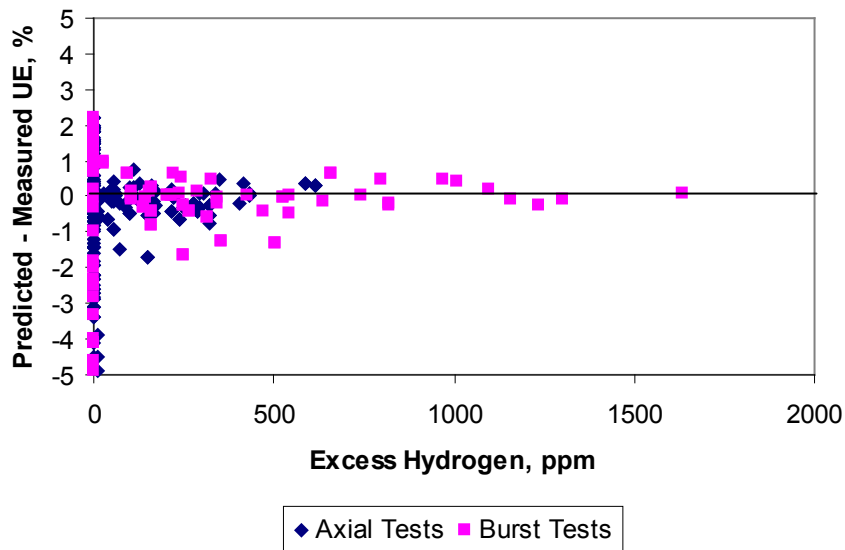
Figure 2.25 Predicted minus measured uniform elongation from irradiated samples from the PNNL database as a function of excess hydrogen ( 293\text{K} \leq T \leq 755\text{K} and 0 \leq \Phi \leq 14 \times 10^{25} \text{ n/m}^2 )
