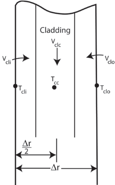
Figure 2.8 Cladding noding
