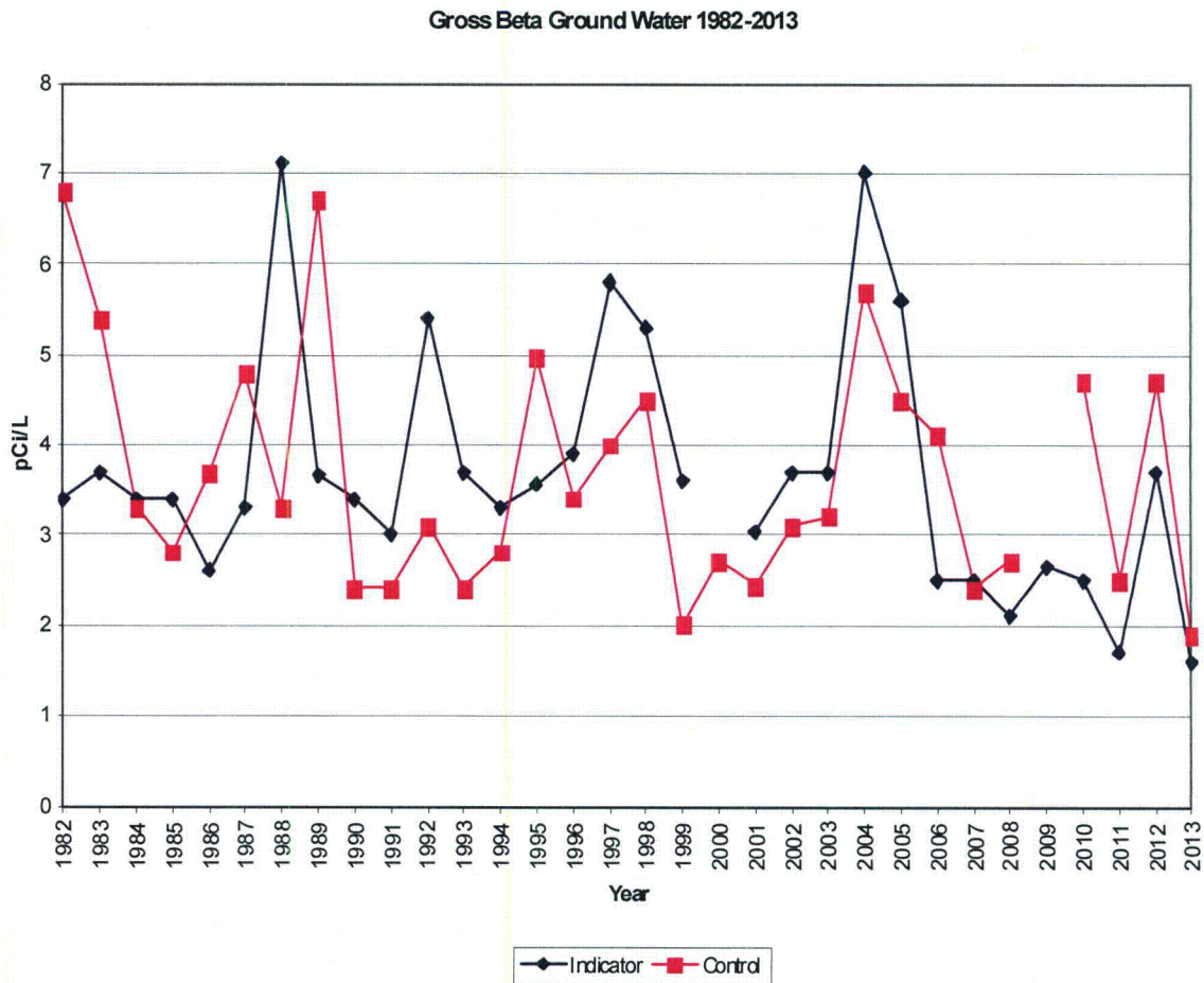
Figure 14: Shown above are the annual averages for gross beta in groundwater from 1982-2013. There were no indicator samples available in 2000 and no control samples available in 2009.
