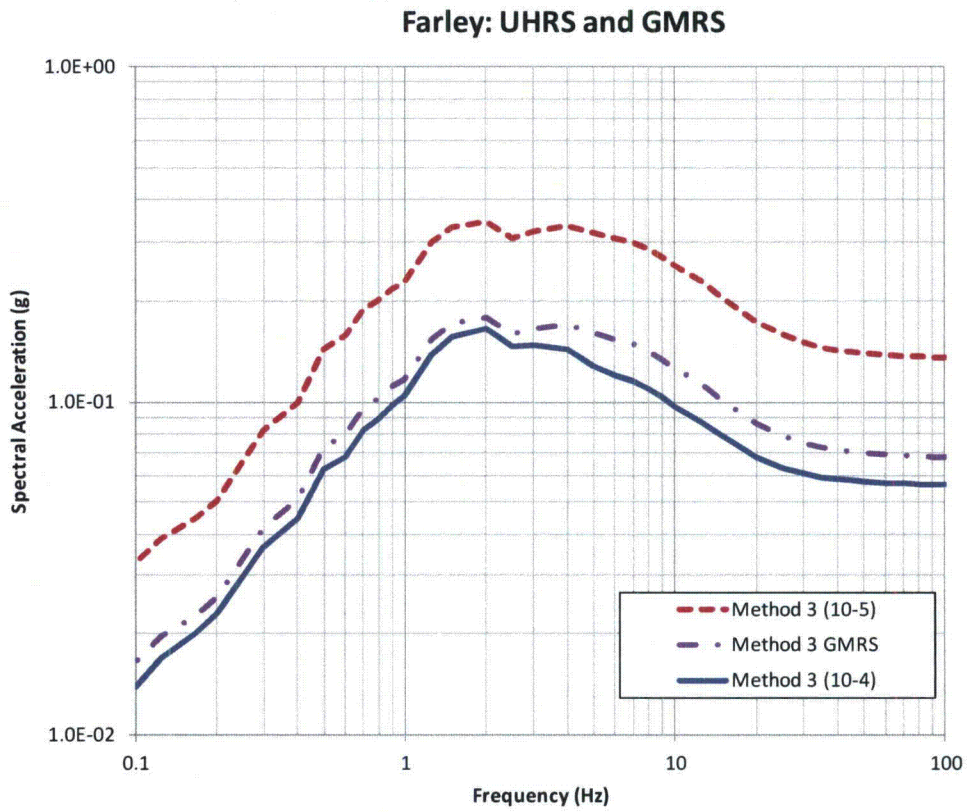
Figure 2.4-1: UHRS for 1E-4 and 1E-5 and GMRS at control point for Farley.
