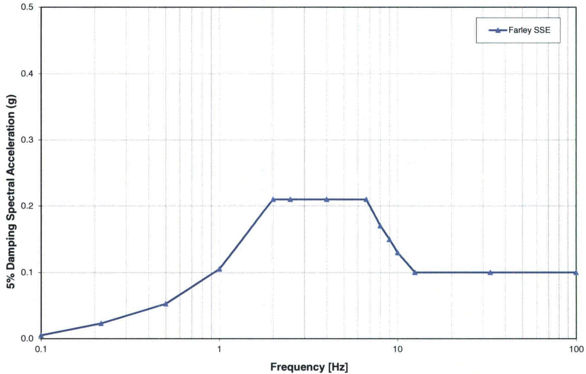
Figure 3.3-1: Horizontal SSE for Plant Farley Units 1 and 2
