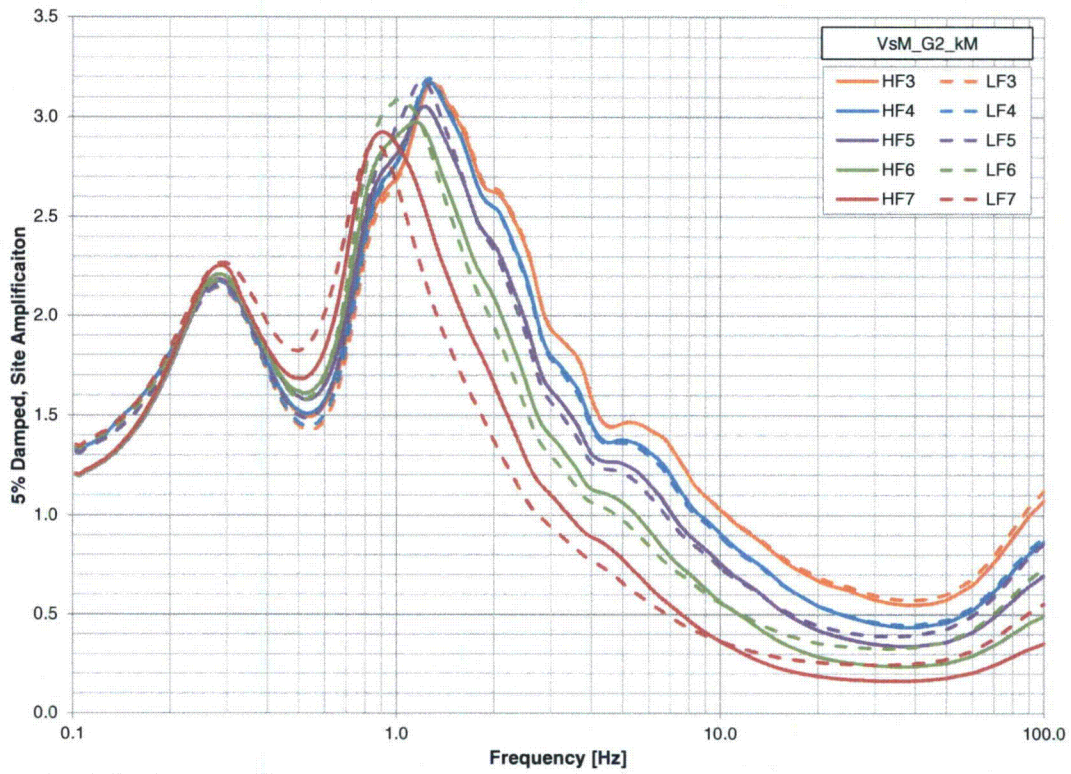
Figure 2.3.6-3: The logarithmic mean site amplification for the VsM_G2_kM site column for the considered input motions.
