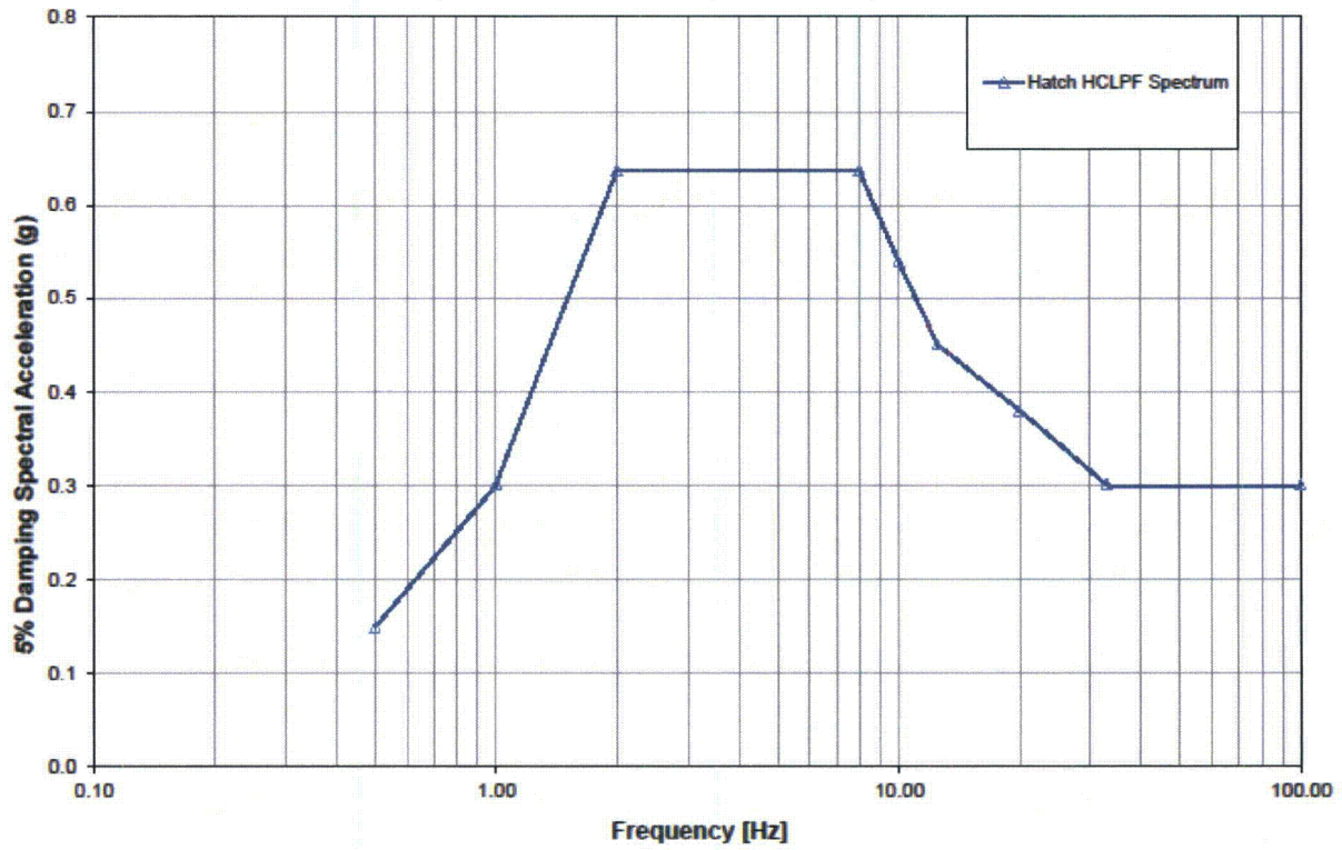
Figure 5.0-1: IPEEE HCLPF Spectrum.
