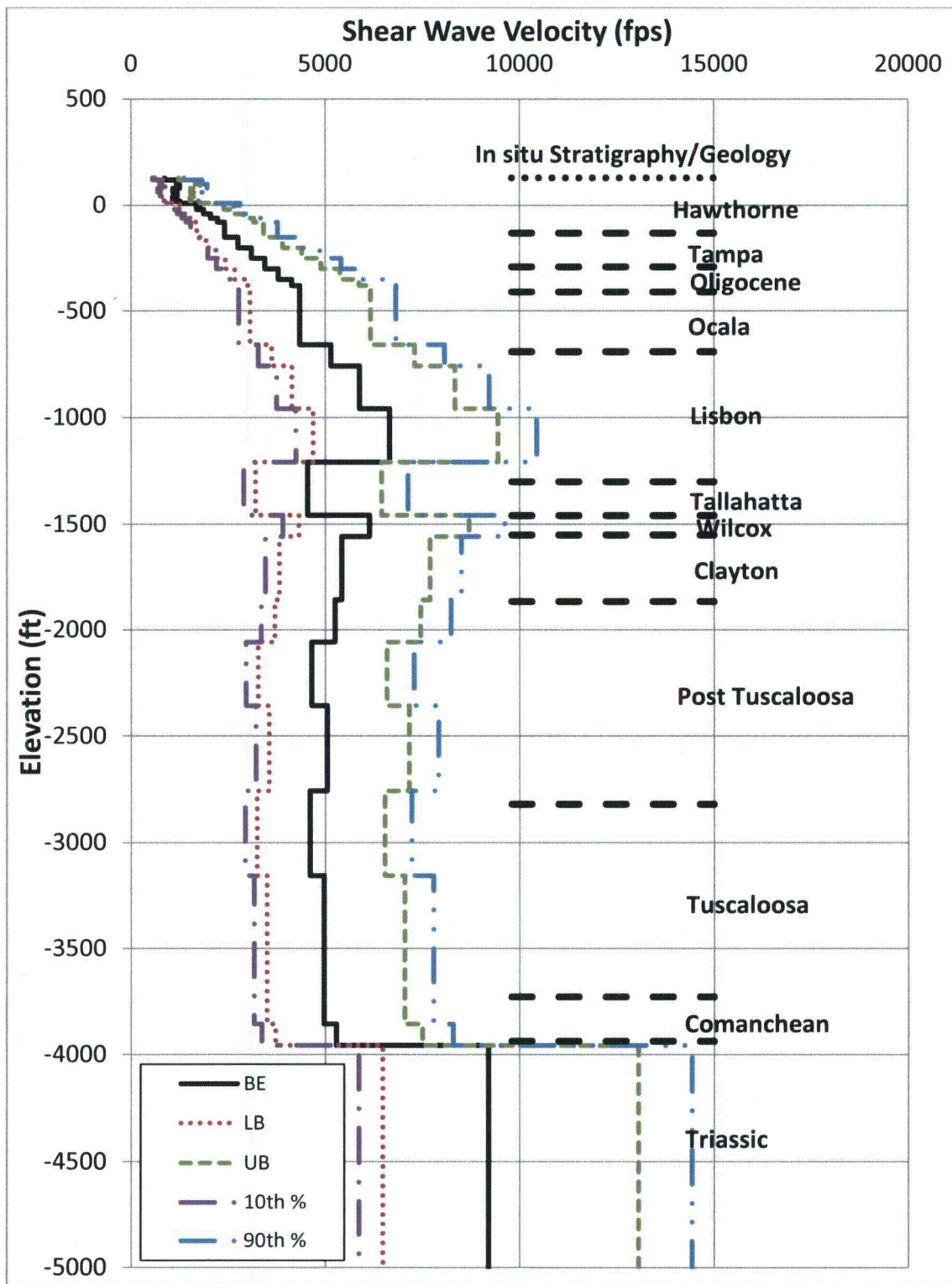
Figure 2.3.2-1: Full Depth Soil/Rock Column Shear Wave Velocity
