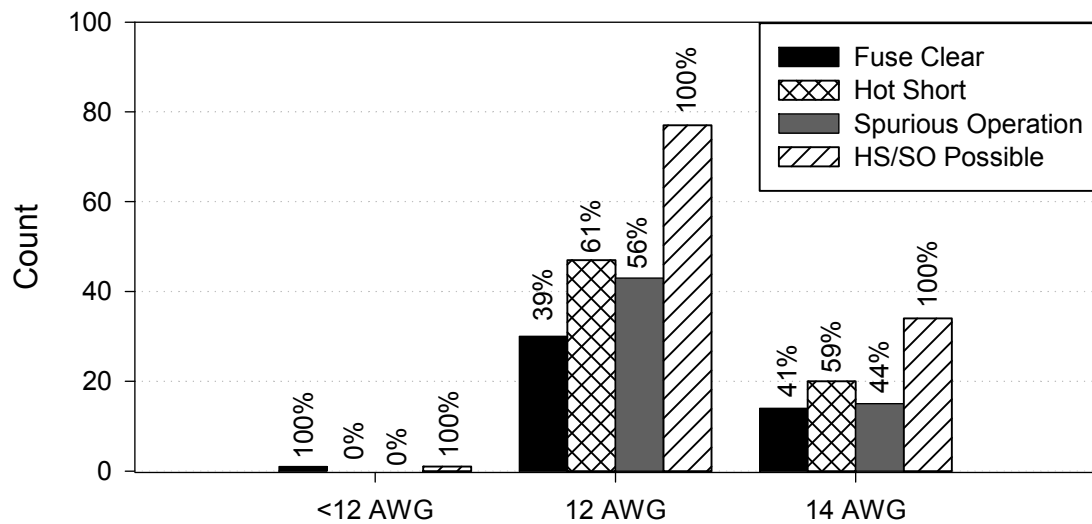
Figure 2-28. Conductor size column plot, global approach, AC tests
