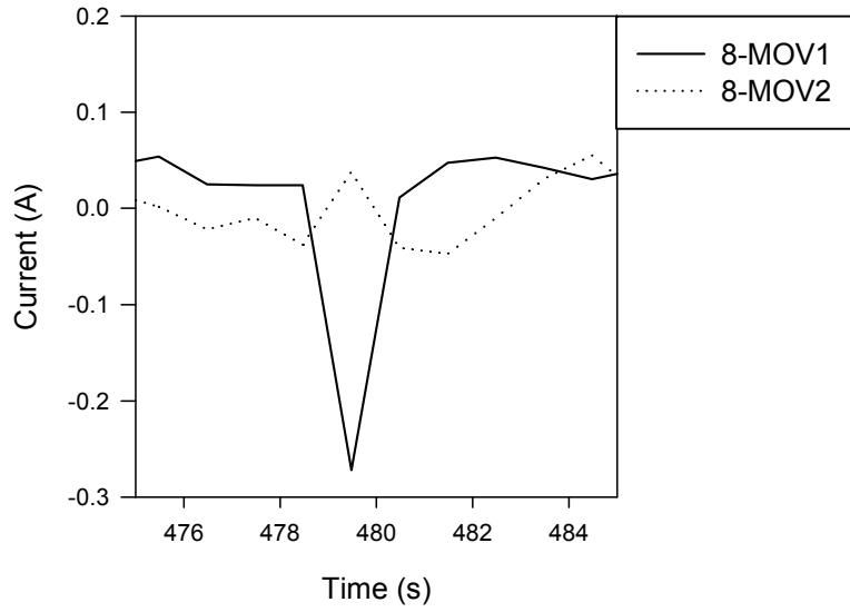
Figure A-1: Outstanding current shorting in Penlight MOV test #8
