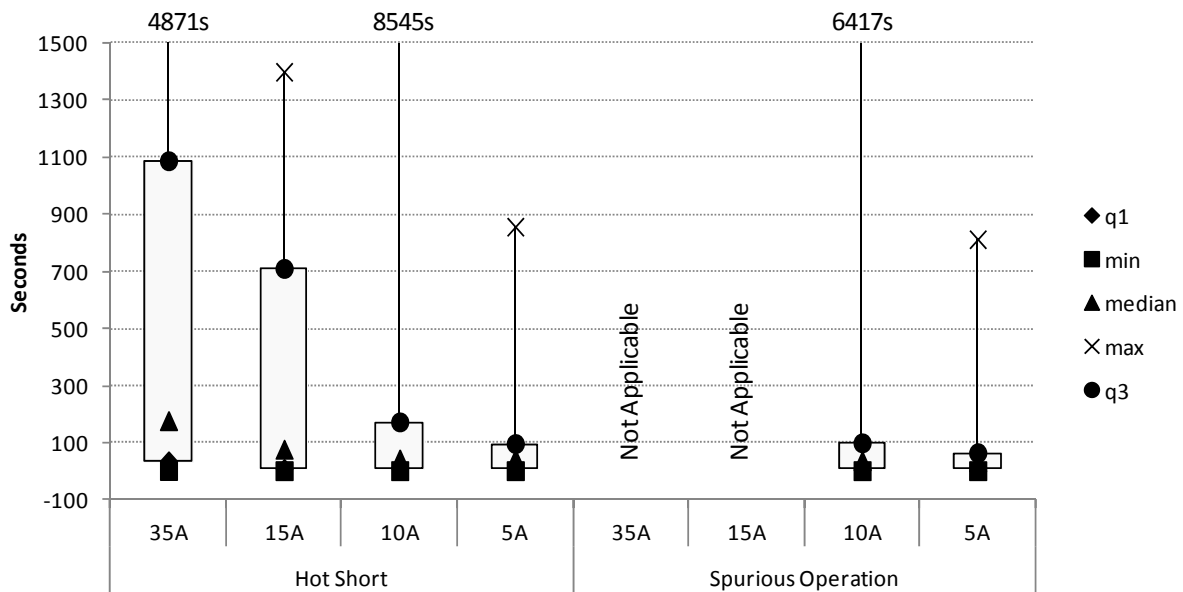
Figure 4-32. Fuse size box plot, duration, DC tests
