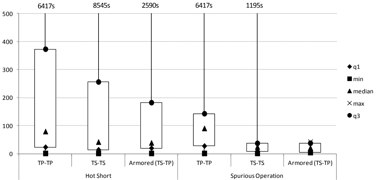
Figure 4-24. Insulation-jacket type box plot, duration, DC tests
