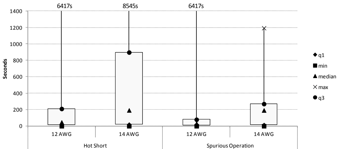
Figure 4-28. Conductor size box plot, duration, DC tests
