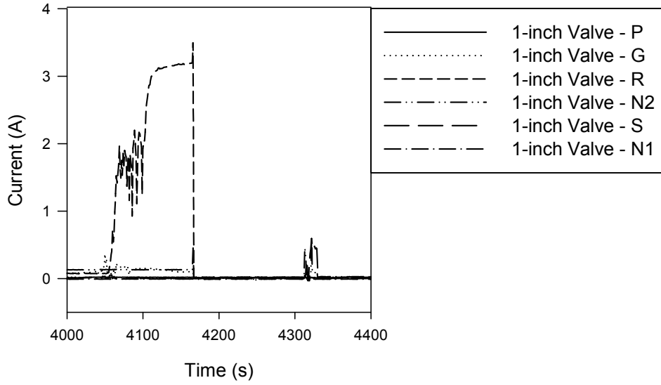
Figure A-41. Penlight 1-inch valve Test #40 current plot
