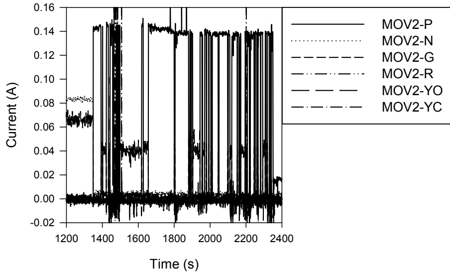
Figure A-6: Penlight MOV-2 test #12 current plot
