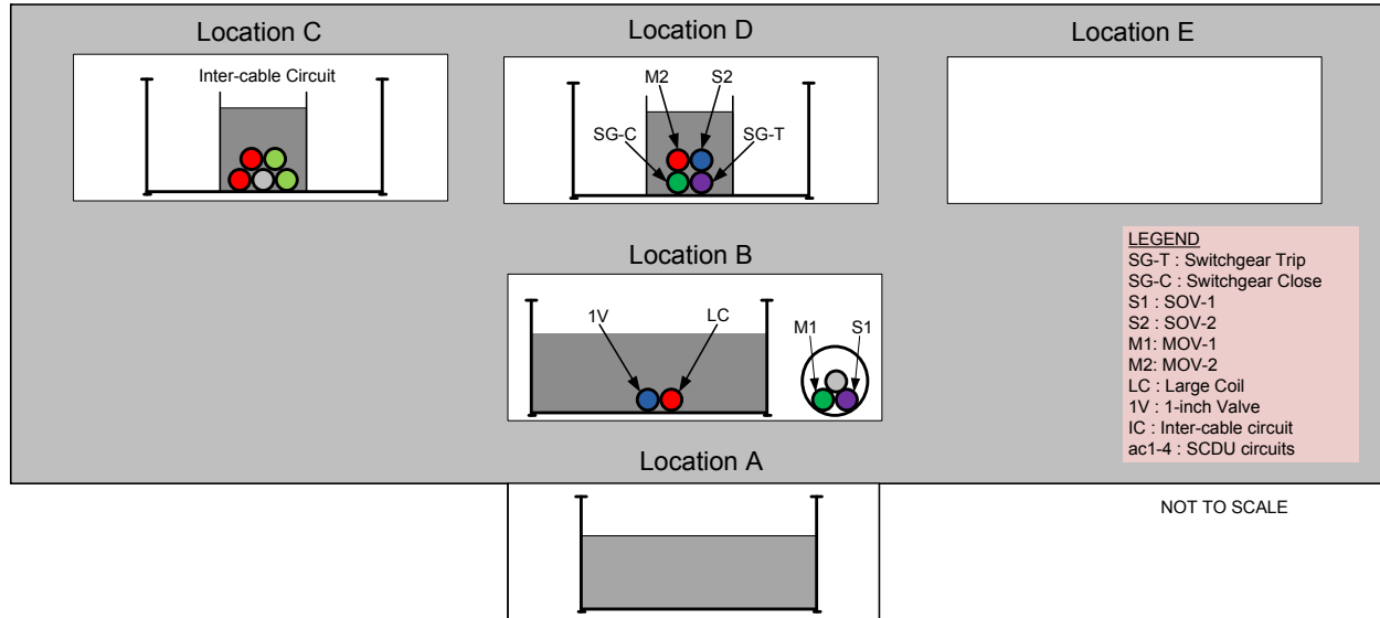
Figure 5-16. Intermediate-scale test 5 cable loading
