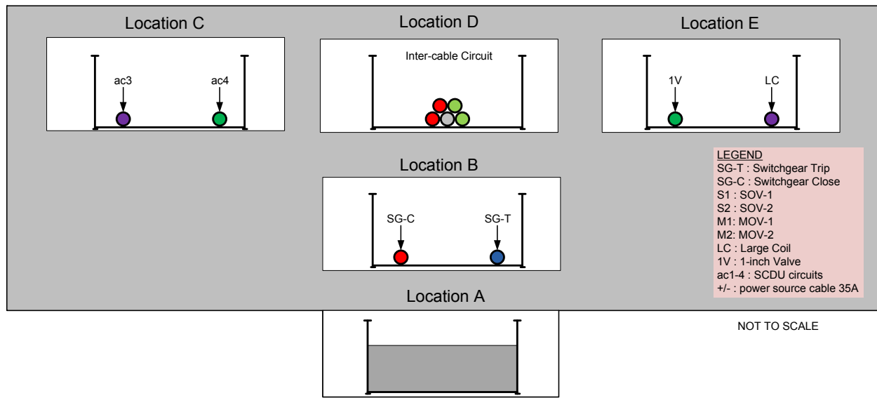
Figure 5-5. Intermediate-scale test preliminary 1 cable loading configuration
