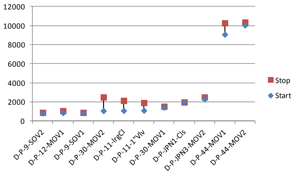
Figure 4-43. Time plot of concurrent spurious operations for DESIREE-FIRE among all Penlight test with exposure temperatures in the range of 325-375°C
