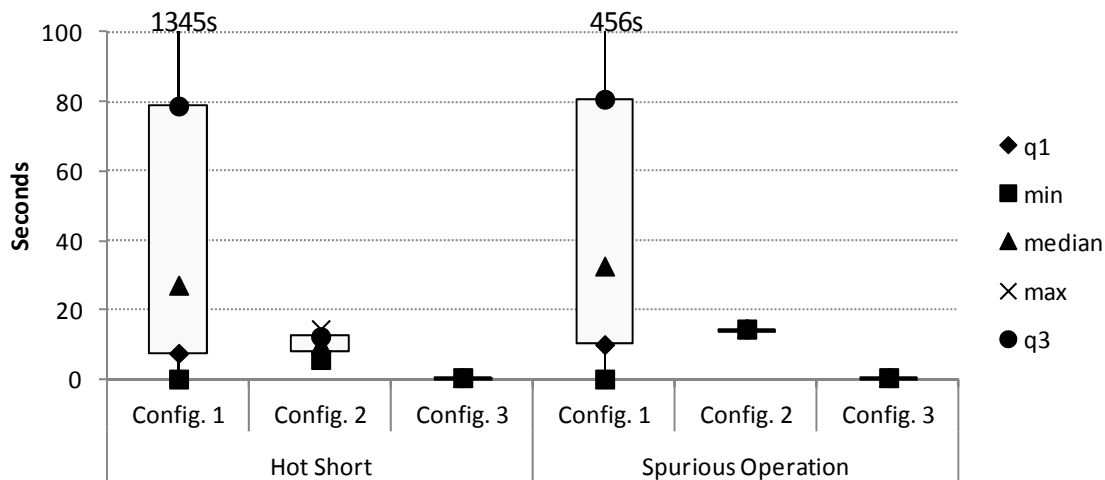
Figure 2-27. Wiring configuration box plot, duration, AC tests
