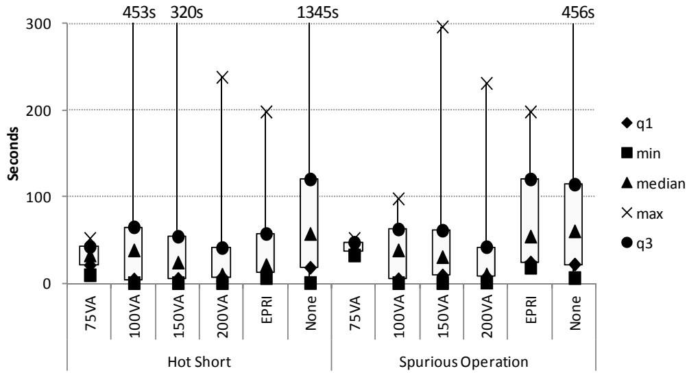
Figure 2-23. CPT size box plot, duration, AC tests
