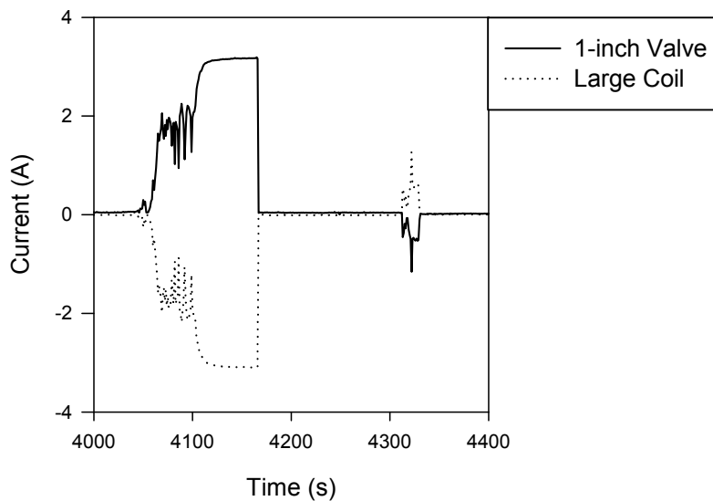
Figure A-40. Outstanding current shorting in Penlight 1-inch valve and large Coil Test #40
