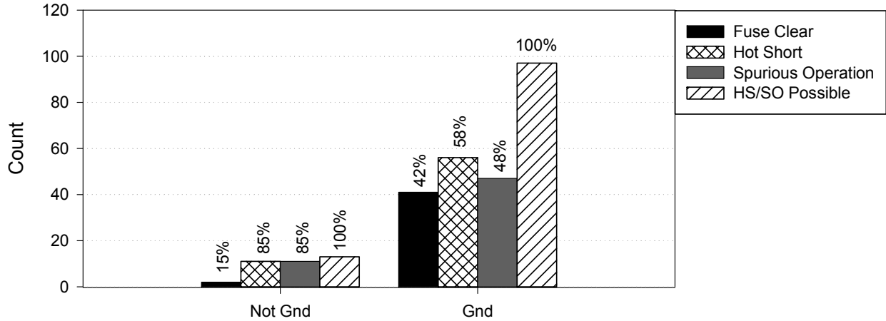
Figure 2-24. Circuit grounding column plot, global approach, AC tests
