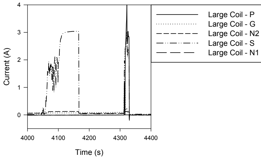
Figure A-42. Penlight large coil Test #40 current plot
