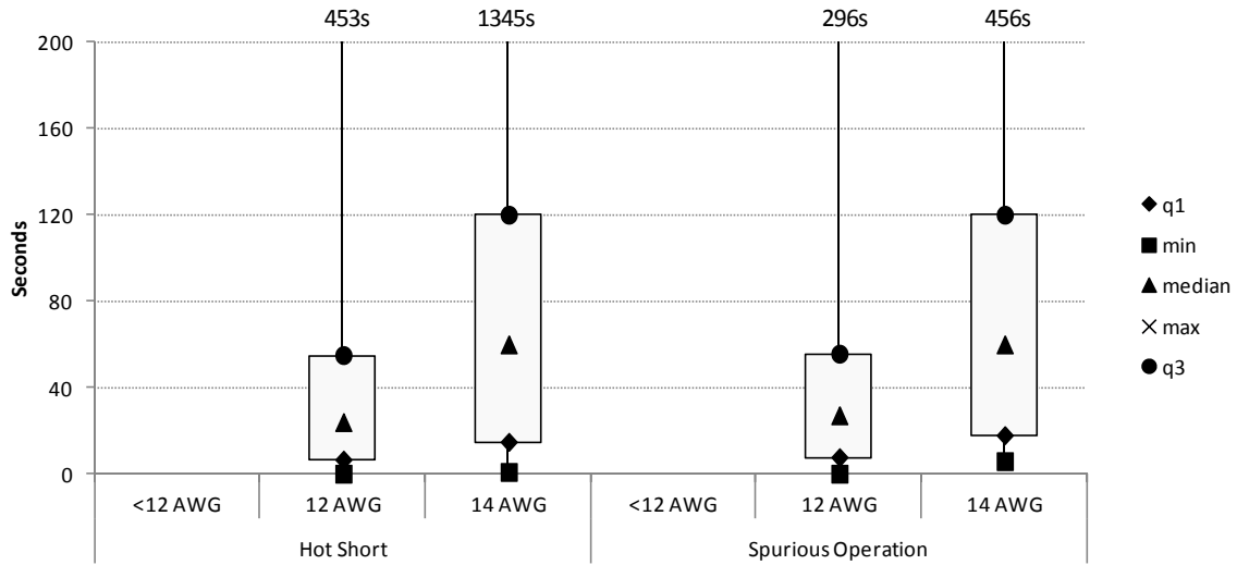
Figure 2-29. Conductor size box plot, duration, AC tests
