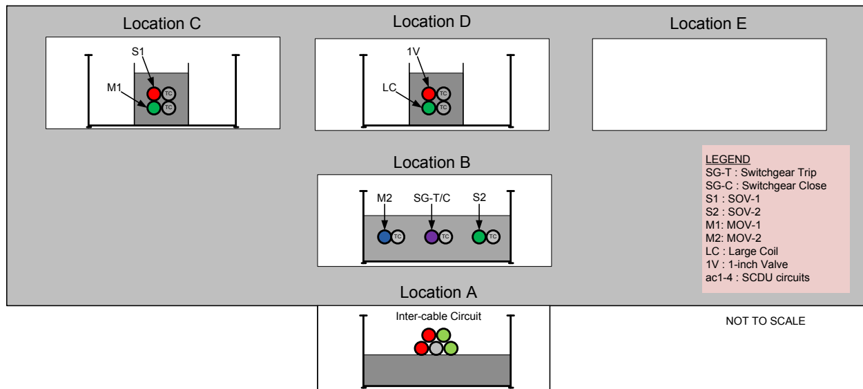
Figure 5-23. Intermediate-scale test 10 cable loading
