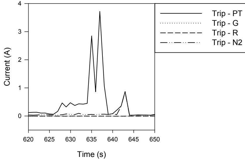
Figure A-45 Penlight SWGR Trip Test #4 current plot
