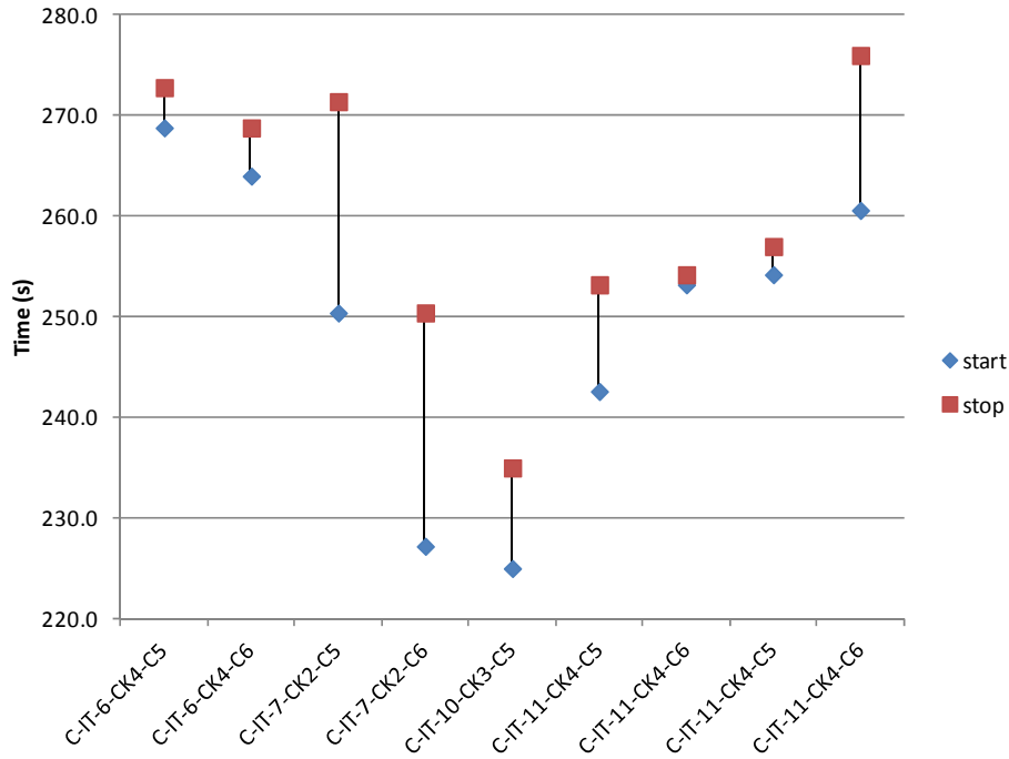
Figure 2-33. Concurrent hot shorts - Location A - 4 cables
