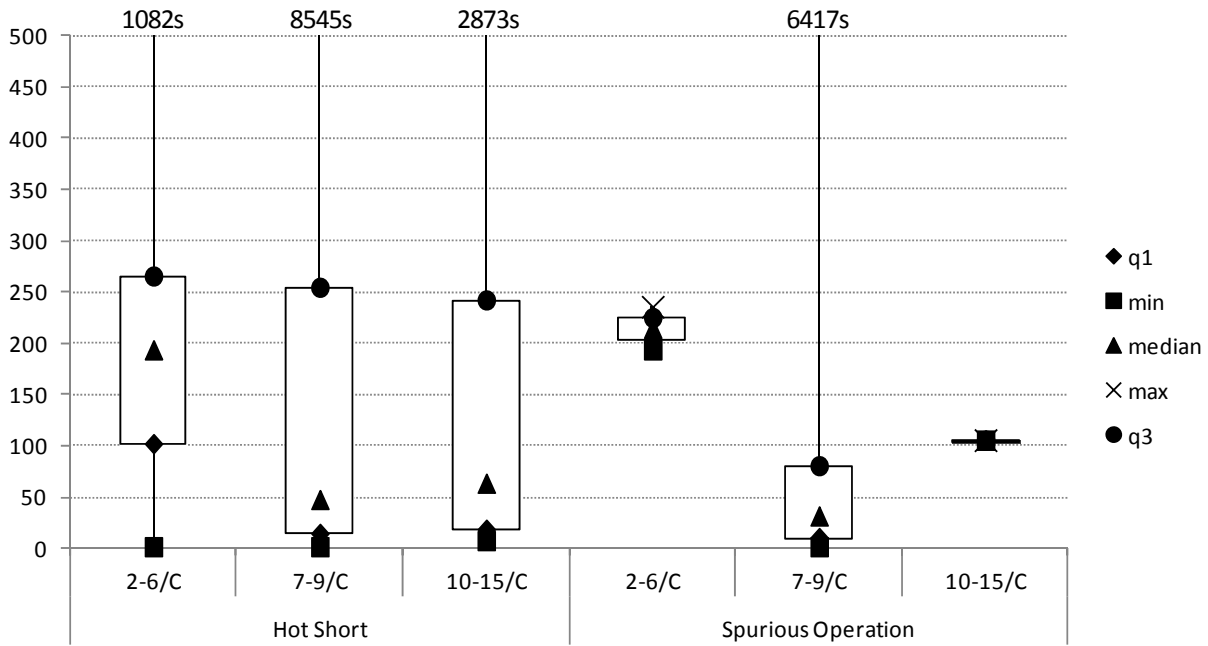
Figure 4-8. Conductor count box plot, duration, DC tests
