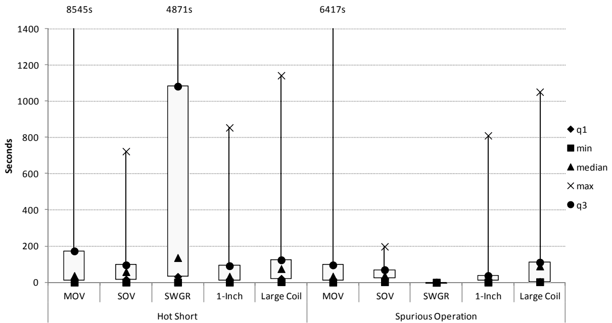
Figure 4-30. Circuit type box plot, duration, DC tests
