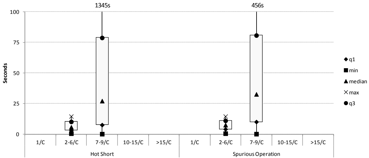
Figure 2-3. Conductor count box plot, duration, AC tests
