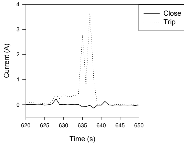
Figure A-43. Outstanding current shorting in Penlight SWGR Test #4
