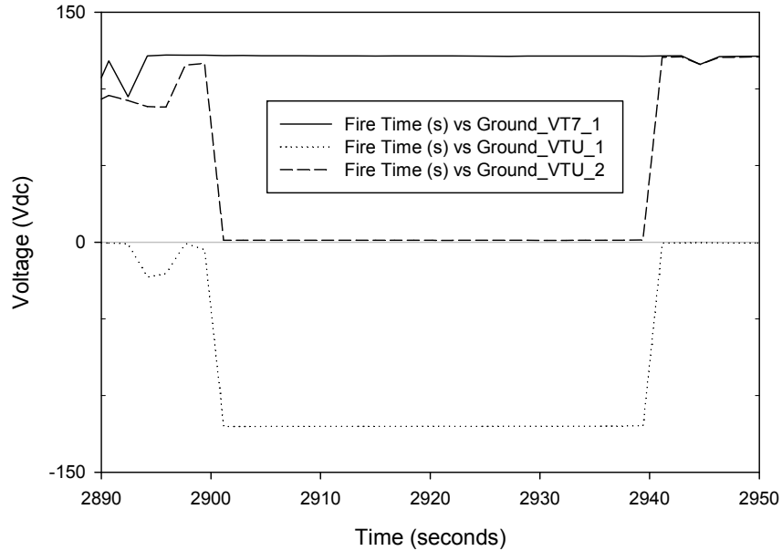
Figure 5-28. Ground fault detection voltage response for second large coil SO
