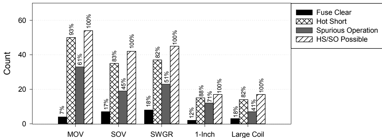
Figure 4-29. Circuit type column plot, global approach, DC tests
