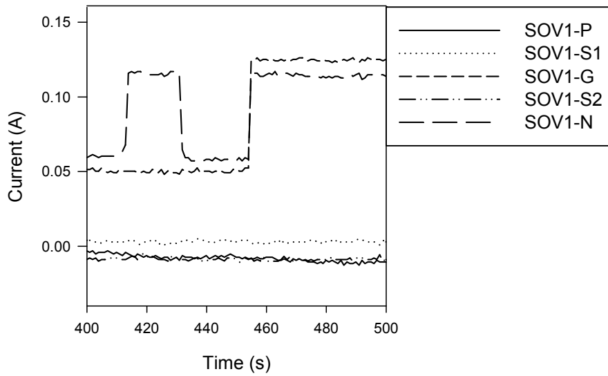
Figure A-35. Penlight SOV-1 Test #31 current plot
