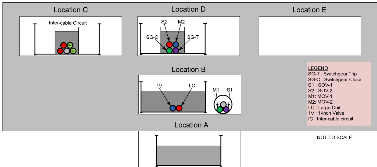
Figure 5-8. Intermediate-scale test 1 cable loading configuration
