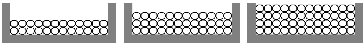
Figure 2-12. Cable tray fill intermediate
