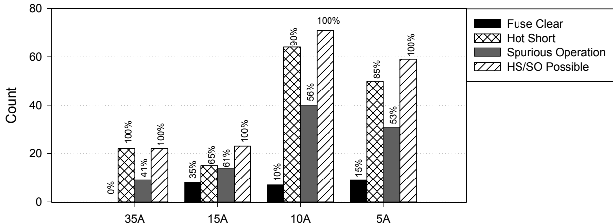
Figure 4-31. Fuse size column plot, global approach, DC tests
