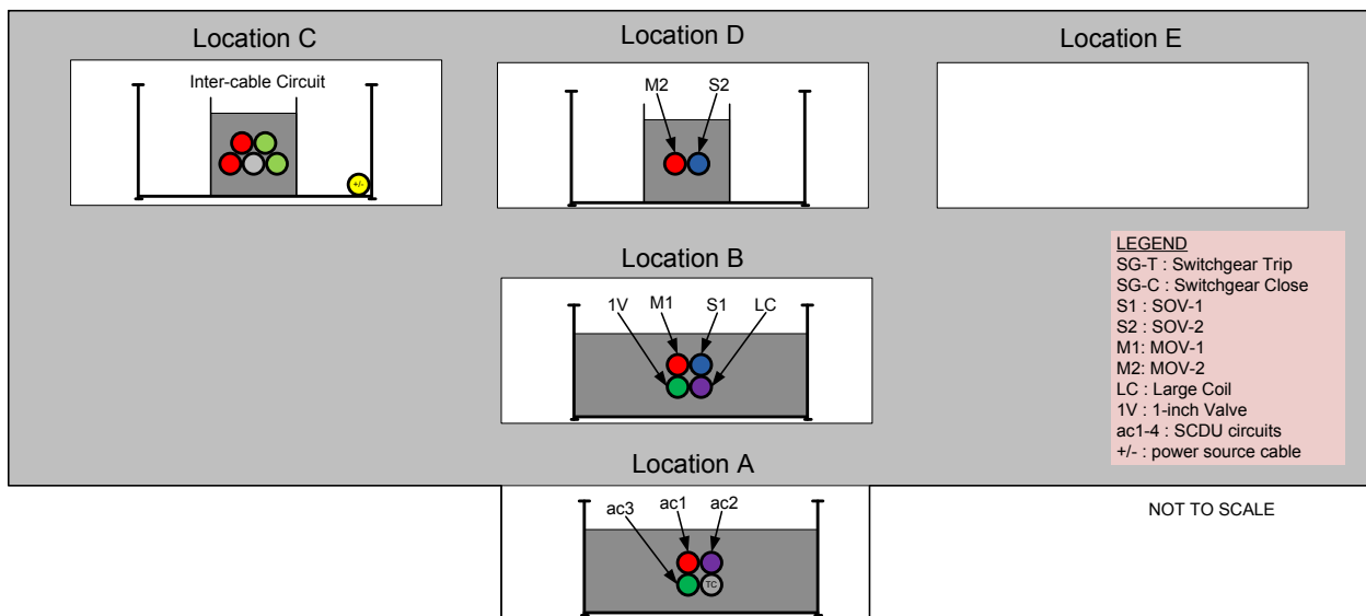
Figure 5-24. Intermediate-scale test 11 cable loading
