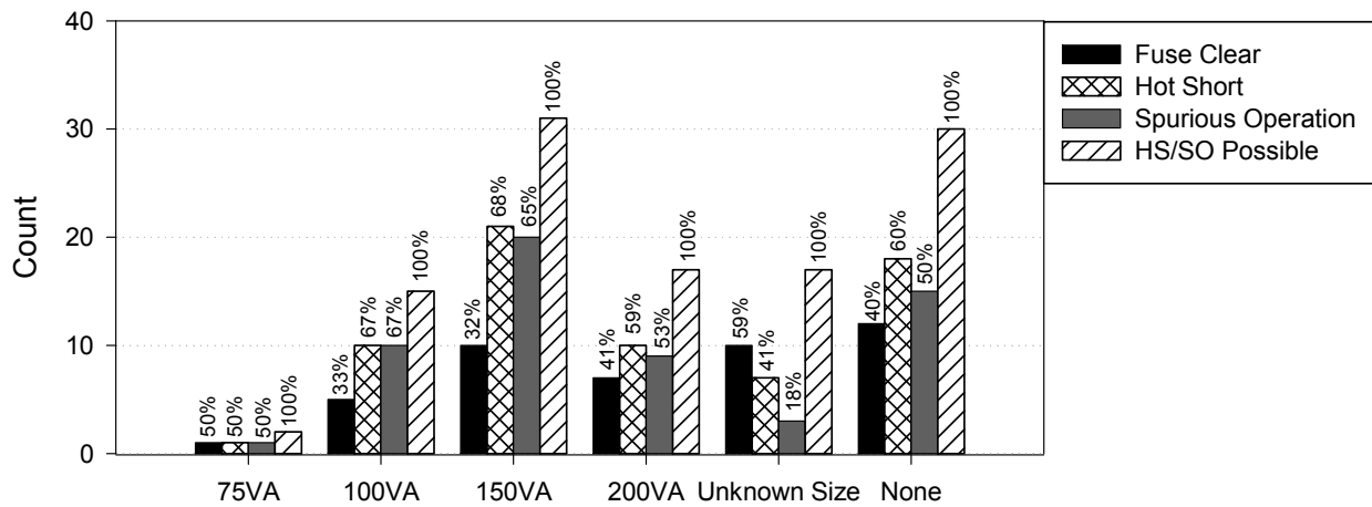
Figure 2-22. CPT size column plot, global approach, AC tests
