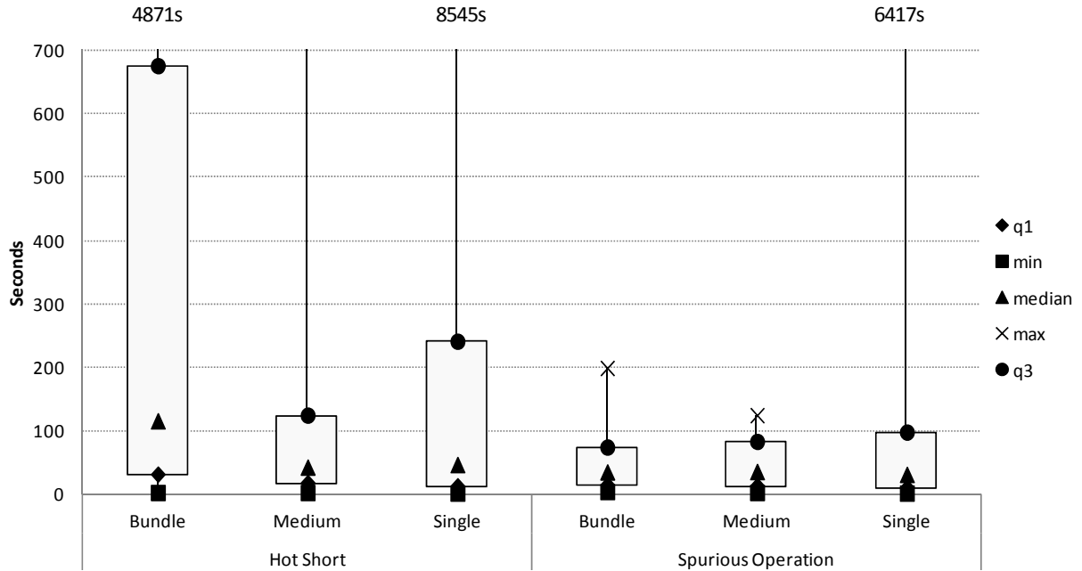
Figure 4-18. Raceway fill box plot, duration, DC tests
