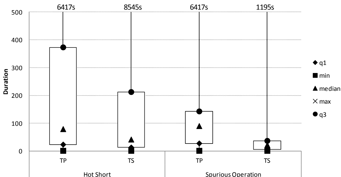
Figure 4-20. Insulation type box plot, duration, DC tests
