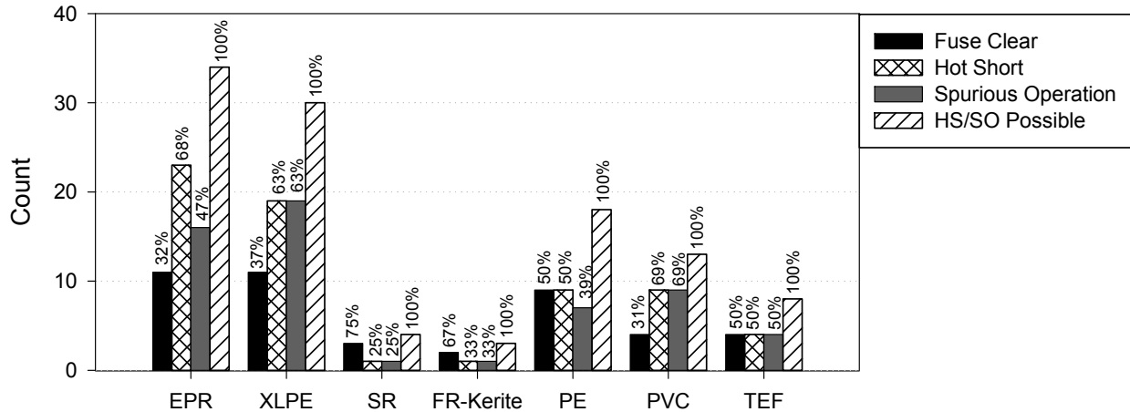
Figure 2-18. Insulation material column plot, global approach, AC tests
