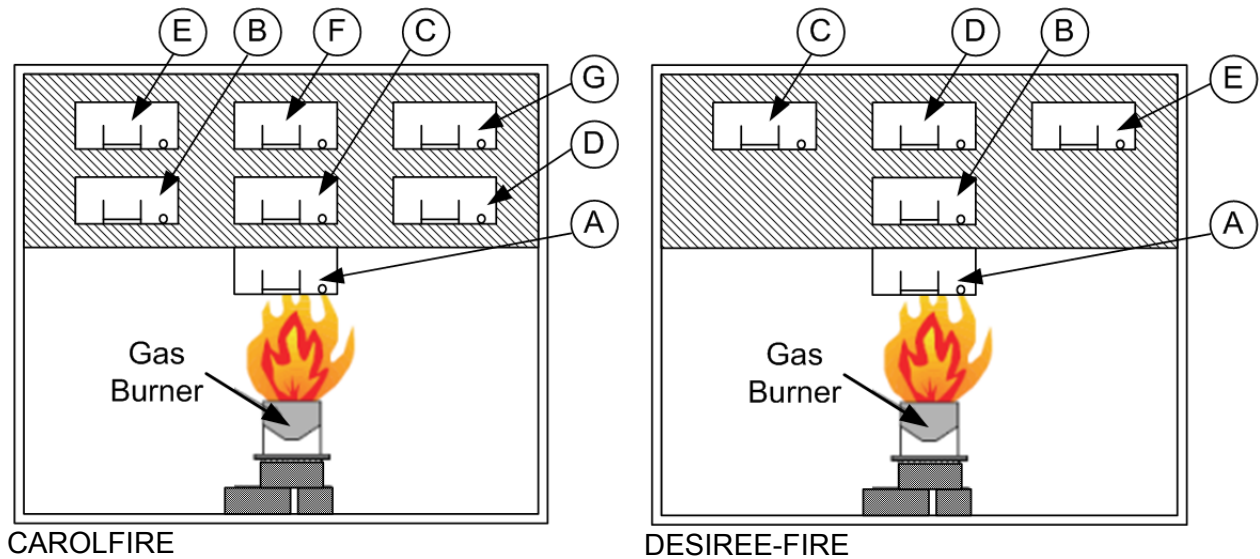
Figure 2-4. Intermediate-scale cable raceway location
