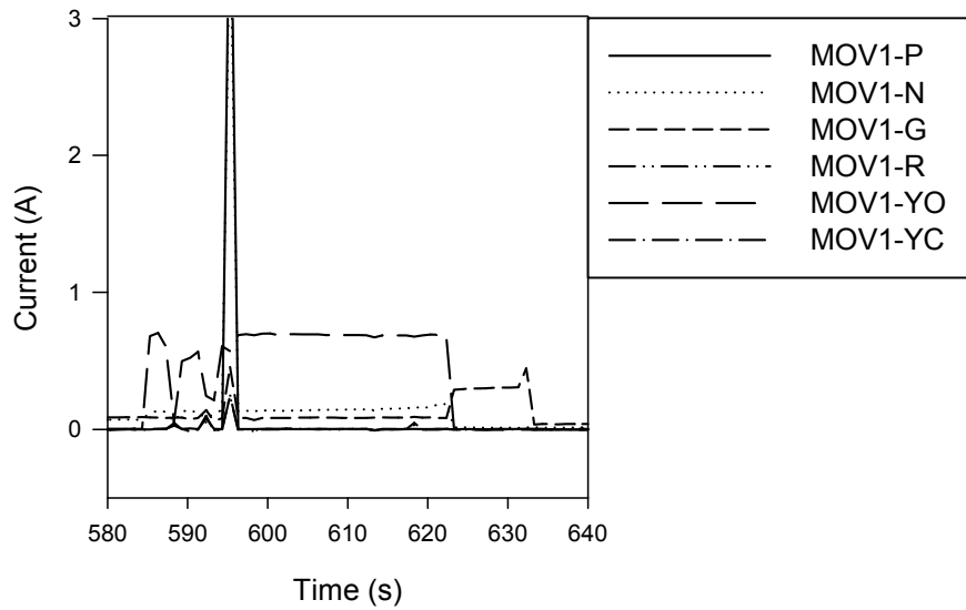
Figure A-8: Penlight MOV-1 test #22 current plot
