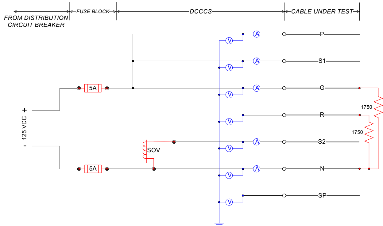
Figure 4-4. Line drawing for DC SOV circuit
