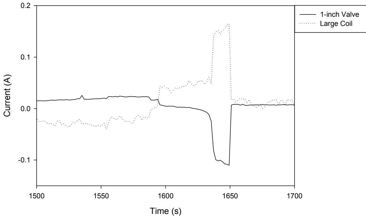
Figure 5-17. Outstanding current shorting in intermediate-scale test 5, between SOV-1 and SWGR-T
