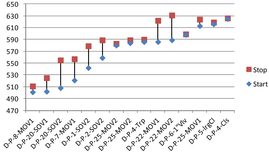
Figure 4-44. Time plot of concurrent spurious operations for DESIREE-FIRE among all Penlight test with exposure temperatures in the range of 400-480°C
