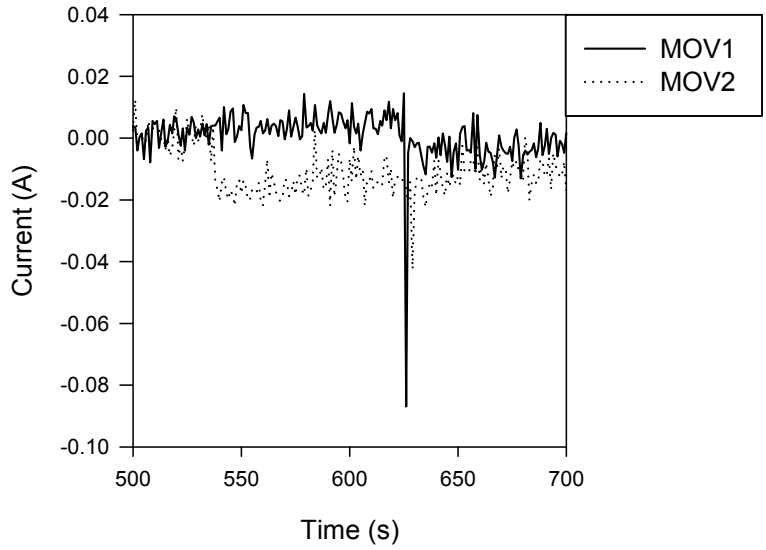
Figure A-10: Outstanding current shorting in Penlight MOV test #33
