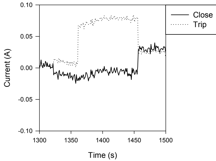
Figure A-46. Outstanding current shorting in Penlight SWGR Test #JPN-2
