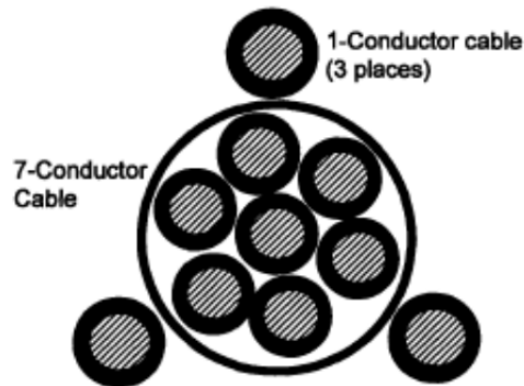
Figure 3-3. NEI/EPRI cable configuration
