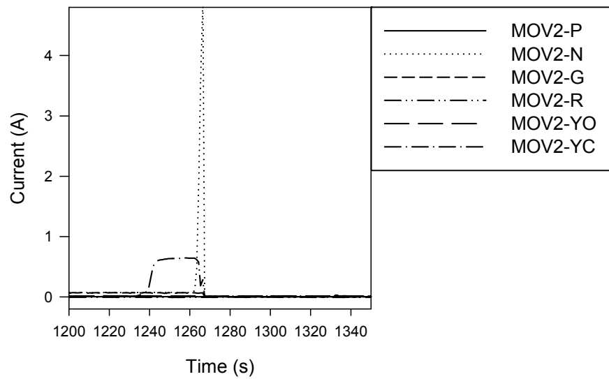
Figure A-24. Penlight MOV-2 Test #50 current plot
