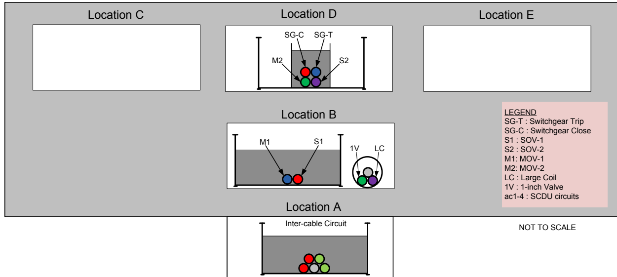
Figure 5-19. Intermediate-scale test 7 cable loading
