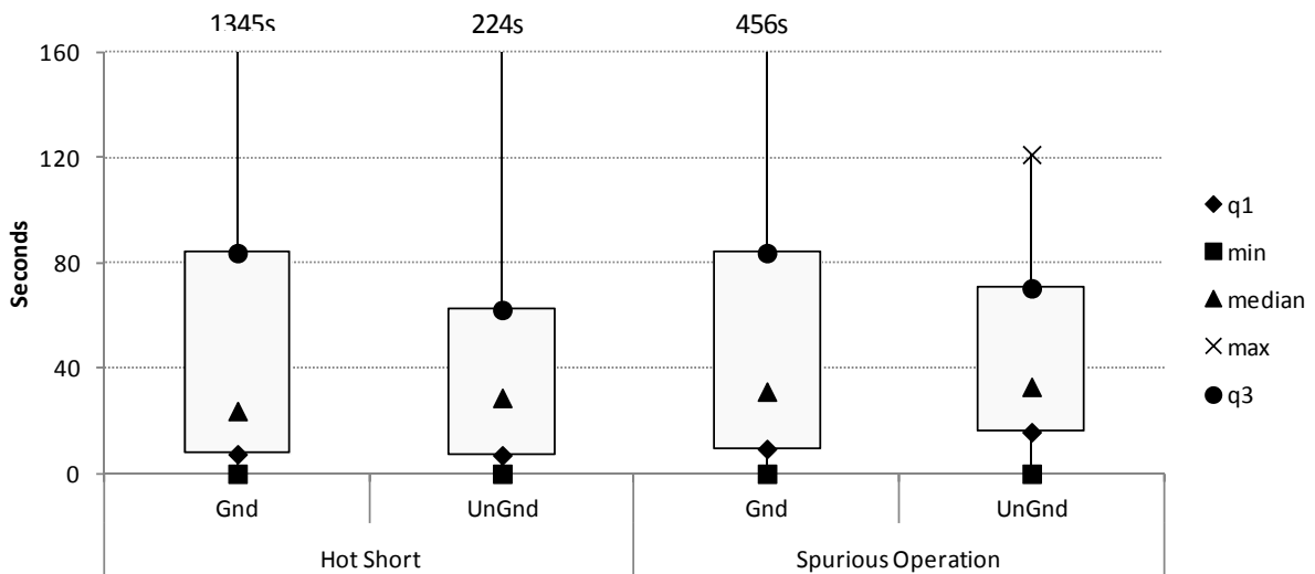
Figure 2-25. Circuit grounding box plot, duration, AC tests
