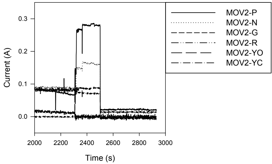
Figure A-27. Penlight MOV-2 Test # JPN-3 current plot
