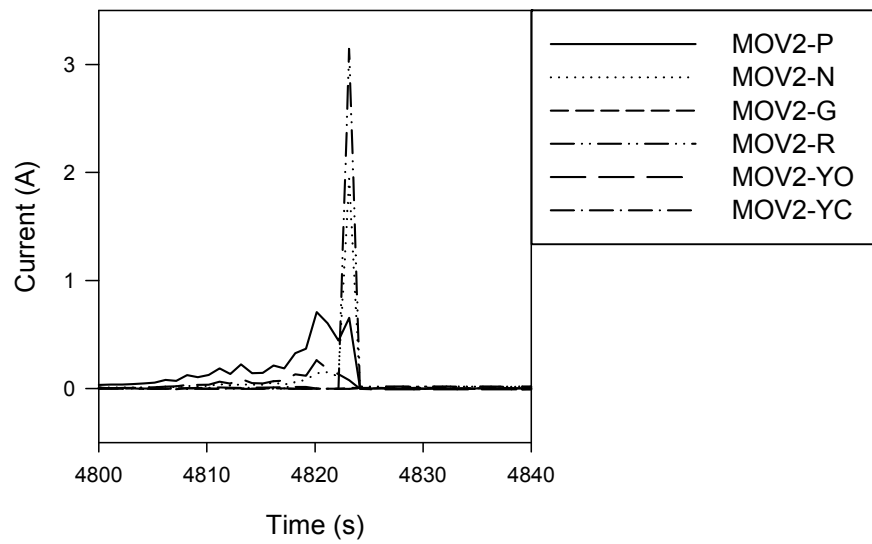
Figure A-21. Penlight MOV-2 Test #49 current plot
