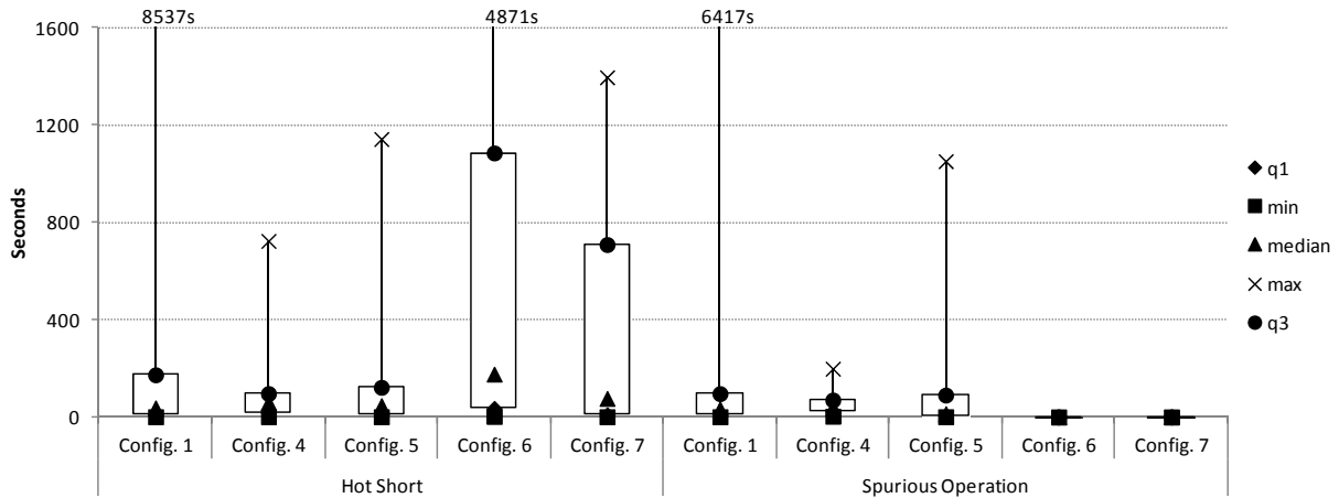
Figure 4-26. Wiring configuration box plot, duration, DC tests
