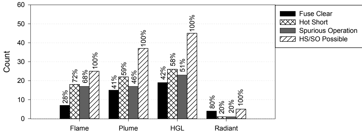
Figure 2-5. Thermal exposure conditions column plot, global approach, AC tests
