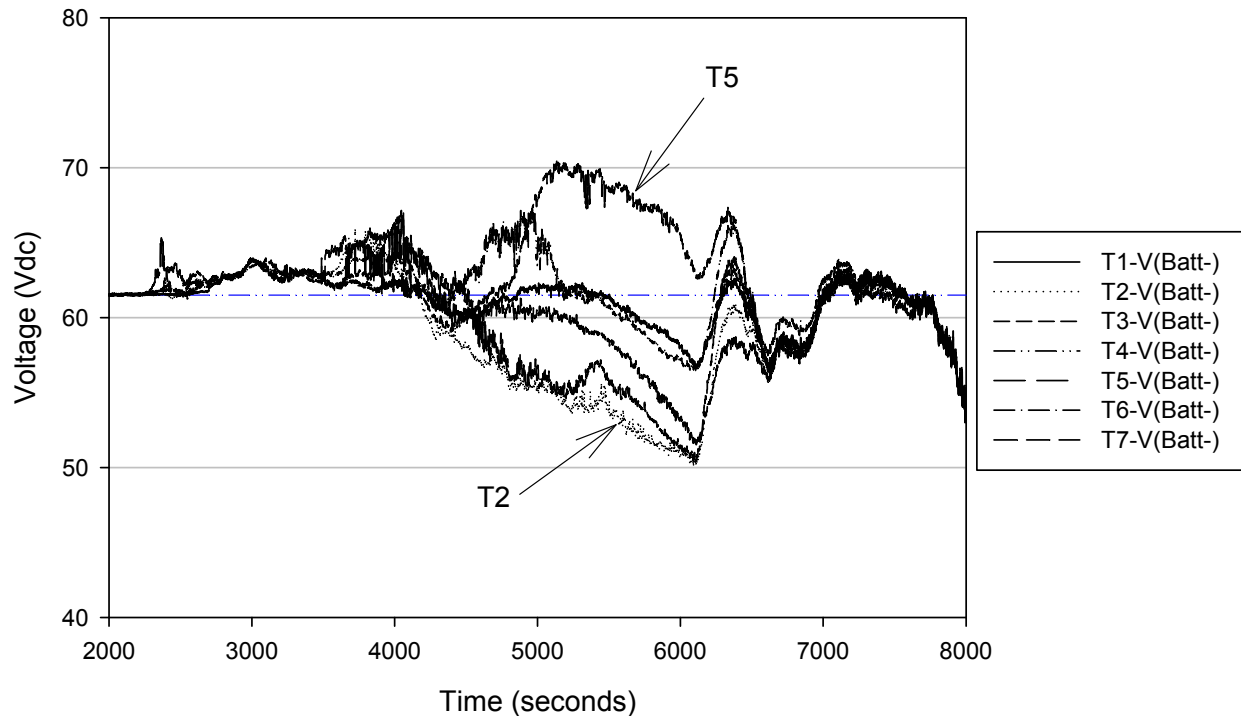
Figure 5-2. DESIREE-FIRE inter-cable test results penlight test 47
