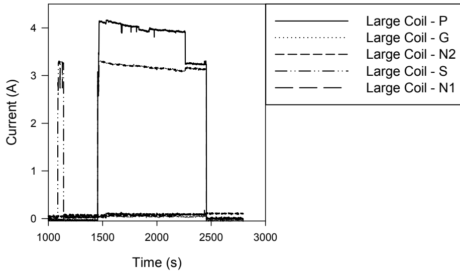
Figure A-39. Penlight large coil Test #11 current plot
