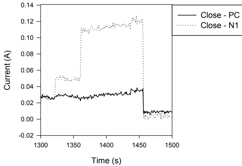
Figure A-47. Penlight SWGR Close Test #JPN-2 current plot
