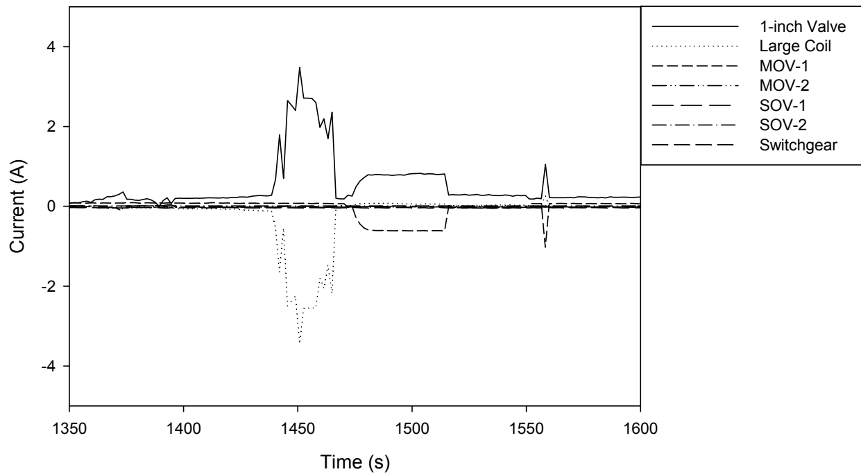
Figure 5-9. Outstanding current hot shorting for intermediate-scale test 1 between 1-inch valve, large coil, and MOV-1 circuits
