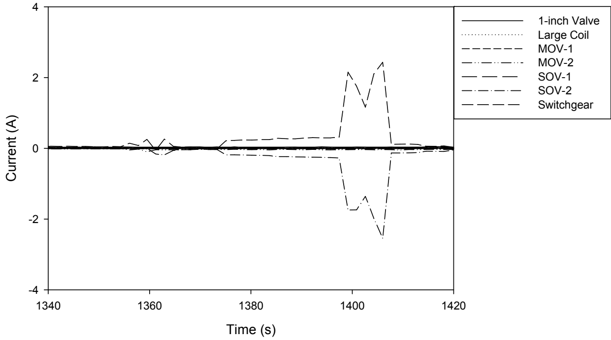
Figure 5-13. Outstanding current shorting in intermediate-scale test 3, between SOV-2 and SWGR-T
