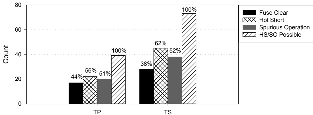
Figure 2-16. Insulation type column plot, global approach, AC tests
