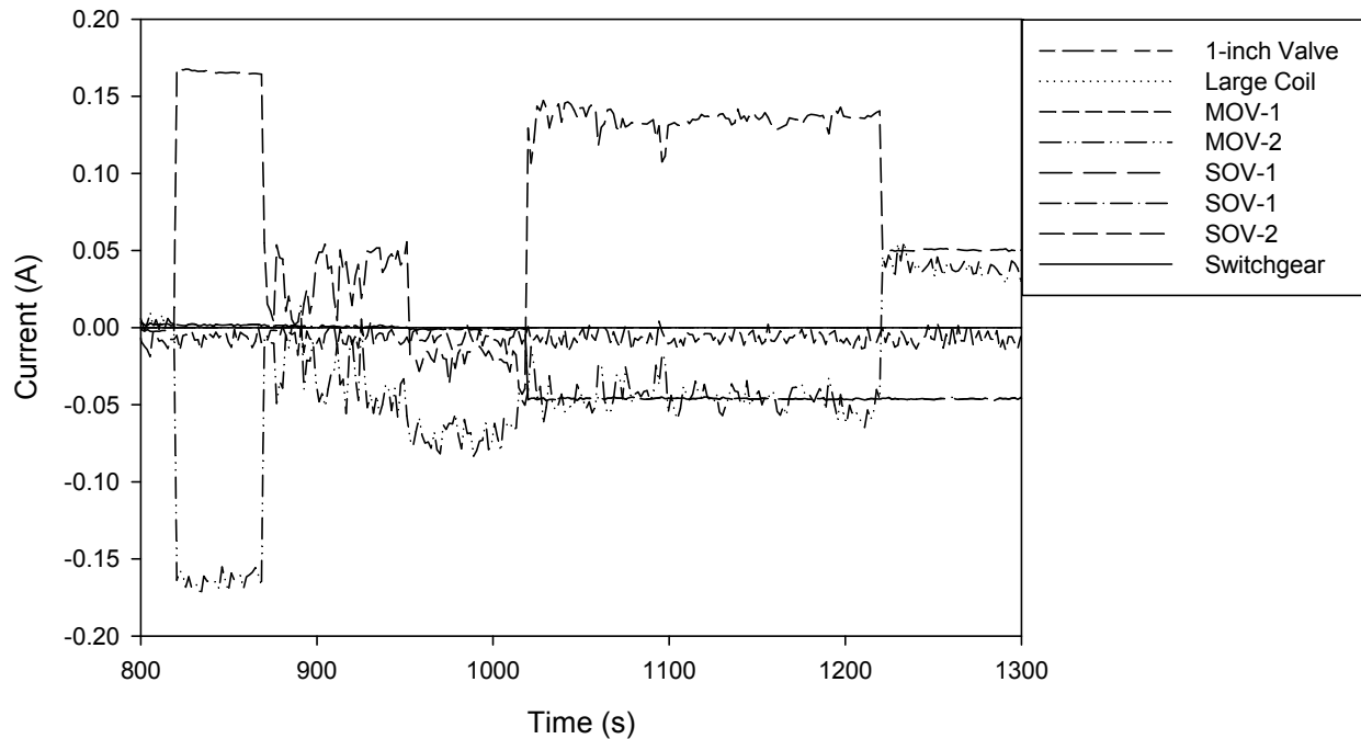
Figure 5-7. Intermediate-scale test preliminary 2 – inter-cable shorting between SOV-2 and MOV-2
