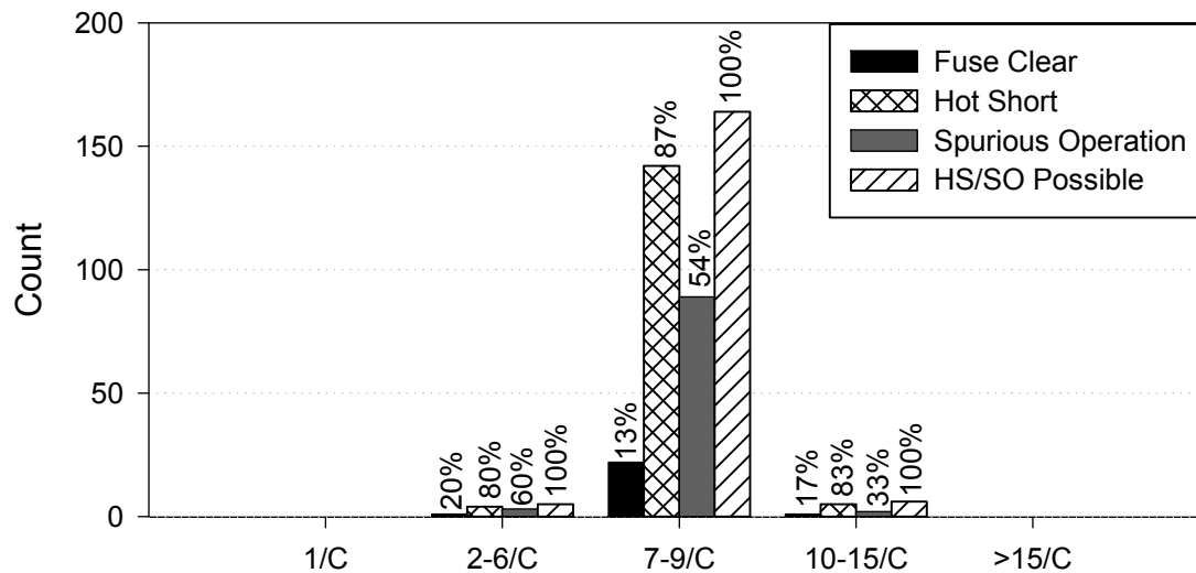
Figure 4-7. Conductor count column plot, global approach, DC tests
