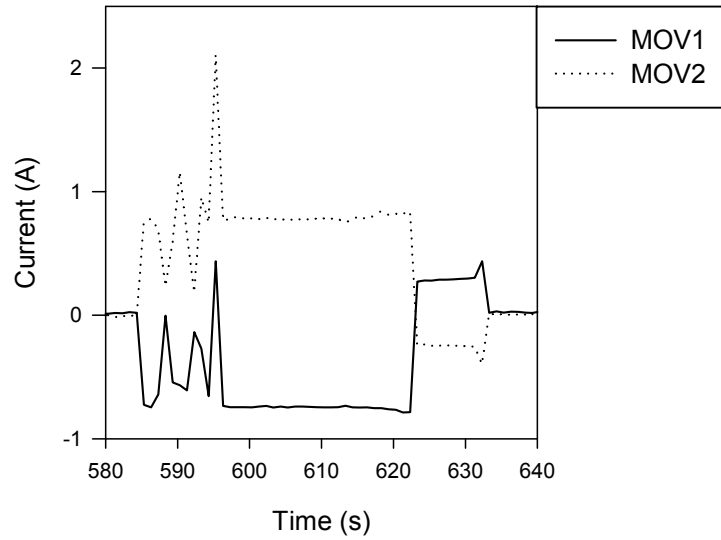
Figure A-7: Outstanding current shorting in Penlight MOV test #22
