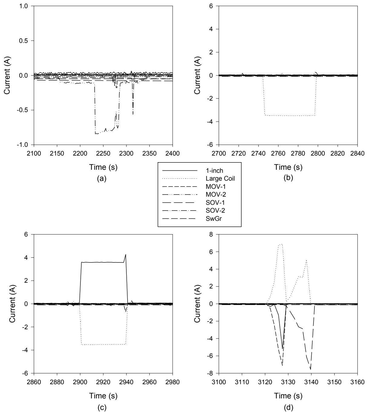
Figure 5-27. Intermediate-scale test 12 current summation plot
