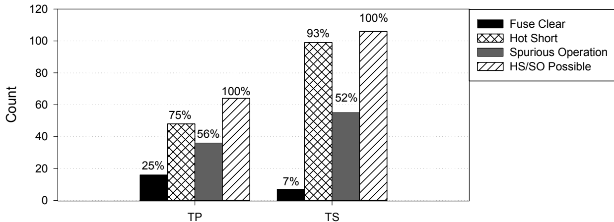
Figure 4-19. Insulation type column plot, global approach, DC tests
