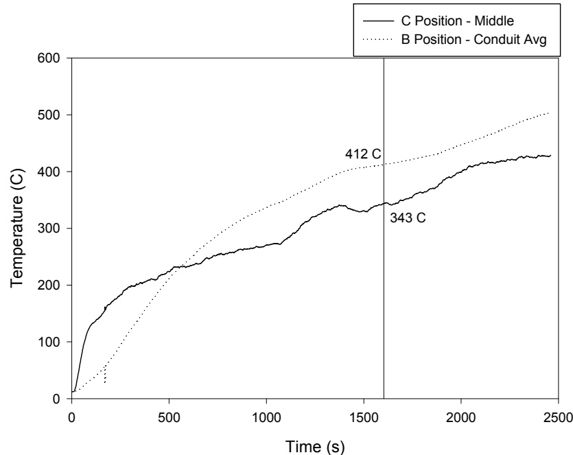
Figure 4-38. Plot of intermediate-scale test 6 for 1-inch valve and switchgear cable locations
