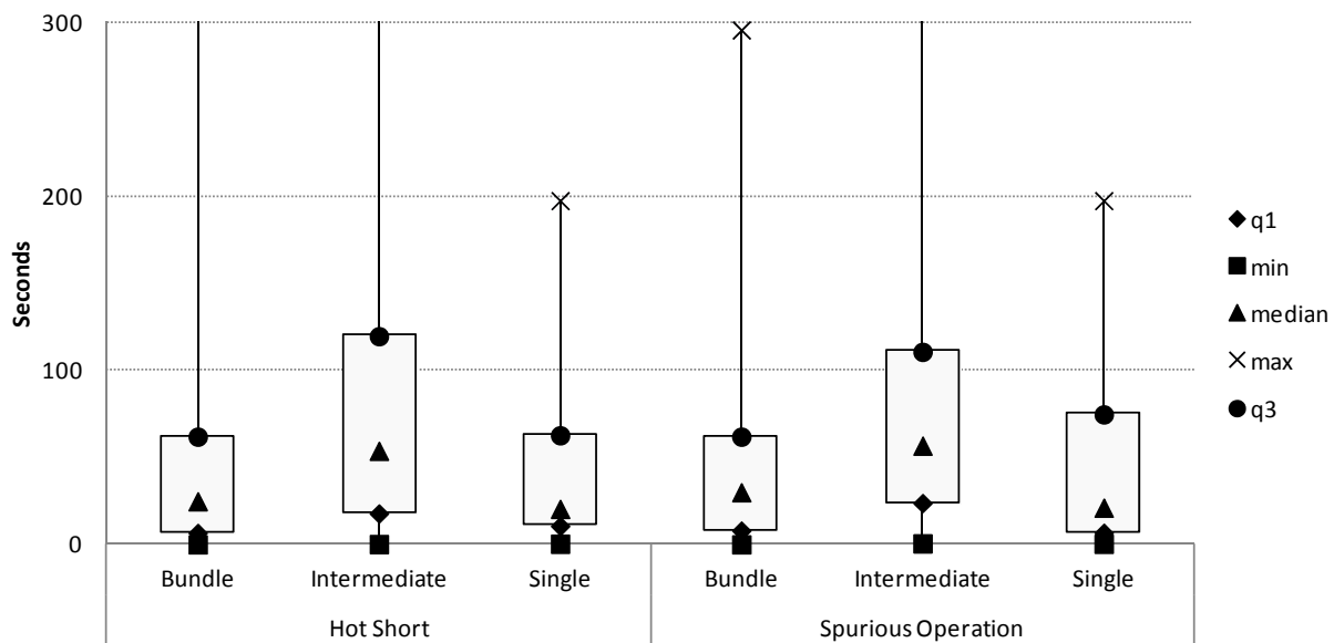
Figure 2-15. Raceway fill box plot, duration, AC tests
