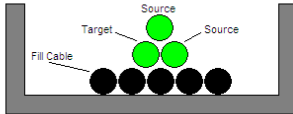
Figure 3-2. CAROLFIRE inter-cable test tray fill
