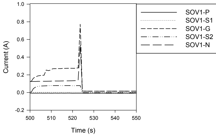
Figure A-29. Penlight SOV-1 Test #20 current plot
