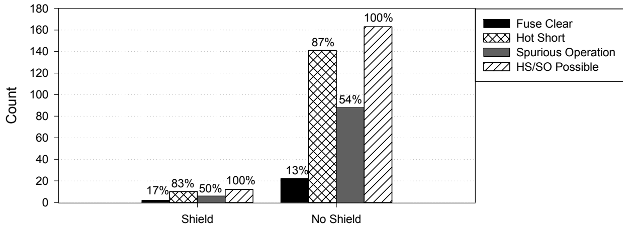
Figure 4-33. Cable shielding column plot, global approach, DC tests
