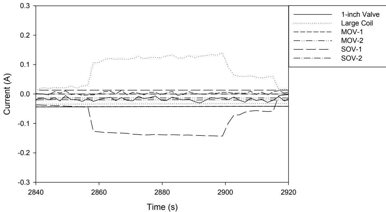
Figure 5-25. Intermediate-scale test 11 current summation
