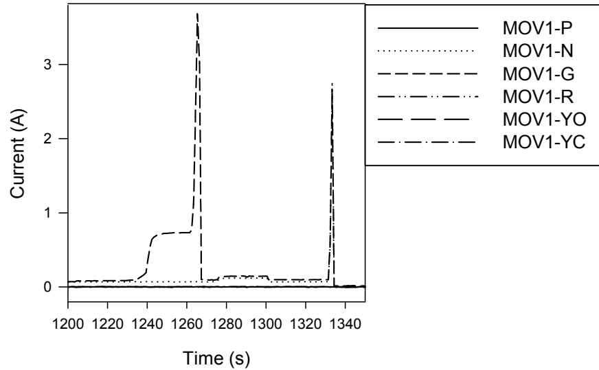
Figure A-23. Penlight MOV-1 Test #50 current plot
