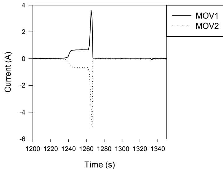
Figure A-22. Outstanding current shorting in Penlight MOV Test #50
