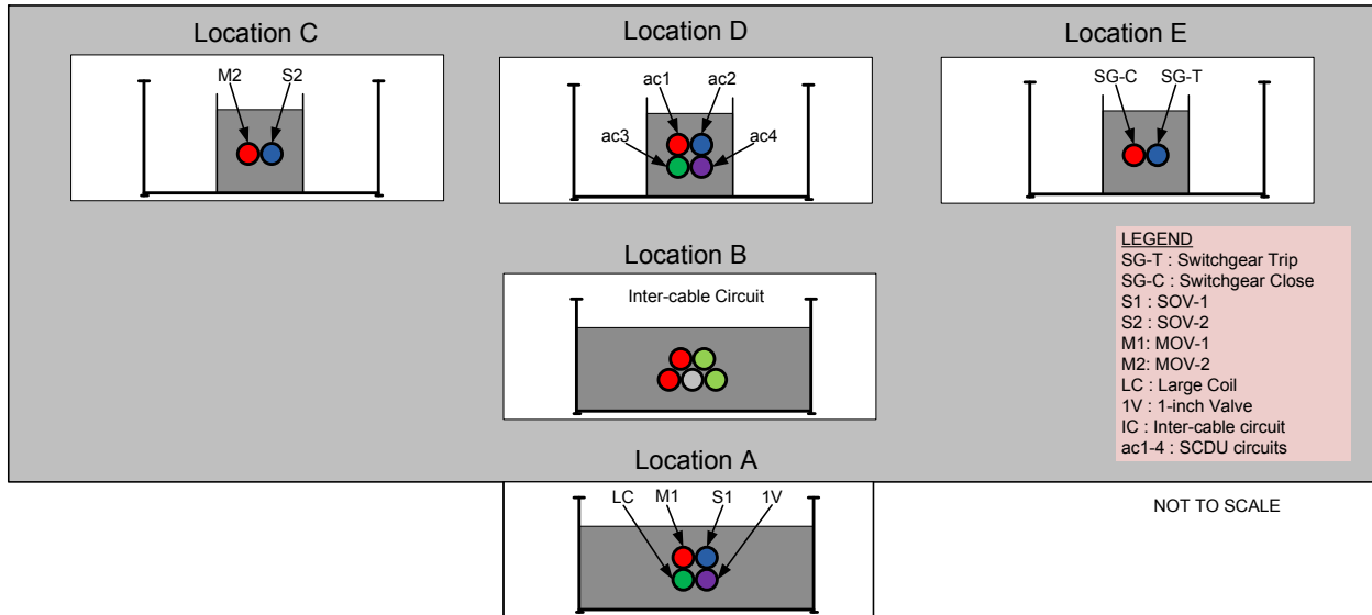
Figure 5-15. Intermediate-scale test 4 cable loading
