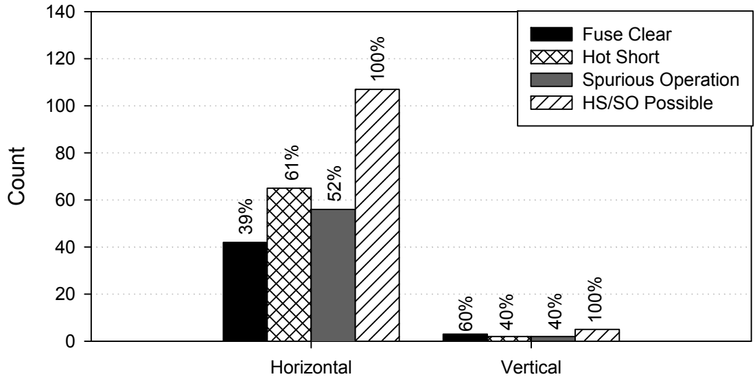
Figure 2-7. Cable orientation column plot, global approach, AC tests
