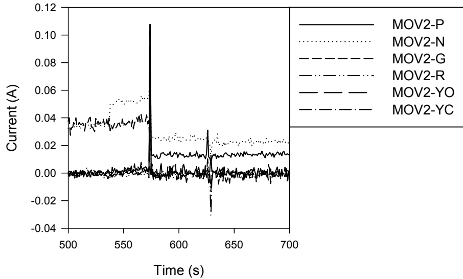
Figure A-12: Penlight MOV-2 test #33 current plot
