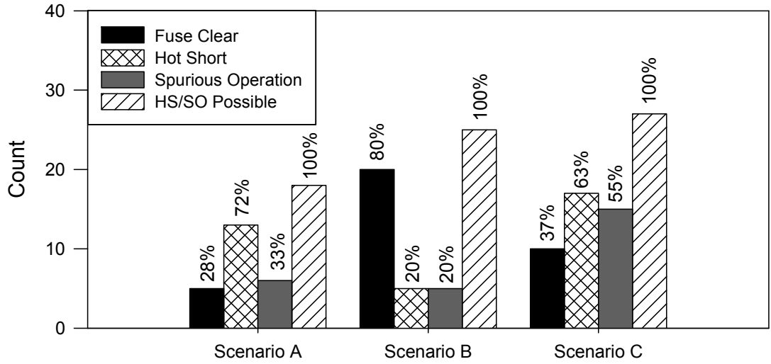
Figure 1-1. Examples global approach failure mode column plot
