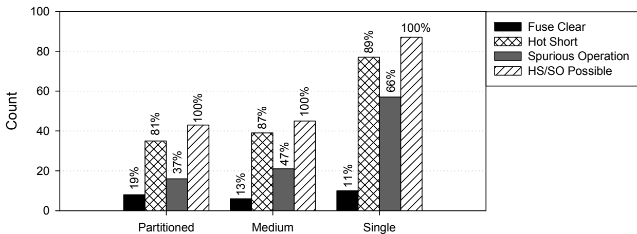
Figure 4-17. Raceway fill column plot, global approach, DC tests
