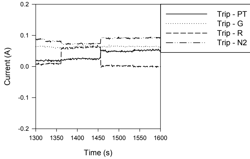
Figure A-48. Penlight SWGR Trip Test #JPN-2 current plot
