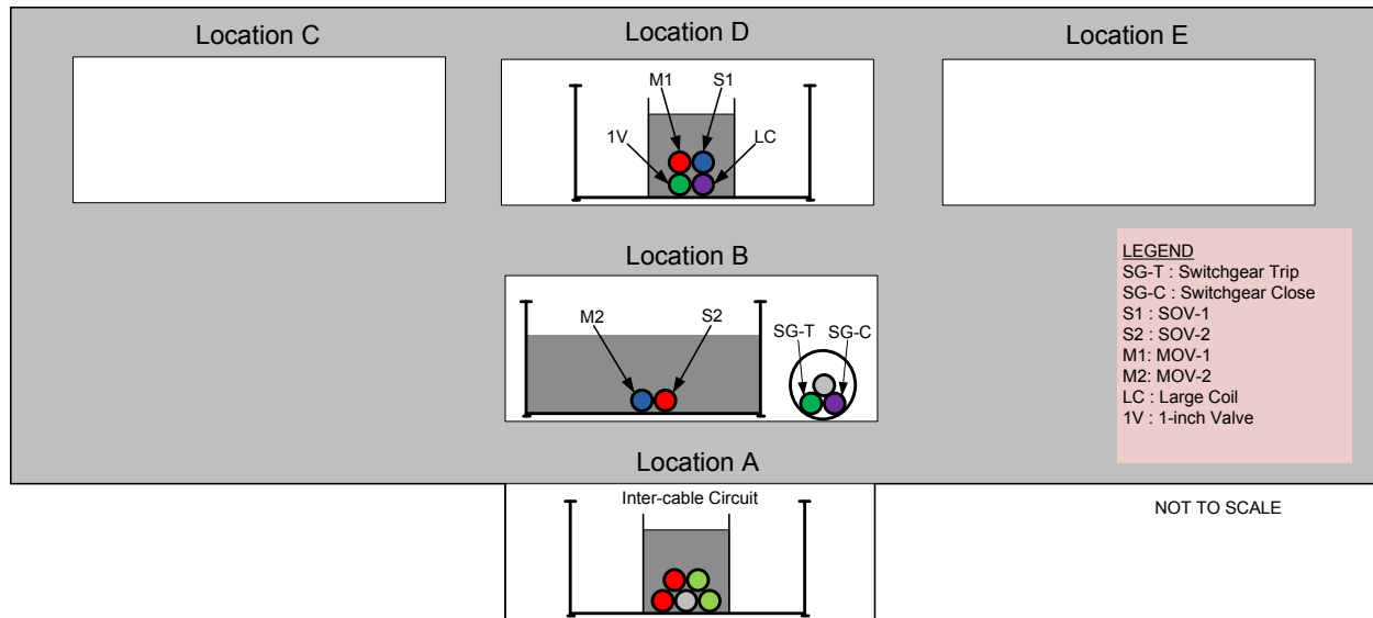
Figure 5-12. Intermediate-scale test 3 cable loading
