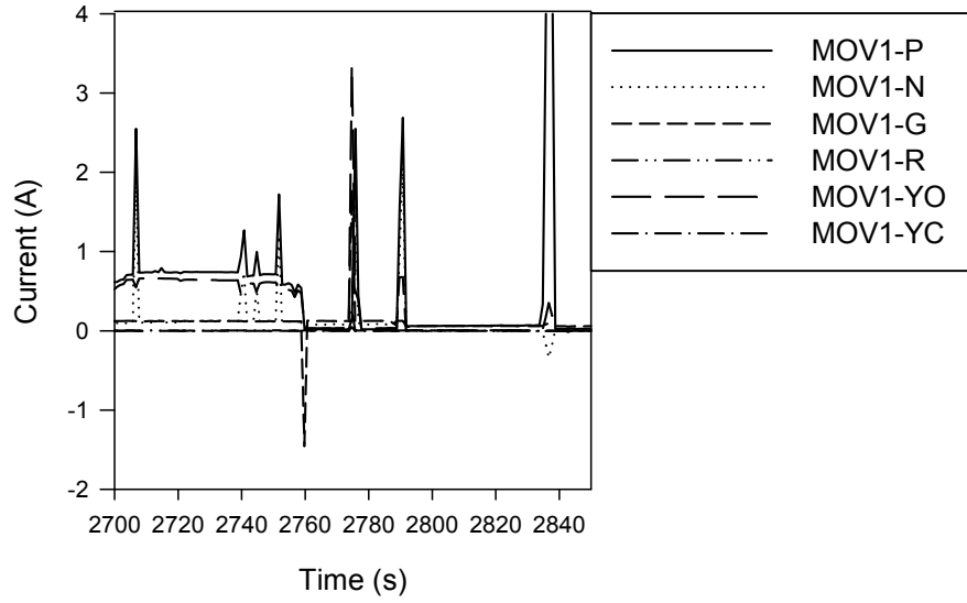
Figure A-17. Penlight MOV-1 Test #41 current plot
