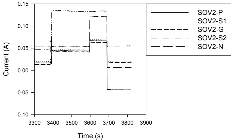
Figure A-33. Penlight SOV-2 Test #28 current plot
