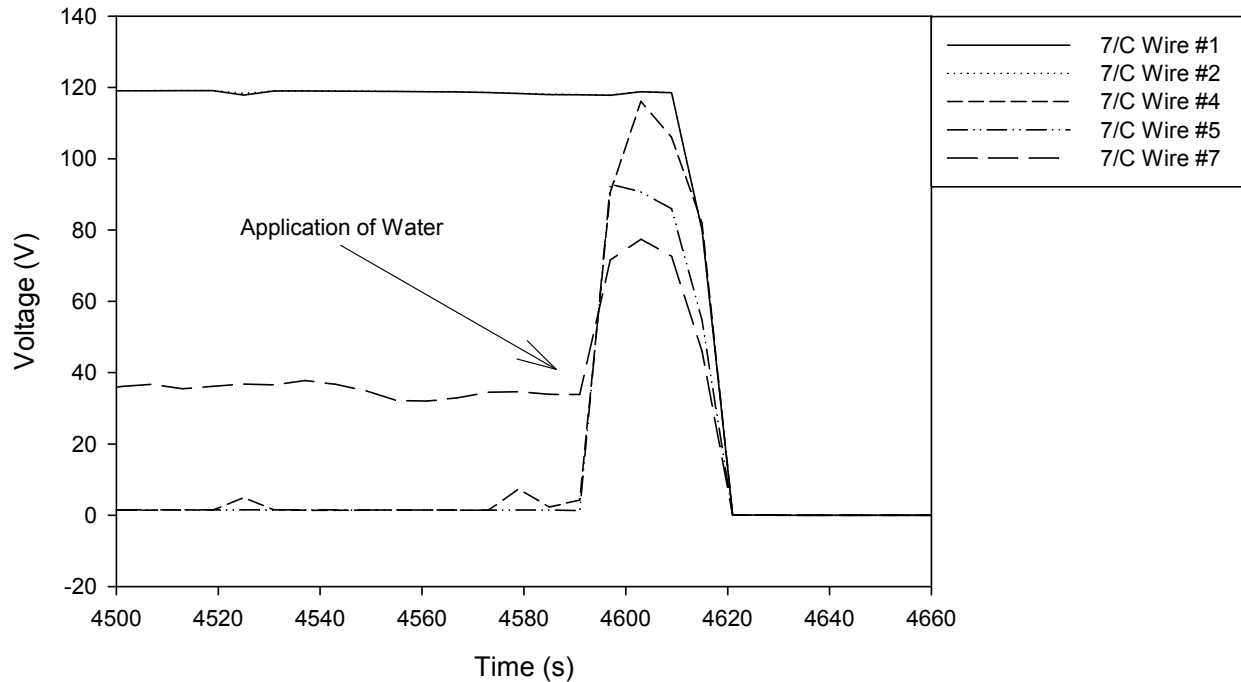
Figure 2-30. NEI/EPRI test 3 voltage plot - water spray
