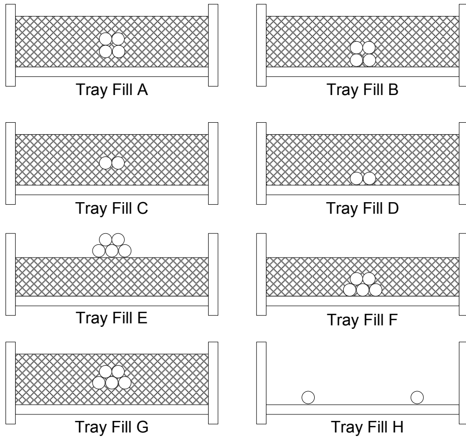
Figure 4-14. Circuit cable orientation for filled trays
