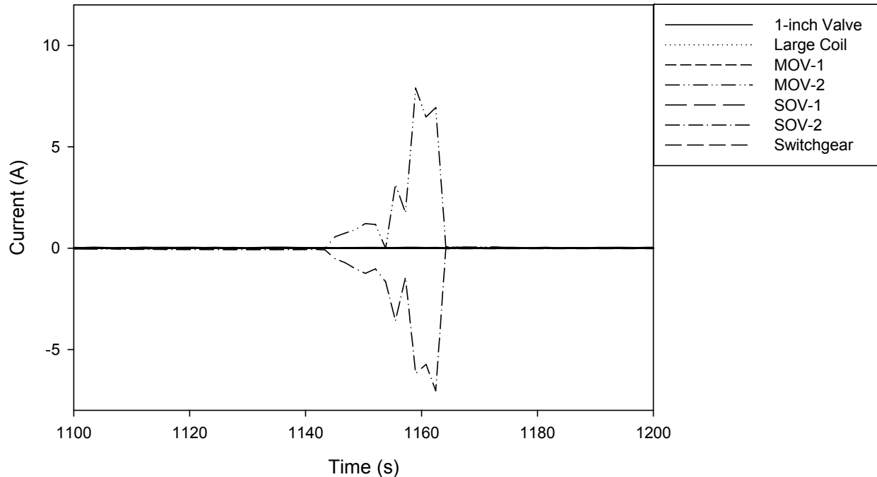
Figure 5-11. Outstanding current shorting in intermediate-scale test 2, between SOV-2 and MOV-2
