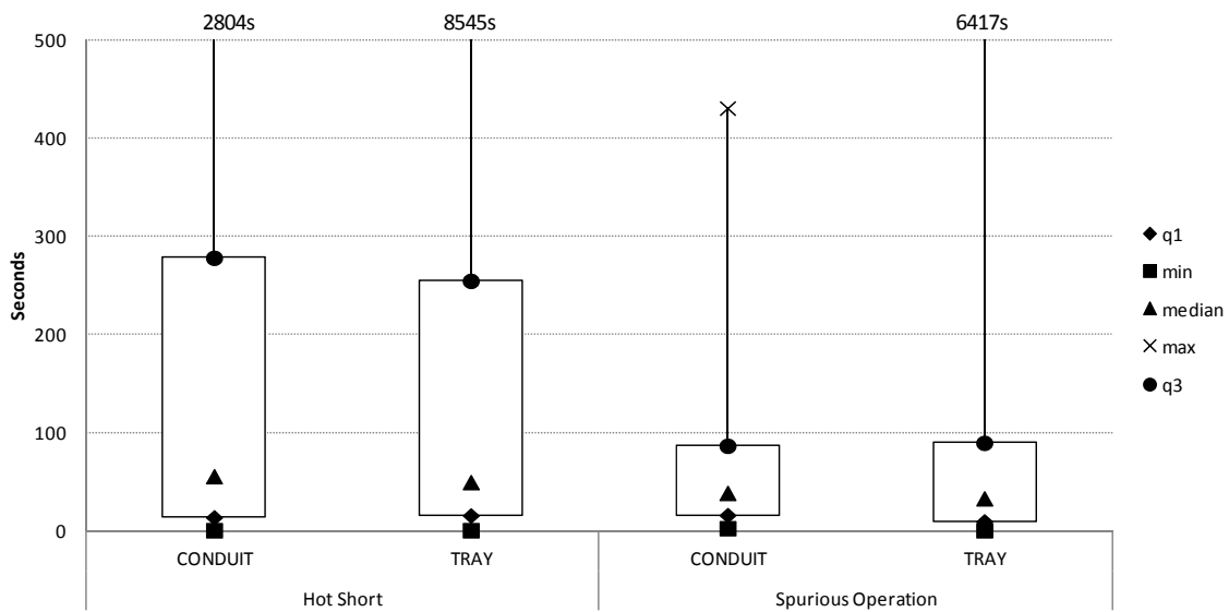
Figure 4-12. Raceway routing box plot, duration, DC tests
