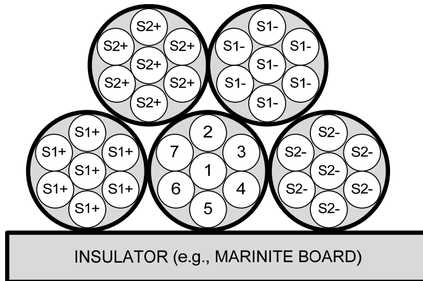
Figure 5-1. DESIREE-FIRE inter-cable configuration
