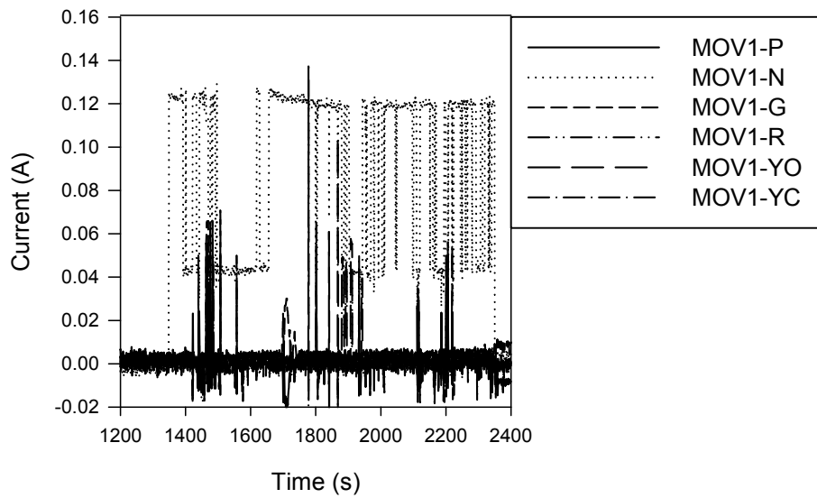
Figure A-5: Penlight MOV-1 test #12 current plot
