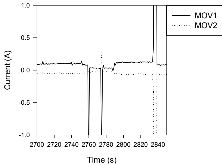
Figure A-16. Outstanding current shorting in Penlight MOV Test #41
