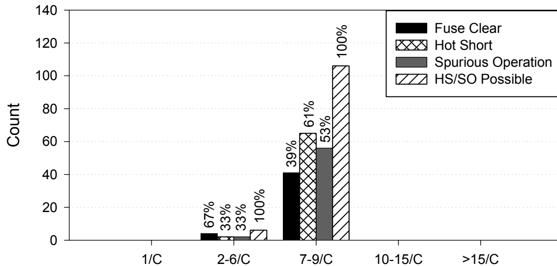
Figure 2-2. Conductor count column plot, global approach, AC tests
