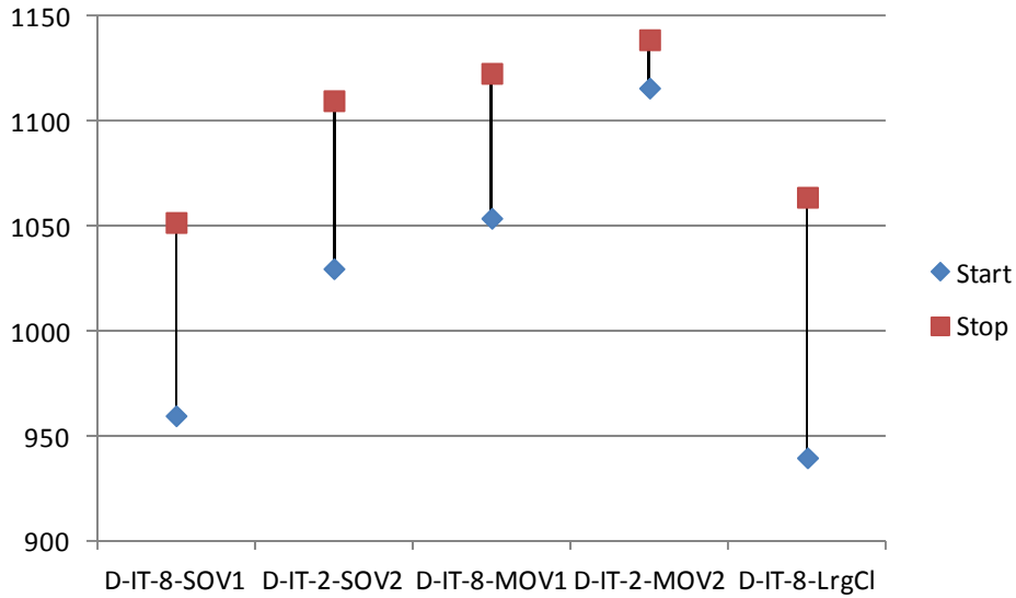
Figure 4-41. Time plot of concurrent spurious operations for DESIREE-FIRE among all test circuits in Location A
