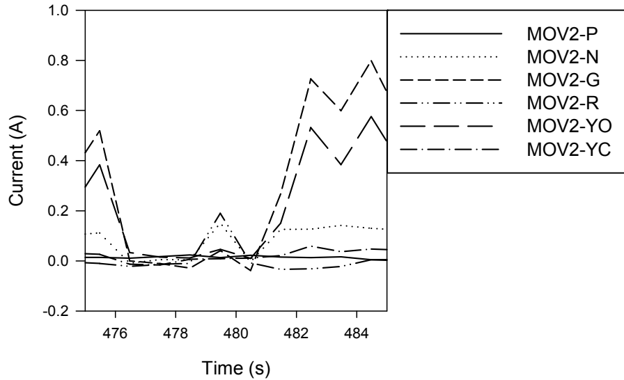
Figure A-3: Penlight MOV-2 test #8 current plot
