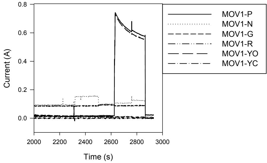
Figure A-26. Penlight MOV-1 Test # JPN-3 current plot
