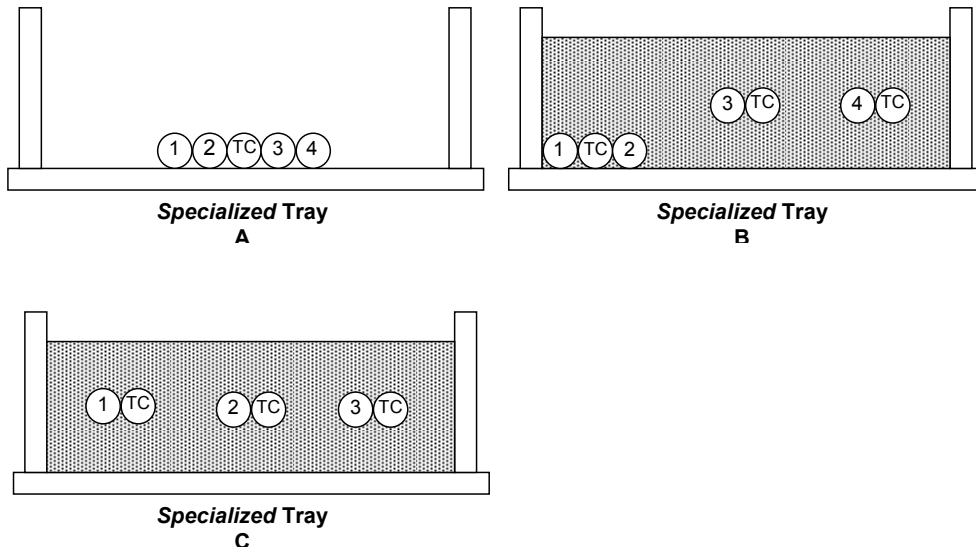
Figure 4-16. Circuit cable orientation for specialized trays
