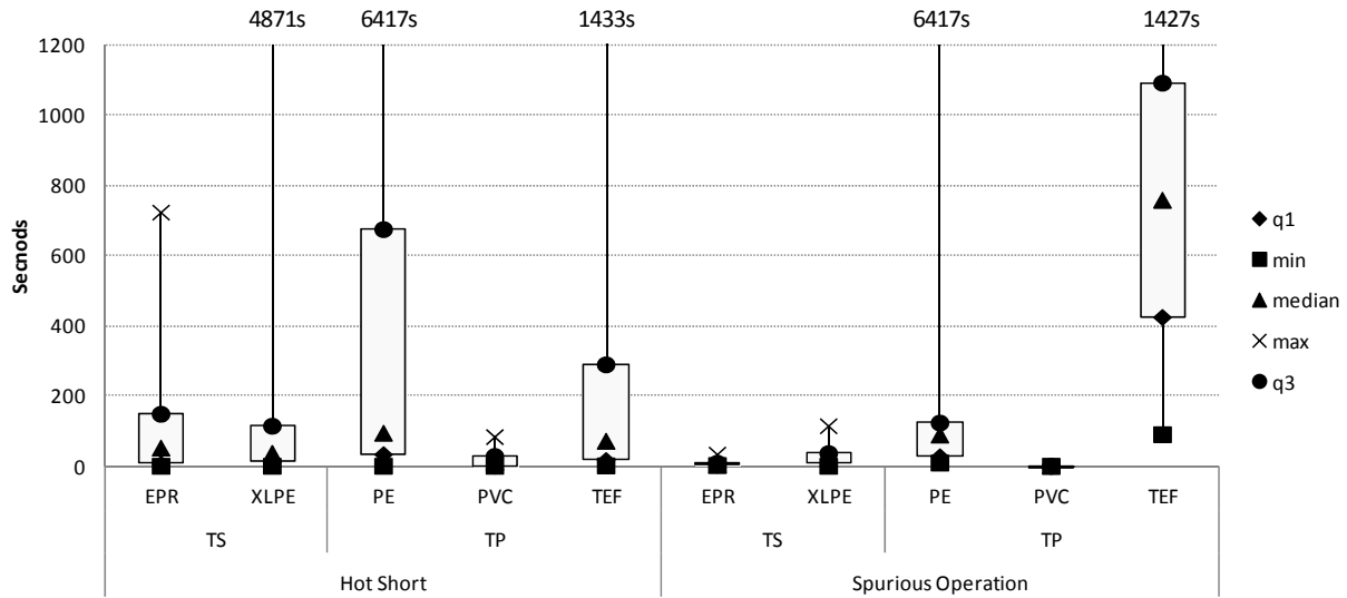
Figure 4-22. Insulation material box plot, duration, DC tests
