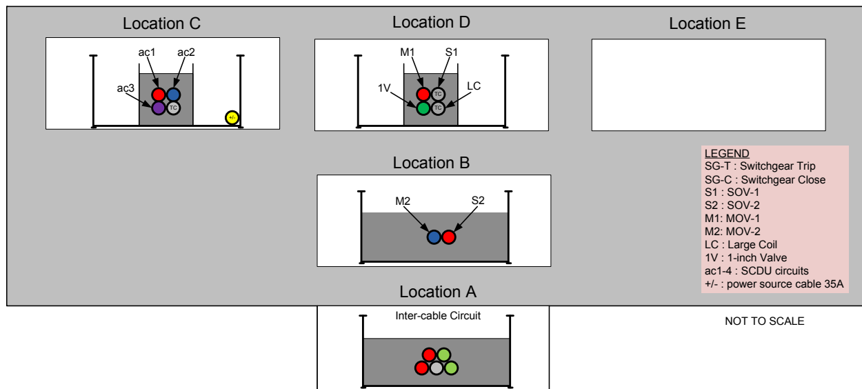
Figure 5-26. Intermediate-scale test 12 cable loading
