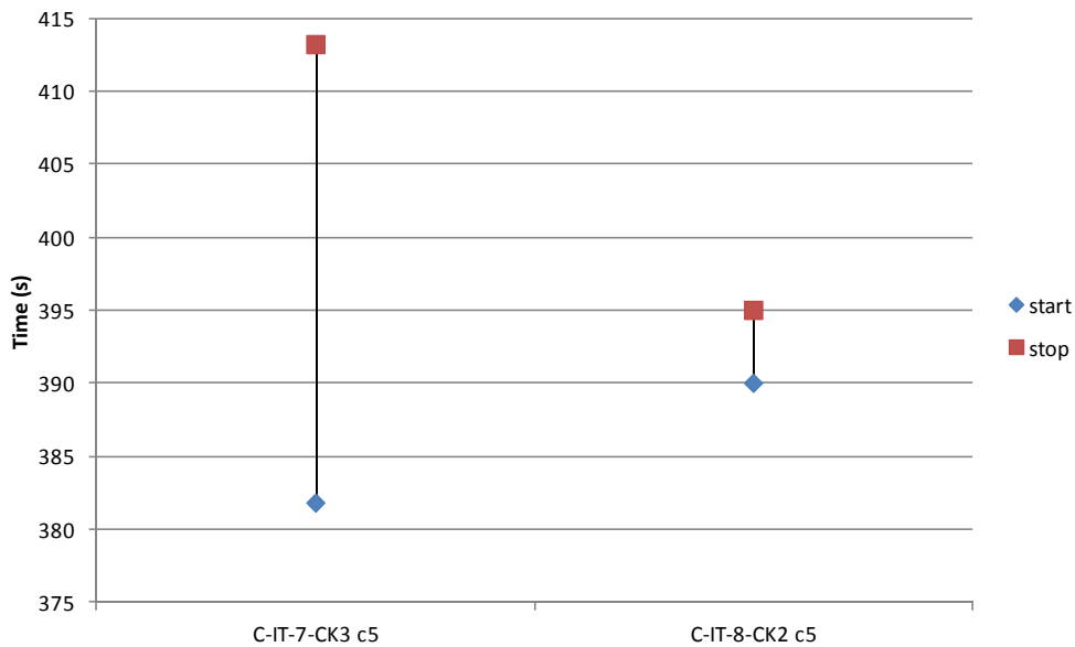
Figure 2-34. Concurrent hot shorts - Location A - 2 cables
