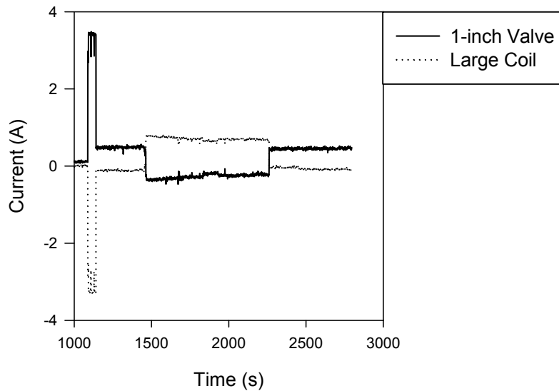
Figure A-37. Outstanding current shorting in Penlight 1-inch valve and large coil Test #11
