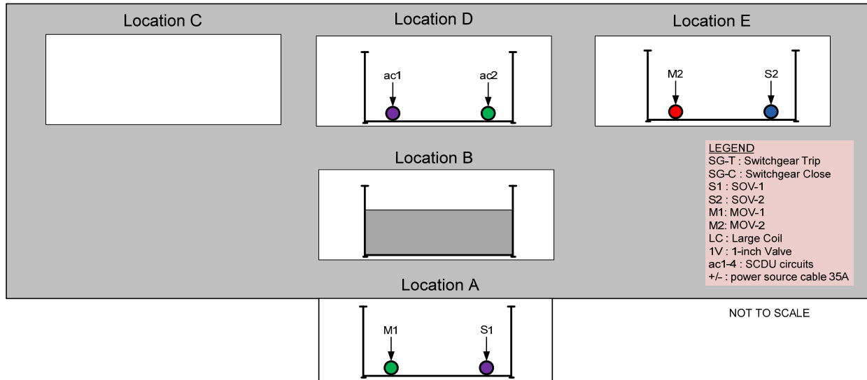
Figure 5-6. Intermediate-scale test preliminary 2 cable loading configuration
