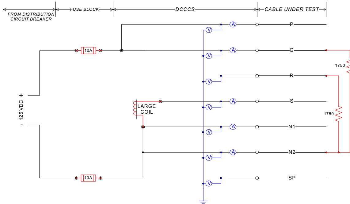
Figure 4-2. Line drawing for the DC large coil circuit
