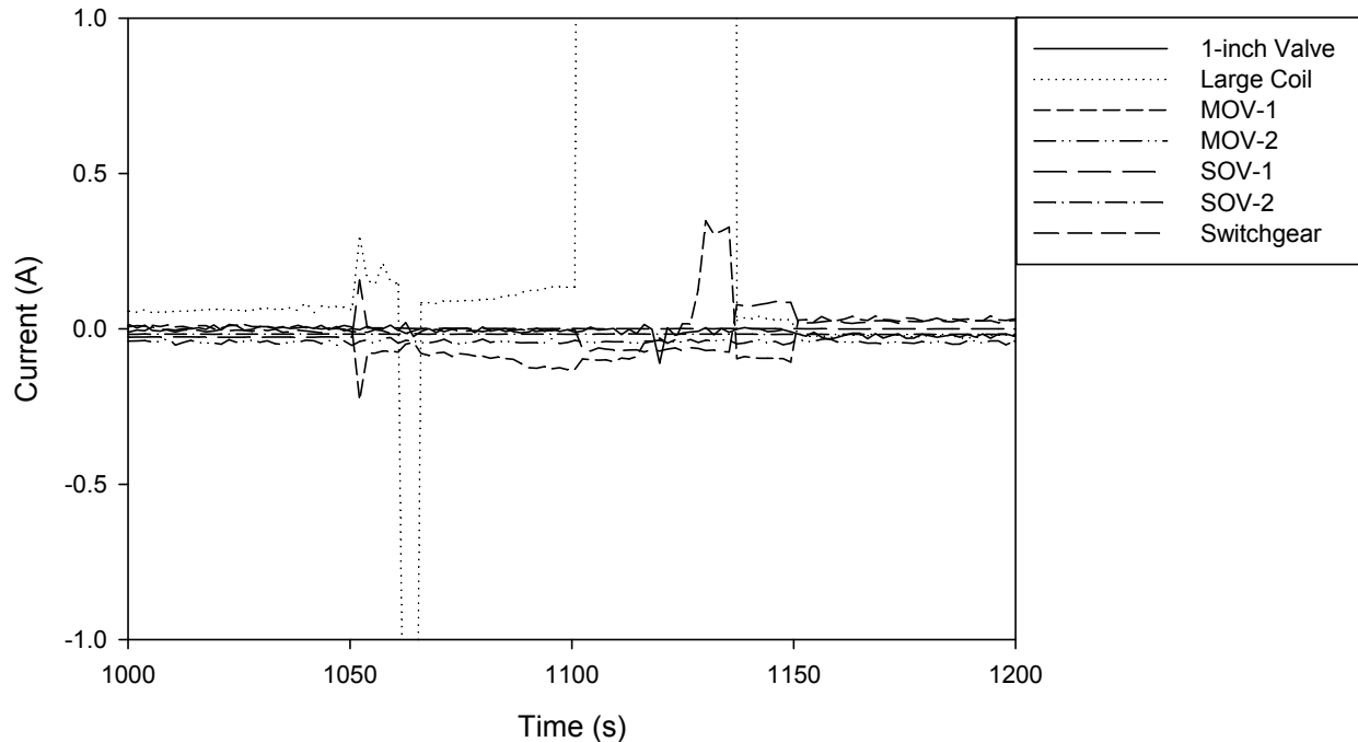
Figure 5-21. Outstanding current shorting in intermediate-scale test 8, between MOV-1 and Lg Coil
