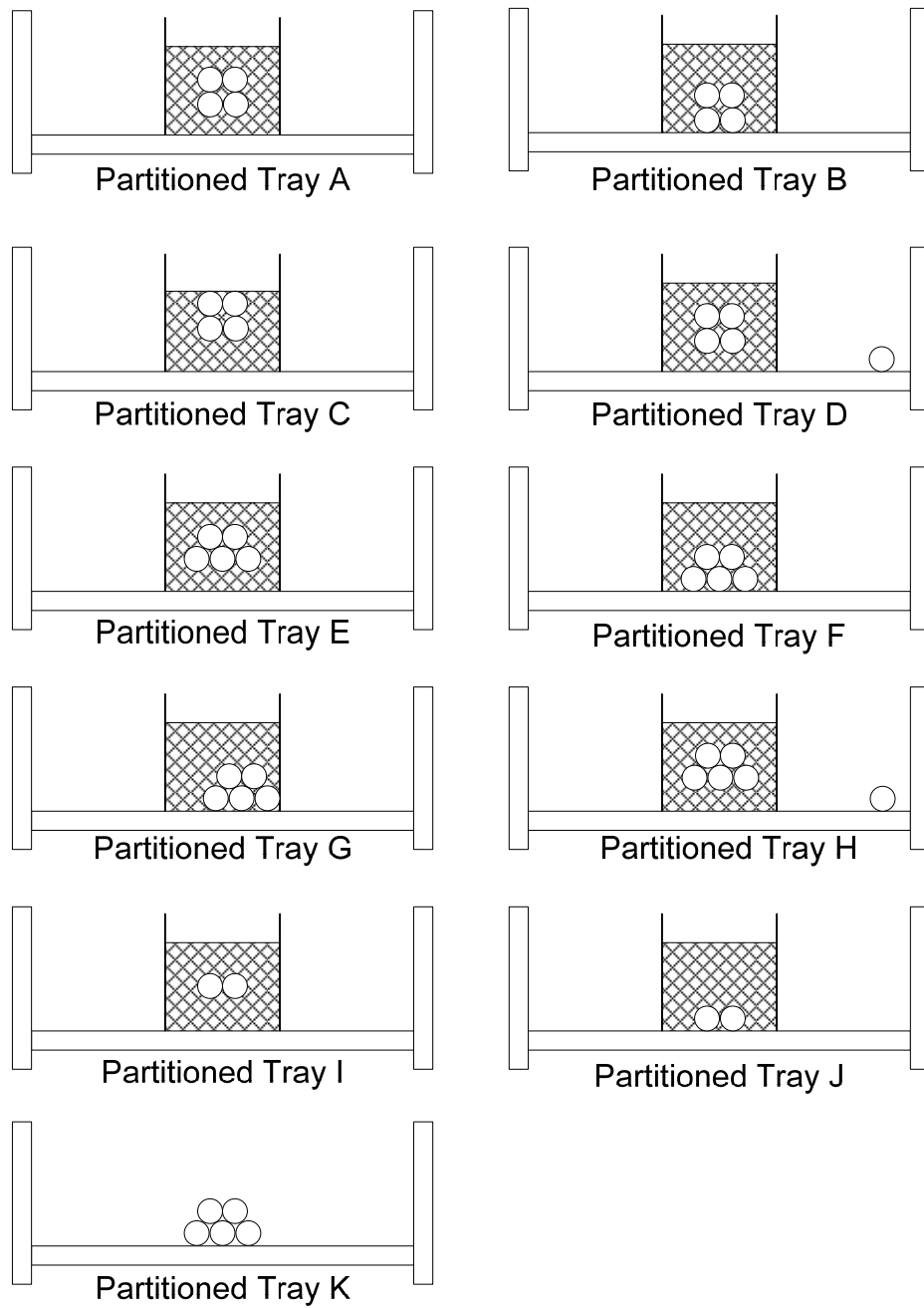
Figure 4-15. Circuit cable orientation for partitioned trays
