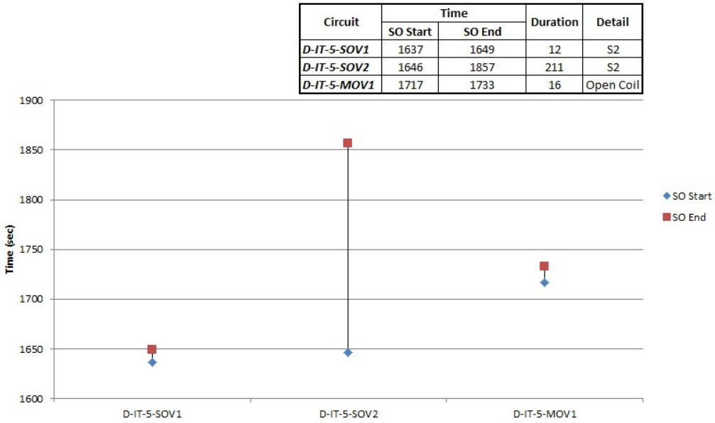
Figure 4-35. Time plot of concurrent hot shorts for DESIREE-FIRE intermediate-scale test 5
