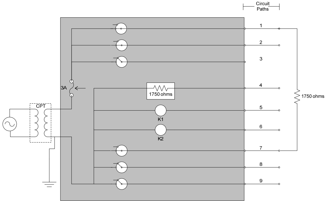
Figure 2-1. CAROLFIRE AC MOV circuit
