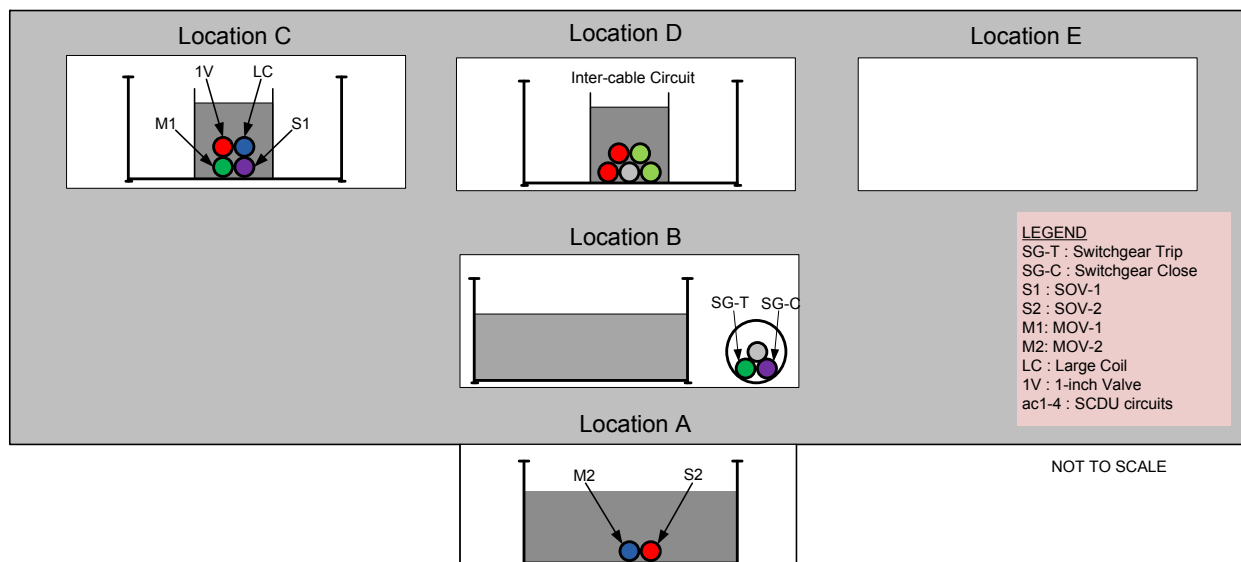
Figure 5-18. Intermediate-scale test 6 cable loading
