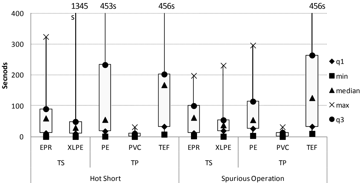
Figure 2-19. Insulation material box plot, duration, AC tests
