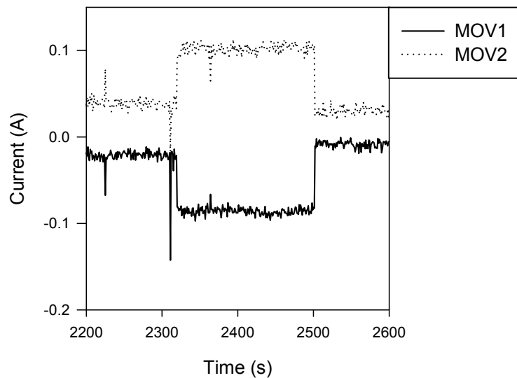
Figure A-25. Outstanding current shorting in Penlight MOV Test #JPN-3
