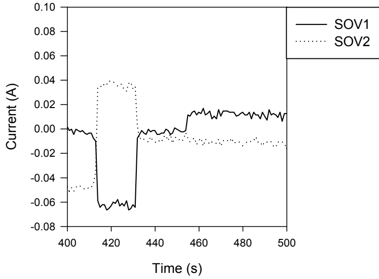
Figure A-34. Outstanding current shorting in Penlight SOV Test #31
