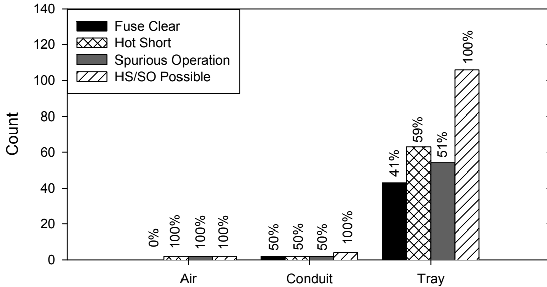
Figure 2-9. Raceway routing column plot, global approach, AC tests
