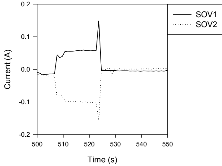
Figure A-28. Outstanding current shorting in Penlight SOV Test #20
