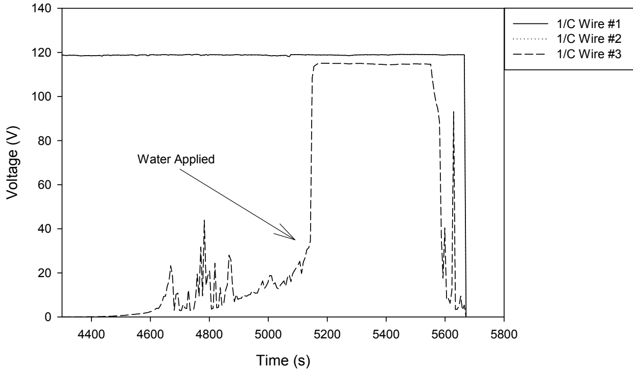
Figure 2-31. NEI/EPRI test 10 voltage response following water spray
