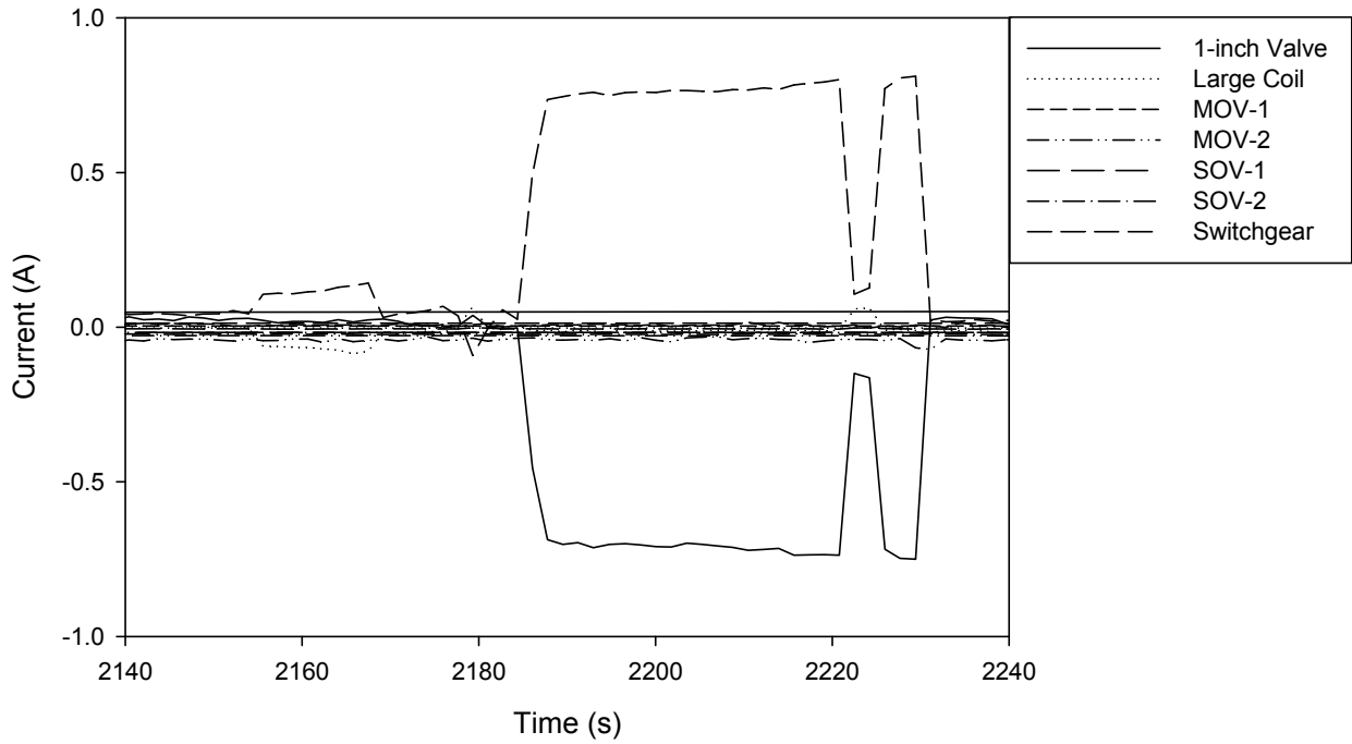
Figure 5-14. Outstanding current shorting in intermediate-scale test 3, between 1 inch valve and SWGR-T
