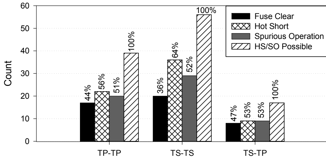
Figure 2-20. Insulation-jacket type column plot, global approach, AC tests
