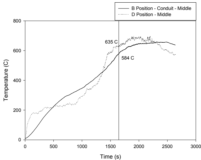
Figure 4-36. Plot of intermediate-scale test 5 for MOV and SOV cable locations
