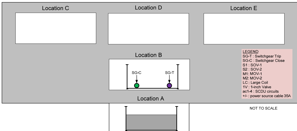
Figure 5-29. Intermediate-scale test contingency A cable loading configuration
