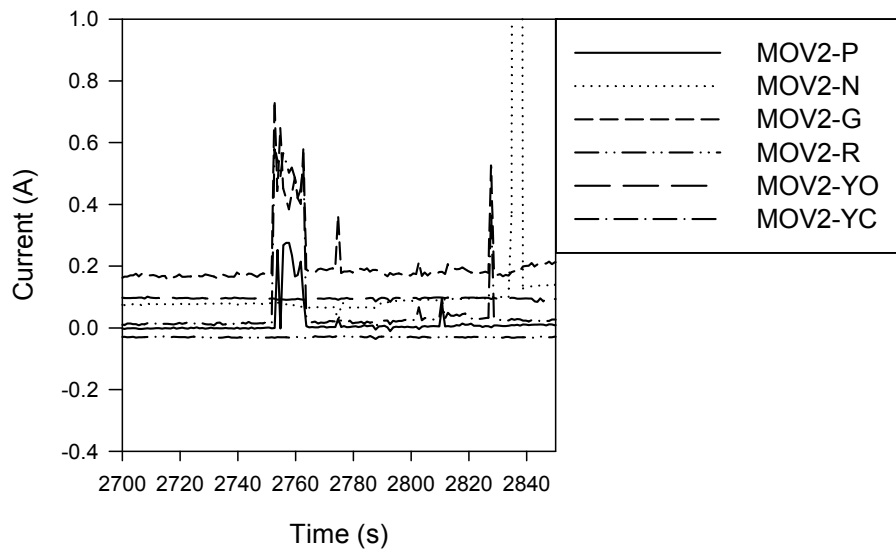
Figure A-18. Penlight MOV-2 Test #41 current plot
