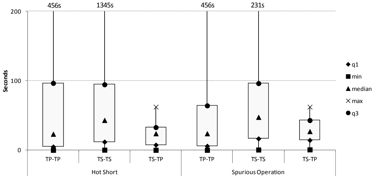
Figure 2-21. Insulation-jacket type box plot, duration, AC tests
