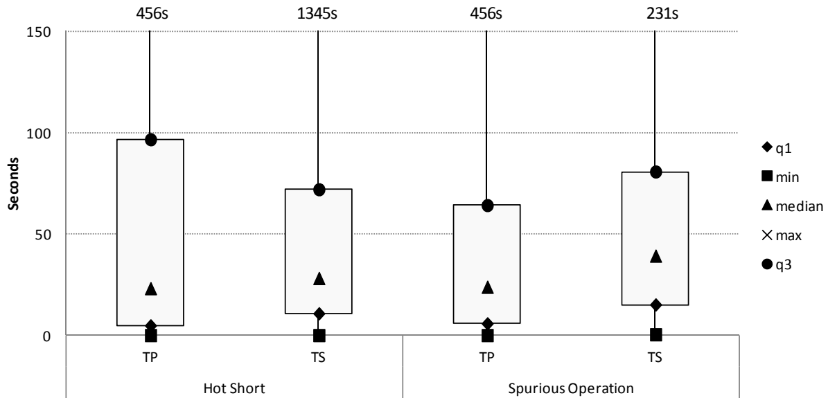
Figure 2-17. Insulation type box plot, duration, AC tests
