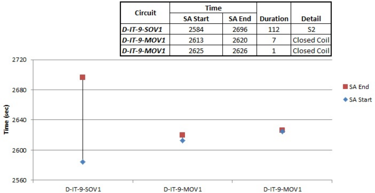
Figure 4-40. Concurrent hot shorts - test 9
