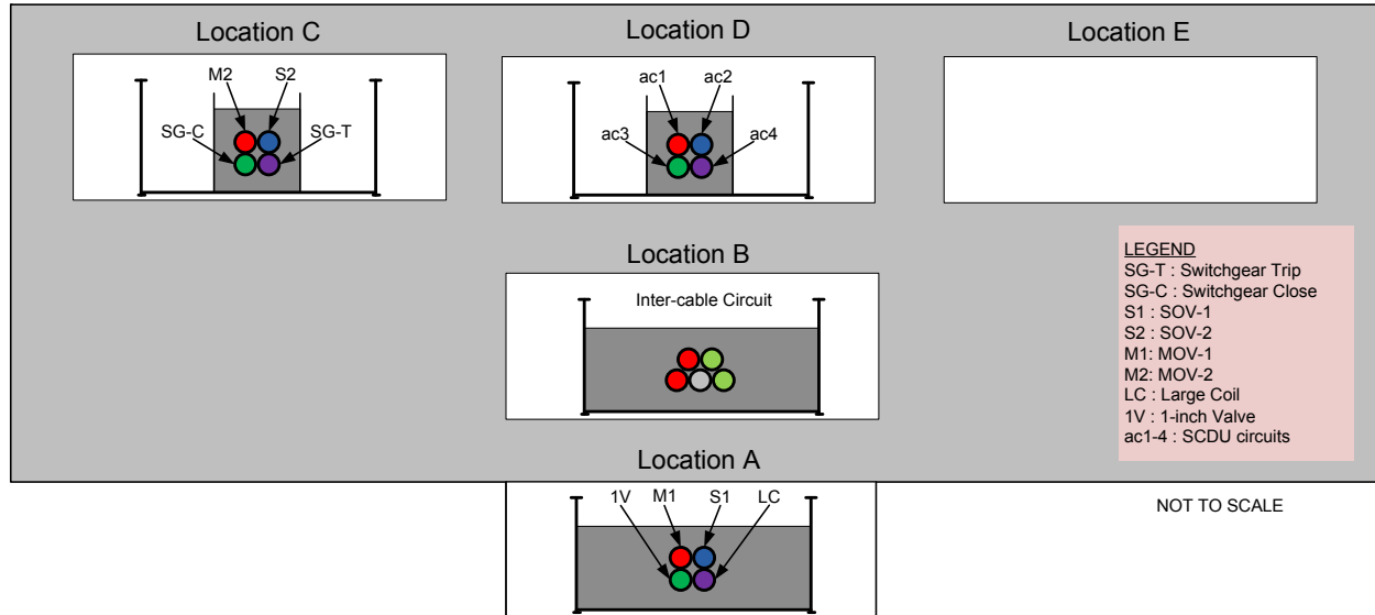
Figure 5-20. Intermediate-scale test 8 cable loading
