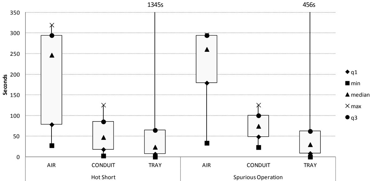
Figure 2-10. Raceway routing box plot, duration, AC tests
