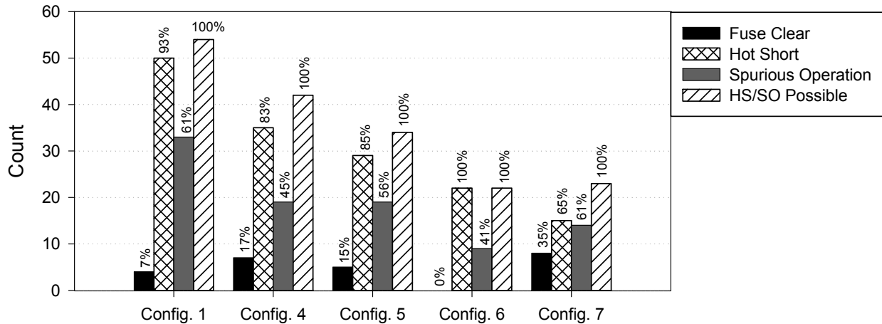
Figure 4-25. Wiring configuration column plot, global approach, DC tests
