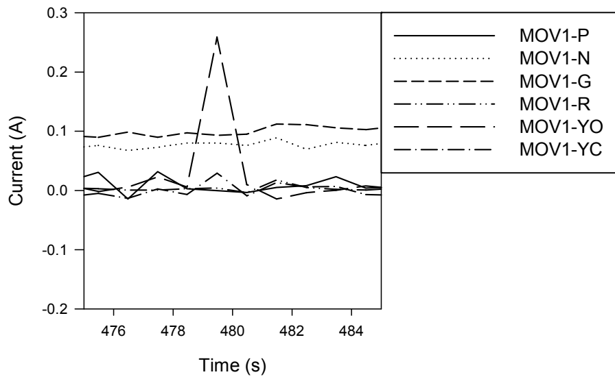
Figure A-2: Penlight MOV-1 test #8 current plot
