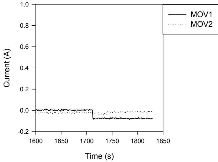
Figure A-13. Outstanding current shorting in Penlight MOV Test #37
