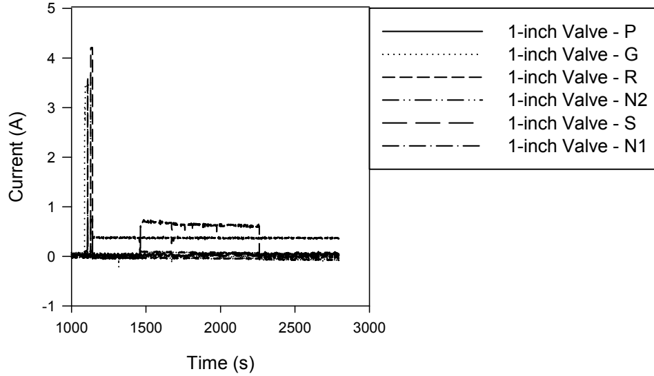
Figure A-38. Penlight 1-inch valve Test #11 current plot
