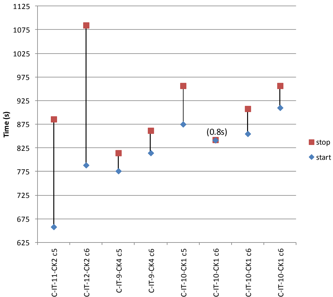
Figure 2-35. Concurrent hot shorts - upper hot gas layer - 4 cables
