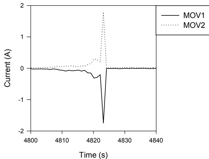
Figure A-19. Outstanding current shorting in Penlight MOV Test #49
