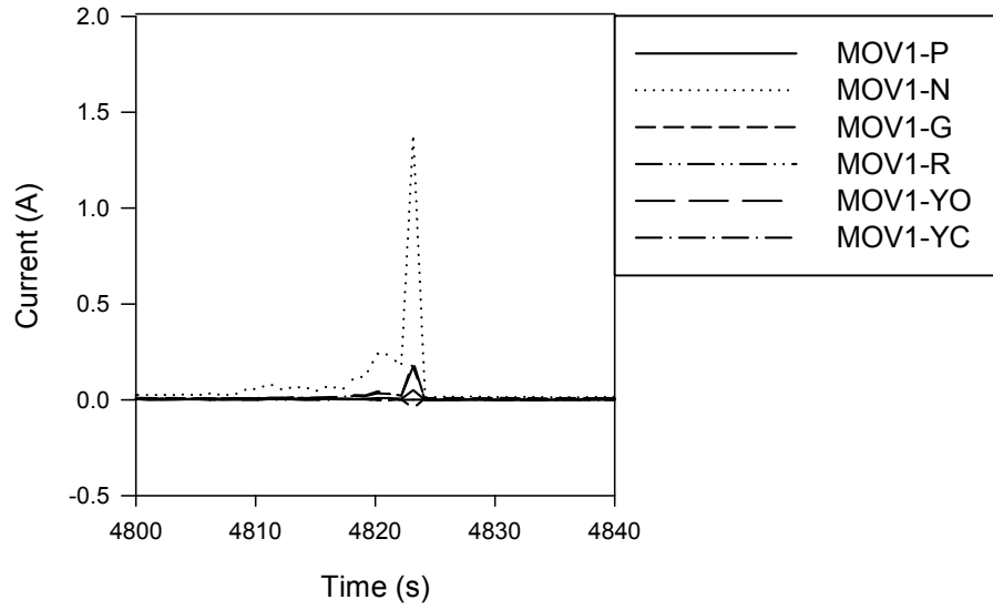
Figure A-20. Penlight MOV-1 Test #49 current plot
