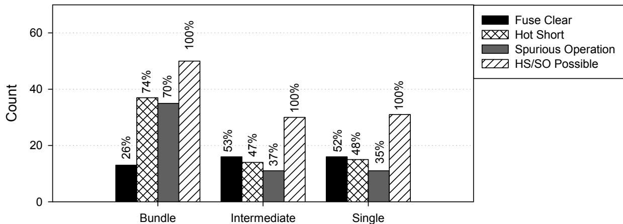
Figure 2-14. Raceway fill column plot, global approach, AC tests
