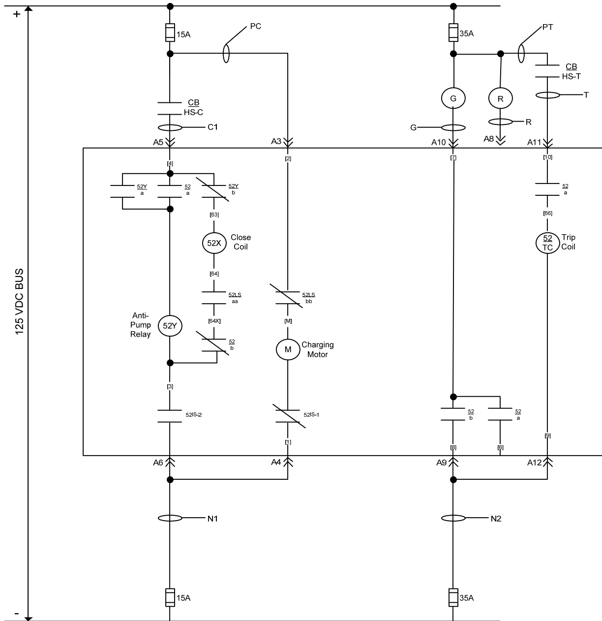
Figure 4-5. Line drawing for DC SWGR 1 circuit
