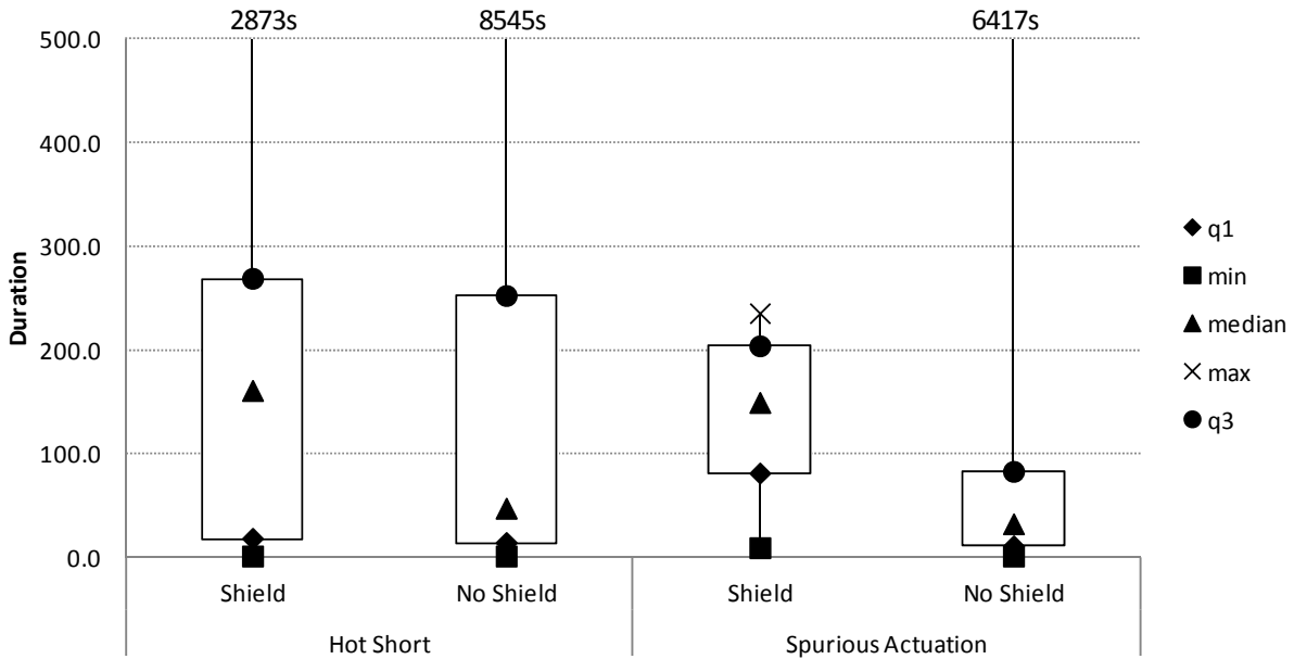
Figure 4-34. Cable Shielding box plot, duration, DC tests
