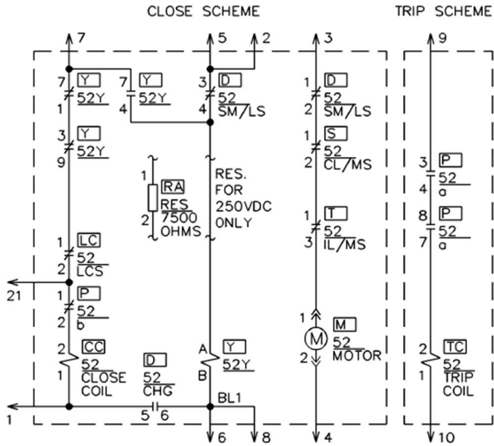
Figure 4-6. Line drawing for DC SWGR 2 circuit
