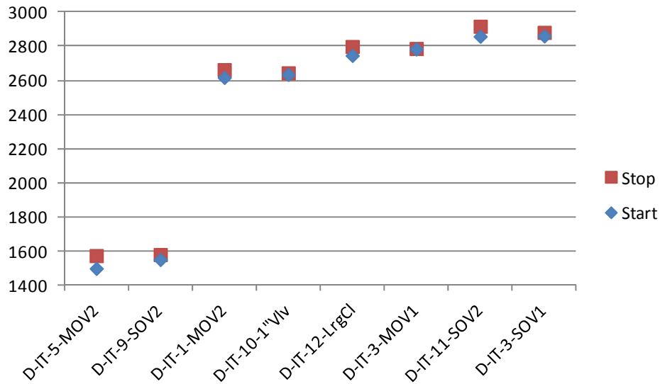
Figure 4-42. Time plot of concurrent spurious operations for DESIREE-FIRE among all test circuits in Location D
