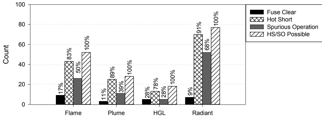
Figure 4-9. Thermal exposure conditions column plot, global approach, DC tests
