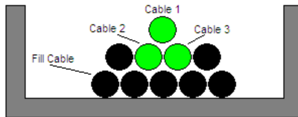
Figure 3-1. NEI/EPRI inter-cable test tray fill
