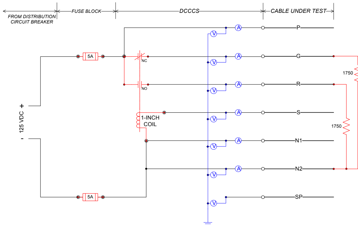
Figure 4-1. Line drawing of the DC-SIM panel layout for a 1-inch coil circuit
