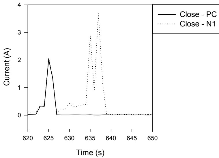
Figure A-44 Penlight SWGR Close Test #4 current plot
