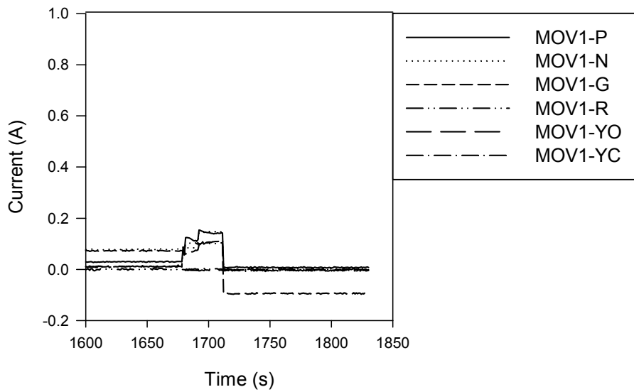
Figure A-14. Penlight MOV-1 Test #37 current plot
