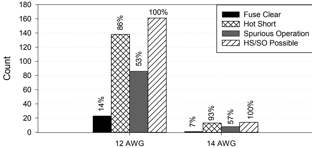
Figure 4-27. Conductor size column plot, global approach, DC tests
