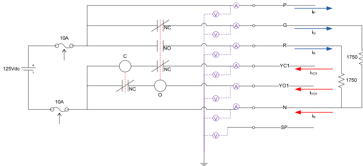
Figure 5-3. DC MOV schematic showing current summation used in identifying inter-cable shorting behavior
