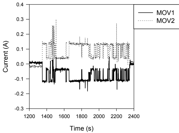
Figure A-4: Outstanding current shorting in Penlight MOV test #12
