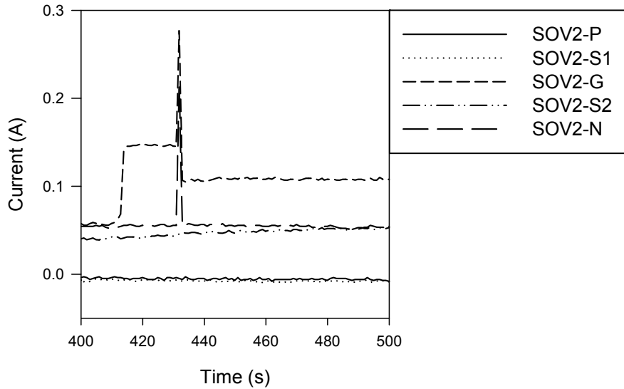
Figure A-36 Penlight SOV-2 Test #31 current plot
