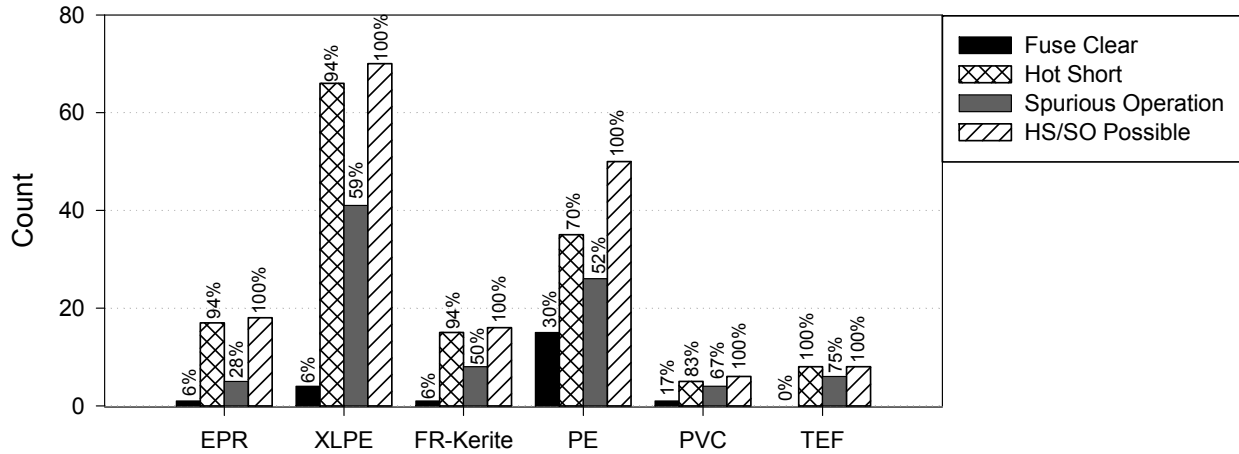
Figure 4-21. Insulation material column plot, global approach, DC tests
