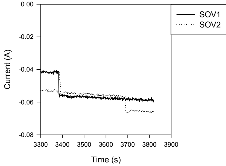
Figure A-31. Outstanding current shorting in Penlight SOV Test #28
