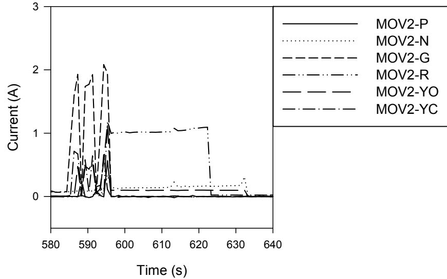
Figure A-9: Penlight MOV-2 Test #22 current plot
