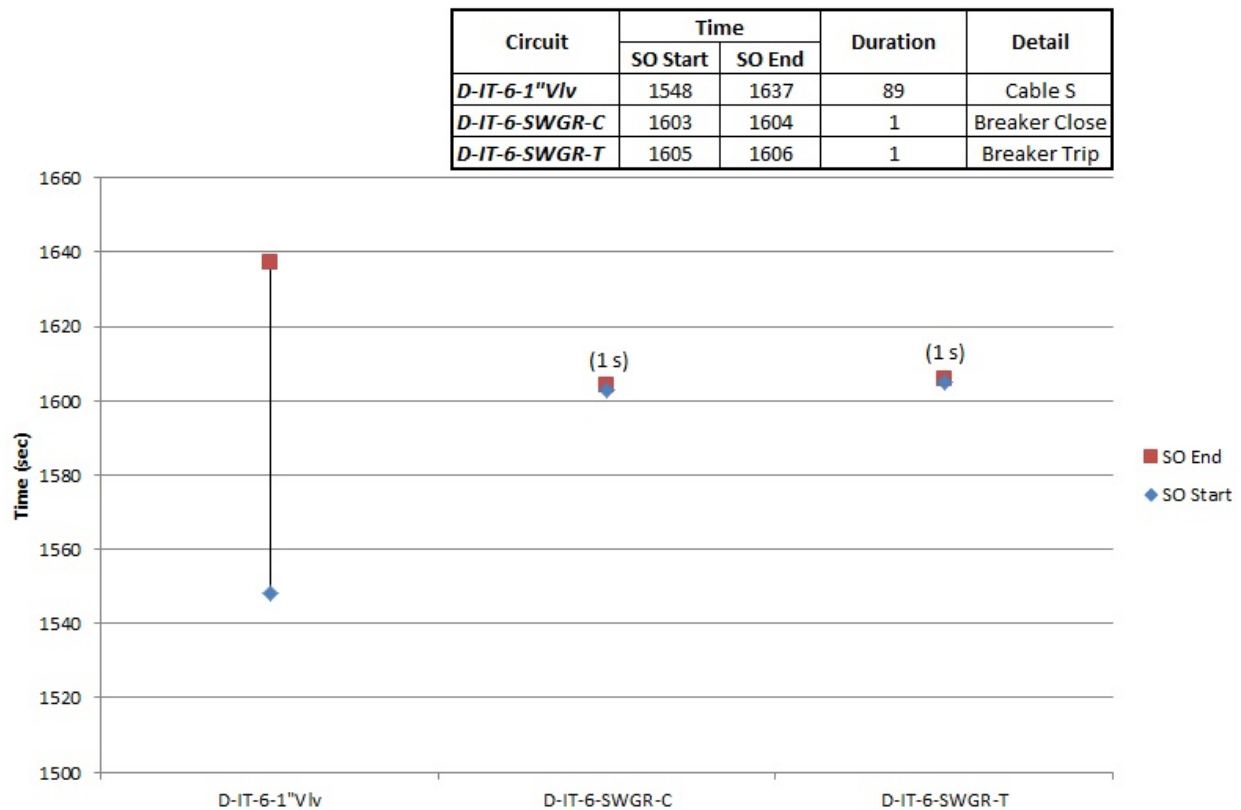
Figure 4-37. Concurrent hot shorts - test 6
