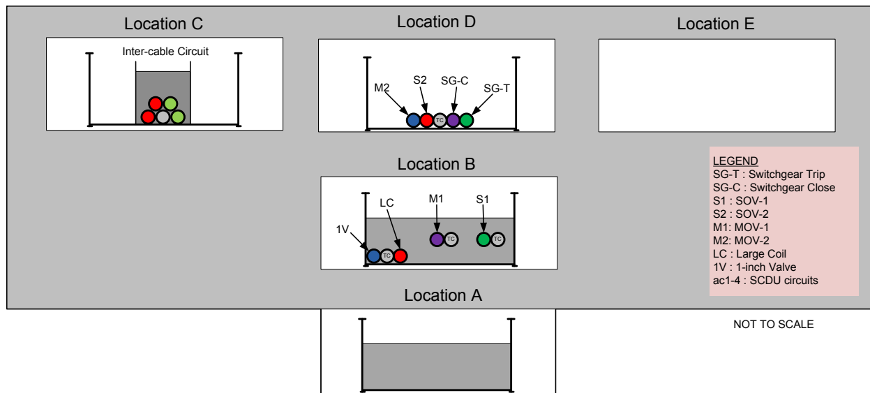
Figure 5-22. Intermediate-scale test 9 cable loading
