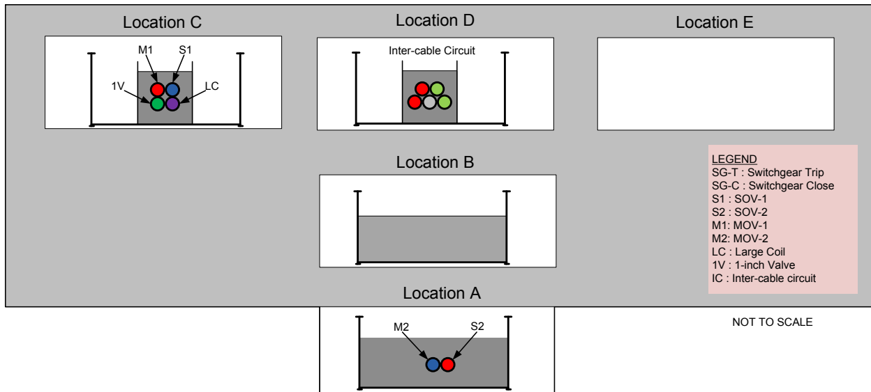
Figure 5-10. Intermediate-scale test 2 cable loading
