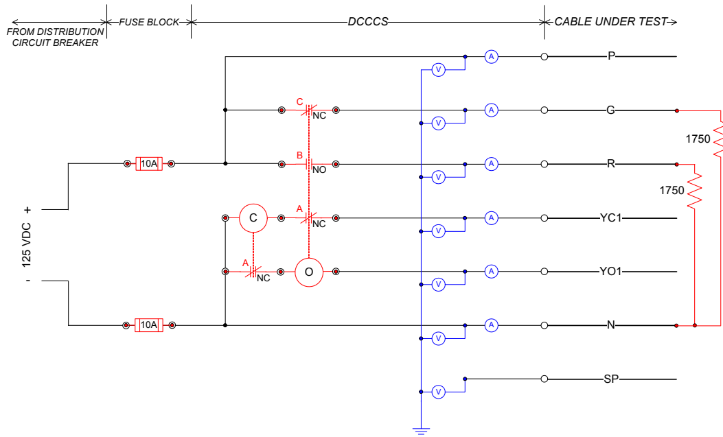
Figure 4-3. Line drawing for DC MOV circuit
