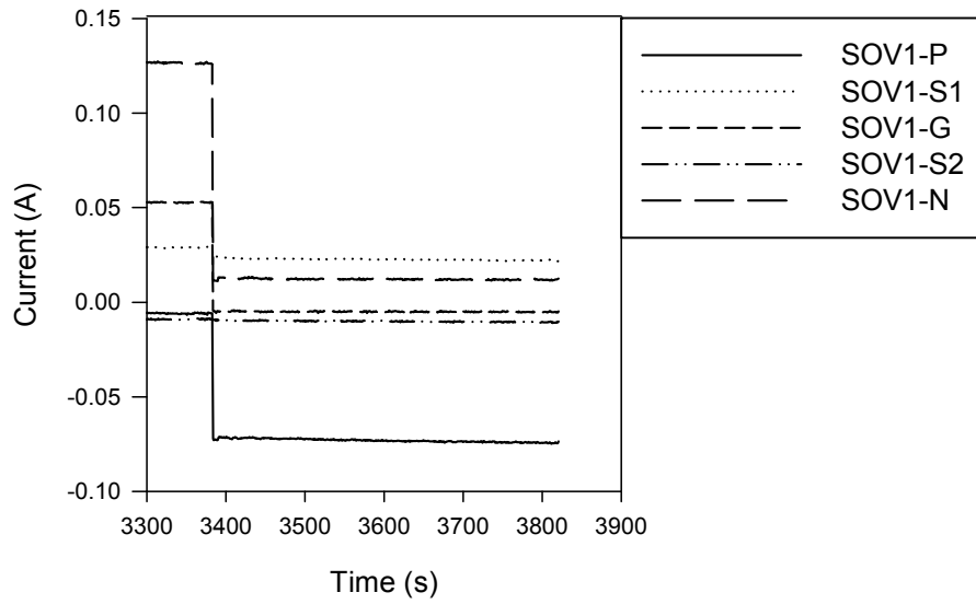
Figure A-32. Penlight SOV-1 Test #28 current plot
