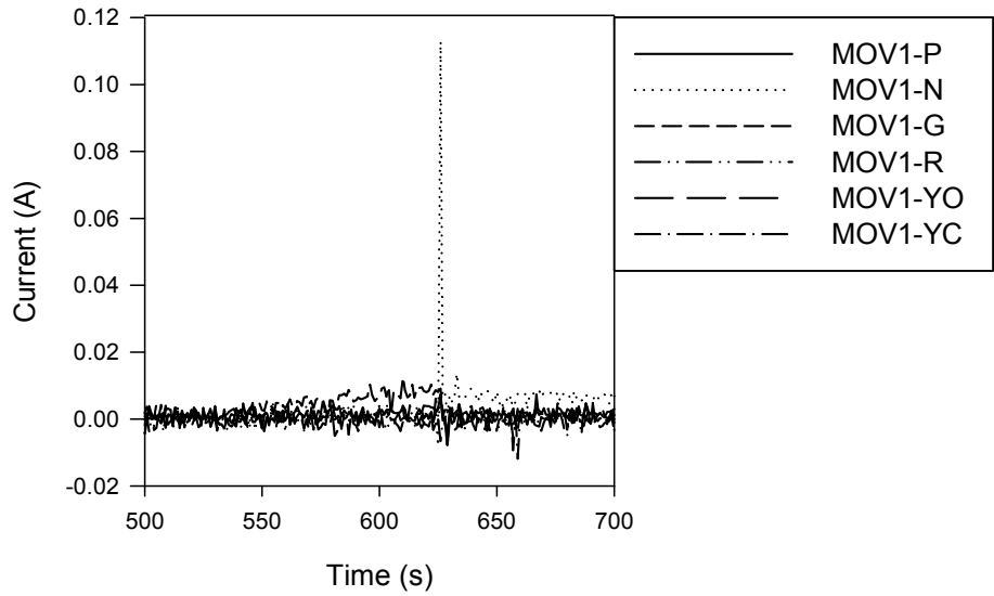
Figure A-11: Penlight MOV-1 test #33 current plot
