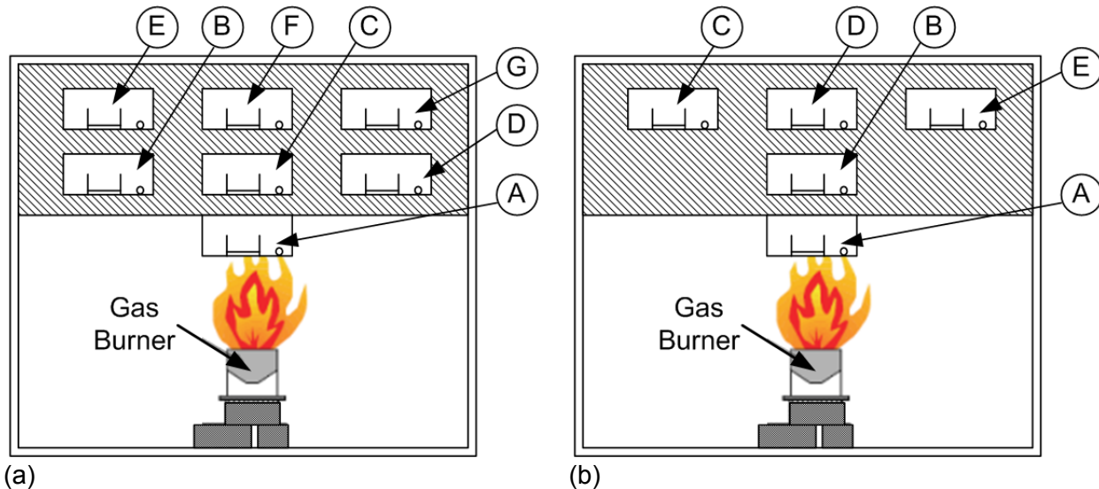
Figure 2-32. (a) CAROLFIRE and (b) DESIREE-FIRE intermediate-scale exposure location designation
