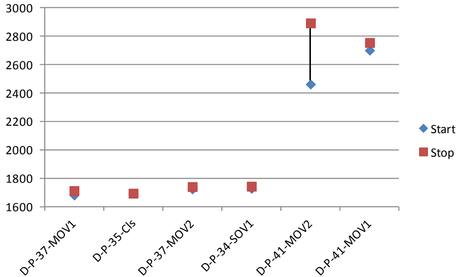
Figure 4-45. Time plot of concurrent spurious operations for DESIREE-FIRE among all Penlight test with exposure temperatures in the range of 500-525°C
