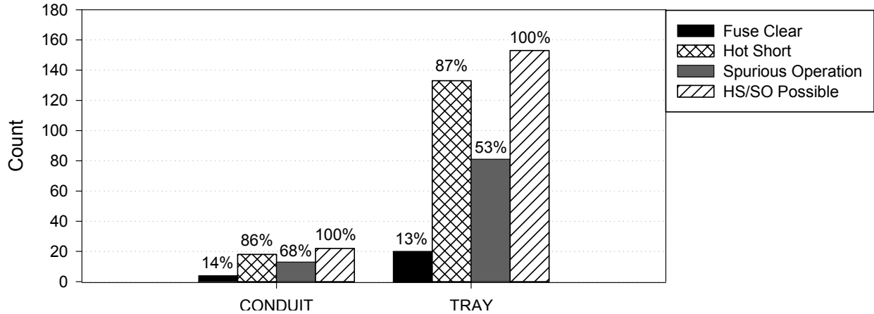
Figure 4-11. Raceway routing column plot, global approach, DC tests
