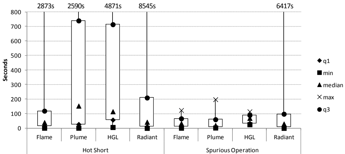
Figure 4-10. Thermal exposure conditions box plot, duration, DC tests
