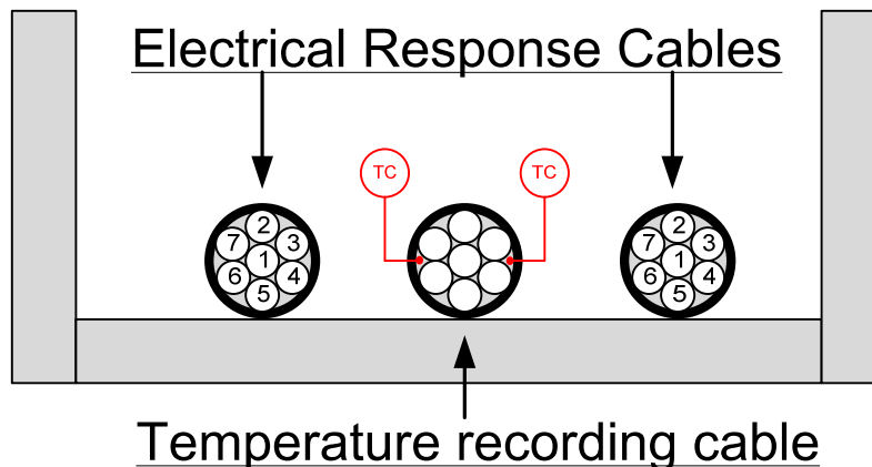
Figure 5-4. Penlight cable tray typical loading, showing two electrically instrumented cables and a thermal response (temperature recording) cable located in the center.
