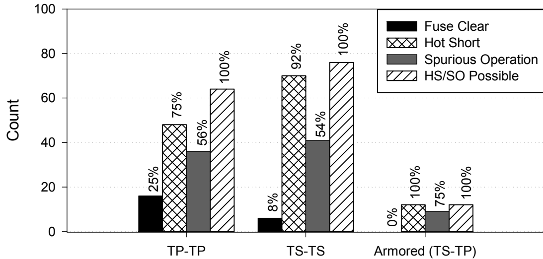
Figure 4-23. Insulation-jacket type column plot, global approach, DC tests
