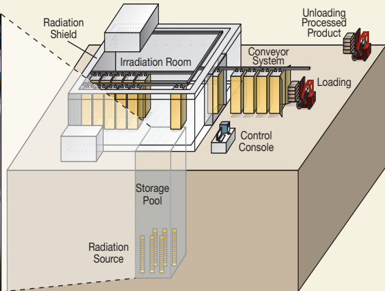
Figure 33. Commercial Irradiator
