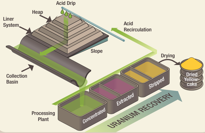
Figure 36. The Heap Leach Recovery Process
