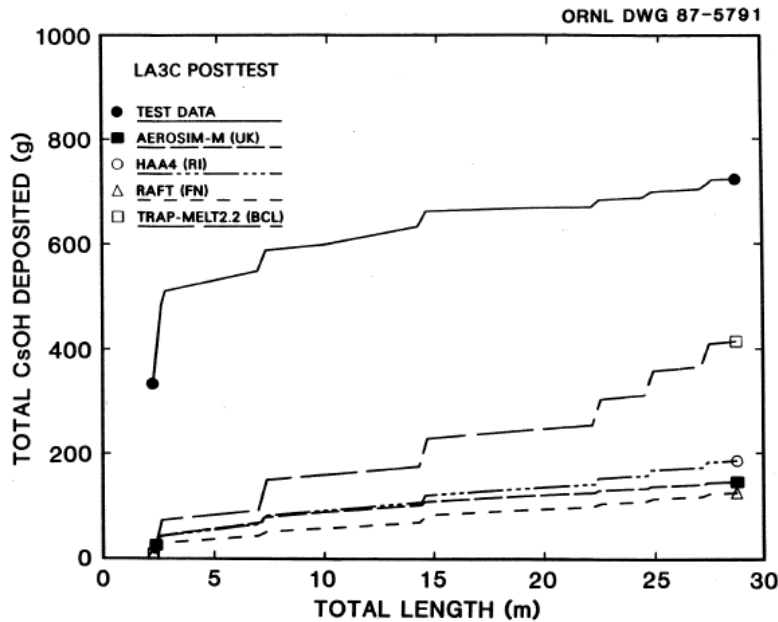
Figure D-56 LA3C post test calculation of CsOH aerosol deposition for codes including bend deposition models (LACE TR-024)
