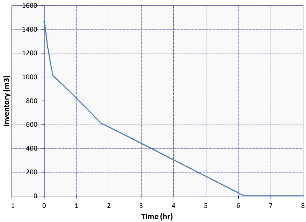
Figure 5-111 ISLOCA RWST Inventory
