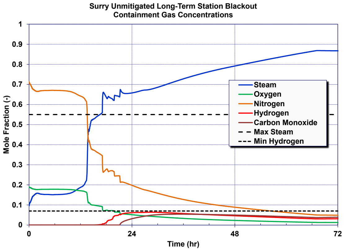
Figure 5-6 Unmitigated long-term station blackout containment gas concentrations
