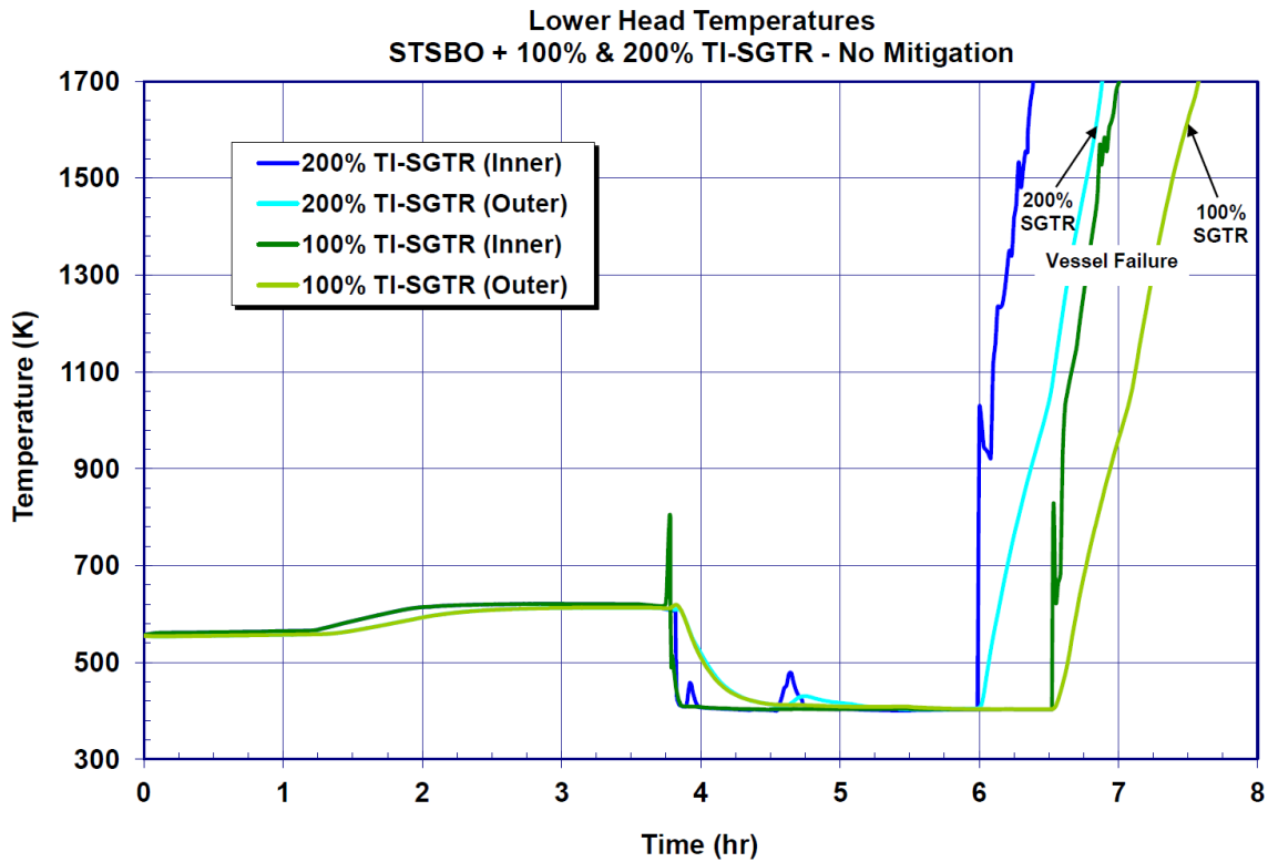
Figure 5-67 Unmitigated 100% and 200% TI-SGTR short-term station blackout lower head inner and outer temperature histories
