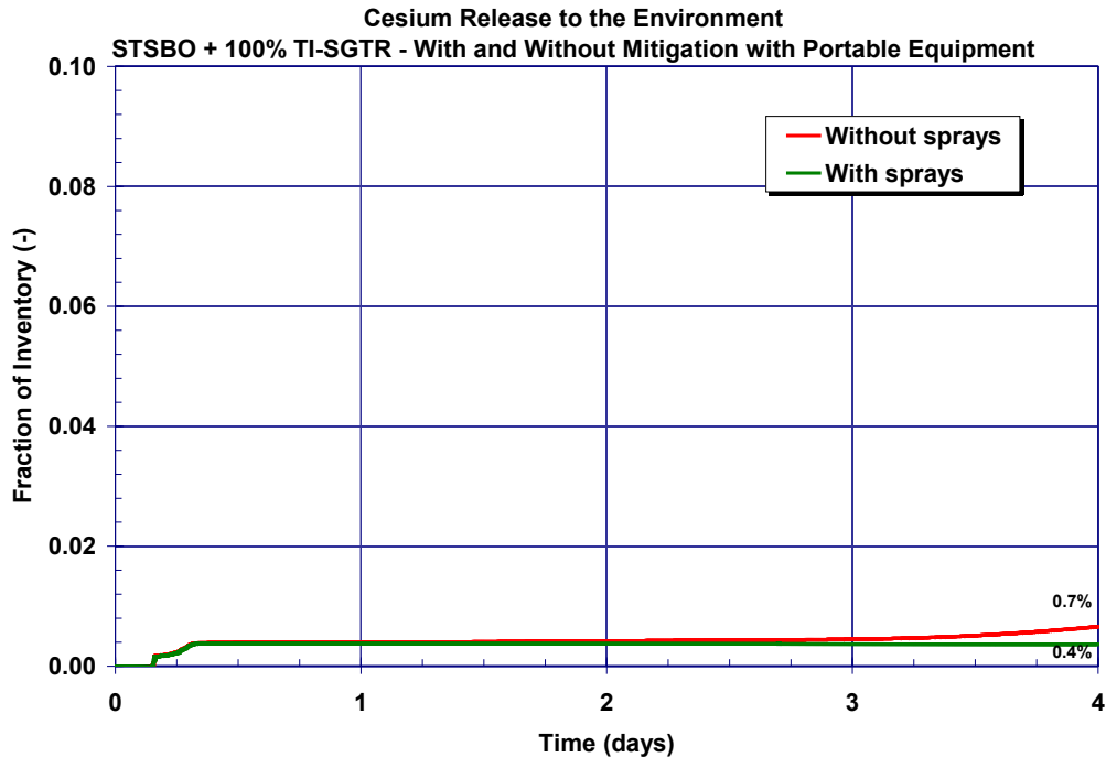
Figure 5-85 The short-term station blackout with a 100% thermally-induced SGTR with and without spray mitigation cesium environmental release
