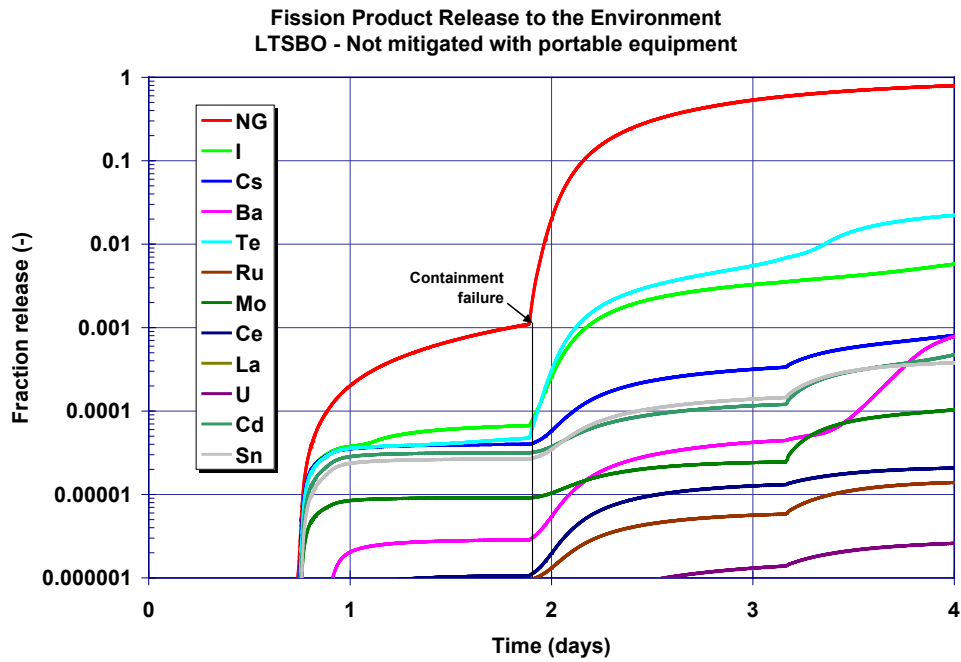
Figure 5-9 Unmitigated LTSBO environmental release history of all fission products
