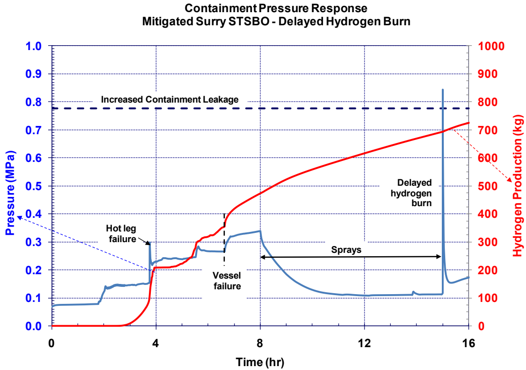
Figure 5-52 Mitigated short-term station blackout containment pressure history for the sensitivity calculation with delayed ignition
