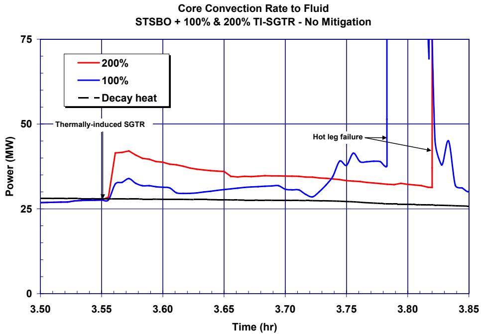
Figure 5-63 Unmitigated 100% and 200% TI-SGTR STSBO vessel convective heat removal rate from the fuel
