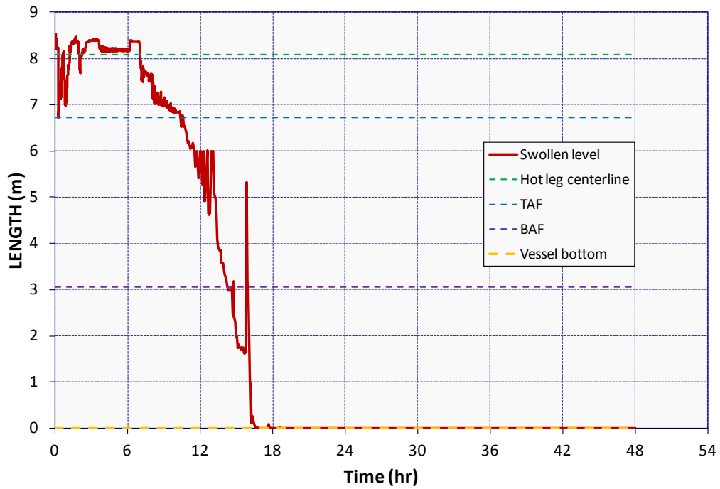
Figure 5-113 ISLOCA Reactor Vessel Water Level
