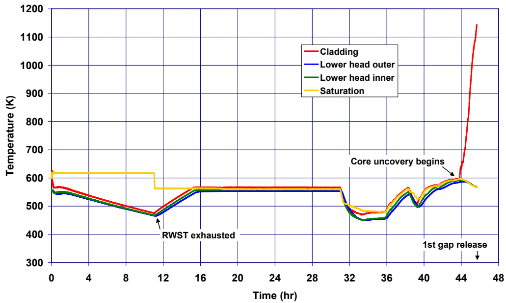
Figure 5-98 SGTR with Failed Operator Action – Maximum Cladding and Lower Head Temperatures
