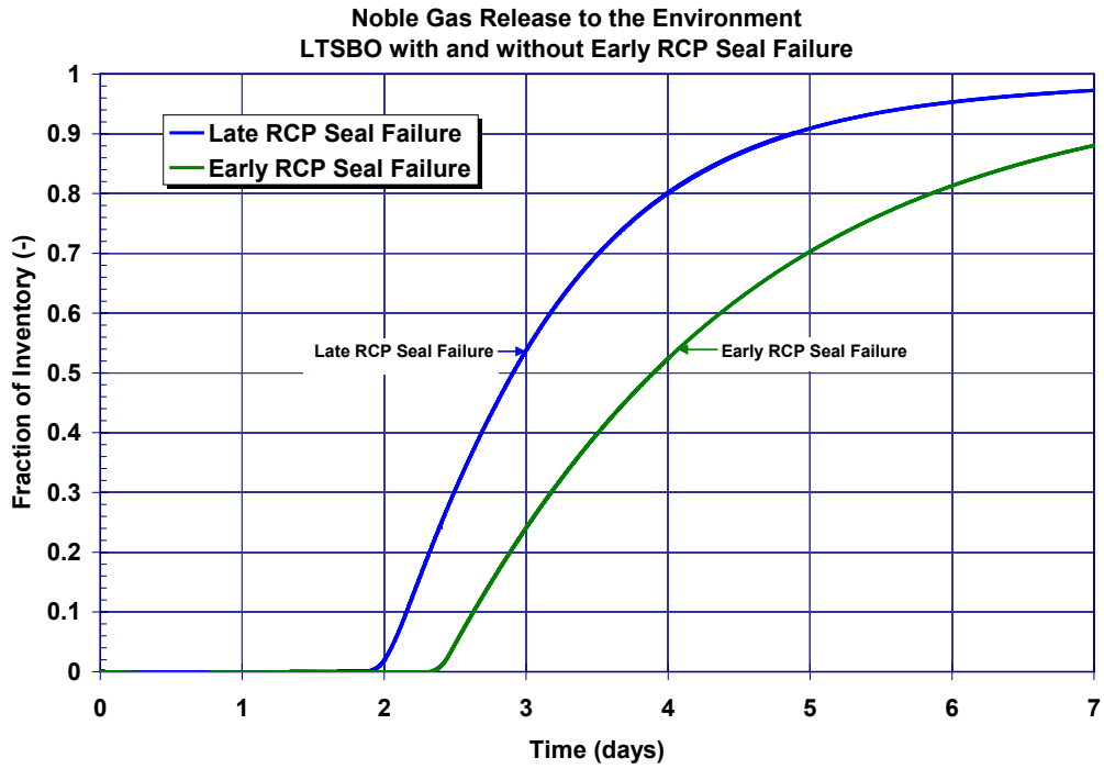
Figure 5-21 Comparison of the unmitigated long-term station blackout noble gas releases to the environment with and without early RCP seal failures
