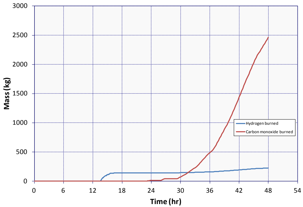
Figure 5-123 ISLOCA Integral Mass of H 2 & CO Burned in Safeguards Area
