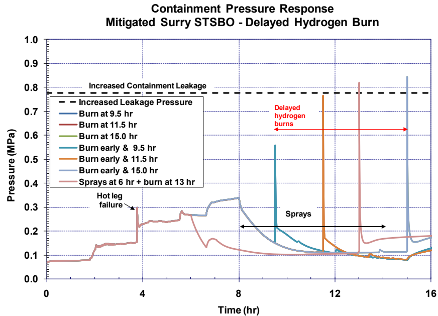
Figure 5-54 Comparison of the containment pressure responses for the sensitivity calculations with delayed ignition
