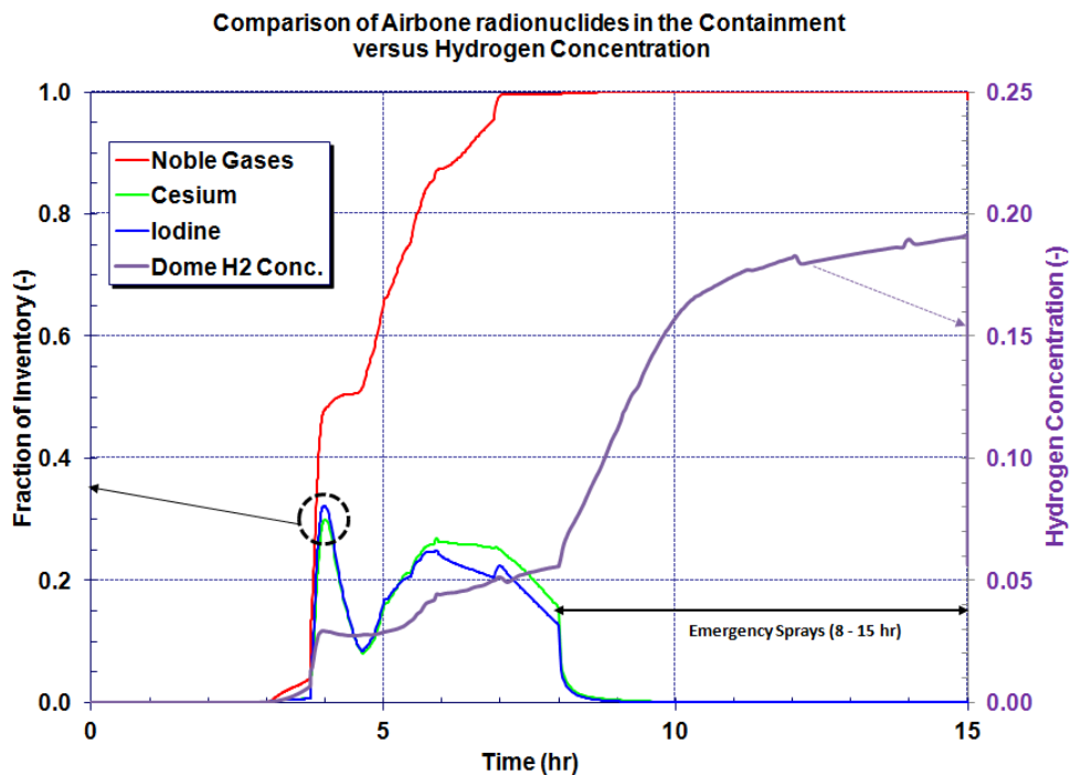
Figure 5-59 Mitigated short-term station blackout containment airborne radionuclide history versus hydrogen concentrations for the sensitivity calculation with delayed ignition
