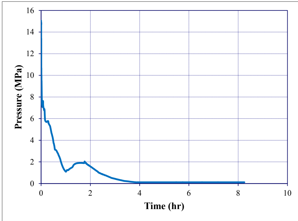
Figure 5-162 ISLOCA HHSI Throttling Sensitivity - RCS Pressure
