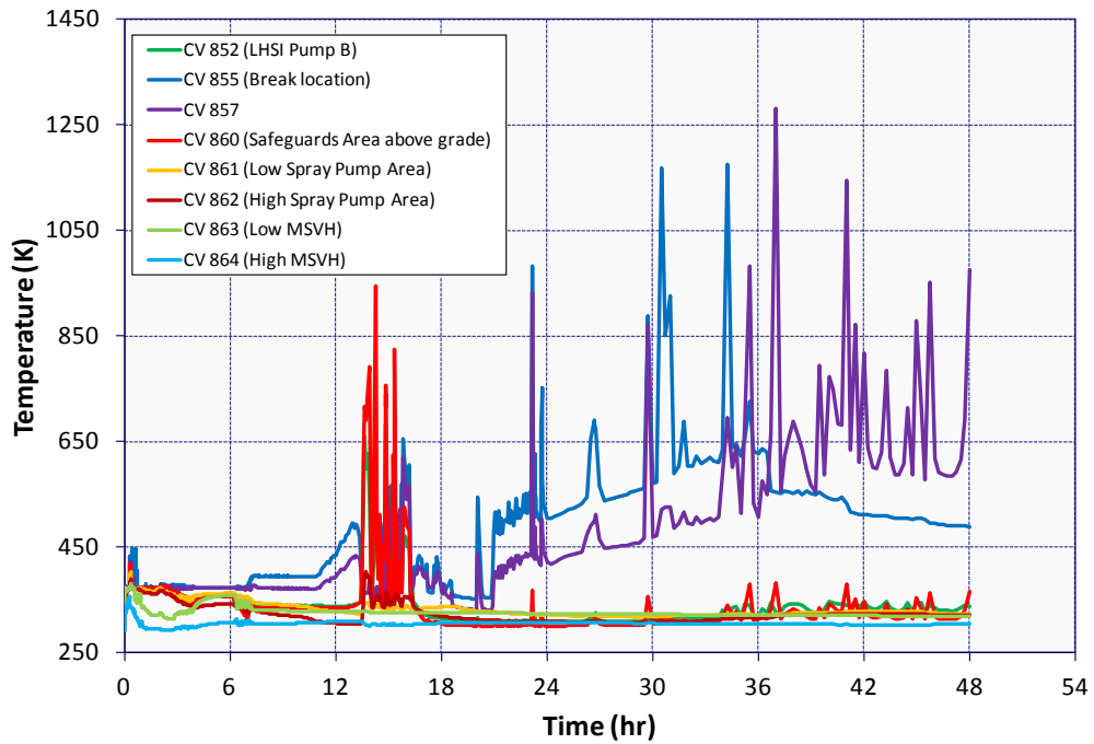
Figure 5-120 ISLOCA Safeguards Temperature
