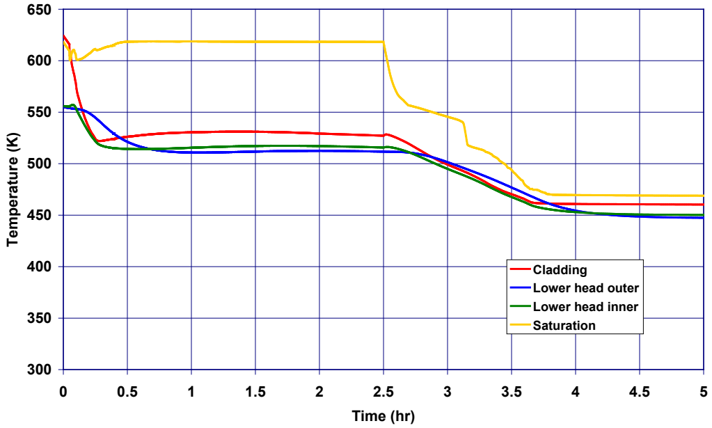
Figure 5-92 SGTR with Operator Action – Maximum Cladding and Lower Head Temperatures
