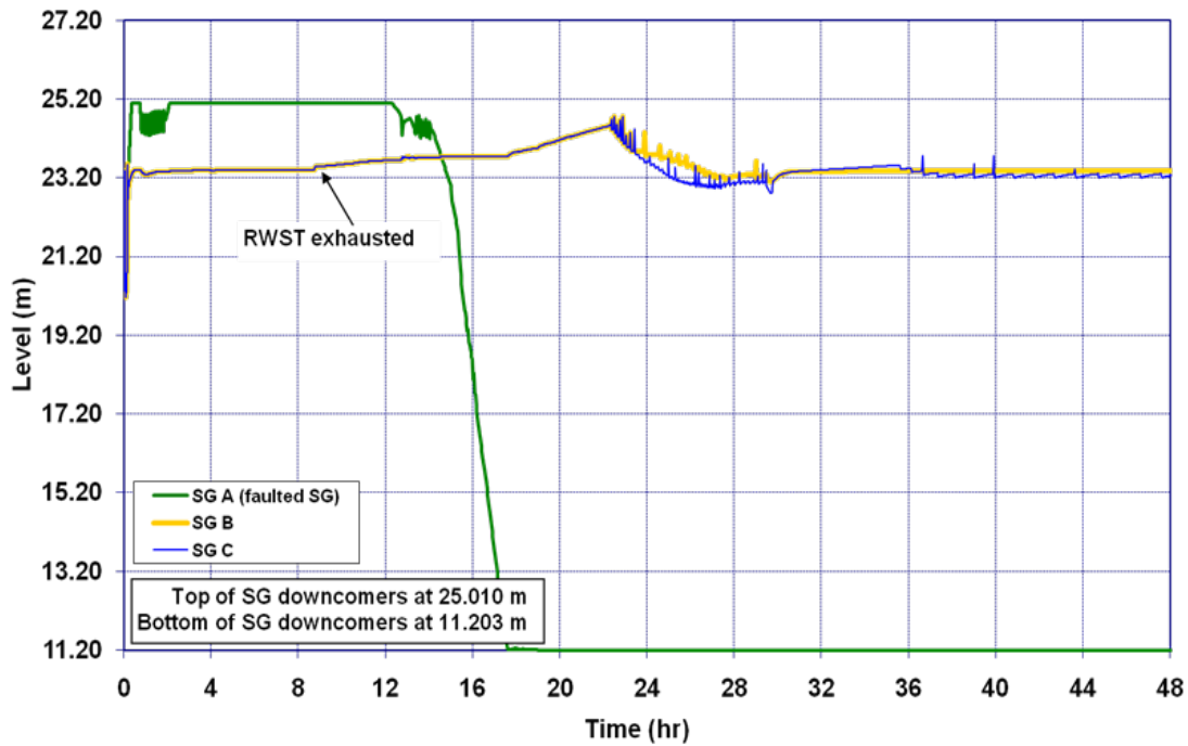
Figure 5-107 SGTR with Failed Operator Action and SORV- Steam Generator Level
