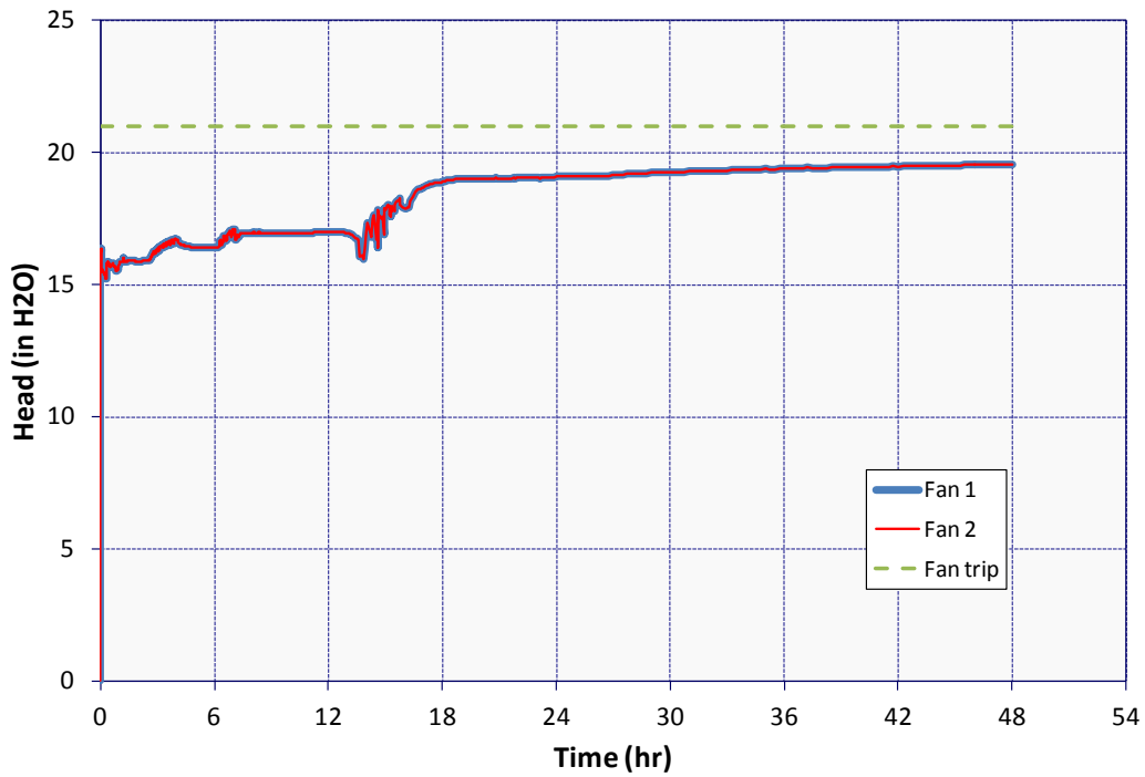
Figure 5-125 ISLOCA Safeguards Exhaust Ventilation Fan Head
