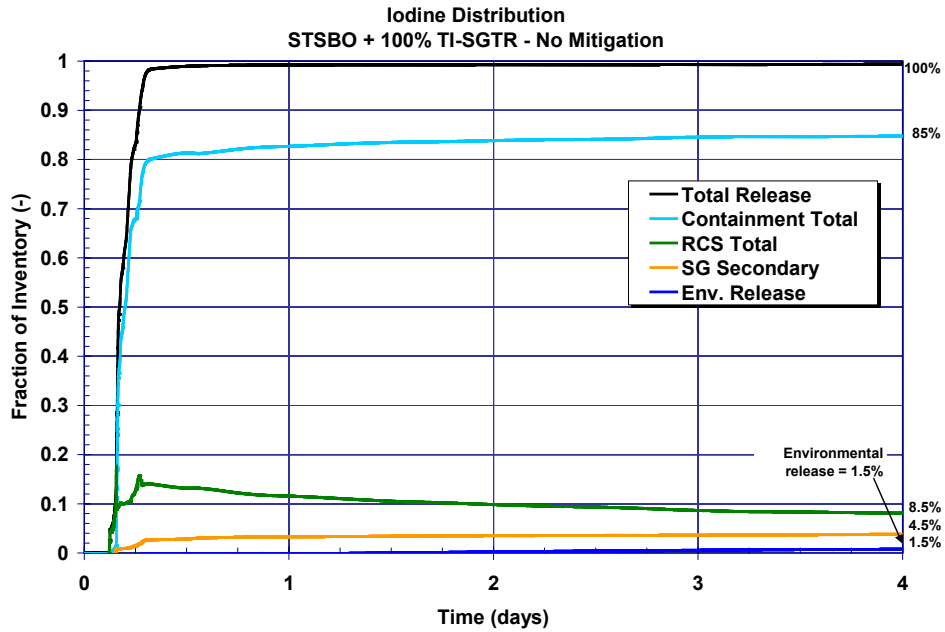
Figure 5-70 Unmitigated 100% TI-SGTR STSBO iodine fission product distribution history
