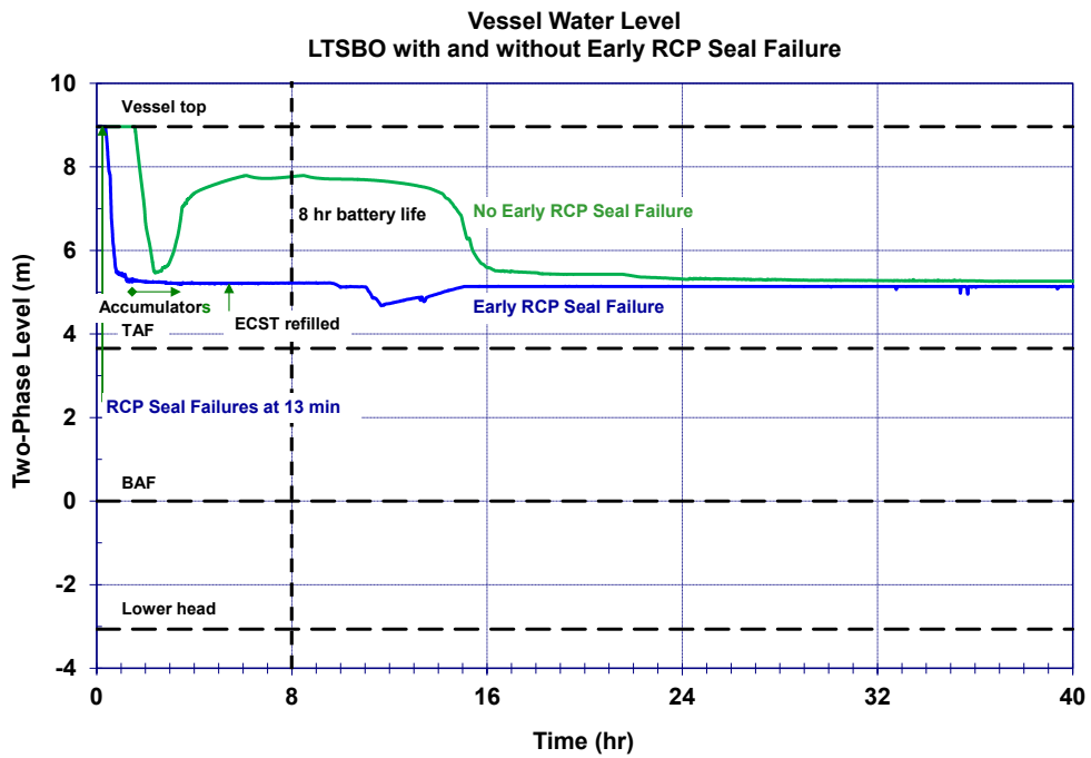
Figure 5-26 Comparison of the mitigated long-term station blackout vessel level with and without early RCP seal failures
