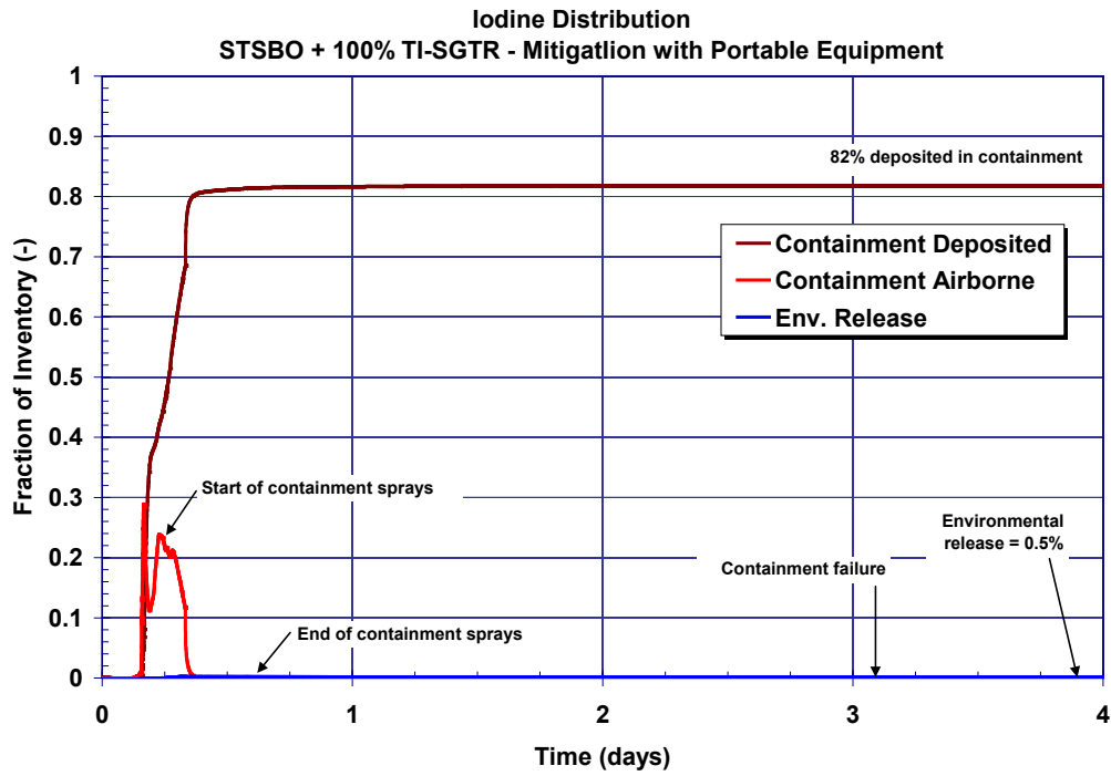
Figure 5-82 The iodine distribution in the containment for short-term station blackout with a 100% thermally-induced SGTR with spray mitigation
