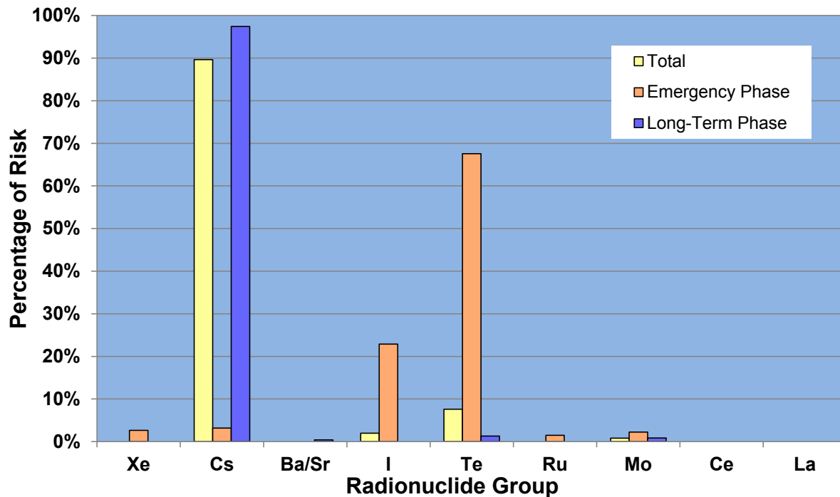
Figure 7-12 Percentage contribution to total, emergency-phase, and long-term-phase, mean, individual risk for the population within 10 miles by chemical class for the Surry unmitigated ISLOCA based on the LNT hypothesis
