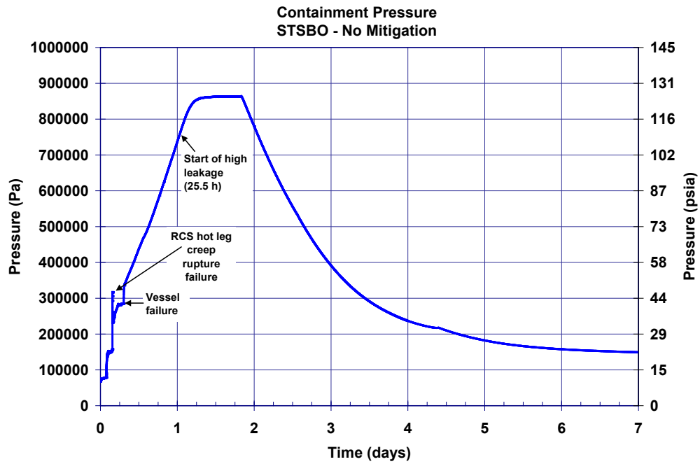
Figure 5-33 Unmitigated short-term station blackout containment pressure history
