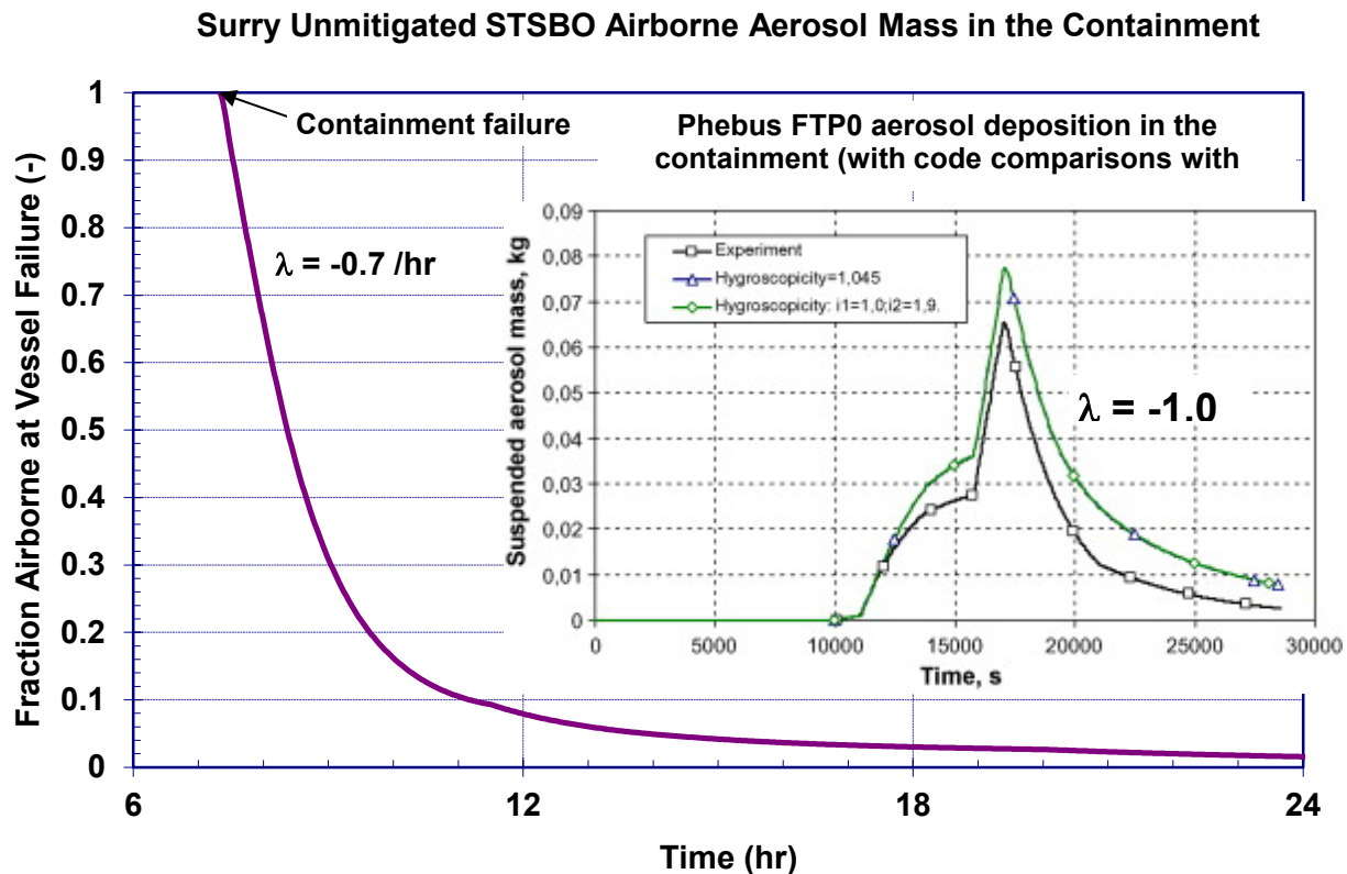
Figure 5-168 Unmitigated STSBO airborne aerosol mass in the containment following vessel failure
