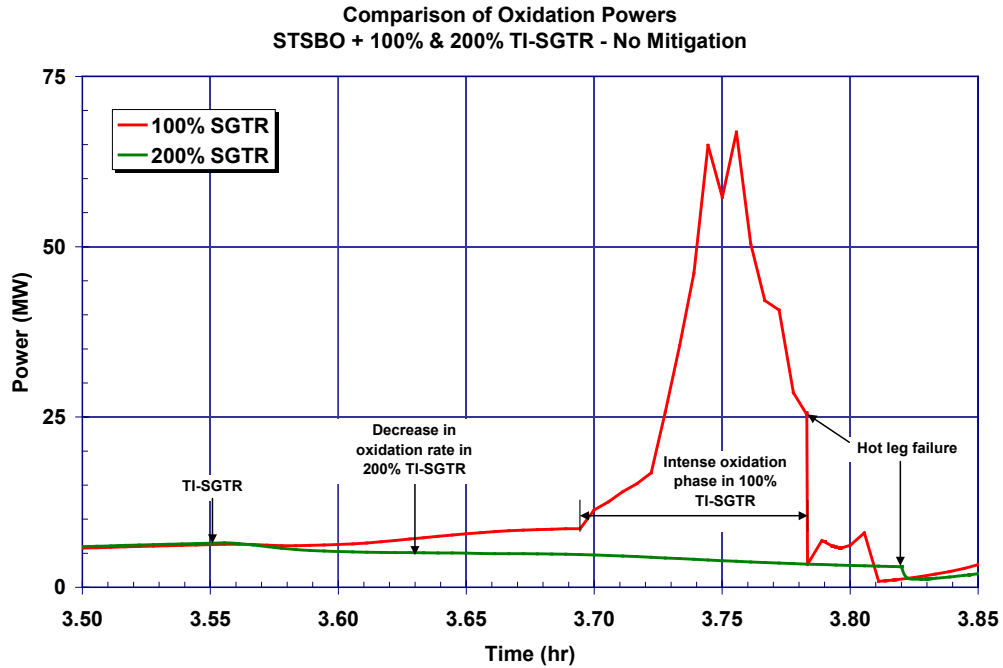
Figure 5-64 Unmitigated 100% and 200% TI-SGTR STSBO fuel oxidation power before the RCS hot leg failure
