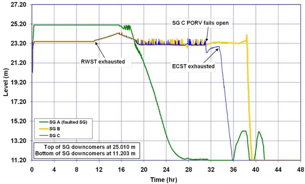
Figure 5-101 SGTR with Failed Operator Action- Steam Generator Level
