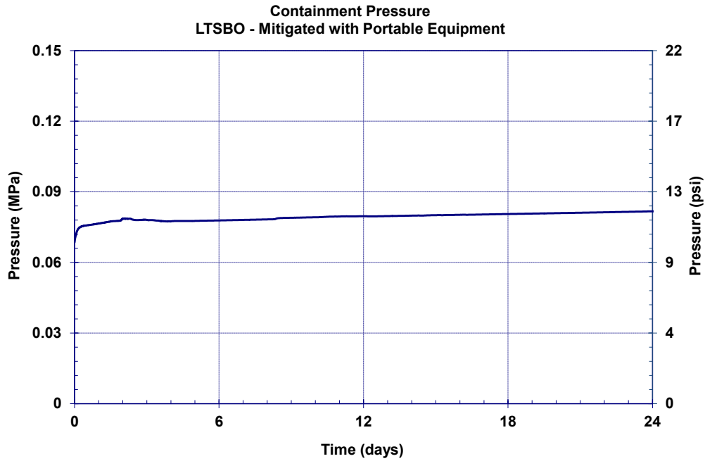
Figure 5-14 Mitigated long-term station blackout containment pressure history
