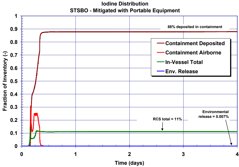
Figure 5-46 Mitigated short-term station blackout iodine fission product distribution history 27
