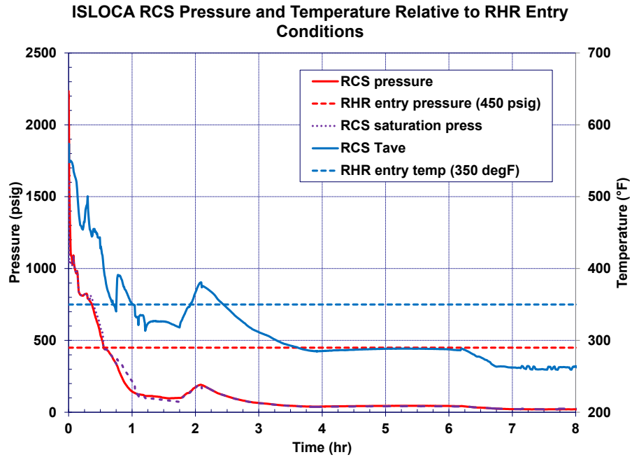
Figure 5-145 ISLOCA RCS Pressure and Temperature Relative to the RHR Entry Pressure and Temperature Criteria for the Unmitigated ISLOCA
