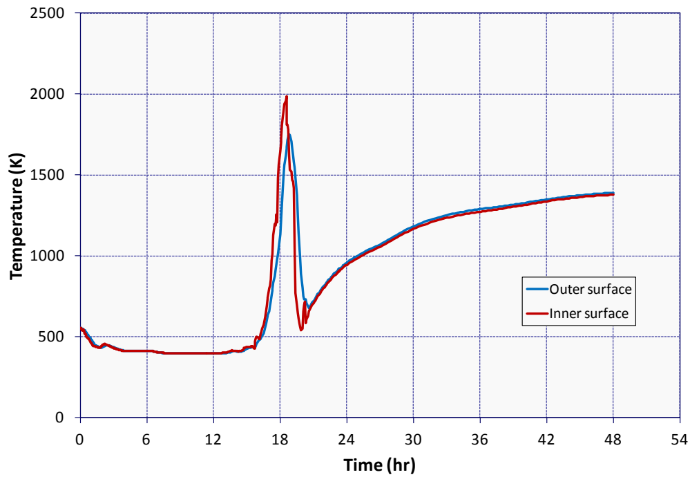
Figure 5-116 ISLOCA Reactor Vessel Lower Head Temperature
