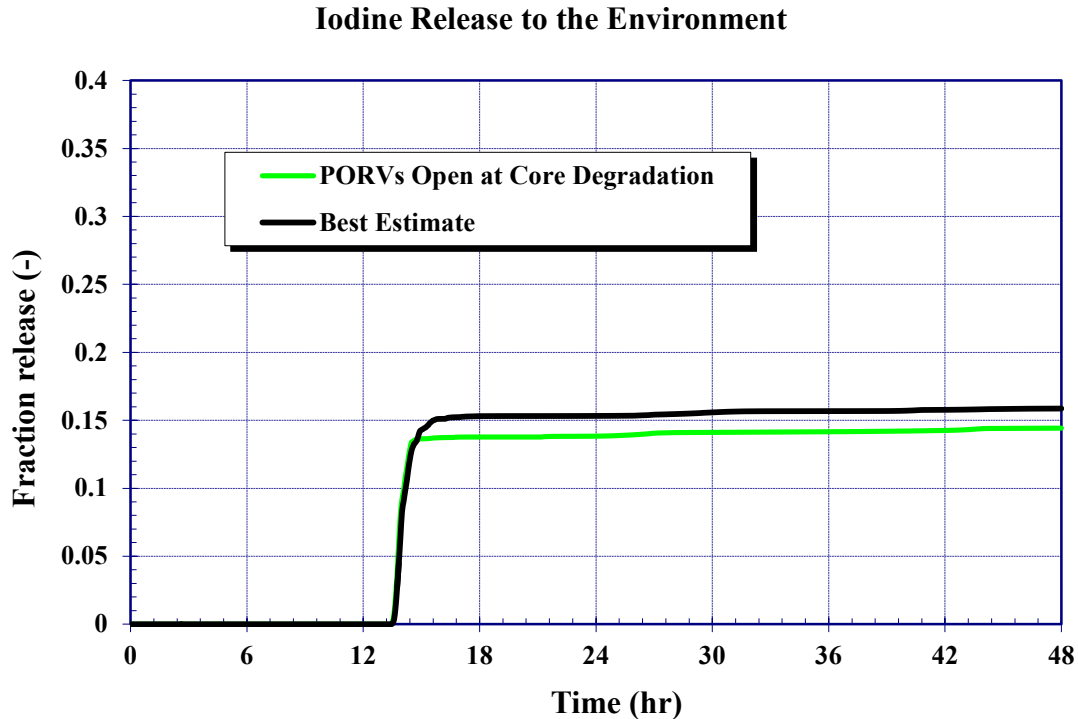
Figure 5-159 Iodine Release to the Environment – PORVs Open at Core Degradation
