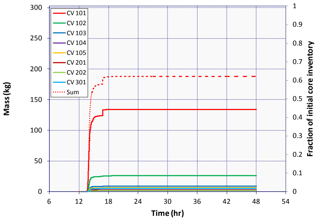
Figure 5-143 Cs 2 MoO 4 Capture along LHSI Piping in ISLOCA Deposition Calculation
