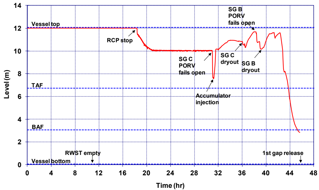
Figure 5-97 SGTR with Failed Operator Action – RPV Water Level
