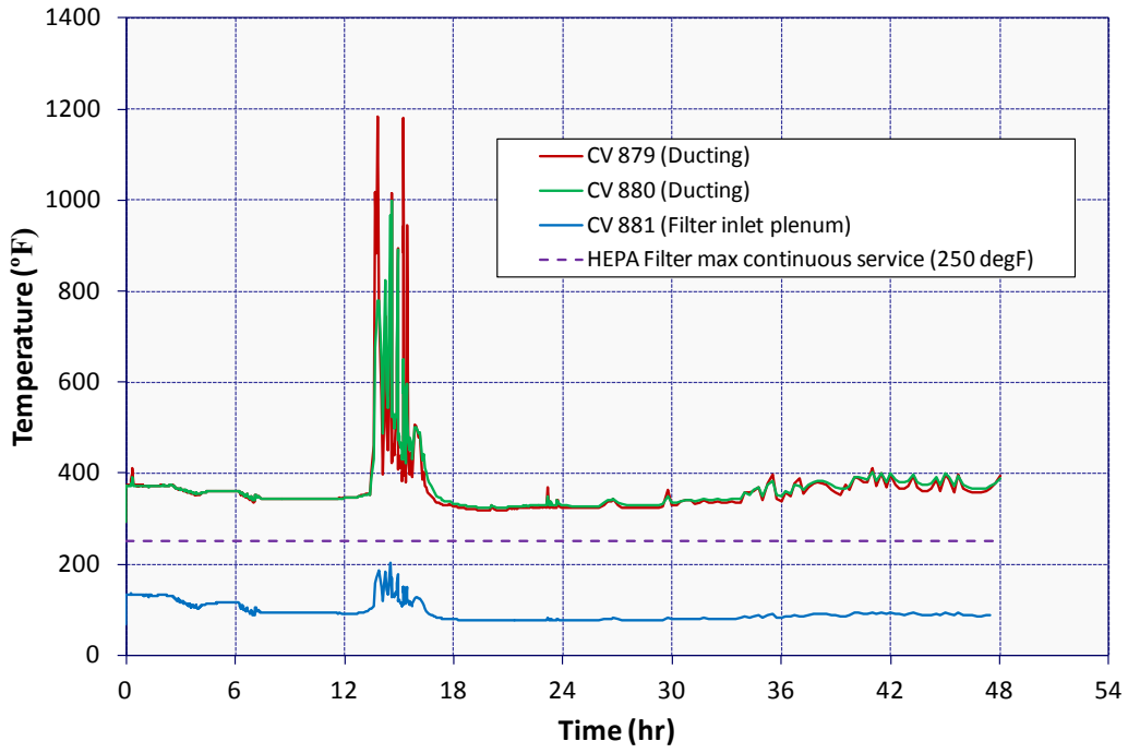
Figure 5-129 ISLOCA Safeguards Exhaust Ventilation Duct and Filter Inlet Temperature
