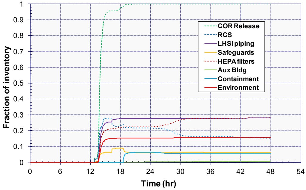
Figure 5-133 ISLOCA Iodine Distribution
