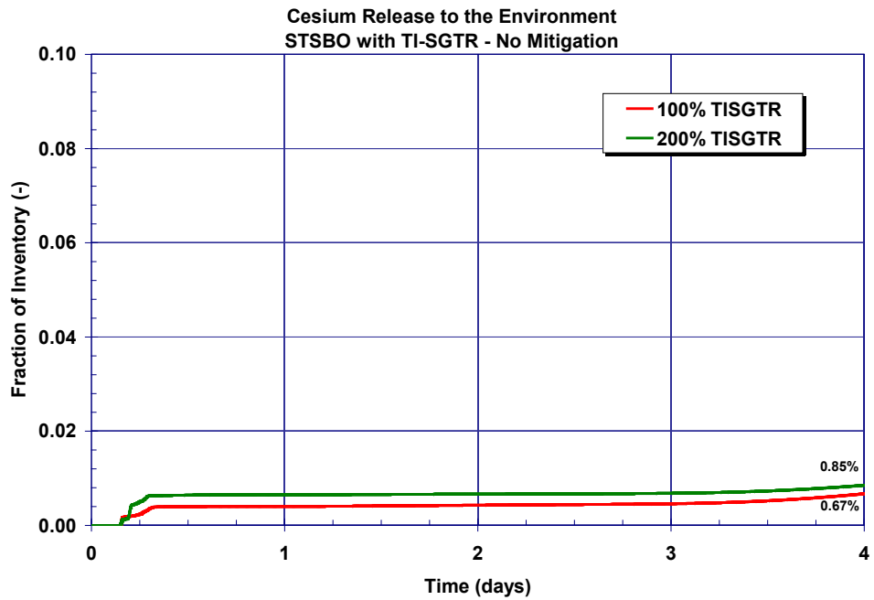
Figure 5-75 The unmitigated 100% and 200% TI-SGTR short-term station blackout cesium fission product distribution history
