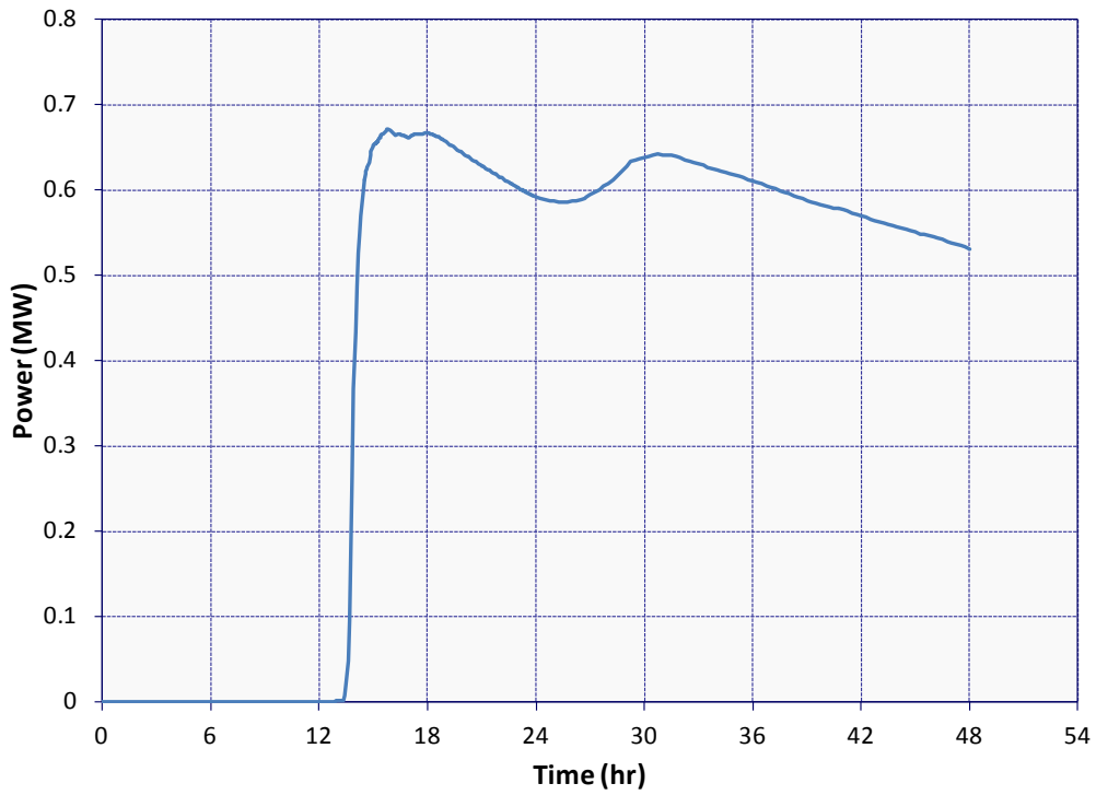
Figure 5-130 ISLOCA Decay Power of Fission Products Captured in Safeguards Exhaust Ventilation HEPA Filters
