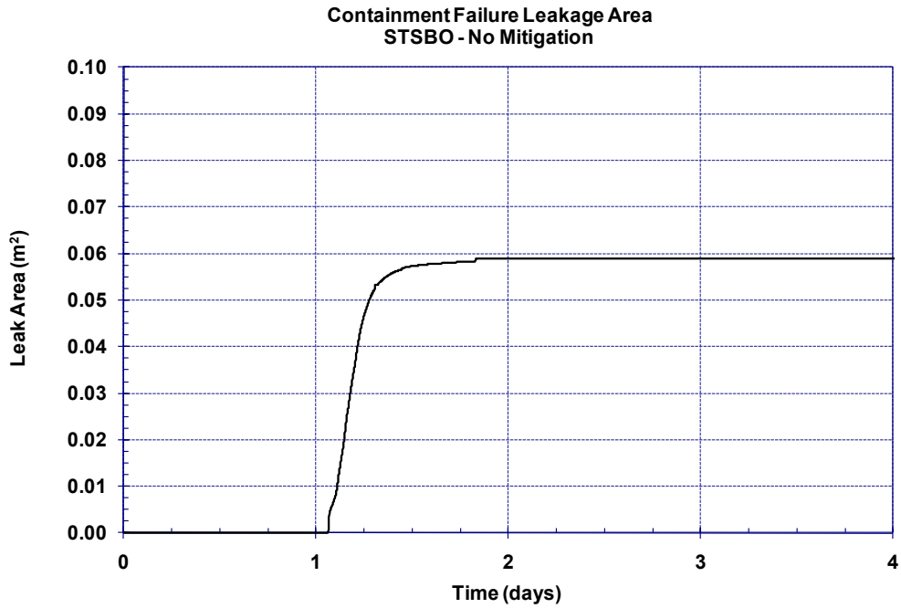
Figure 5-34 Unmitigated short-term station blackout containment leakage area
