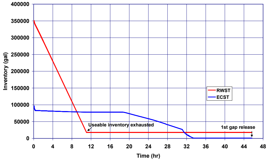
Figure 5-99 SGTR with Failed Operator Action – RWST and ECST Inventories
