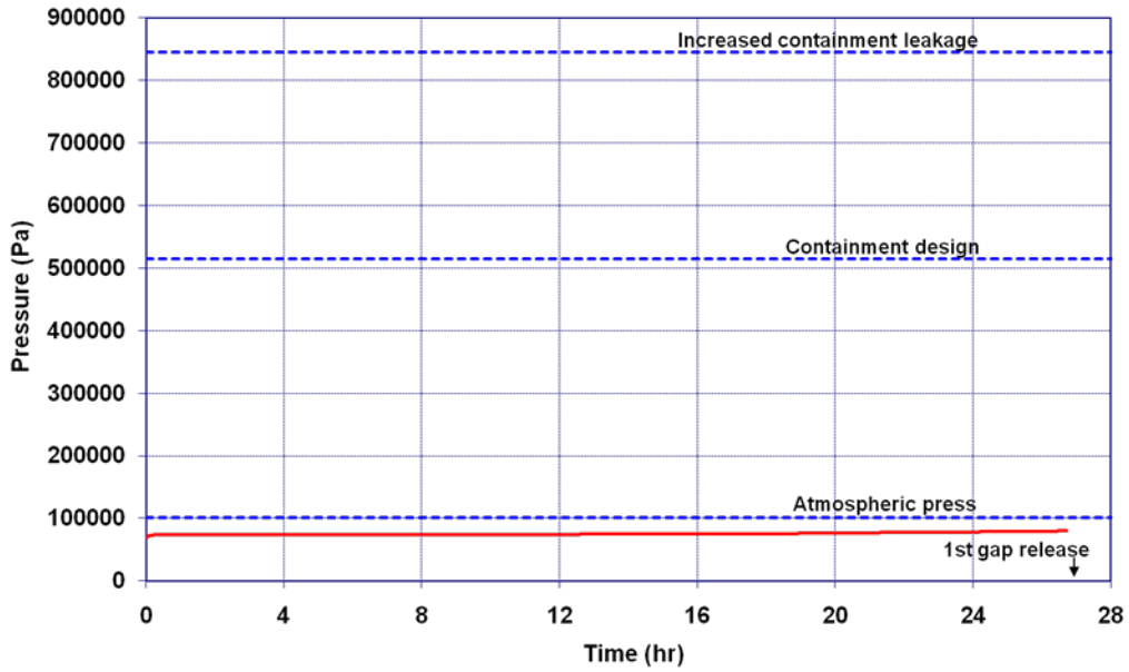
Figure 5-106 SGTR with Failed Operator Action and SORV- Containment Pressure
