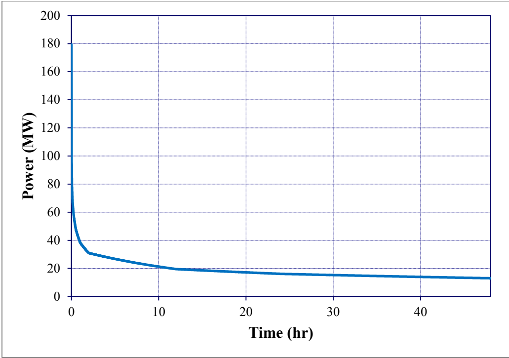
Figure 5-161 ISLOCA HHSI Throttling Sensitivity - Fission Product Decay Power
