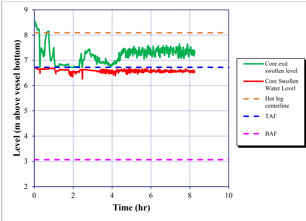
Figure 5-163 ISLOCA HHSI Throttling Sensitivity - Core Water Level
