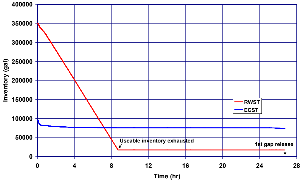
Figure 5-105 SGTR with Failed Operator Action with SORV – RWST and ECST Inventories
