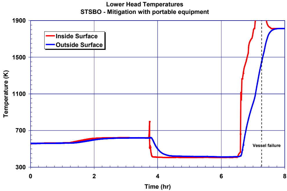
Figure 5-42 Mitigated STSBO lower head inner and outer temperature history
