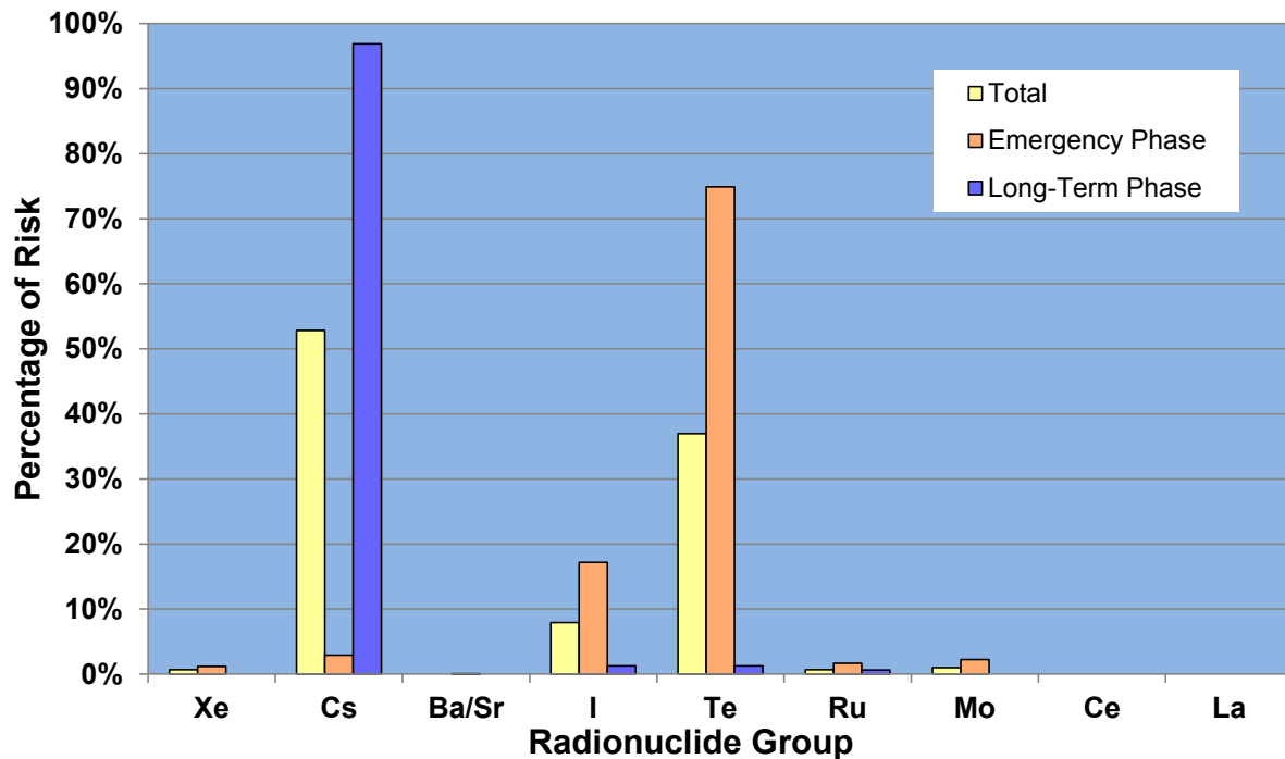
Figure 7-15 Percentage contribution to total, emergency-phase, and long-term-phase, mean, individual risk for the population within 20 miles by chemical class for the Surry unmitigated ISLOCA based on LNT hypothesis
