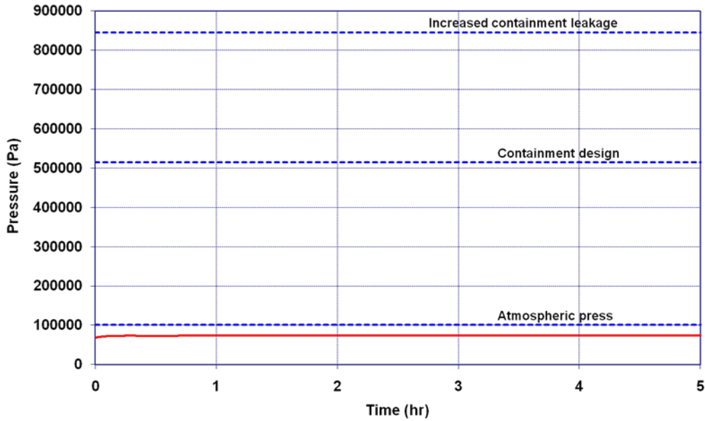
Figure 5-94 SGTR with Operator Action- Containment Pressure
