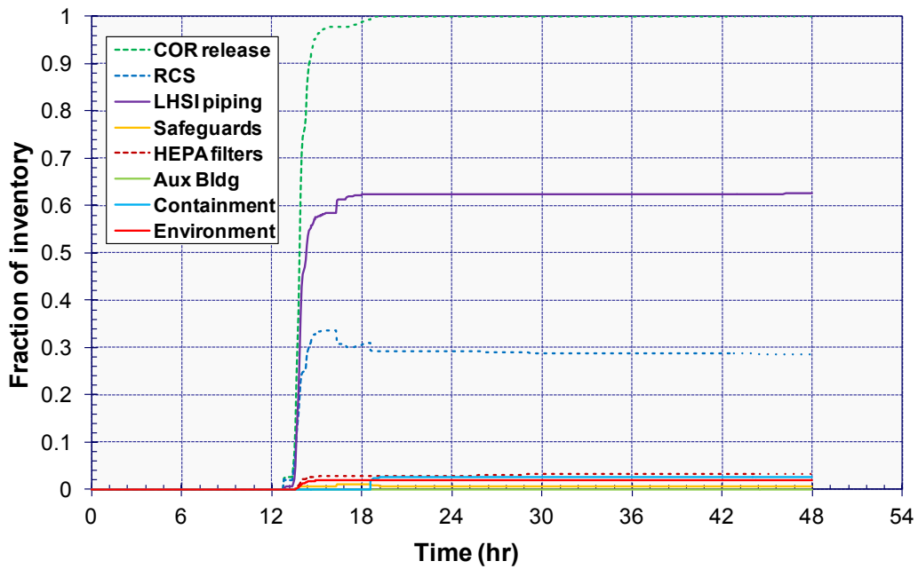
Figure 5-132 ISLOCA Cesium Distribution
