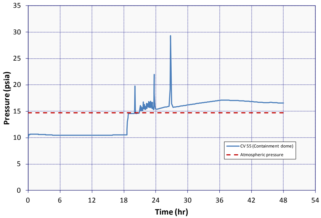
Figure 5-117 ISLOCA Containment Pressure
