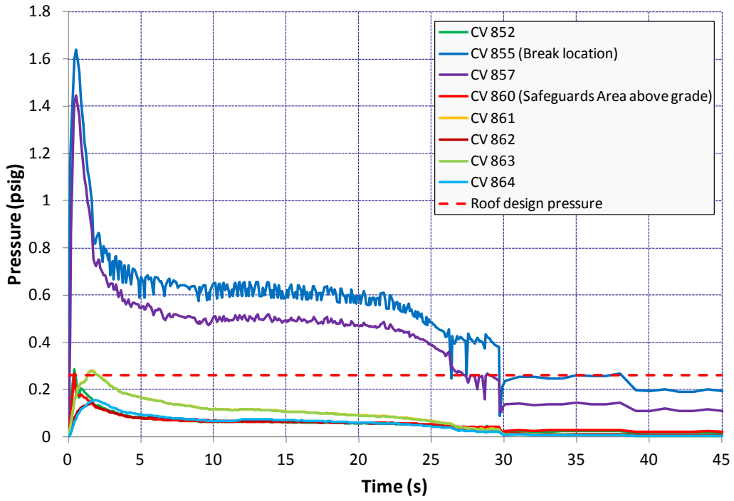
Figure 5-119 ISLOCA Safeguards Pressure
