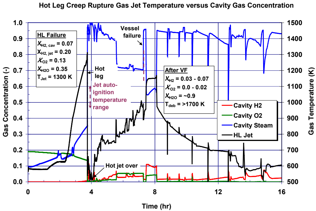
Figure 5-50 Comparison of the mitigated short-term station blackout containment cavity gas concentration history and potential ignition source temperatures
