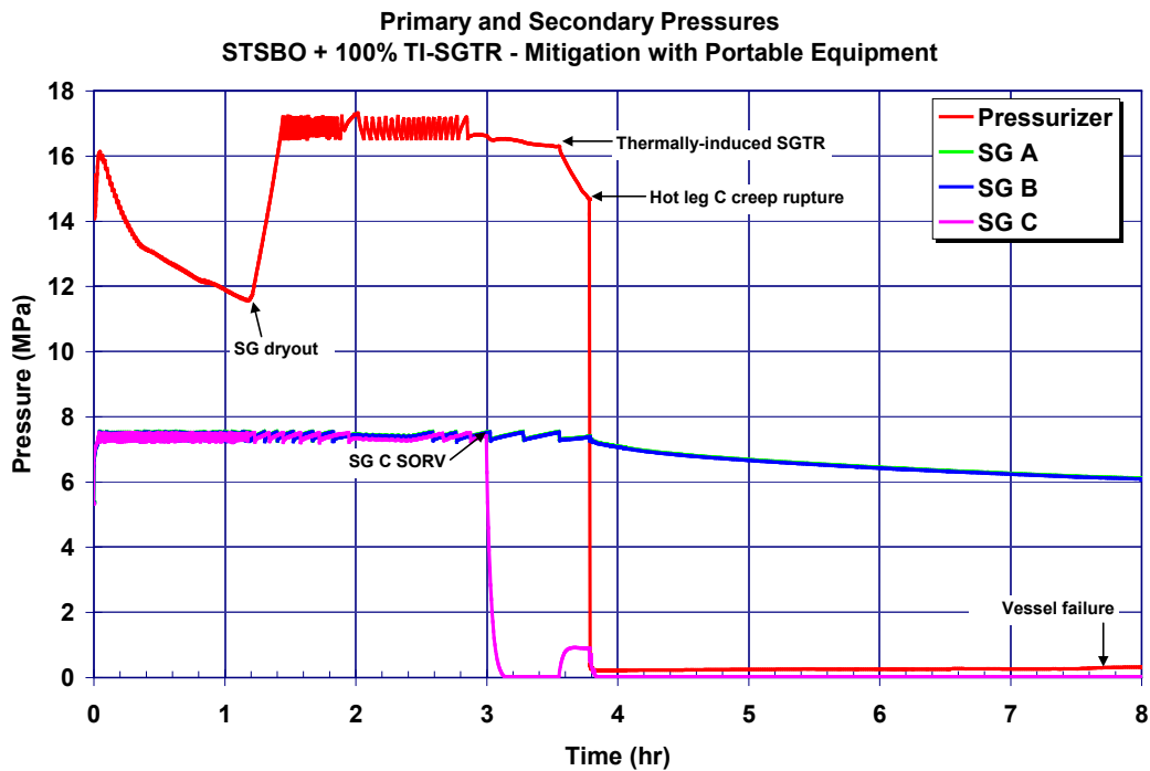
Figure 5-78 The mitigated STSBO primary and secondary pressure history
