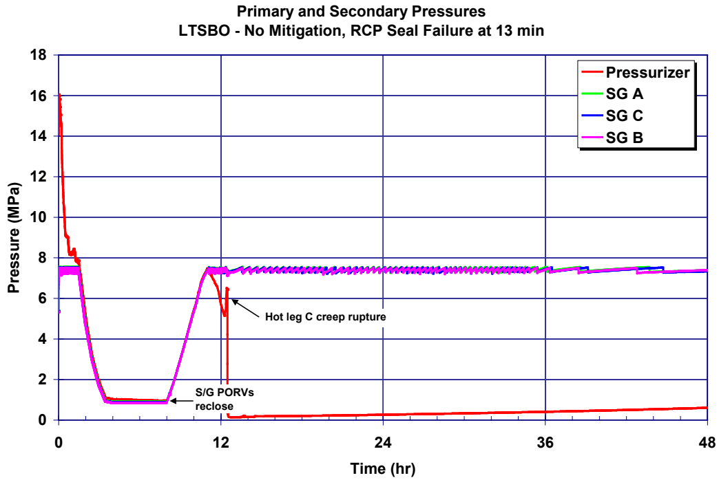
Figure 5-16 Unmitigated long-term station blackout primary and secondary pressure history
