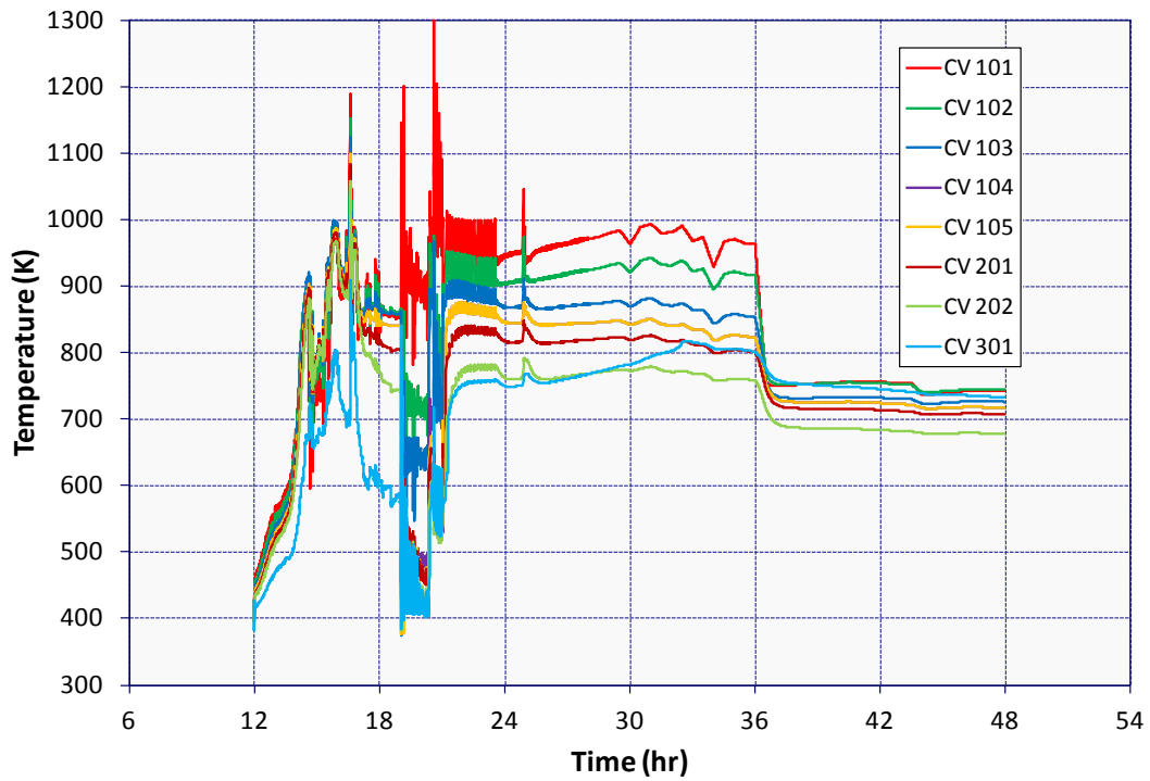
Figure 5-136 Vapor Temperature Along LHSI Piping in ISLOCA Deposition Calculation
