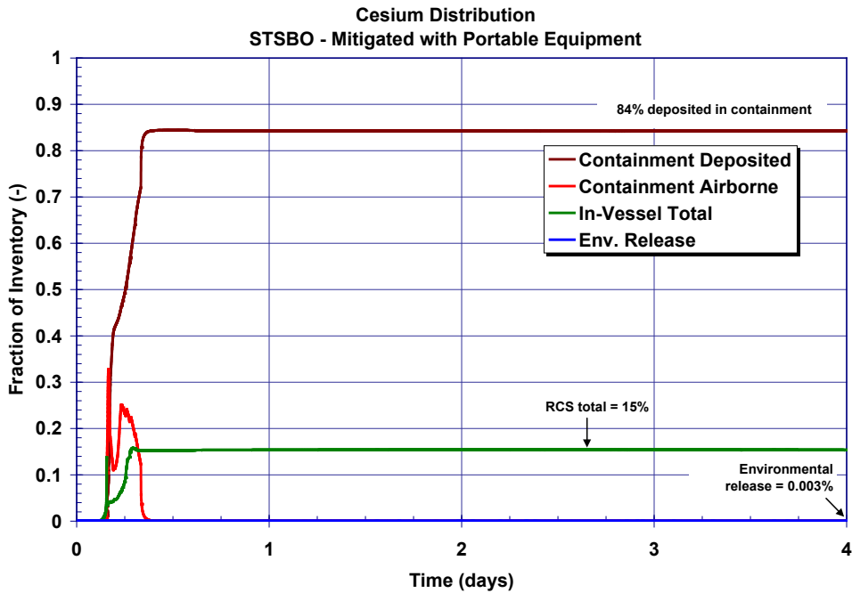
Figure 5-47 Mitigated STSBO cesium fission product distribution history
