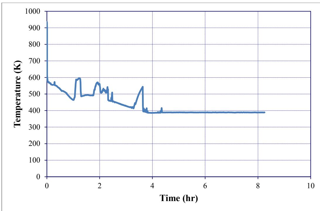
Figure 5-164 ISLOCA HHSI Throttling Sensitivity - Maximum Core Temperature
