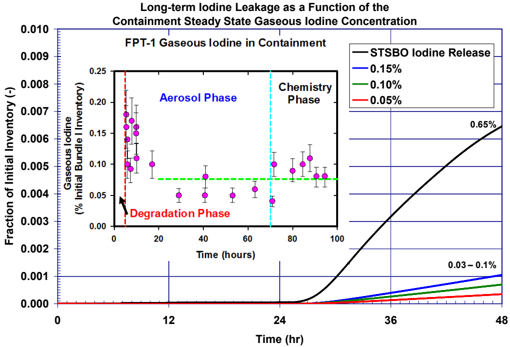
Figure 5-165 The additional gaseous iodine source term using Phebus data is compared to the iodine source term for the unmitigated short-term station blackout
