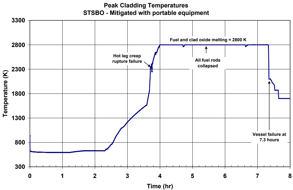
Figure 5-41 Mitigated short-term station blackout core temperature history
