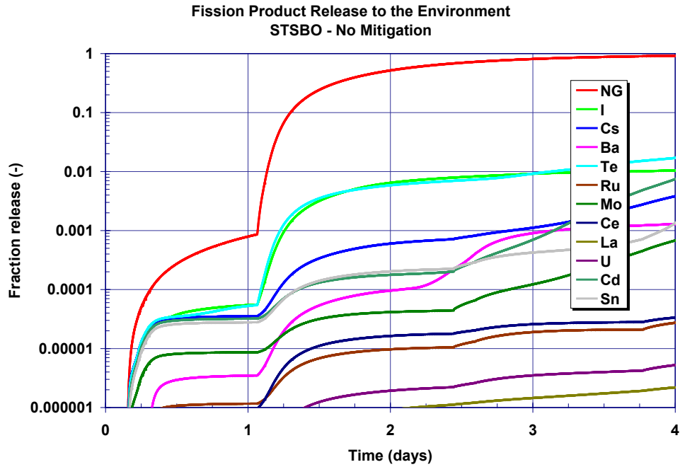
Figure 5-38 Unmitigated STSBO environmental release history of all fission products
