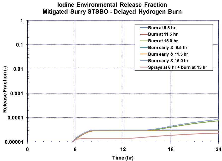
Figure 5-56 Comparison of the iodine release to the environment for the sensitivity calculations with delayed ignition
