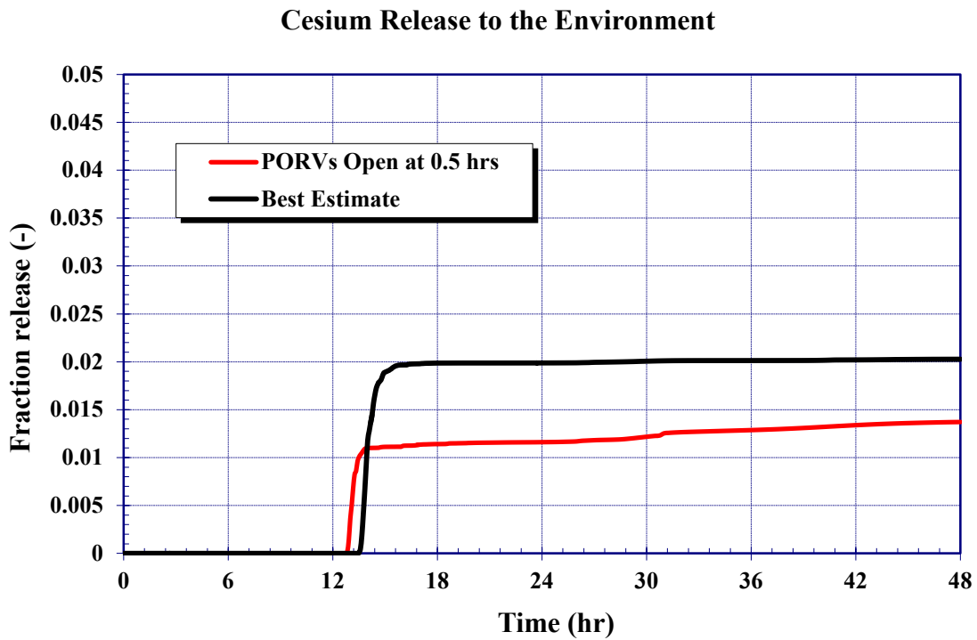
Figure 5-154 Cesium Release to the Environment – PORVs Open at 0.5 hrs
