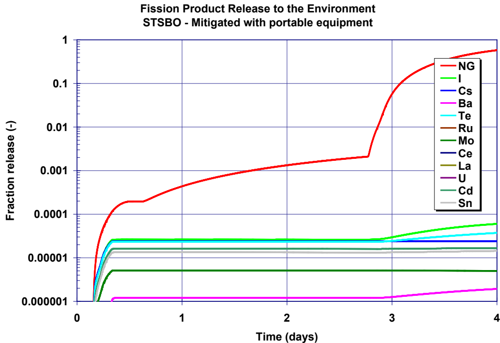
Figure 5-48 Mitigated STSBO environmental release history of all fission products
