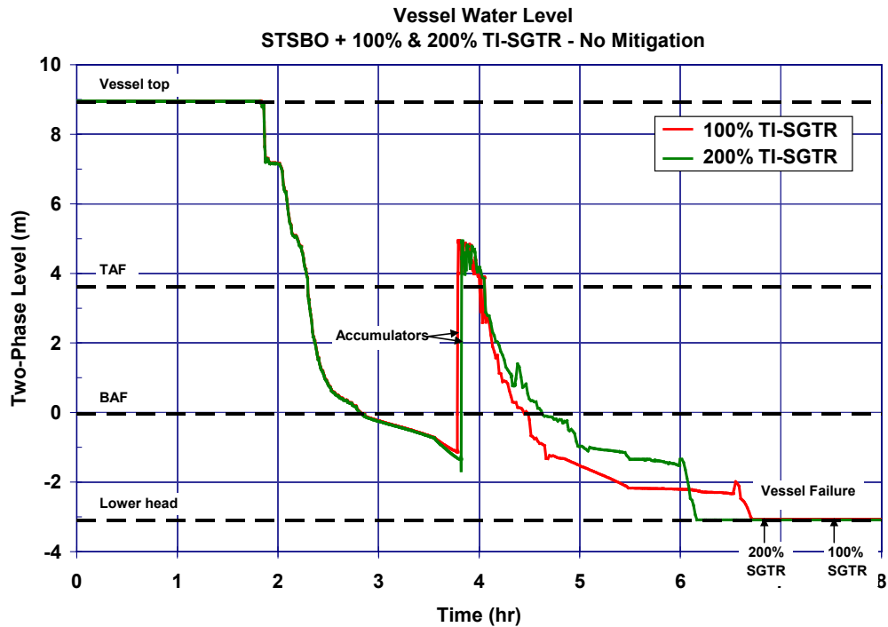
Figure 5-65 Unmitigated 100% and 200% TI-SGTR short-term station blackout vessel two-phase coolant level
