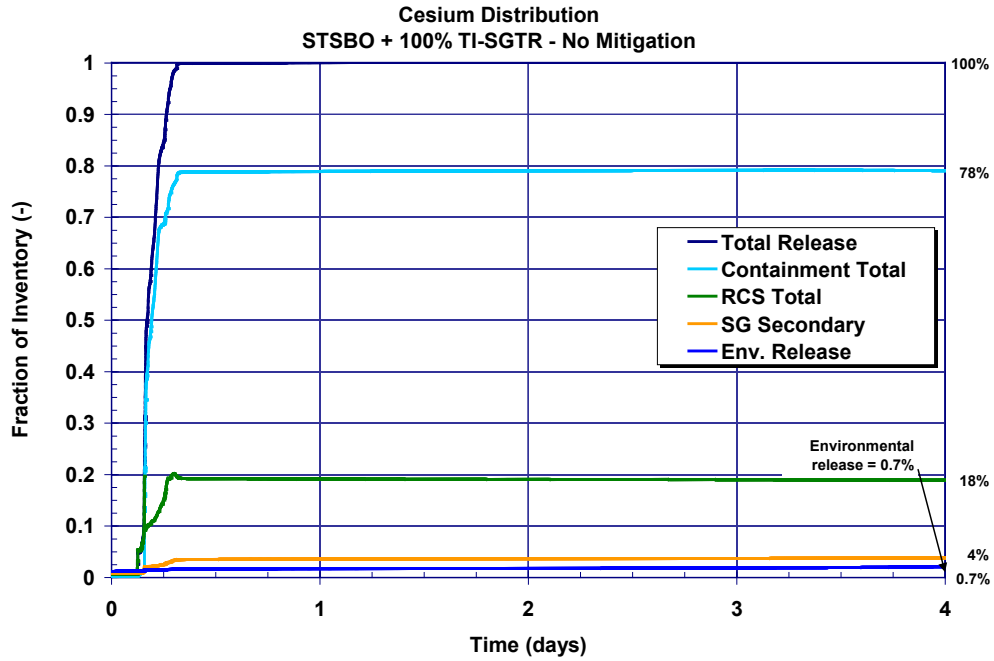
Figure 5-72 The unmitigated 100% TI-SGTR short-term station blackout cesium fission product distribution history
