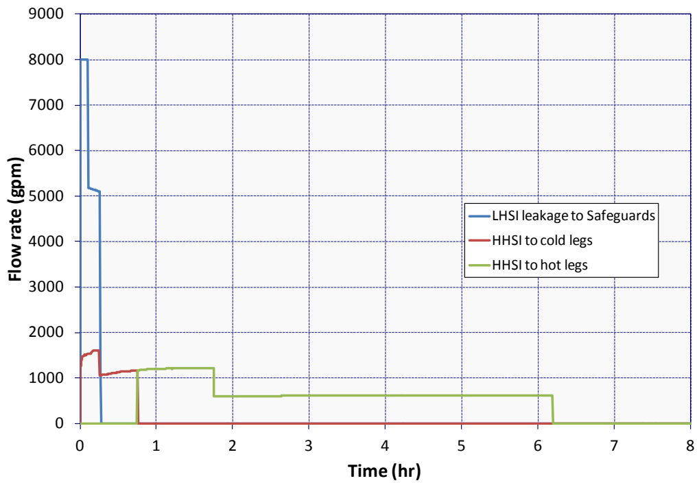
Figure 5-110 ISLOCA ECCS Flow
