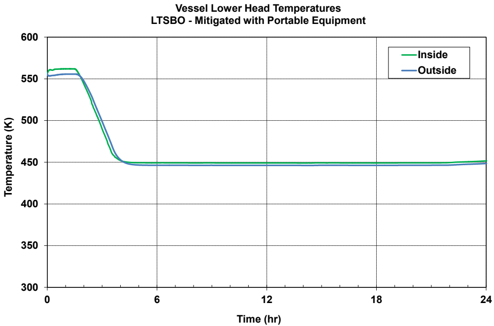
Figure 5-13 Mitigated long-term station blackout lower head inner and outer temperature history
