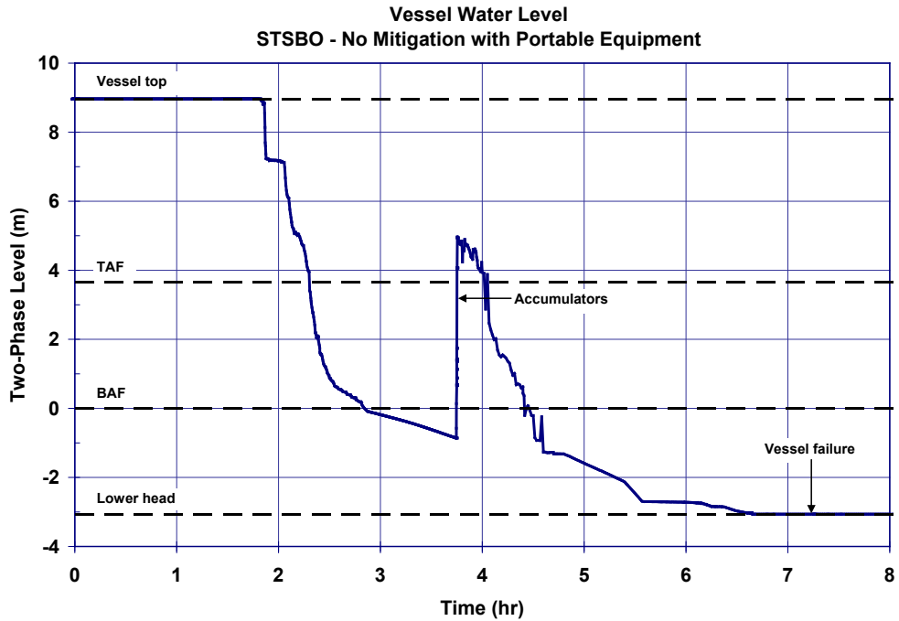
Figure 5-29 Unmitigated short-term station blackout vessel two-phase coolant level
