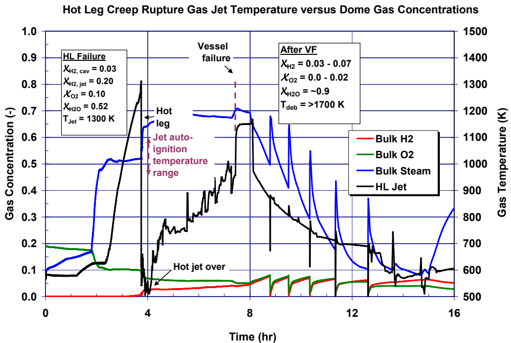
Figure 5-51 Comparison of the mitigated short-term station blackout containment dome gas concentration history and potential ignition source temperature
