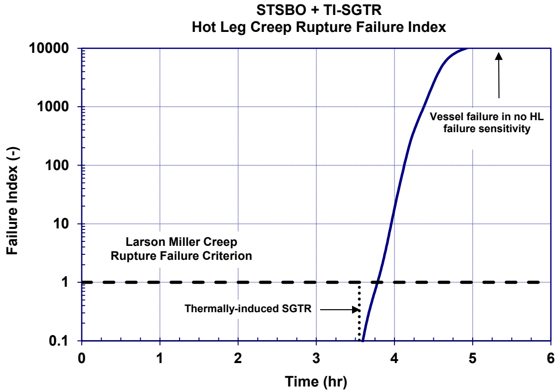
Figure 5-86 The hot leg creep rupture failure index in the short-term station blackout sensitivity case with a 100% thermally-induced SGTR and no hot leg failure
