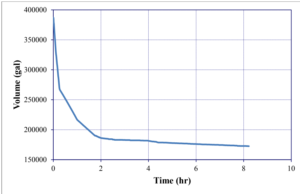
Figure 5-160 ISLOCA HHSI Throttling Sensitivity - RWST Inventory
