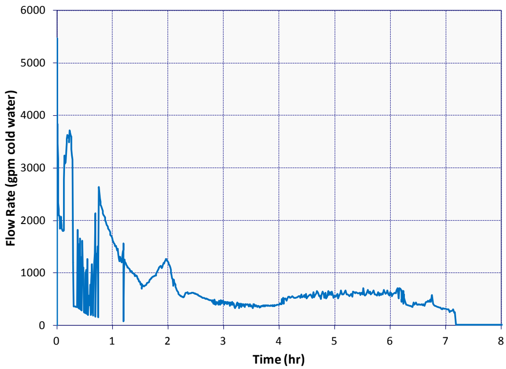
Figure 5-109 ISLOCA Break Flow (RCS to Safeguards)
