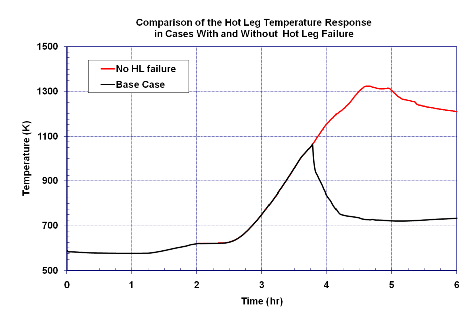
Figure 5-87 The hot leg temperature response in the thermally-induced steam generator tube rupture cases with and without hot leg failure
