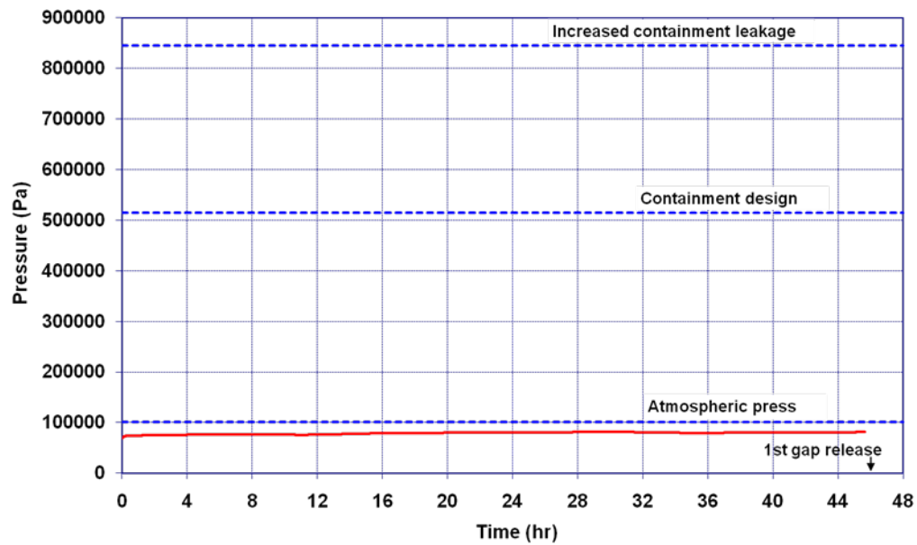
Figure 5-100 SGTR with Failed Operator Action-Containment Pressure
