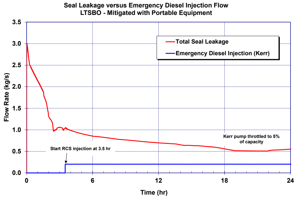
Figure 5-15 Mitigated LTSBO vessel emergency make up and pump seal leakage flows
