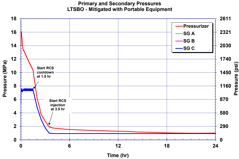
Figure 5-10 Mitigated long-term station blackout primary and secondary pressure history
