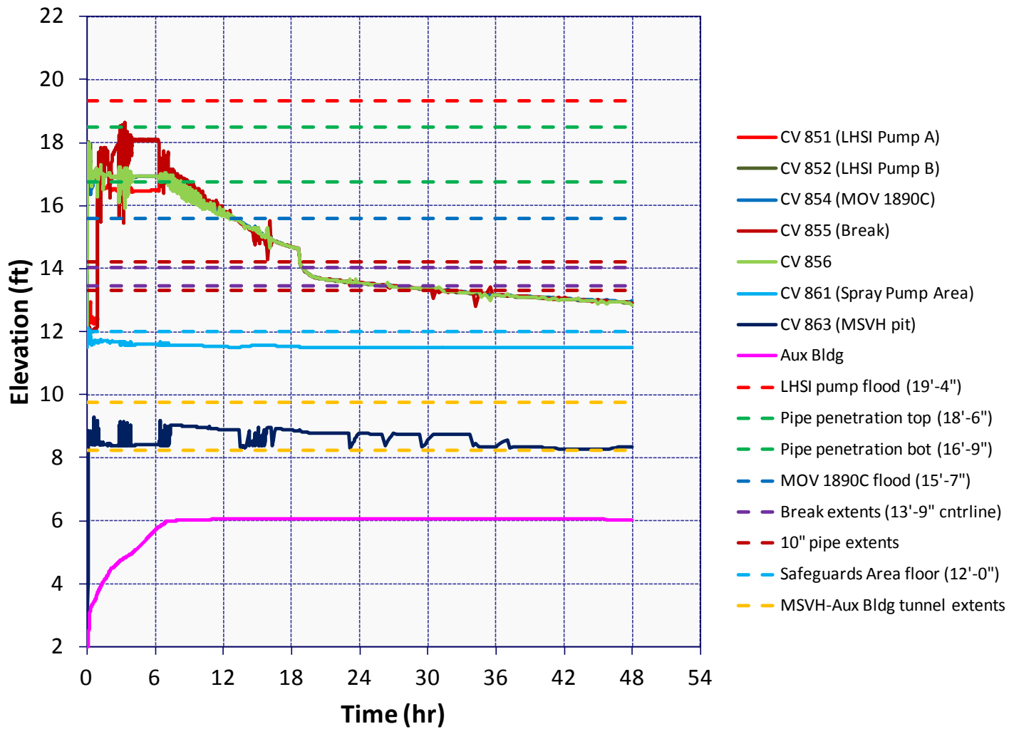
Figure 5-122 ISLOCA Safeguards Level Long Term
