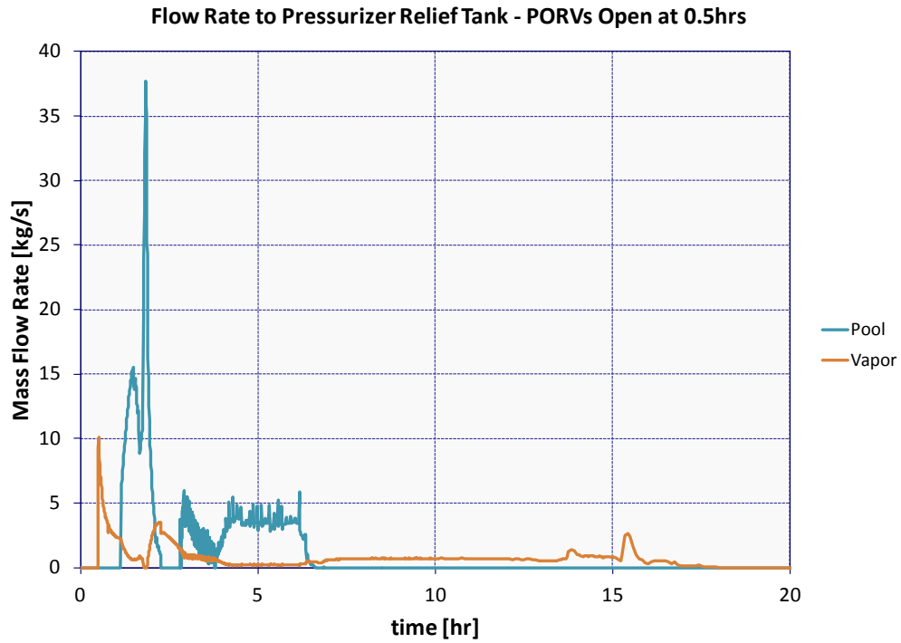
Figure 5-152 Flow Rate to Pressurizer Relief Tank – PORVs Open at 0.5 hrs
