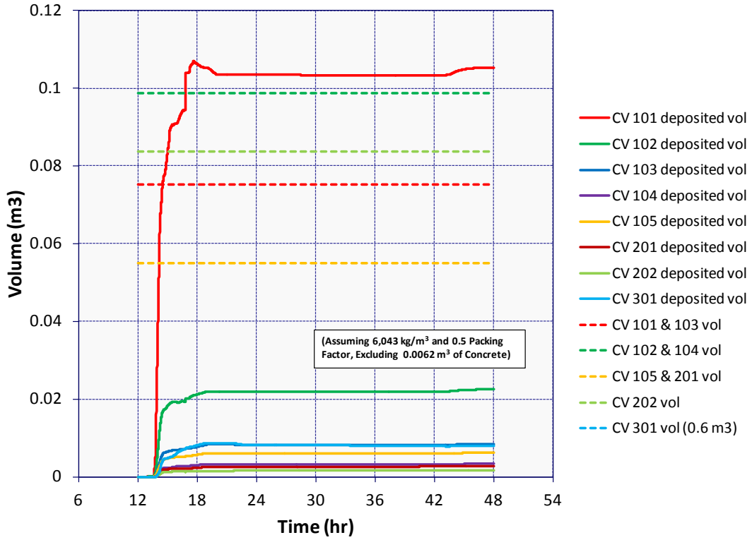
Figure 5-144 Captured Particulate Volume versus Pipe Volume in ISLOCA Deposition Calculation
