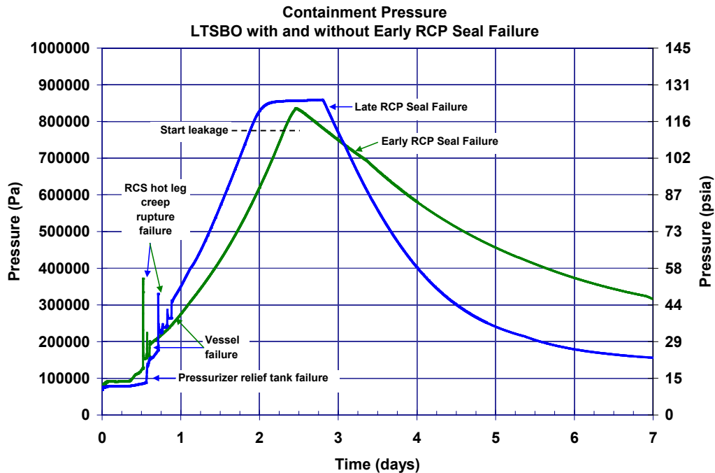
Figure 5-19 Comparison of the unmitigated long-term station blackout containment pressure responses with and without early RCP seal failures
