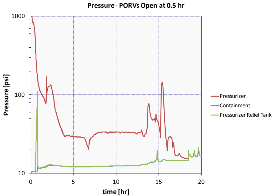
Figure 5-150 Facility pressure response to PORV actuation at 0.5hrs
