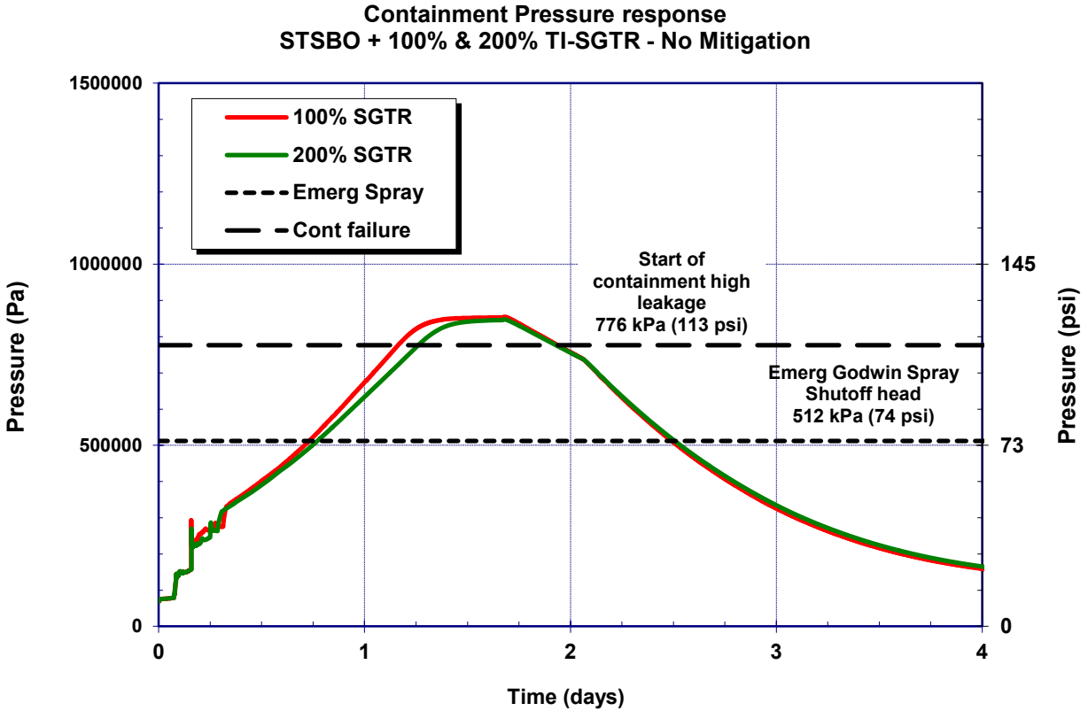
Figure 5-68 Unmitigated 100% and 200% TI-SGTR short-term station blackout containment pressure histories
