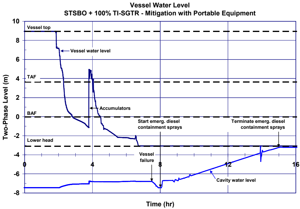
Figure 5-79 The mitigated short-term station blackout vessel two-phase coolant level
