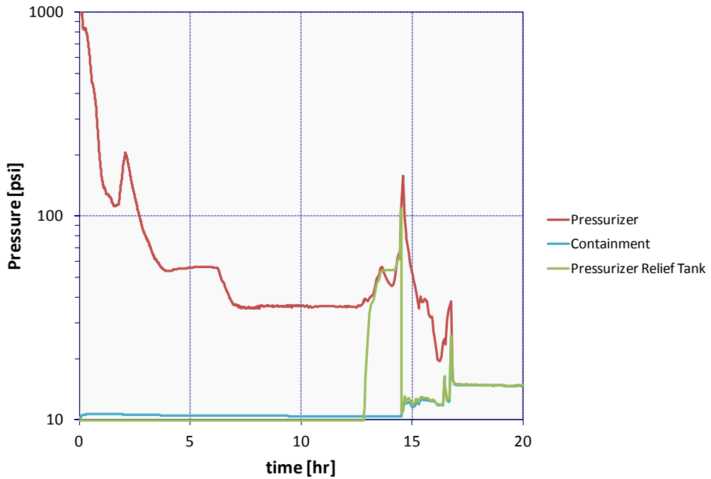
Figure 5-156 Facility pressure response to PORV actuation at Core Degradation
