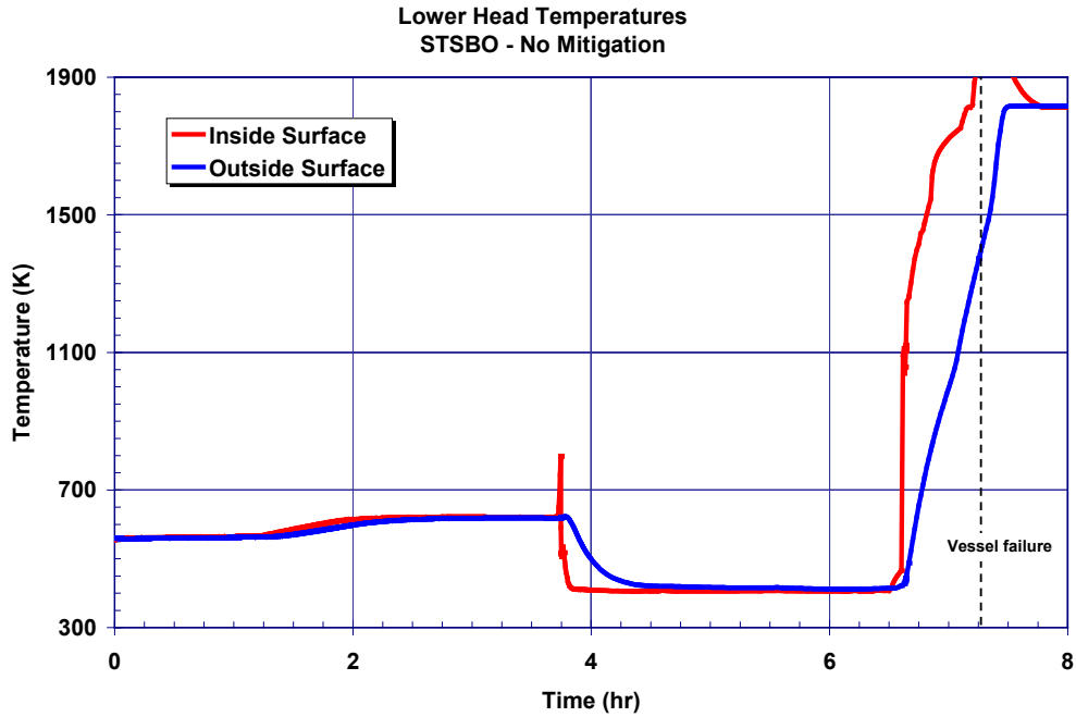
Figure 5-32 Unmitigated STSBO lower head inner and outer temperature history
