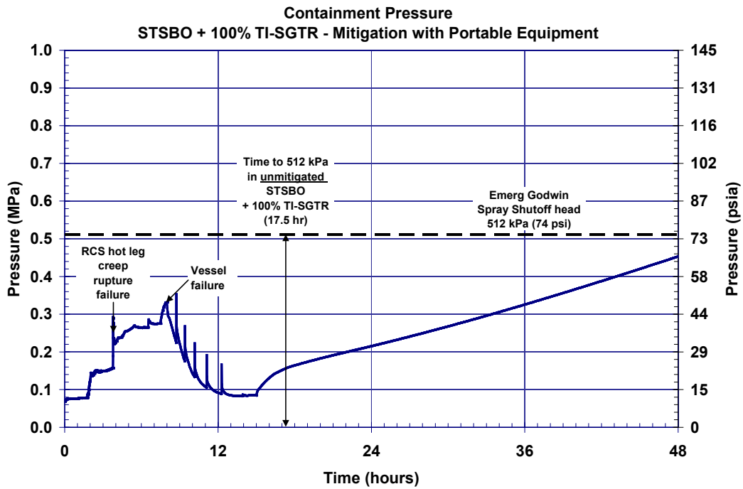
Figure 5-80 The mitigated short-term station blackout containment pressure history
