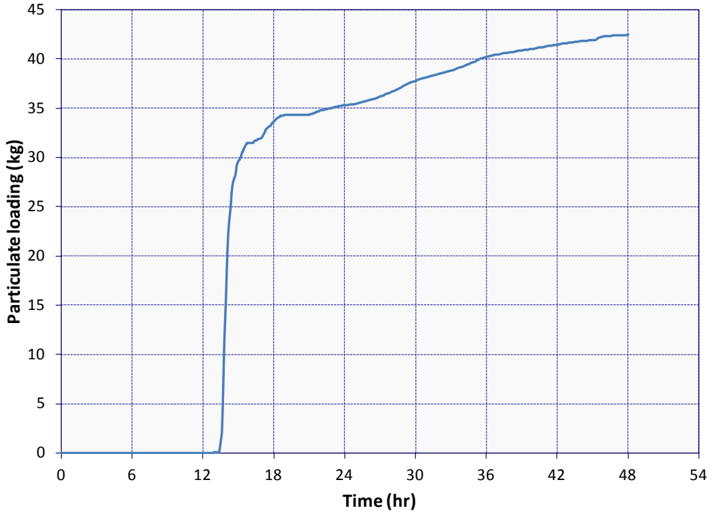
Figure 5-127 ISLOCA Safeguards Exhaust Ventilation Filter Aerosol Loading
