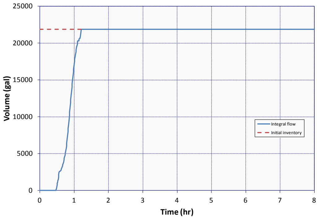
Figure 5-112 ISLOCA Integral Accumulator Flow
