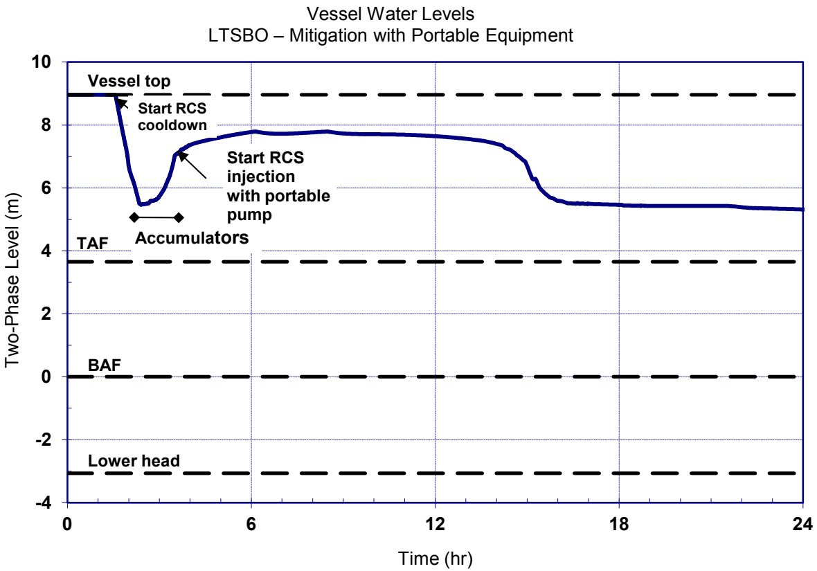
Figure 5-11 Mitigated long-term station blackout vessel two-phase coolant level
