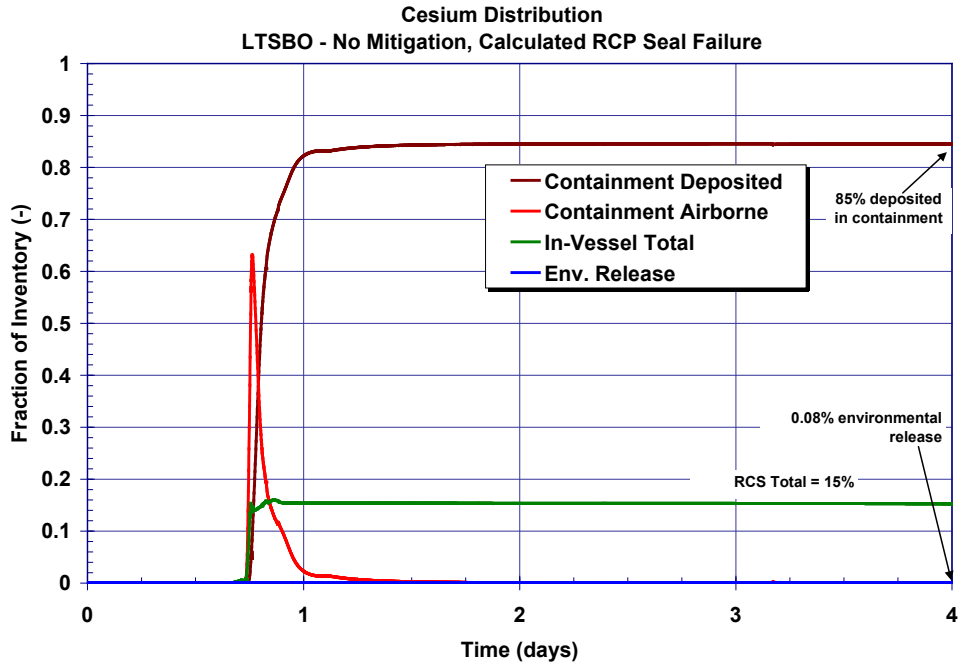
Figure 5-8 Unmitigated LTSBO cesium fission product distribution history
