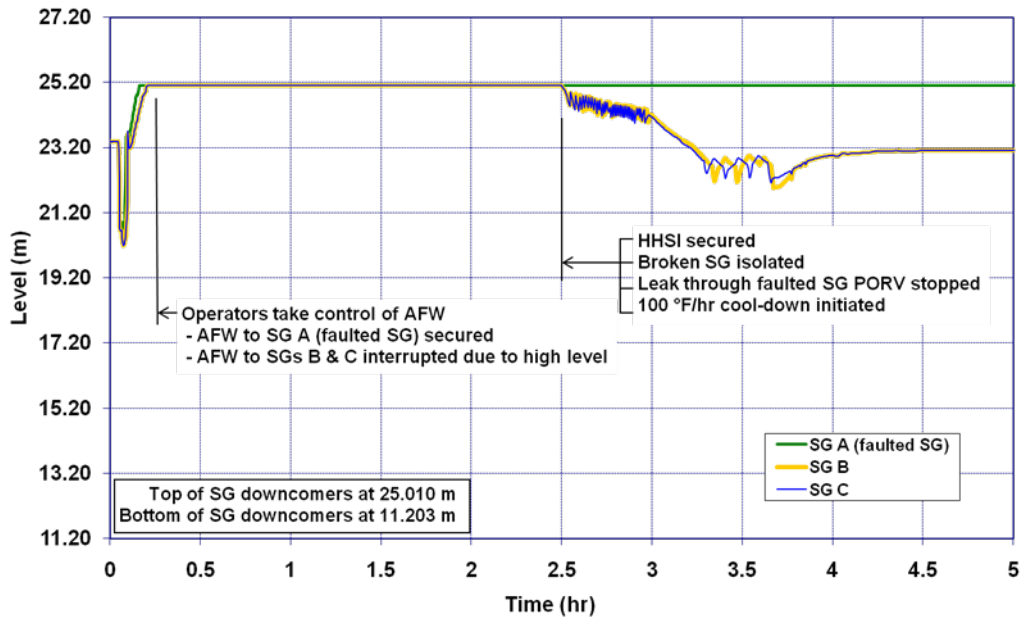
Figure 5-95 SGTR with Operator Action- Steam Generator Level
