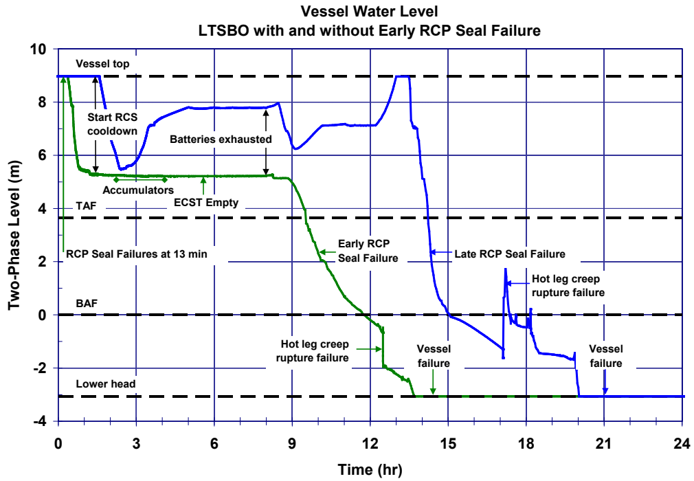
Figure 5-18 Comparison of the unmitigated long-term station blackout vessel level responses with and without early RCP seal failures
