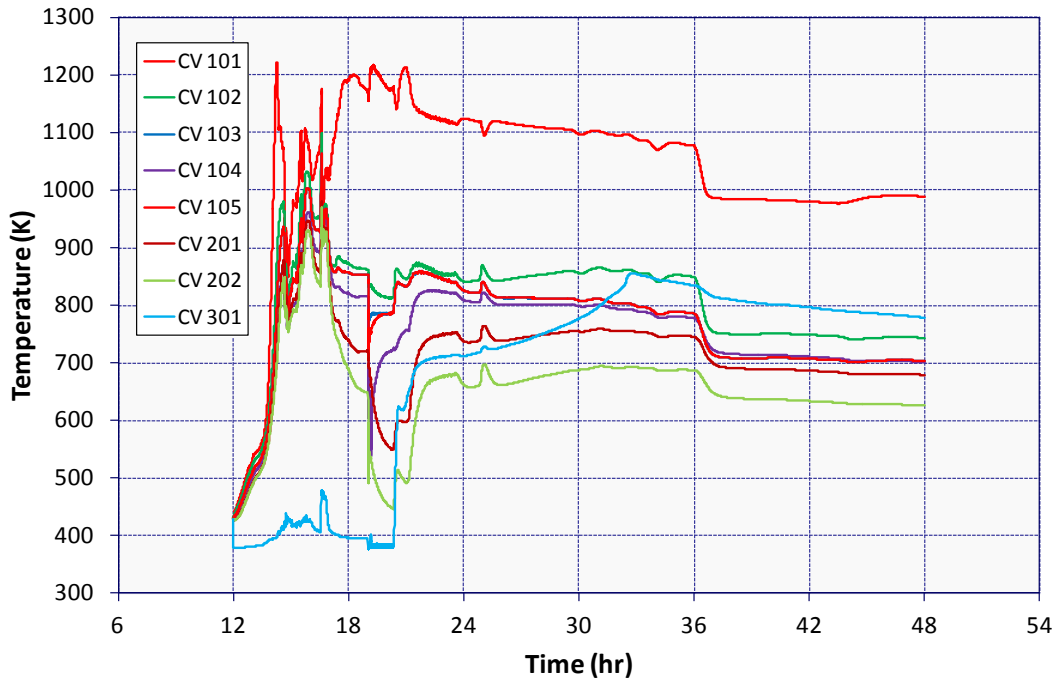
Figure 5-137 Pipe Wall Inside Surface Temperature Along LHSI Piping in ISLOCA Deposition Calculation
