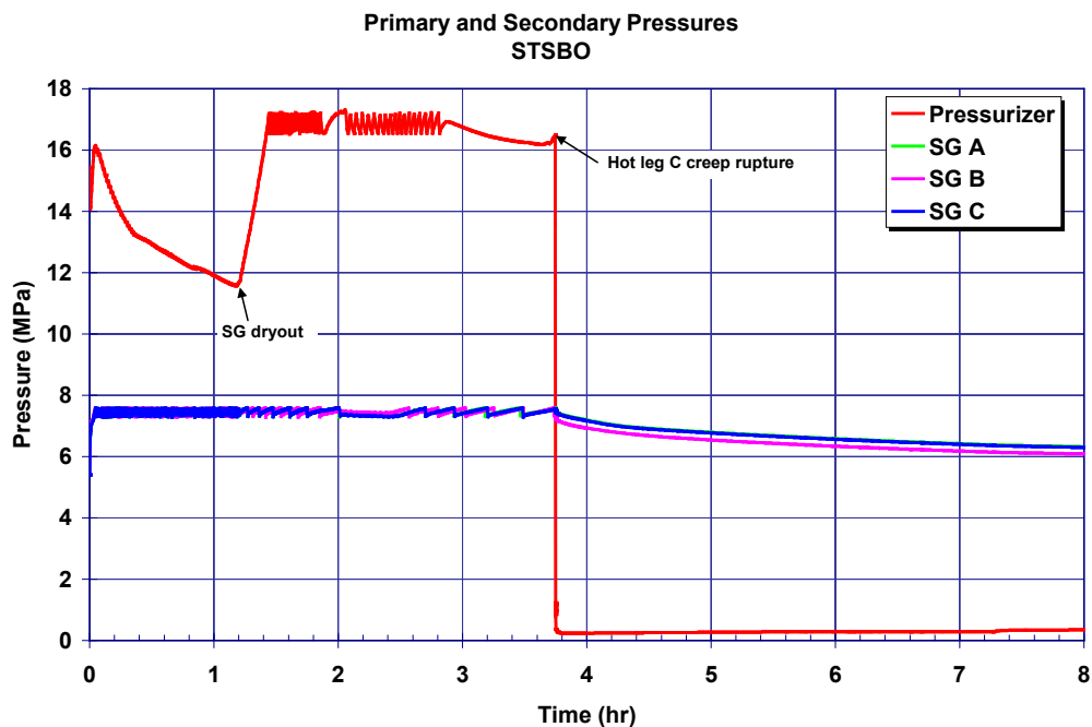
Figure 5-39 Mitigated STSBO primary and secondary pressure history
