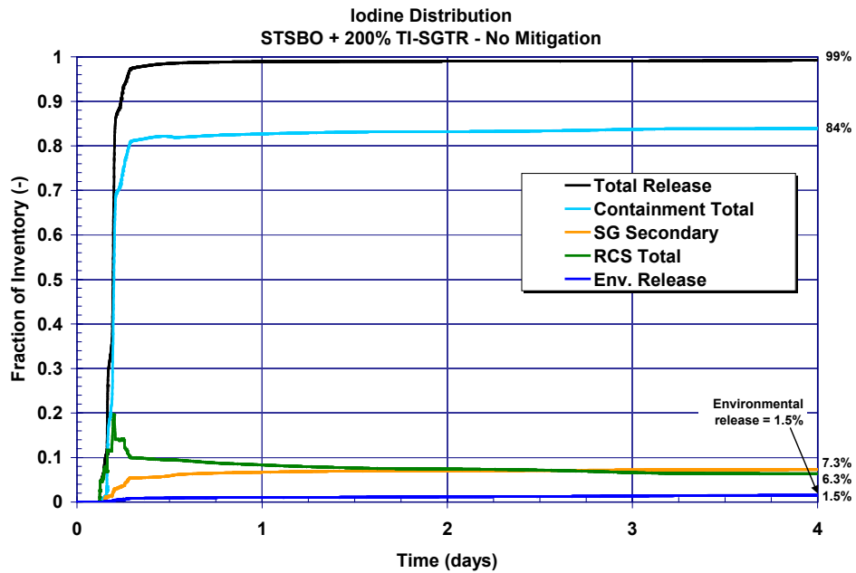
Figure 5-71 The unmitigated 200% TI-SGTR short-term station blackout iodine fission product distribution history
