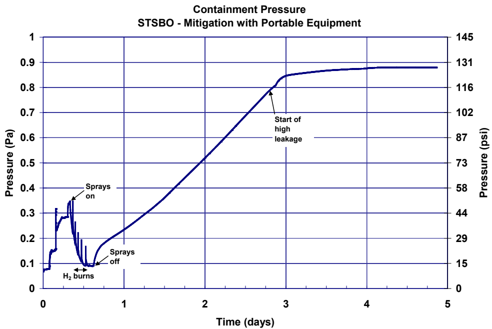
Figure 5-43 Mitigated short-term station blackout containment pressure history
