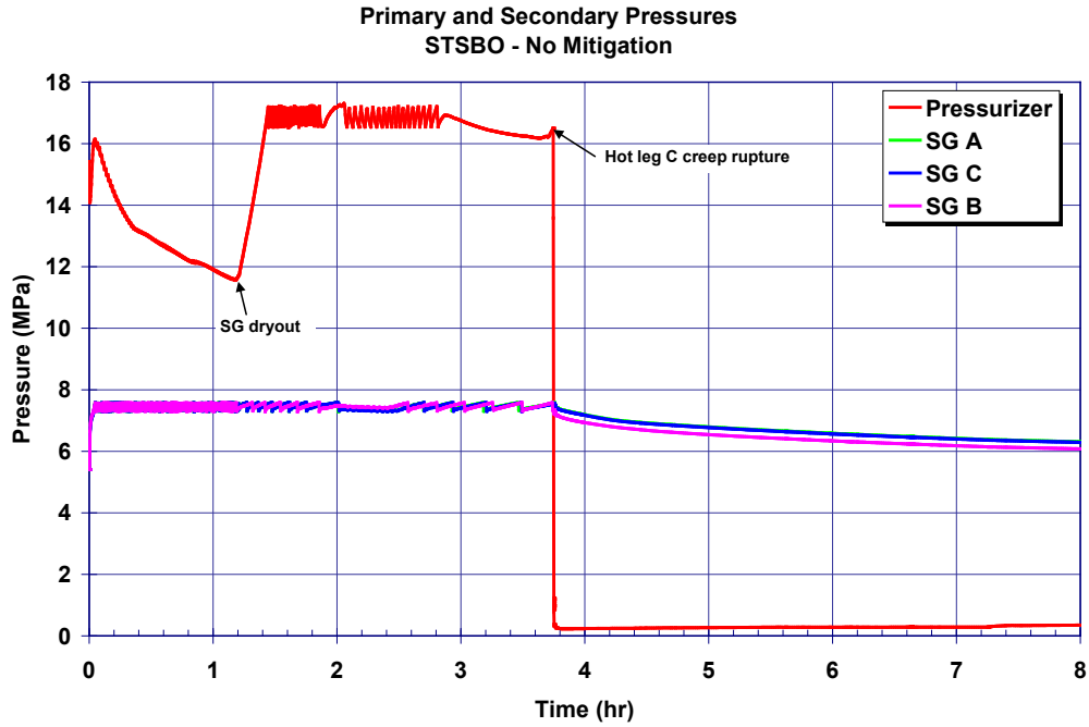
Figure 5-28 Unmitigated STSBO primary and secondary pressures history
