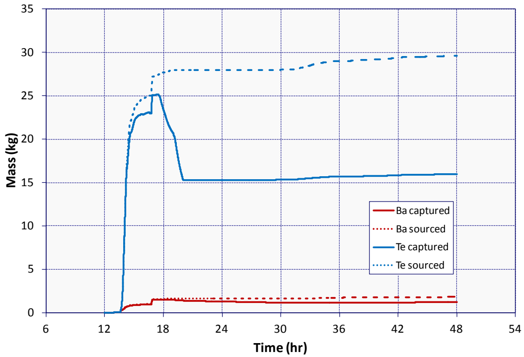
Figure 5-140 LHSI Piping Ba and Te Capture in ISLOCA Deposition Calculation
