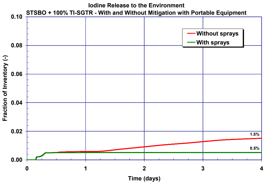
Figure 5-84 The short-term station blackout with a 100% thermally-induced SGTR with and without spray mitigation iodine environmental release
