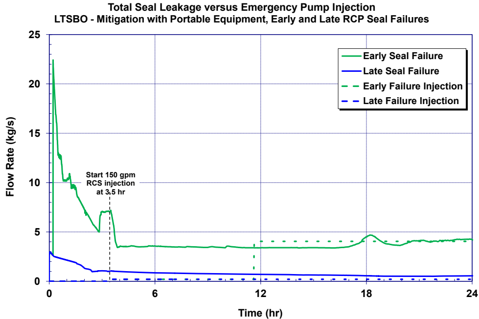
Figure 5-27 Comparison of the mitigated long-term station blackout portable pump injection rates with and without early RCP seal failures
