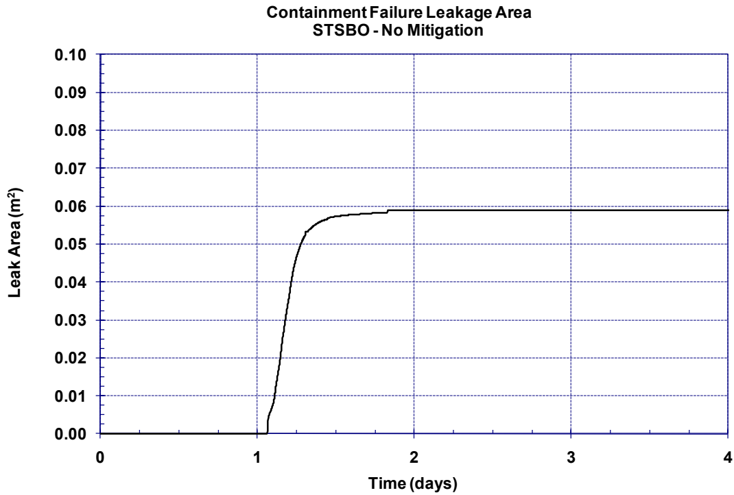
Figure 5-31 Unmitigated STSBO containment leakage area
