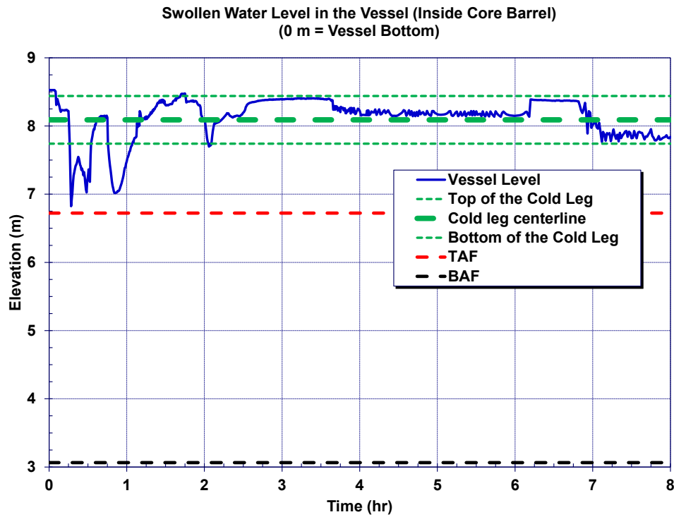
Figure 5-146 ISLOCA Vessel Swollen Water Level for the Unmitigated ISLOCA
