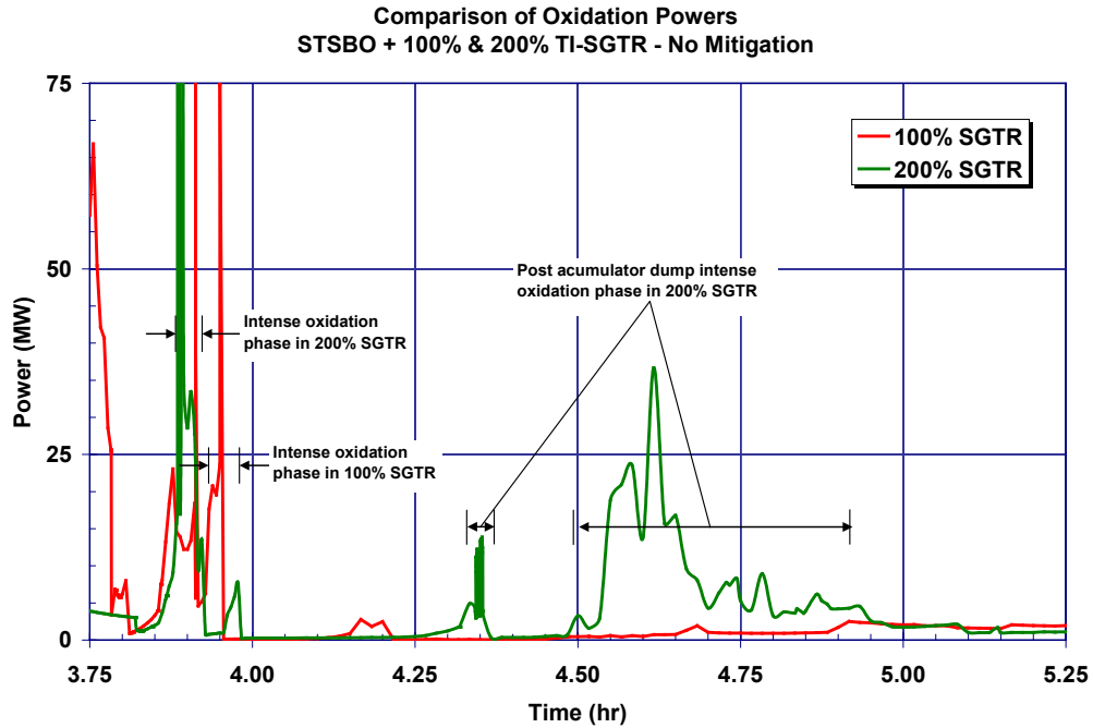
Figure 5-66 Unmitigated 100% and 200% TI-SGTR short-term station blackout fuel oxidation power after the RCS hot leg failure
