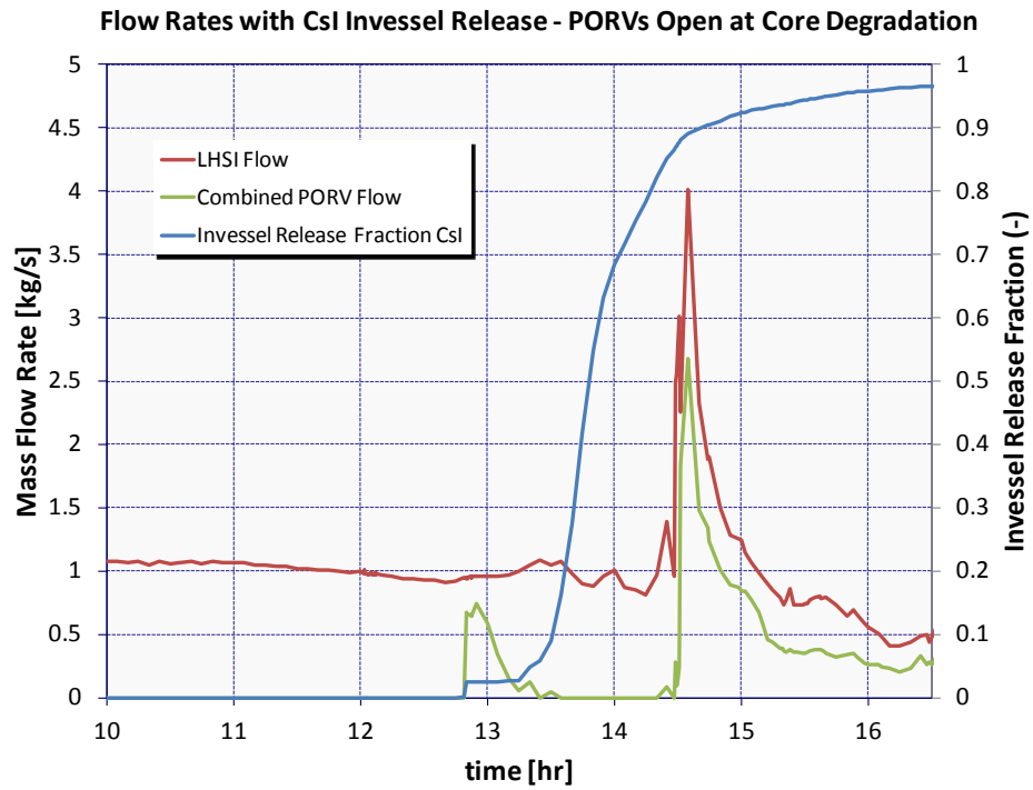
Figure 5-157 Flow Rates with CsI Invesel Release – PORVs Open at Core Degradation
