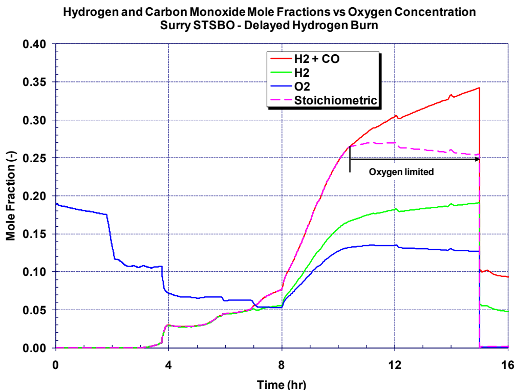
Figure 5-53 Mitigated short-term station blackout containment dome gas concentrations versus stoichiometric
