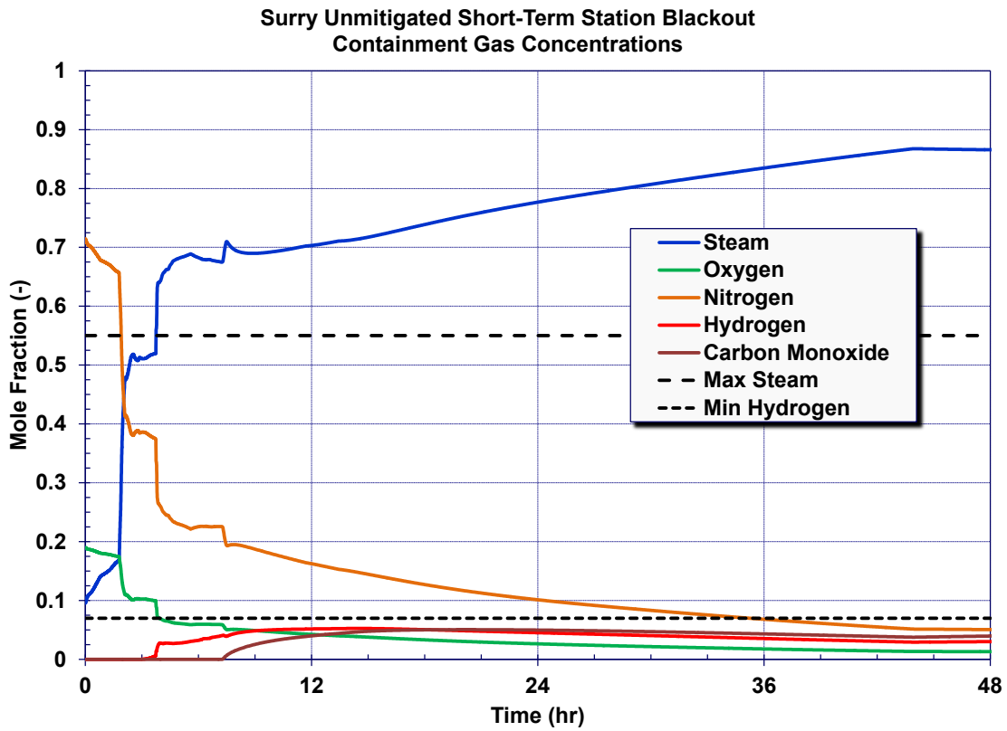
Figure 5-35 Unmitigated short-term station blackout containment gas concentrations
