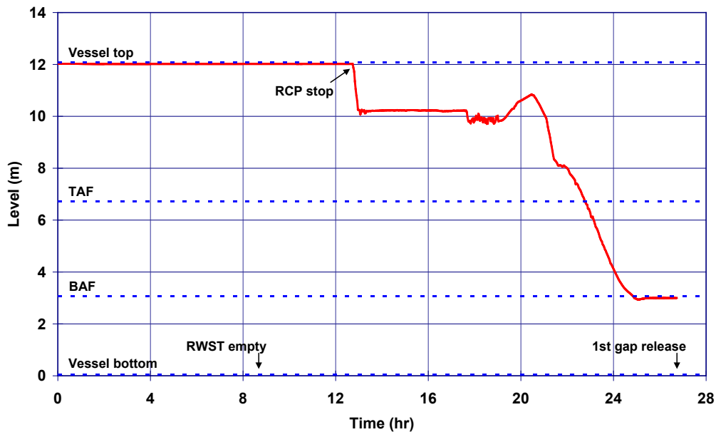
Figure 5-103 SGTR with Failed Operator Action and SORV – RPV Water Level
