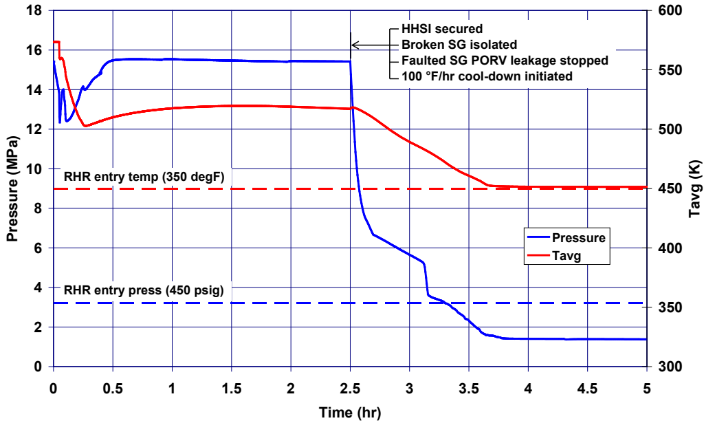
Figure 5-90 SGTR with Operator Action – RCS Conditions Relative to RHR Entry Conditions
