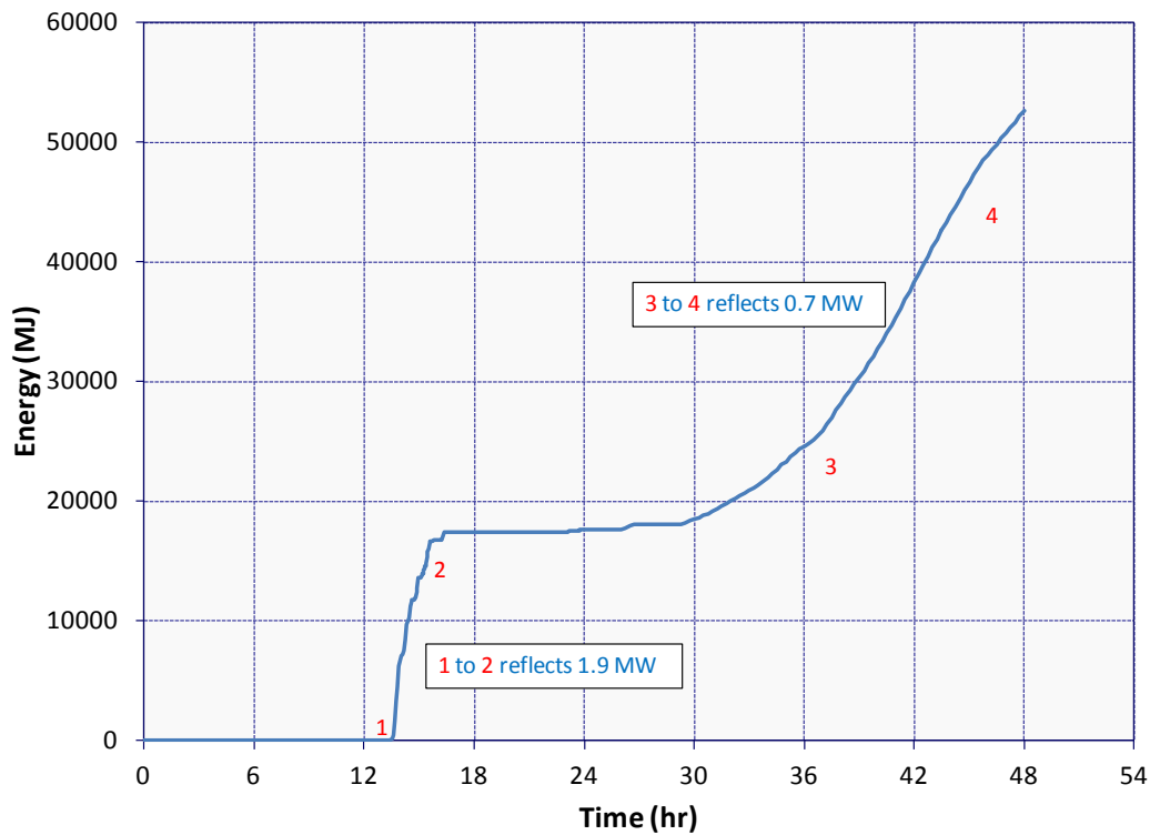
Figure 5-124 ISLOCA Energy Release from H 2 and CO Burns in Safeguards Area
