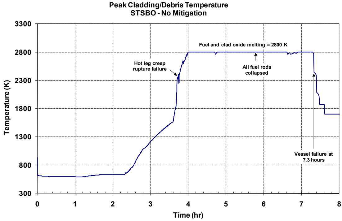
Figure 5-30 Unmitigated STSBO core temperature history
