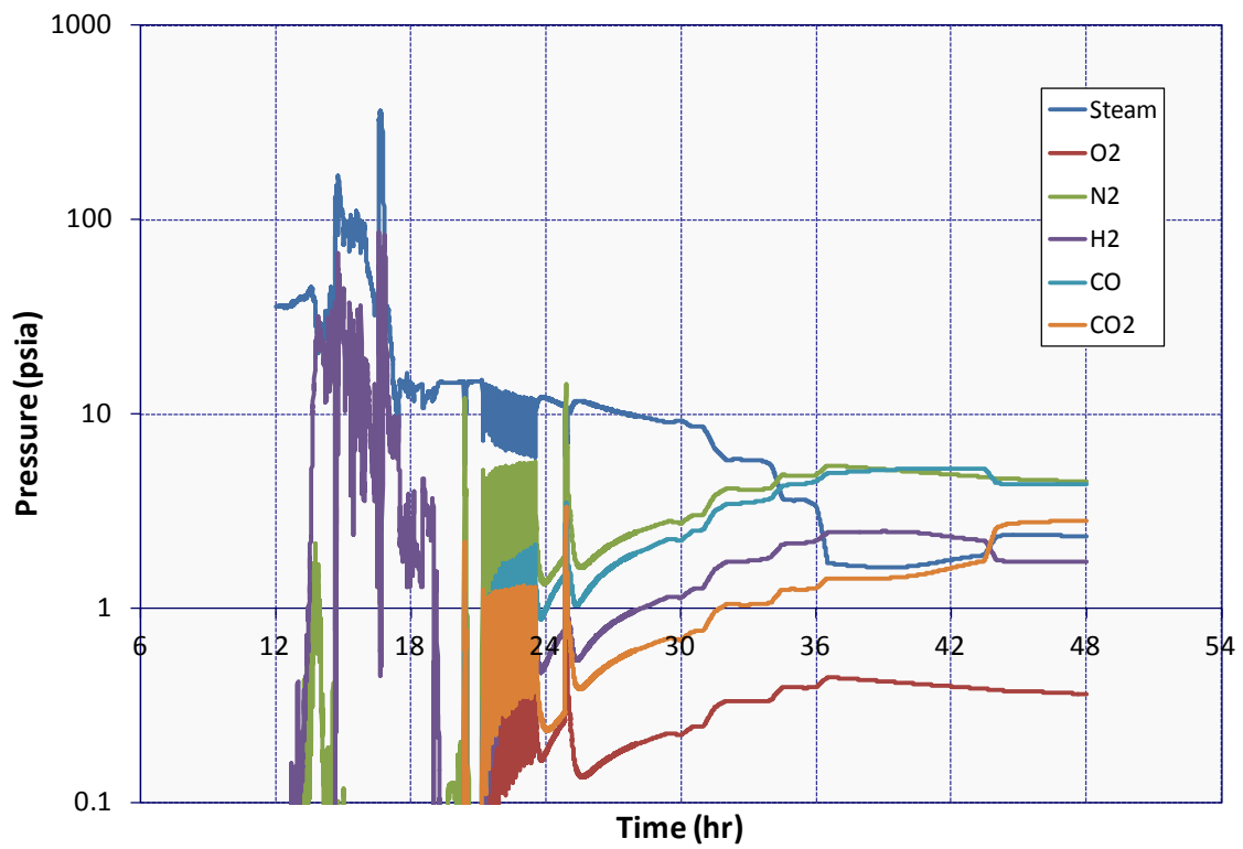
Figure 4-18 Cold Leg Partial Pressure Imposed on ISLOCA Deposition Calculati
