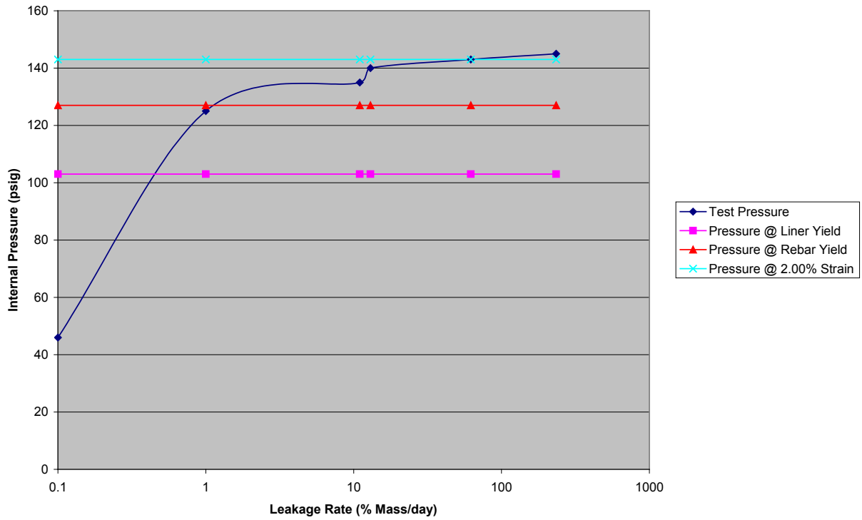
1:6 Scale Containment Reinforced Concrete Containment Test Pressure Vs. Leakage Rate
