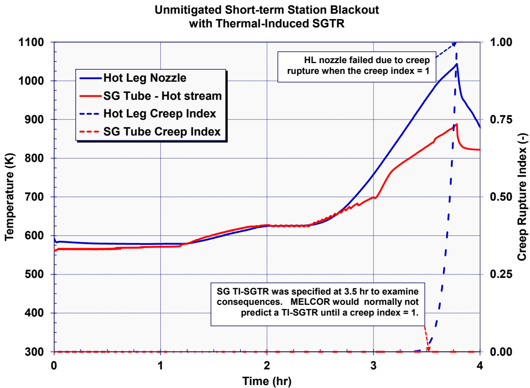
Figure 5-61 Comparison of the hot leg nozzle and steam generator tube structure temperatures and creep rupture indices for the STSBO with TI-SGTR
