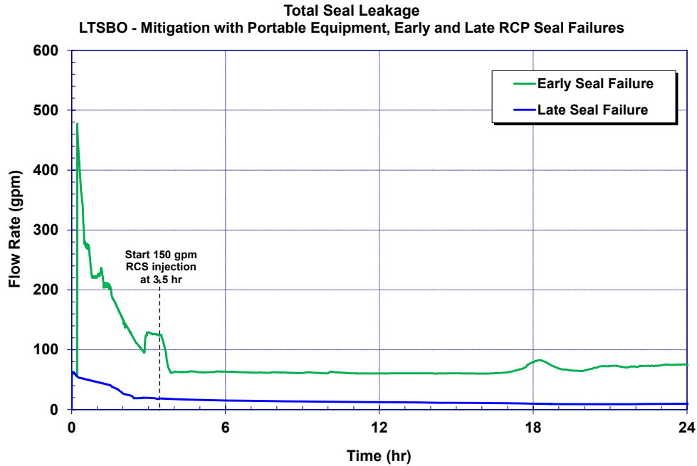
Figure 5-25 Comparison of the mitigated long-term station blackout RCP seal leakages with and without early RCP seal failures
