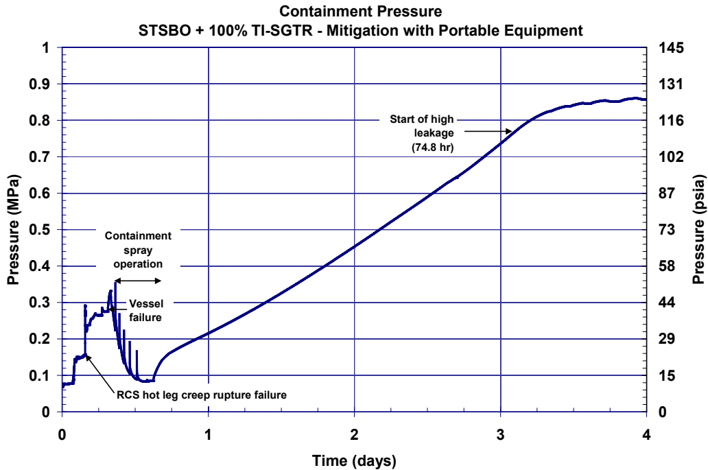
Figure 5-81 The mitigated short-term station blackout containment pressure history
