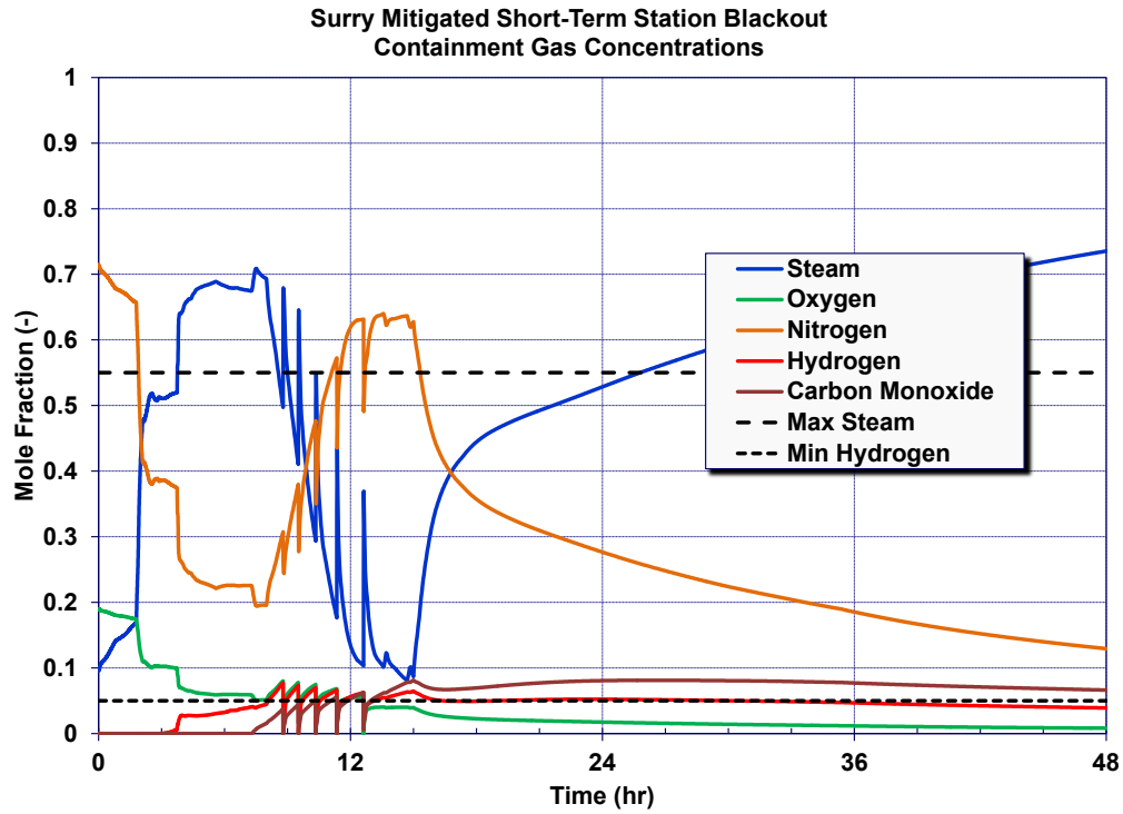
Figure 5-44 Mitigated short-term station blackout containment gas concentrations
