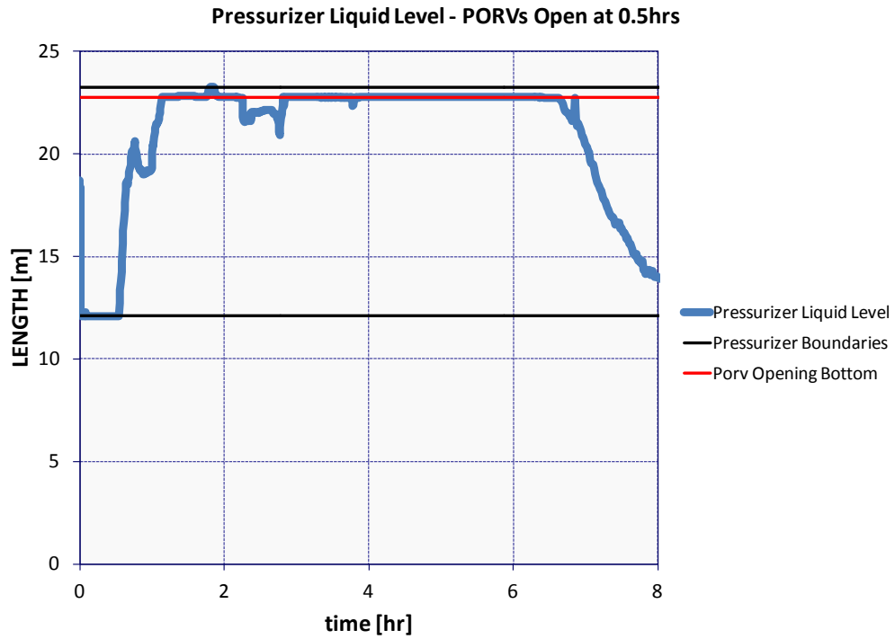
Figure 5-151 Pressurizer liquid level response to PORV actuation at 0.5hrs
