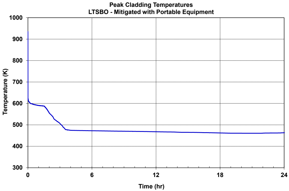
Figure 5-12 Mitigated long-term station blackout core temperature history
