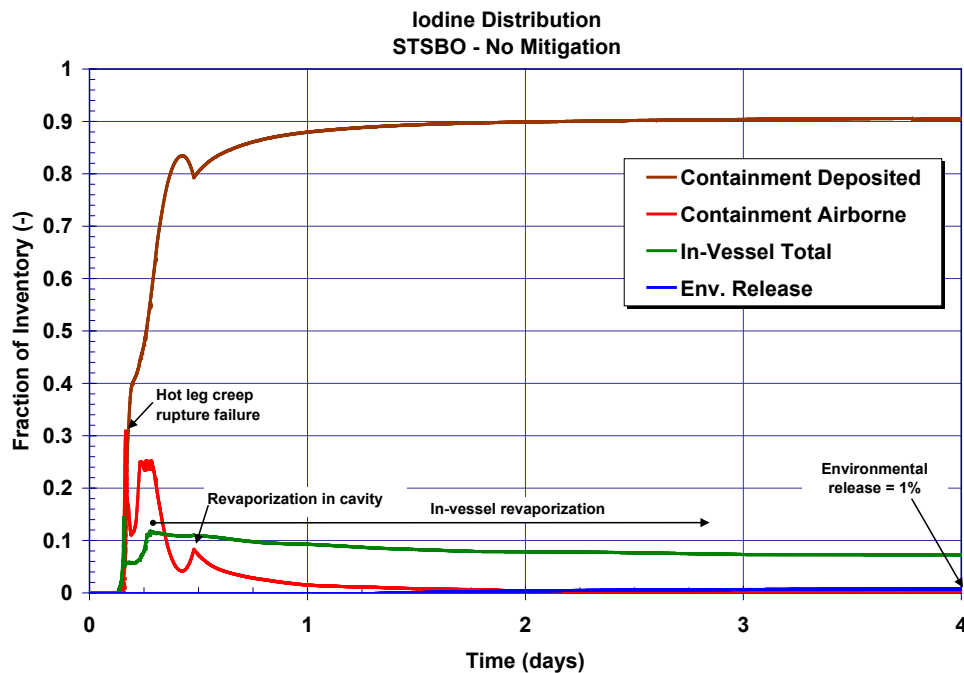
Figure 5-36 Unmitigated STSBO iodine fission product distribution history 23
