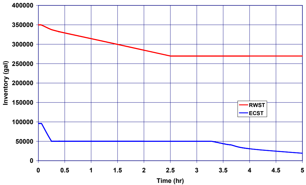
Figure 5-93 SGTR with Operator Action – RWST and ECST Inventories
