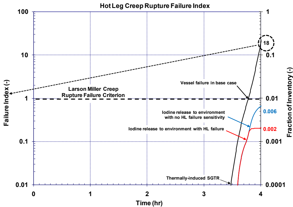
Figure 5-88 The hot leg creep rupture failure index and iodine release to environment for the thermally-induced SGTR cases with and without hot leg failure
