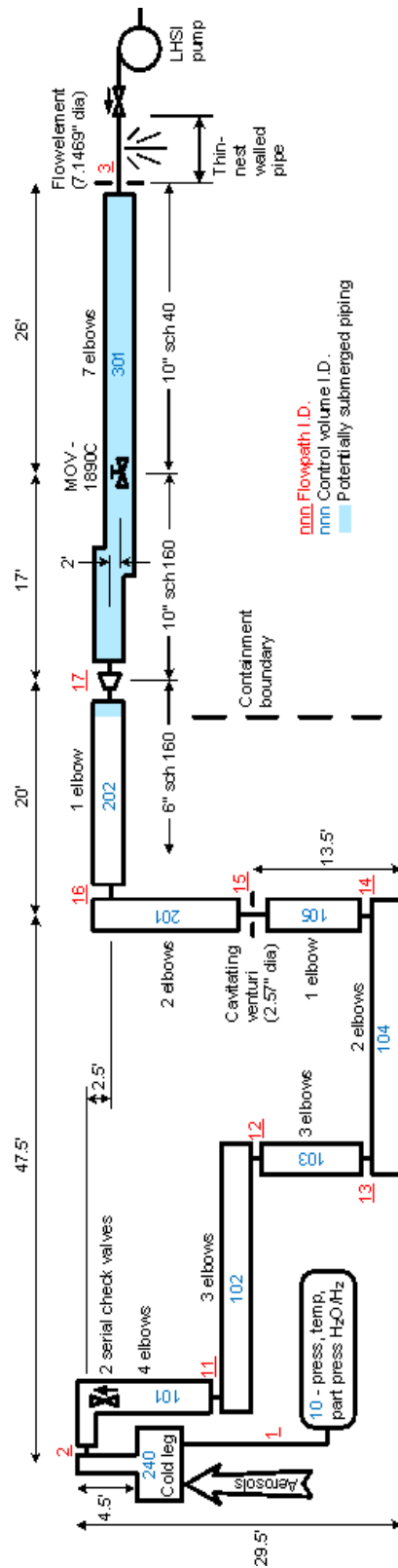
Figure 4-15 Low Head Safety Injection Piping MELCOR Nodalization
