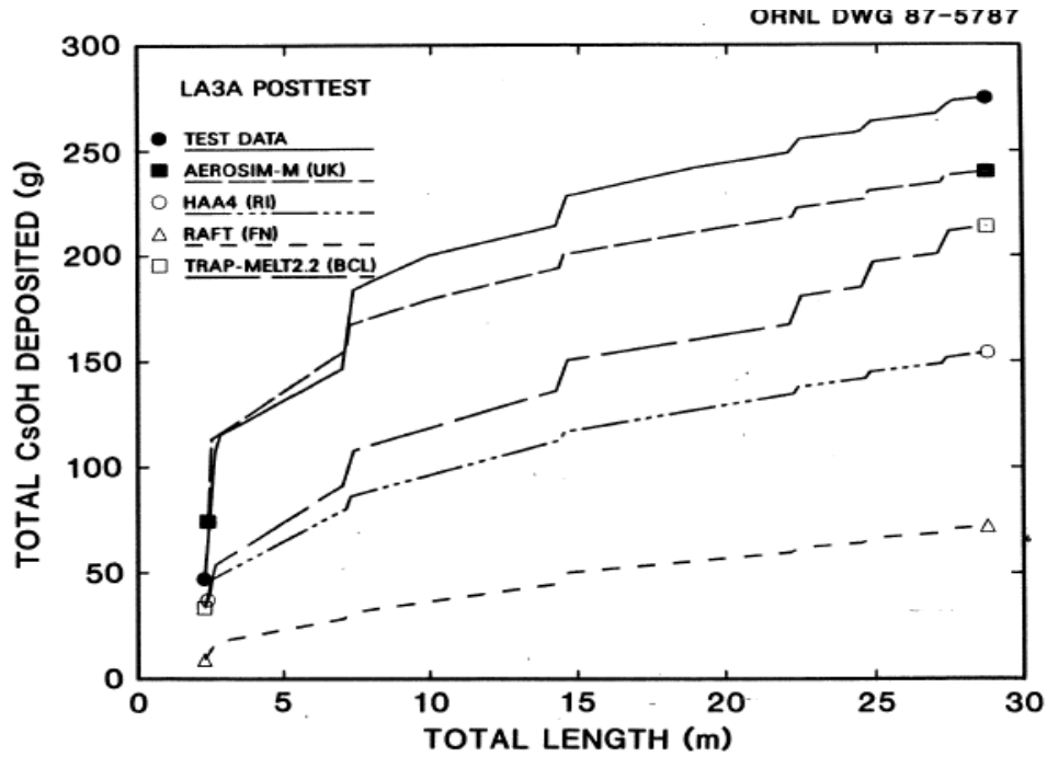
Figure D-38 LA3A post test calculation of CsOH aerosol deposition for codes including bend deposition models (LACE TR-024)
