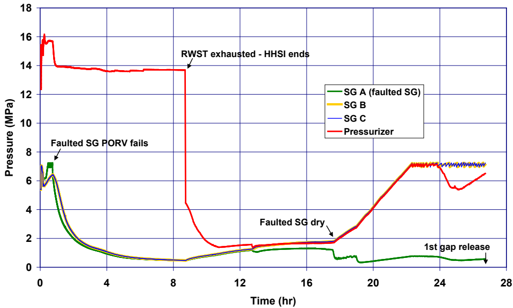
Figure 5-102 SGTR with Failed Operator Action and SORV – System Pressures
