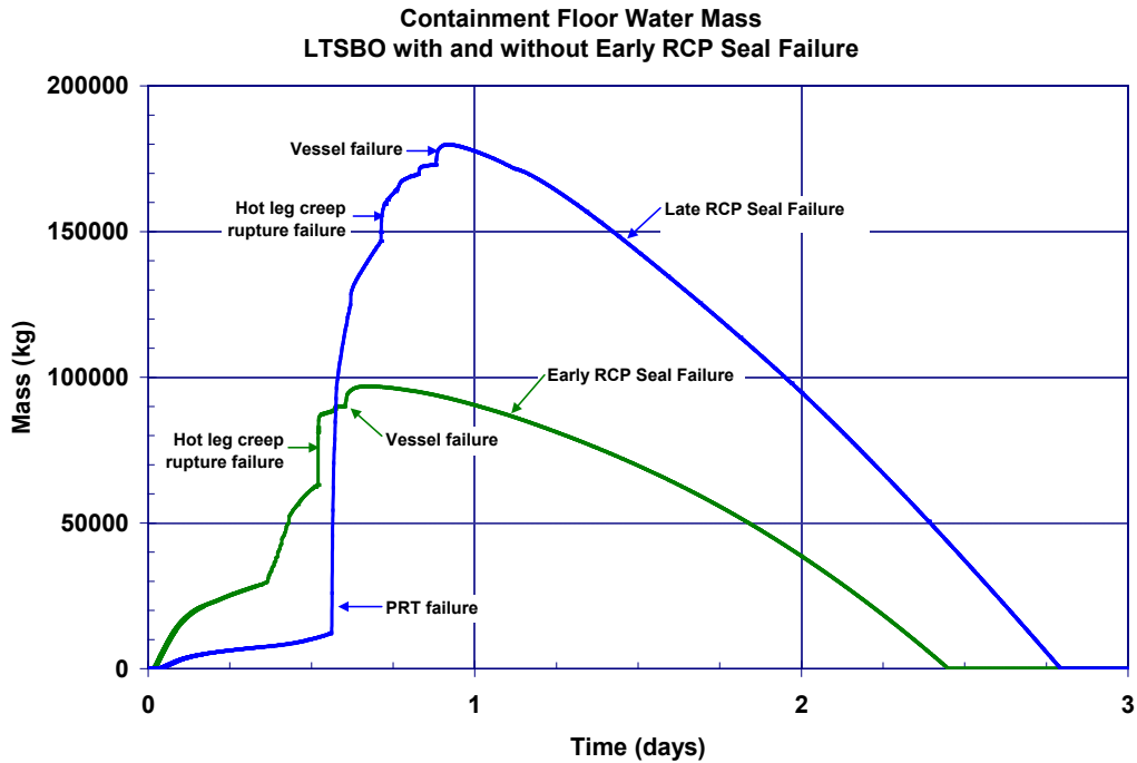
Figure 5-20 Comparison of the unmitigated long-term station blackout containment water pool masses with and without early RCP seal failures
