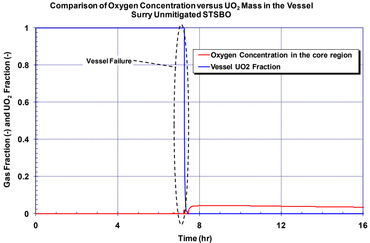
Figure 5-167 Comparison of the oxygen concentration and UO 2 mass in the vessel during the unmitigated STSBO
