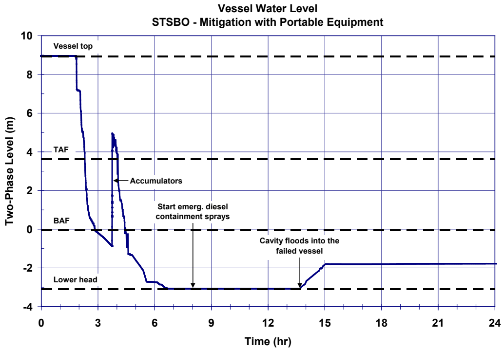
Figure 5-40 Mitigated short-term station blackout vessel two-phase coolant level
