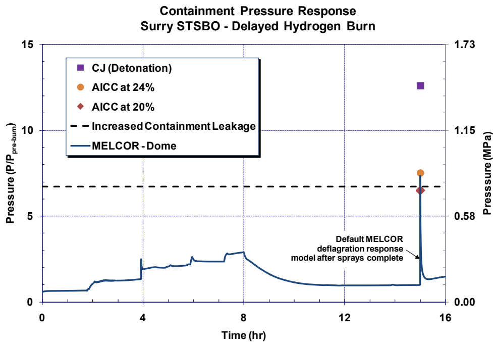
Figure 5-58 Mitigated short-term station blackout containment pressure history for the sensitivity calculation with delayed ignition
