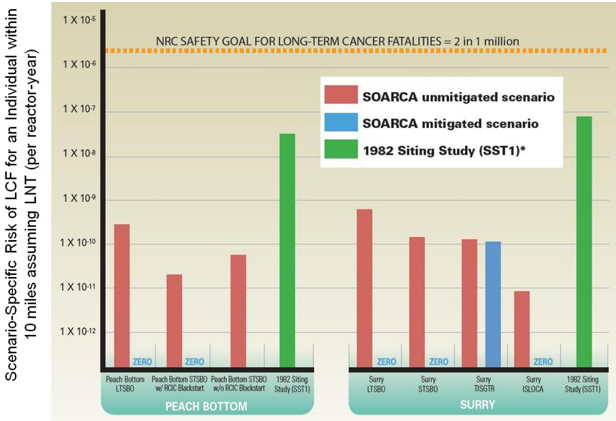
Figure ES-3 Comparison of individual LCF risk results for SOARCA mitigated and unmitigated scenarios to the NRC Safety Goal and to extrapolations of the 1982 Siting Study SST1 (plotted on logarithmic scale)
