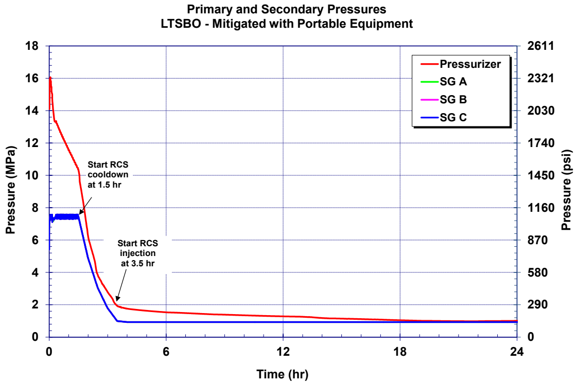
Figure 5-24 Primary and secondary pressure responses for the mitigated long-term station blackout with early RCP seal failure
