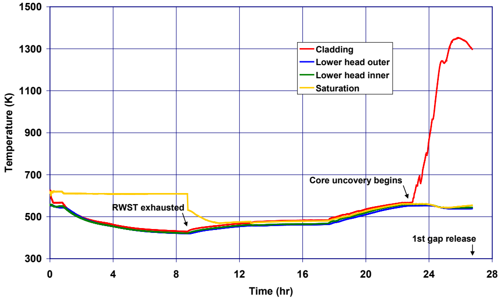
Figure 5-104 SGTR with Failed Operator Action and SORV – Max Clad and Lower Head Temperature
