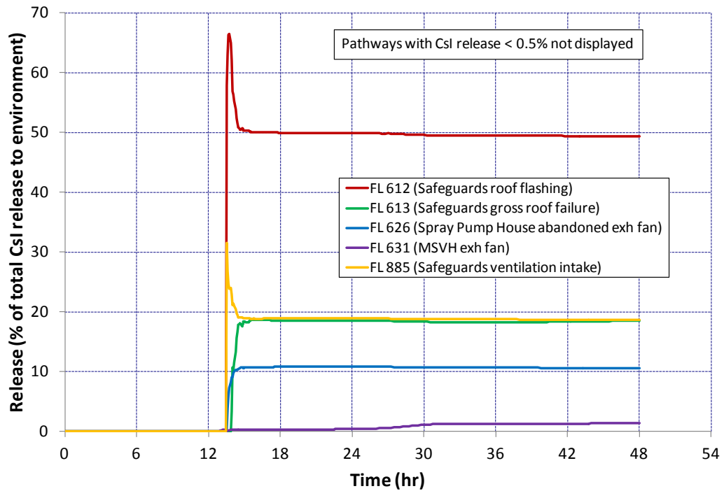
Figure 5-134 ISLOCA CsI Releases by Available Pathways (% of Instantaneous Total)
