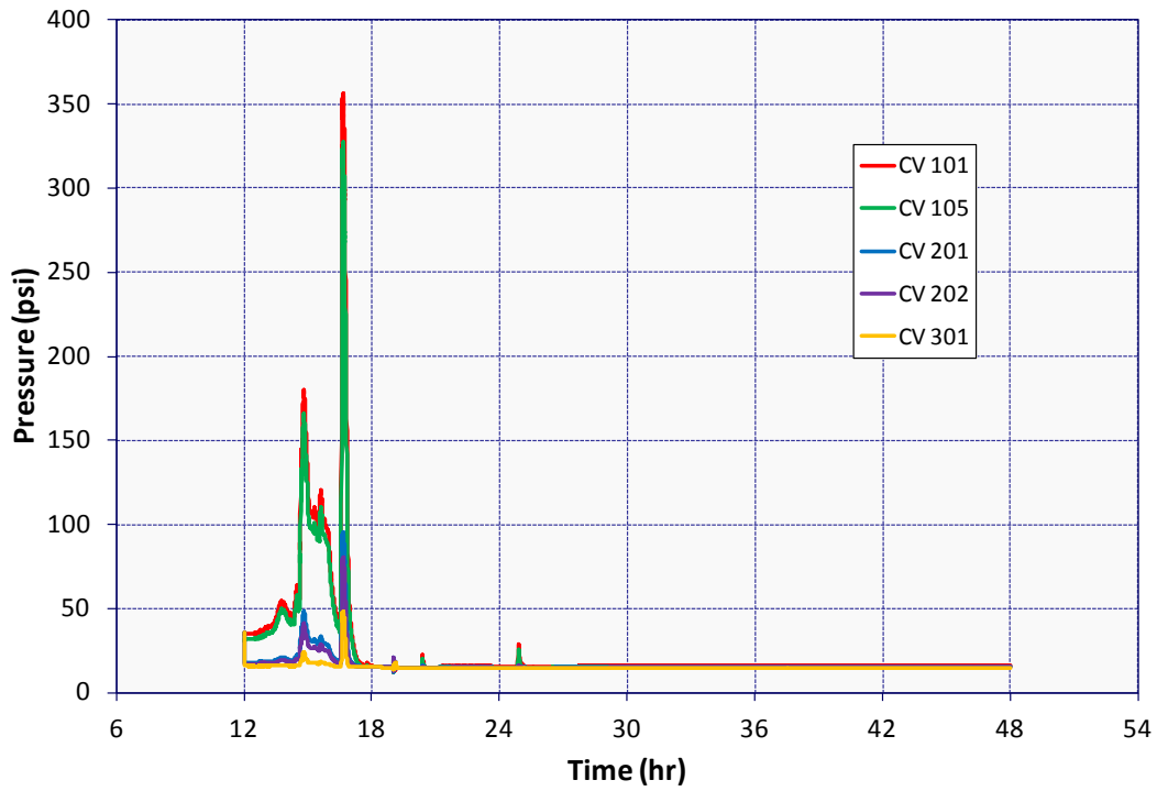
Figure 5-135 Pressure Along LHSI Piping in ISLOCA Deposition Calculation
