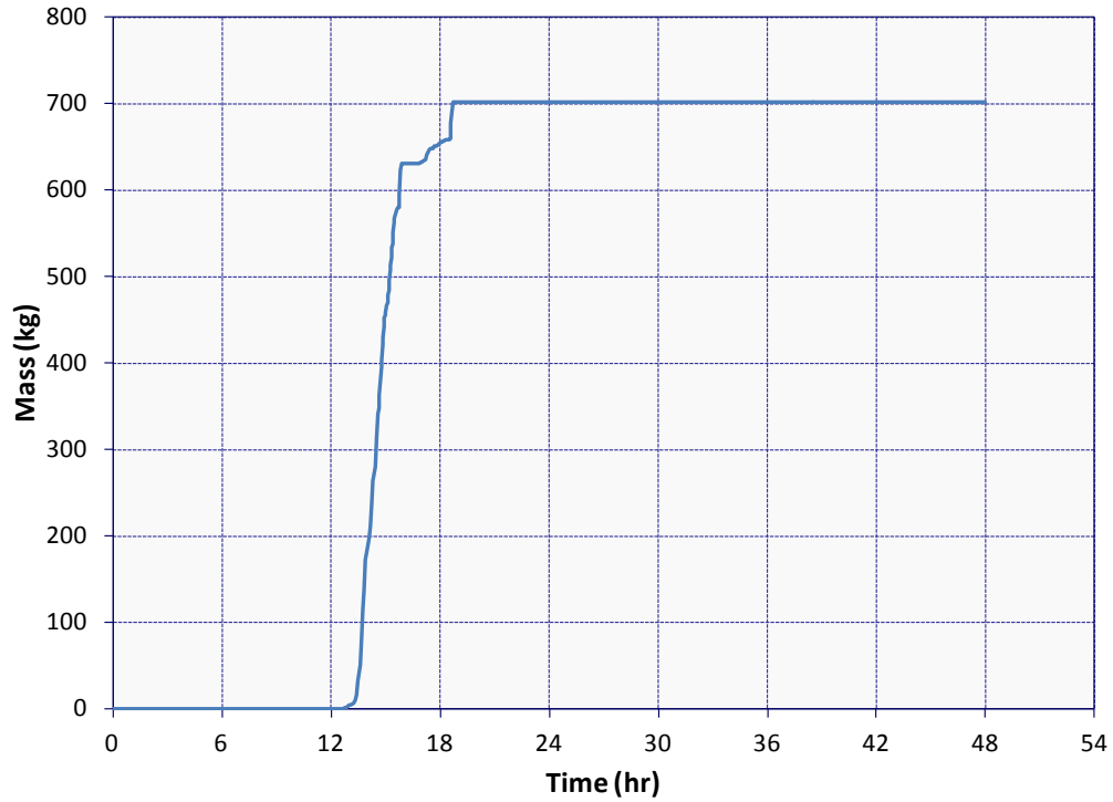
Figure 5-114 ISLOCA In-Vessel Hydrogen Production
