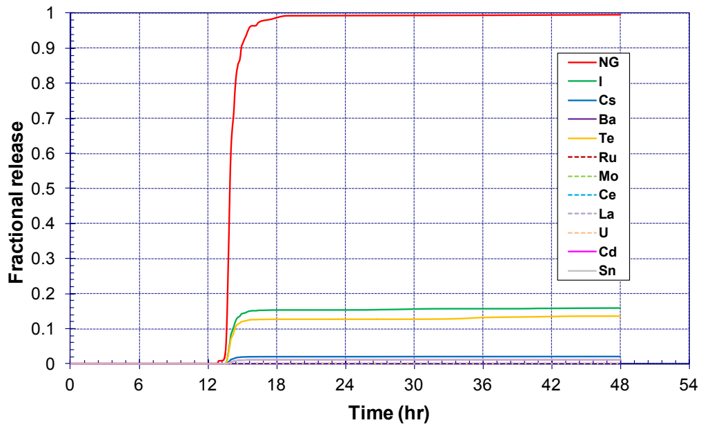
Figure 5-131 ISLOCA Fission Product Release to the Environment
