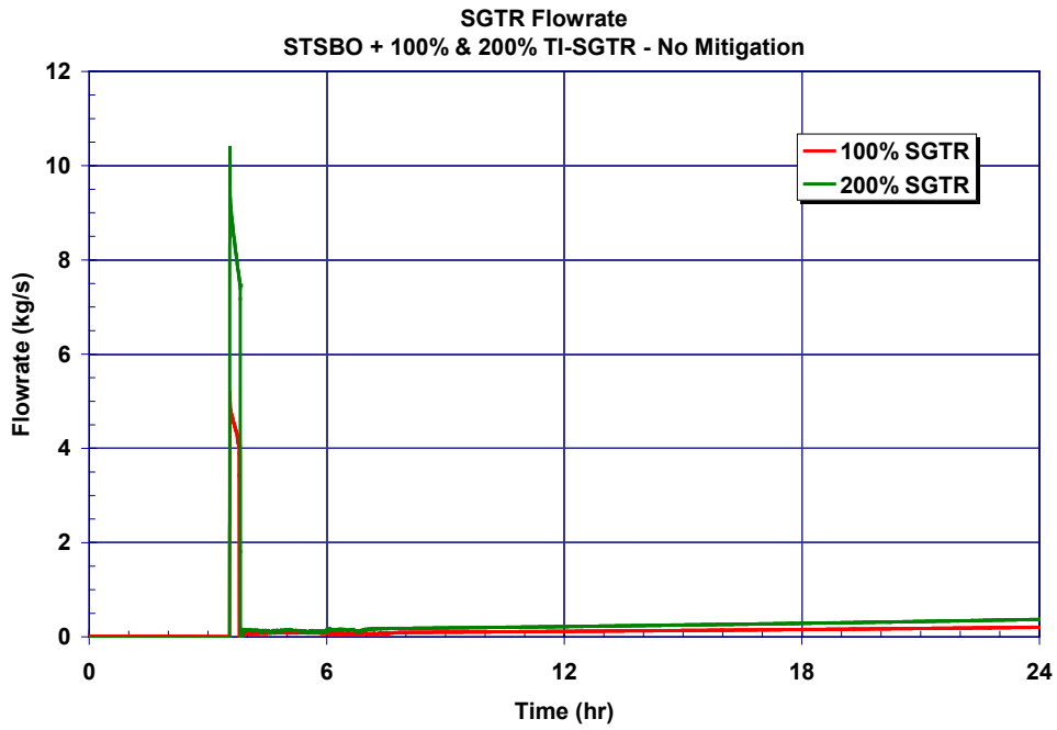
Figure 5-62 Unmitigated 100% and 200% TI-SGTR STSBO primary and TI-SGTR flowrate histories
