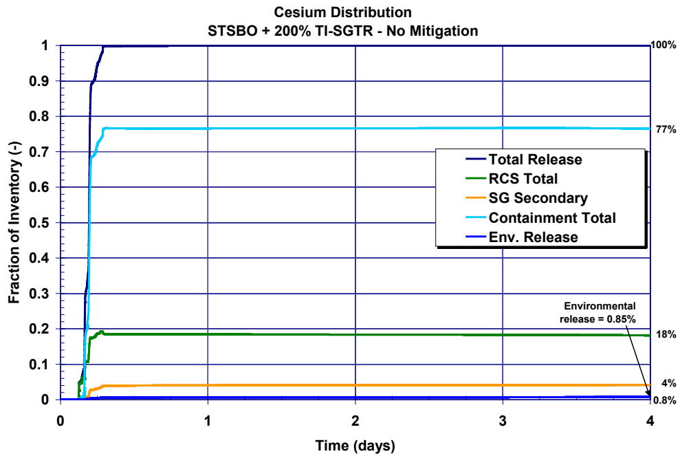
Figure 5-73 The unmitigated 200% TI-SGTR short-term station blackout cesium fission product distribution history
