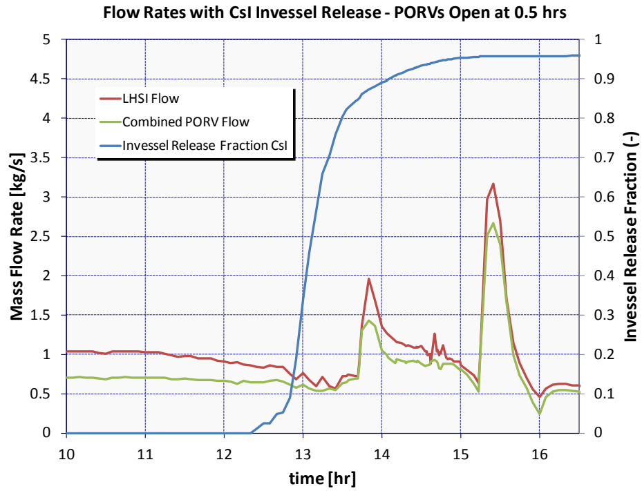
Figure 5-153 Flow Rates with Csl Invesel Release – PORVs Open at 0.5 hrs
