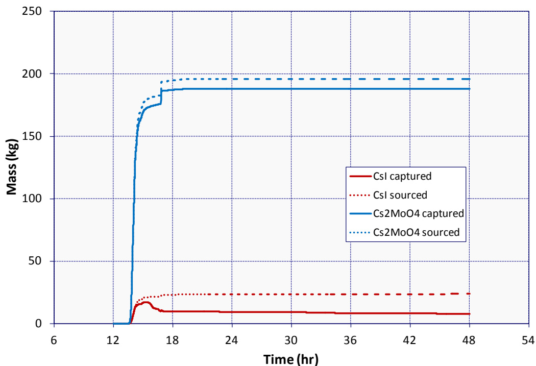
Figure 5-139 LHSI Piping CsI and Cs 2 MoO 4 Capture in ISLOCA Deposition Calculation
