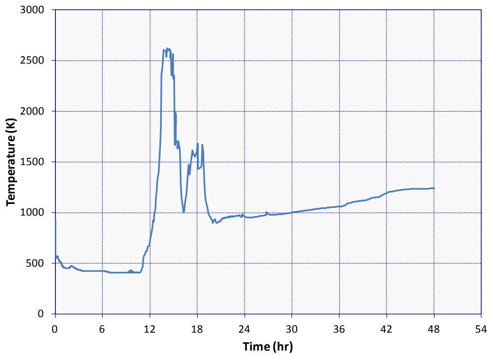
Figure 5-115 ISLOCA Maximum Core Temperature
