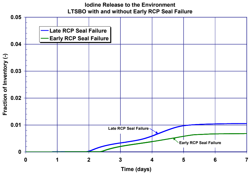
Figure 5-22 Comparison of the unmitigated long-term station blackout iodine releases to the environment with and without early RCP seal failures
