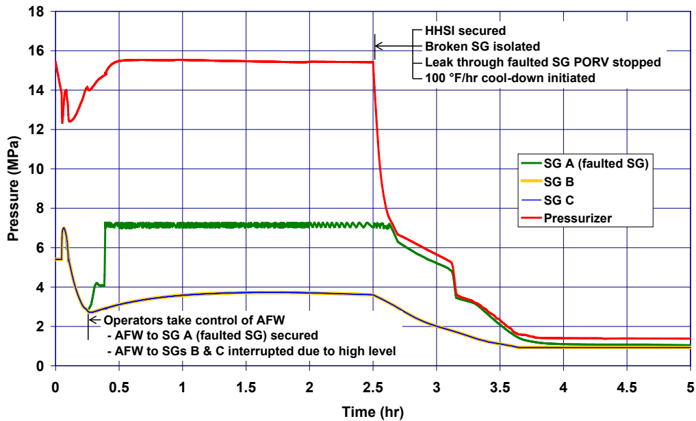
Figure 5-89 SGTR with Operator Action – System Pressures
