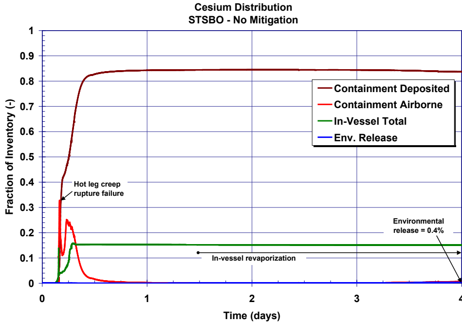
Figure 5-37 Unmitigated STSBO cesium fission product distribution history 24
