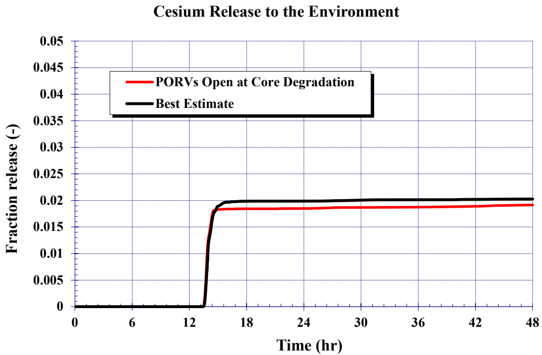
Figure 5-158 Cesium Release to the Environment – PORVs Open at Core Degradation
