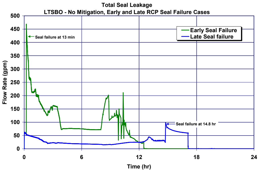
Figure 5-17 Comparison of the unmitigated long-term station blackout RCP seal leakages with and without early RCP seal failures
