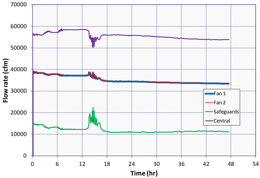
Figure 5-126 ISLOCA Safeguards Exhaust Ventilation Flows
