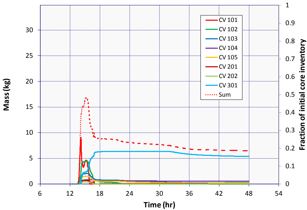
Figure 5-142 CsI Capture along LHSI Piping in ISLOCA Deposition Calculation
