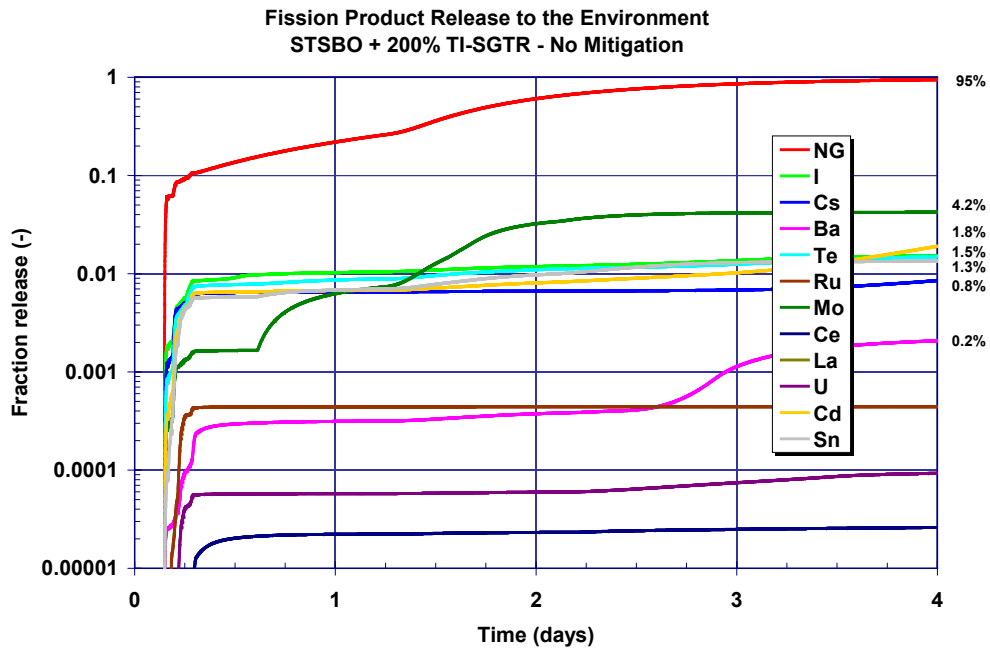
Figure 5-77 The unmitigated 200% TI-SGTR short-term station blackout environmental release history of all fission products
