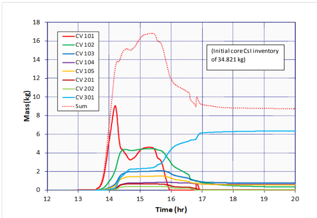
Figure 5-141 CsI Capture along LHSI Piping in ISLOCA Deposition Calculation (Early)
