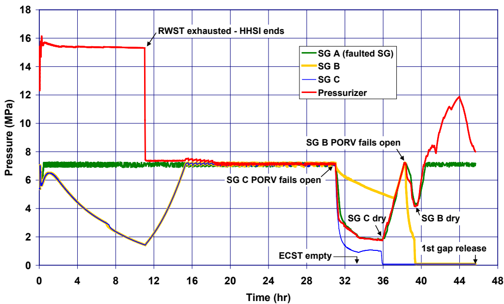
Figure 5-96 SGTR with Failed Operator Action – System Pressures
