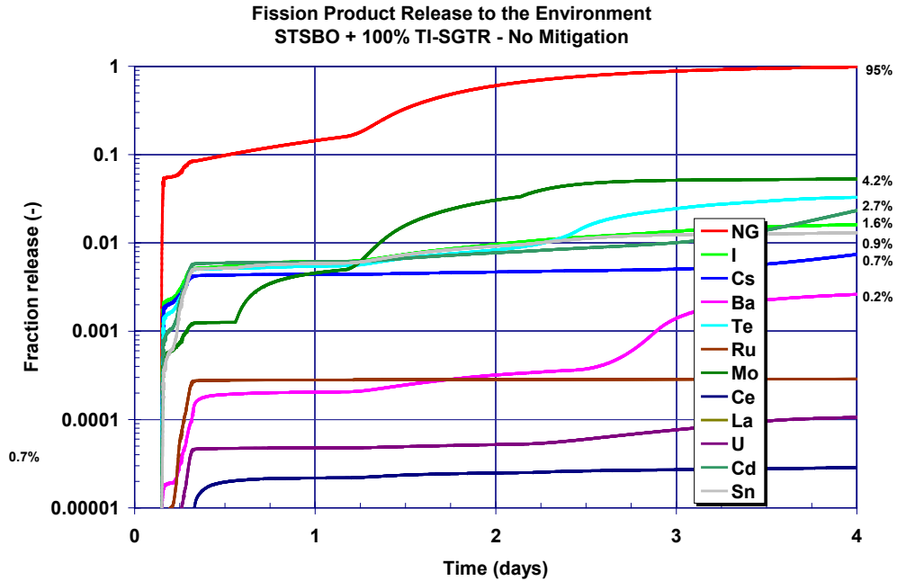
Figure 5-76 The unmitigated 100% TI-SGTR short-term station blackout environmental release history of all fission products
