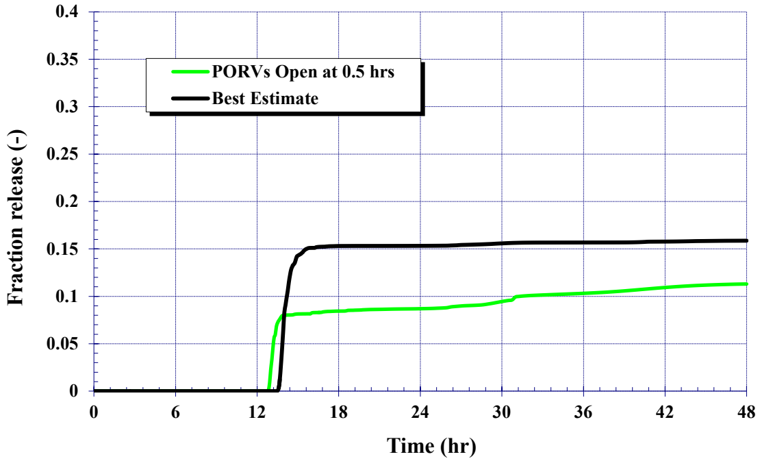
Figure 5-155 Iodine Release to the Environment – PORVs Open at 0.5 hrs
