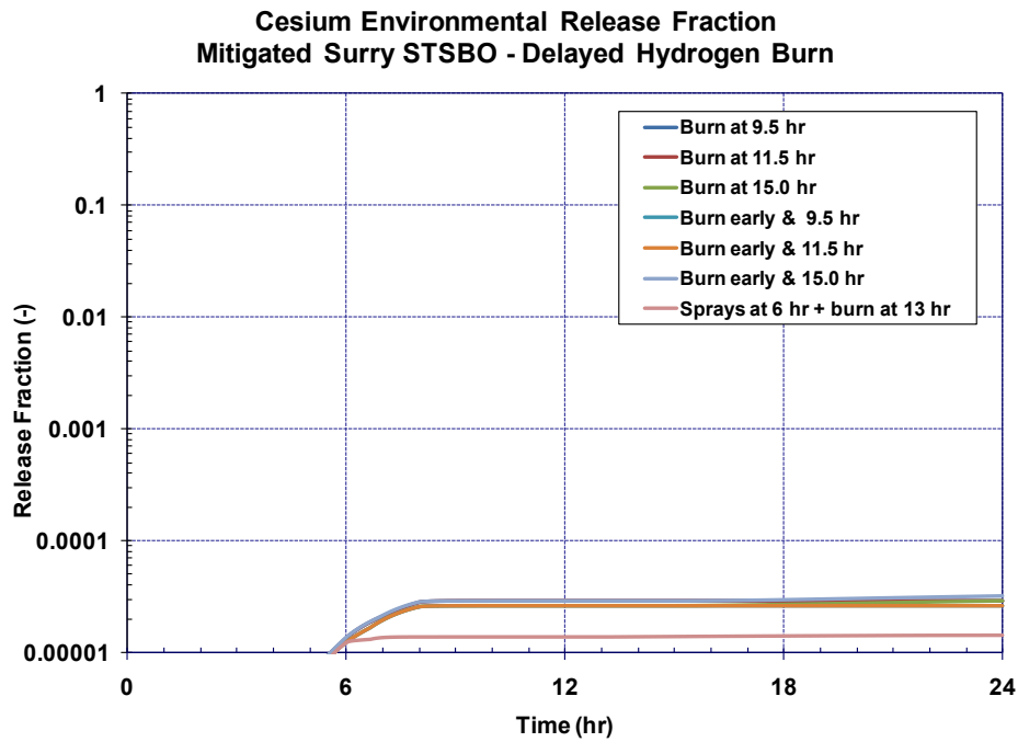
Figure 5-55 Comparison of the cesium release to the environment for the sensitivity calculations with delayed ignition
