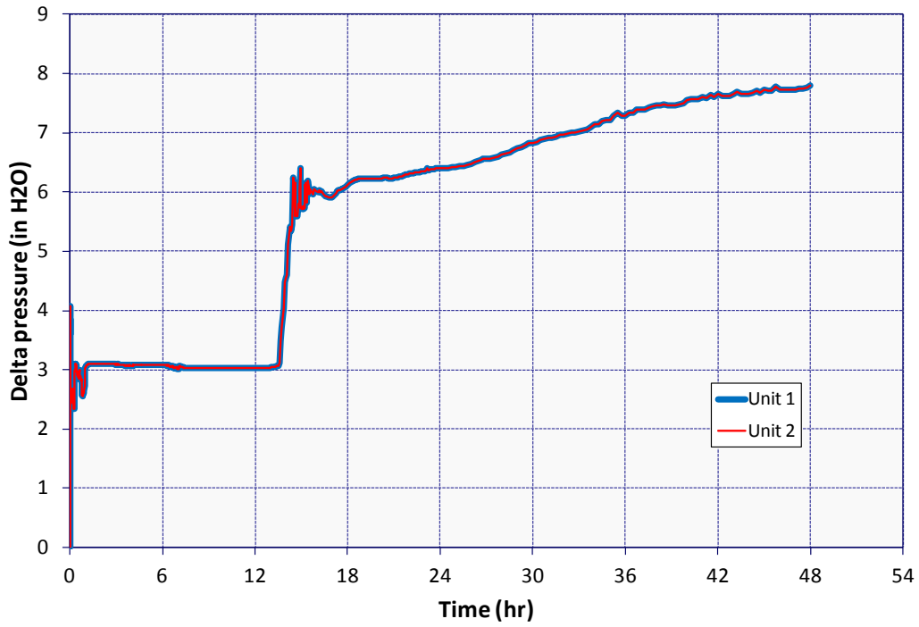
Figure 5-128 ISLOCA Safeguards Exhaust Ventilation Filter Unit Pressure Differential
