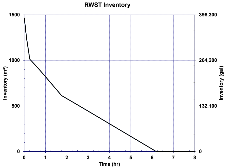
Figure 5-148 RWST Volume for the Unmitigated ISLOCA
