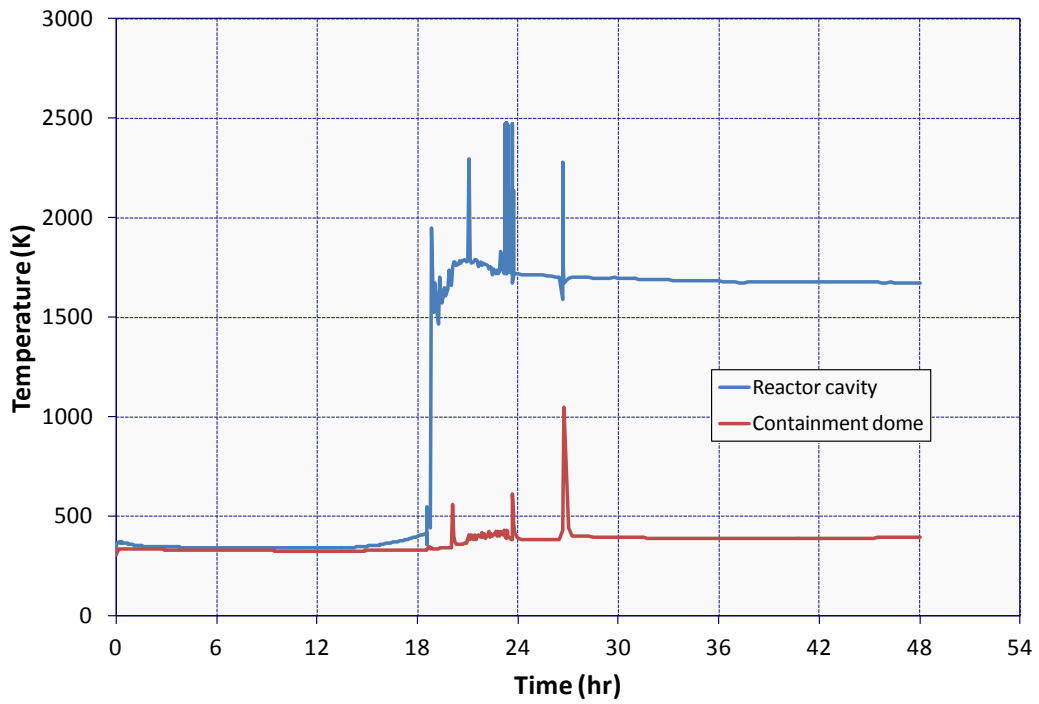
Figure 5-118 ISLOCA Containment Temperature
