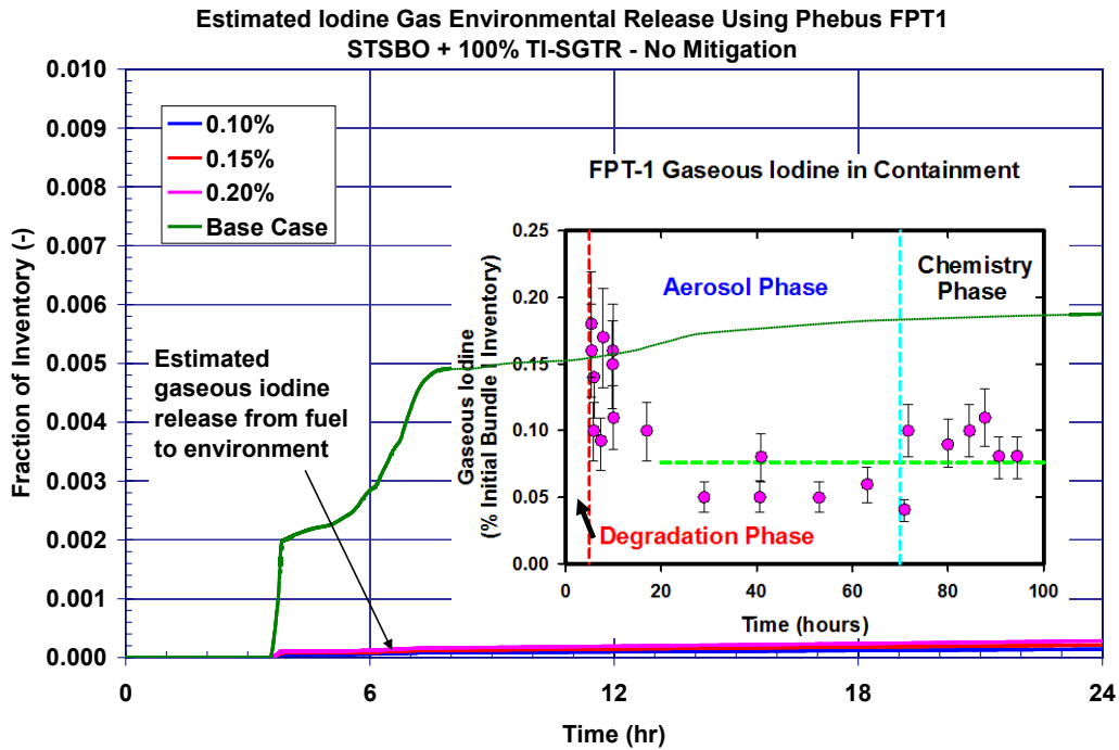
Figure 5-166 The additional gaseous iodine source term using Phebus data is compared to the iodine source term for the unmitigated short-term station blackout with a thermally-induced steam generator tube rupture
