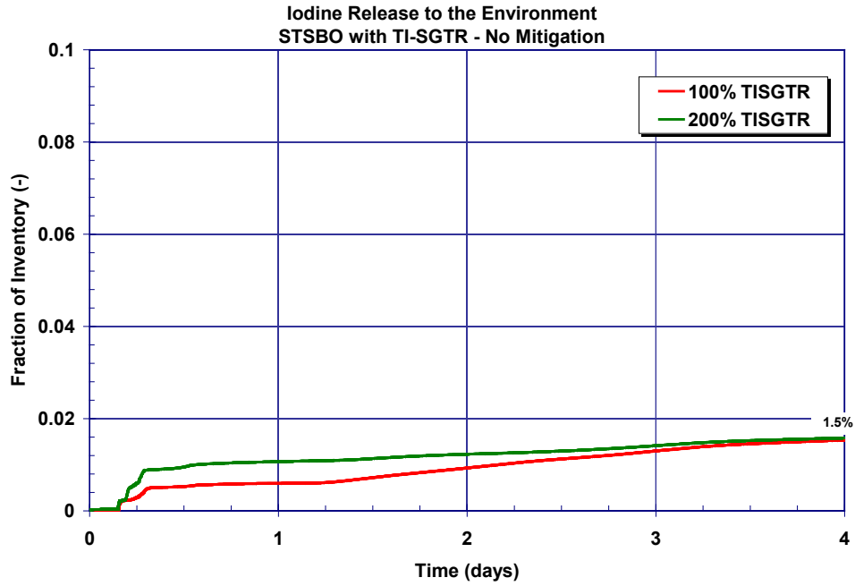
Figure 5-74 The unmitigated 100% and 200% TI-SGTR short-term station blackout iodine fission product distribution history
