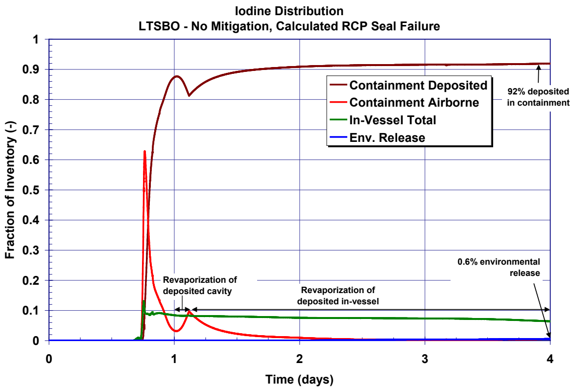
Figure 5-7 Unmitigated LTSBO iodine fission product distribution history
