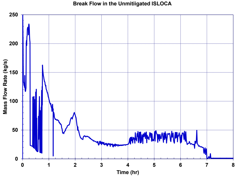
Figure 5-147 ISLOCA Break Flow for the Unmitigated ISLOCA
