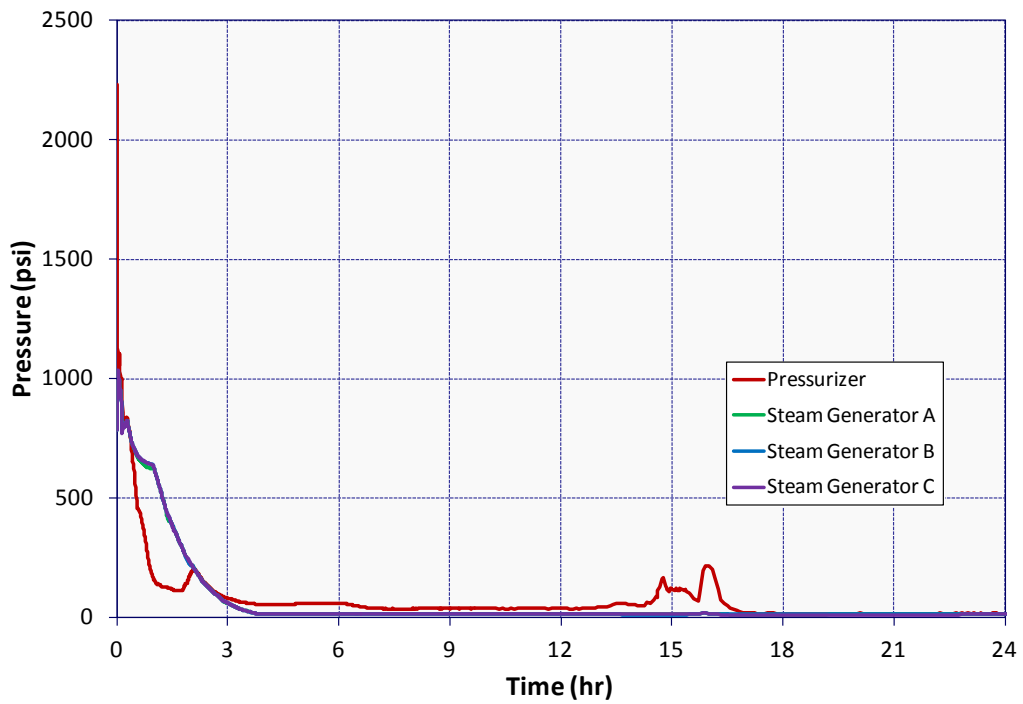
Figure 5-108 ISLOCA Reactor System Pressure
