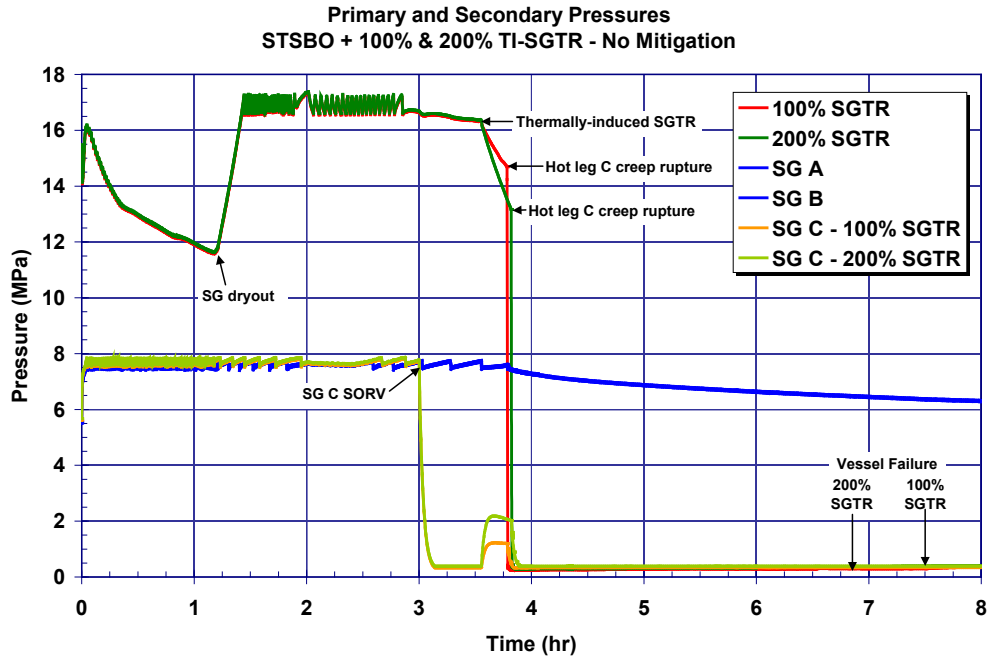
Figure 5-60 Unmitigated 100% and 200% TI-SGTR STSBO primary and secondary pressures histories
