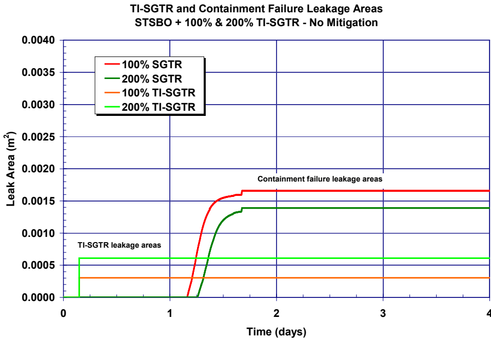
Figure 5-69 Unmitigated 100% and 200% TI-SGTR short-term station blackout containment and TI-SGTR leakage areas
