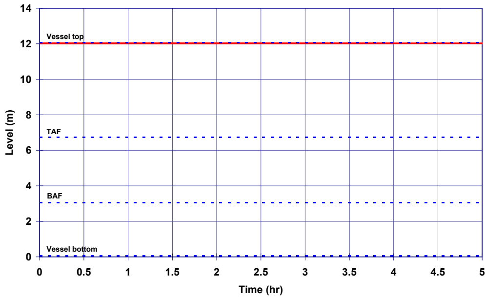
Figure 5-91 SGTR with Operator Action – RPV Level
