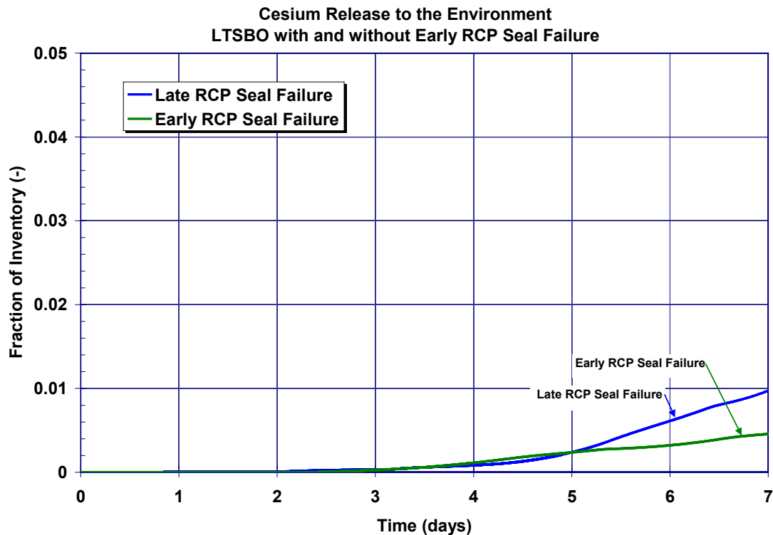
Figure 5-23 Comparison of the unmitigated long-term station blackout cesium releases to the environment with and without early RCP seal failures
