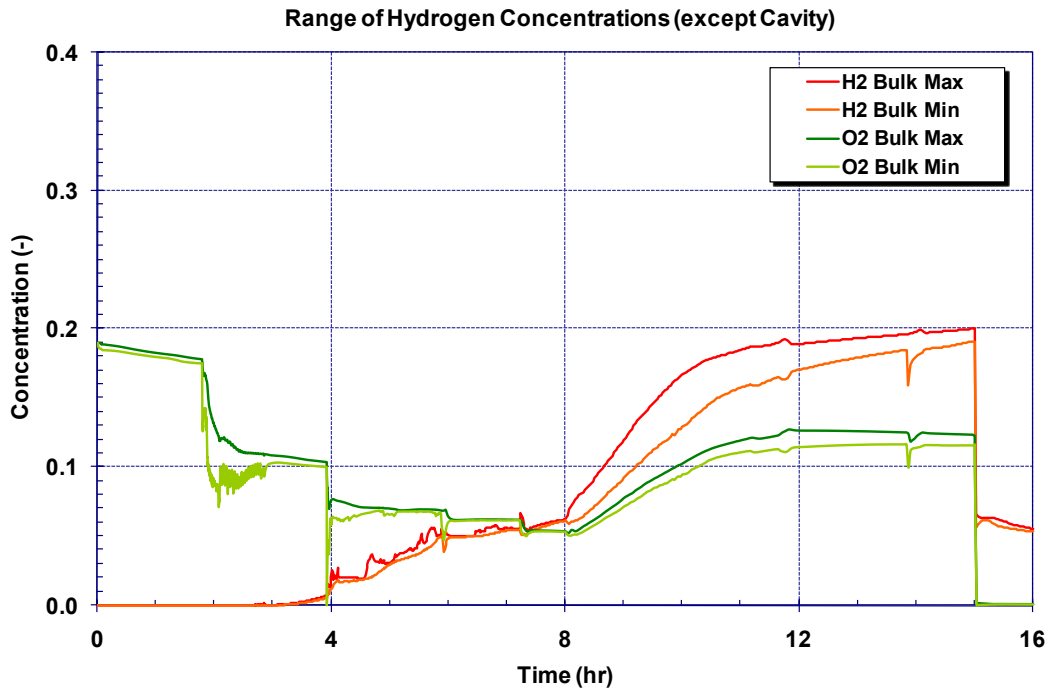
Figure 5-57 Mitigated short-term station blackout containment gas concentration history for the sensitivity calculation with delayed ignition
