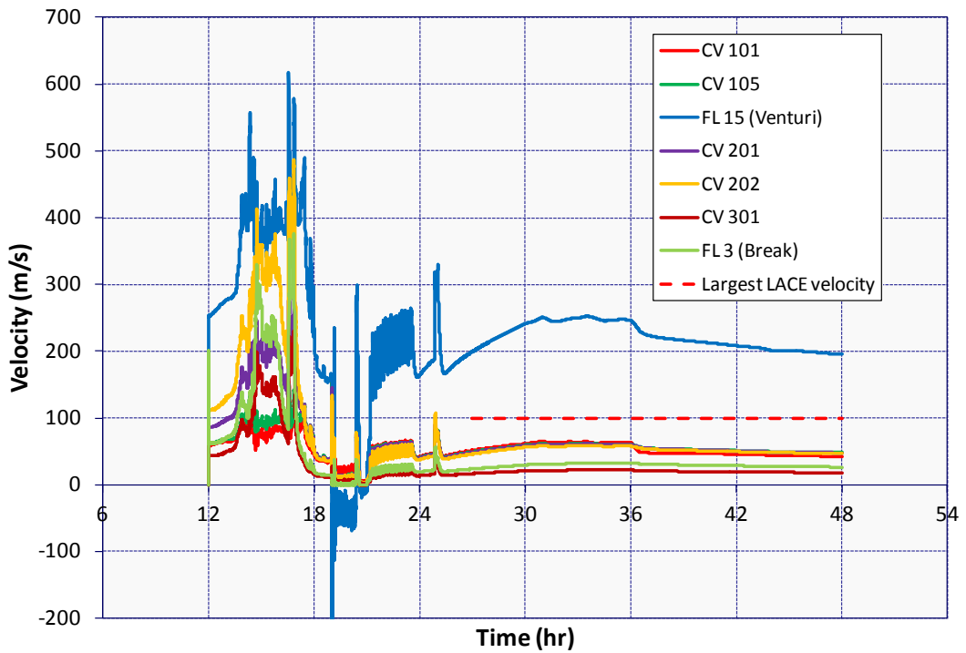
Figure 5-138 Vapor Velocity Along LHSI Piping in ISLOCA Deposition Calculation
