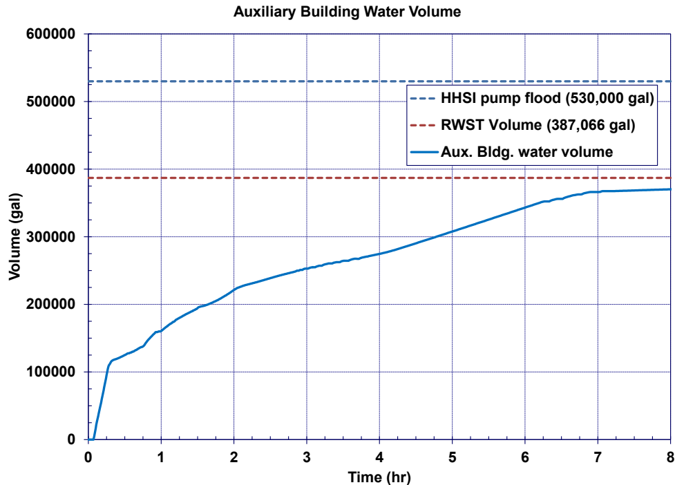
Figure 5-149 Auxiliary Building Water Volume for the Unmitigated ISLOCA
