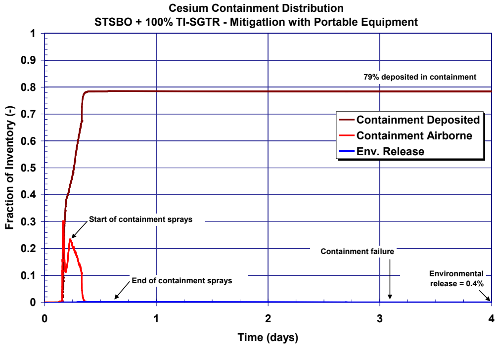
Figure 5-83 The cesium distribution in the containment for short-term station blackout with a 100% thermally-induced SGTR with spray mitigation
