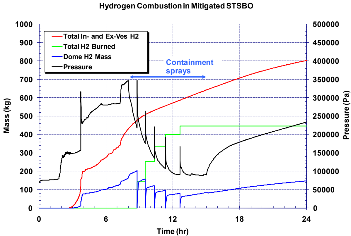
Figure 5-49 Comparison of the mitigated short-term station blackout containment pressure history versus the dome hydrogen mass and total hydrogen production
