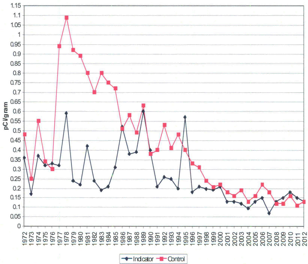
Figure 15: The concentration of Cesium-137 in soil has steadily declined in recent years. The peak seen in 1978 was due to fallout from nuclear weapons testing.
