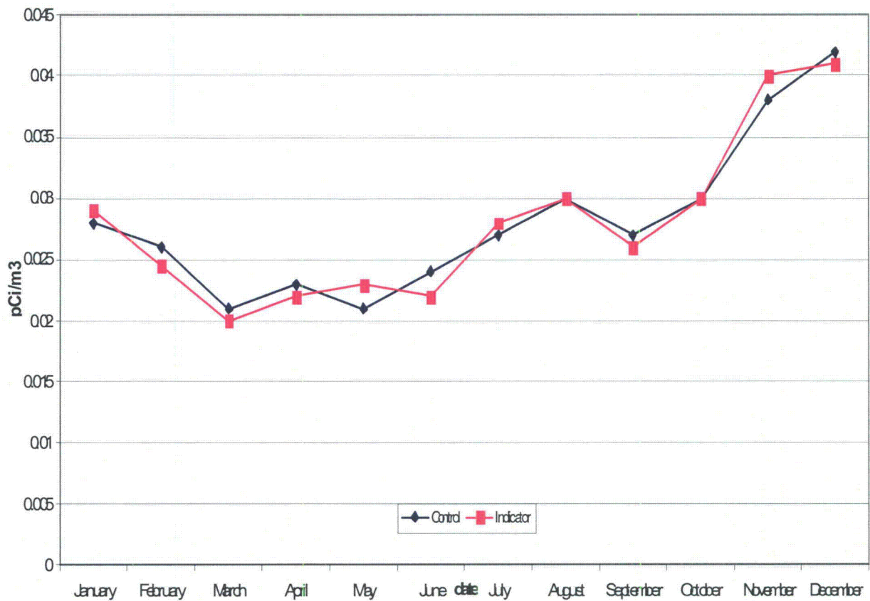
Figure 10. Concentrations of beta-emitting radionuclides in airborne particulate samples were nearly identical at indicator and control locations during 2012.
