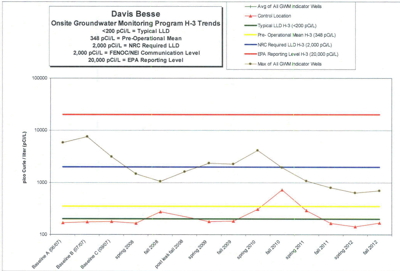
Figure 30 - Onsite Groundwater Monitoring
