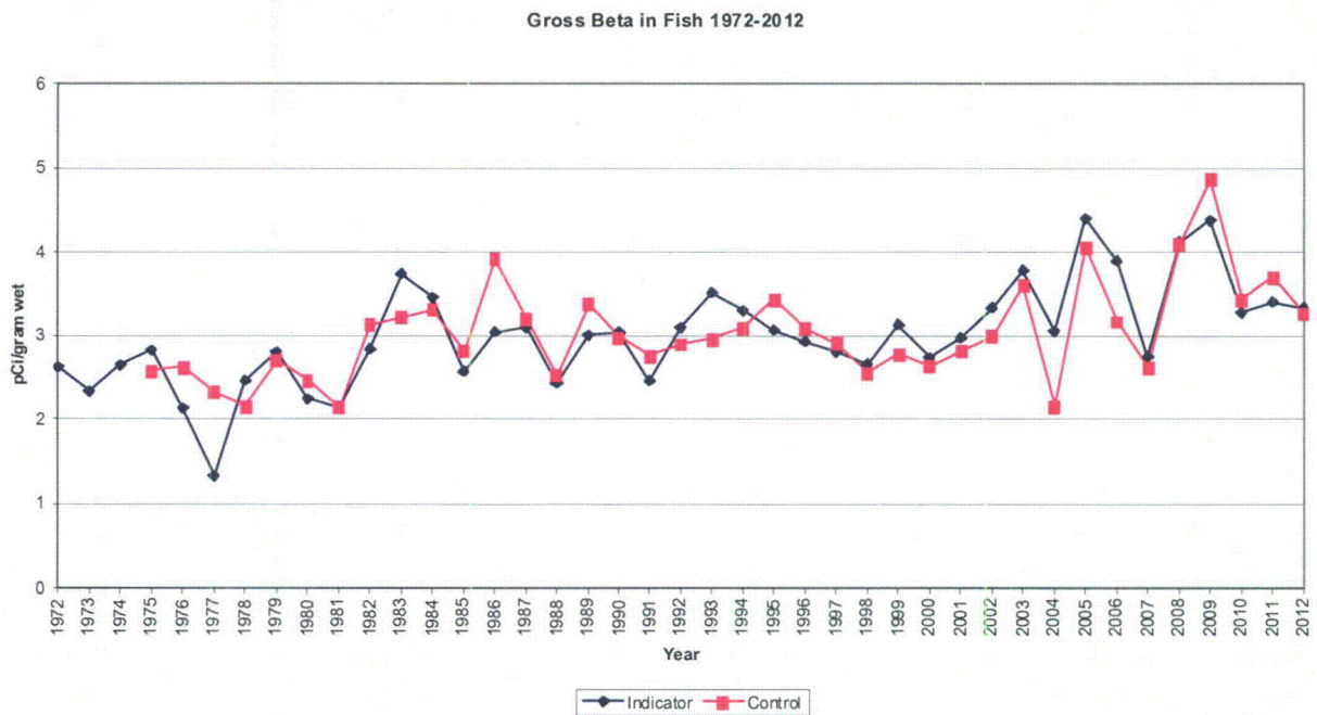
Figure 21: Average concentrations of beta-emitting radionuclides in fish samples were similar at indicator and control locations, and were comparable to results of previous years.
