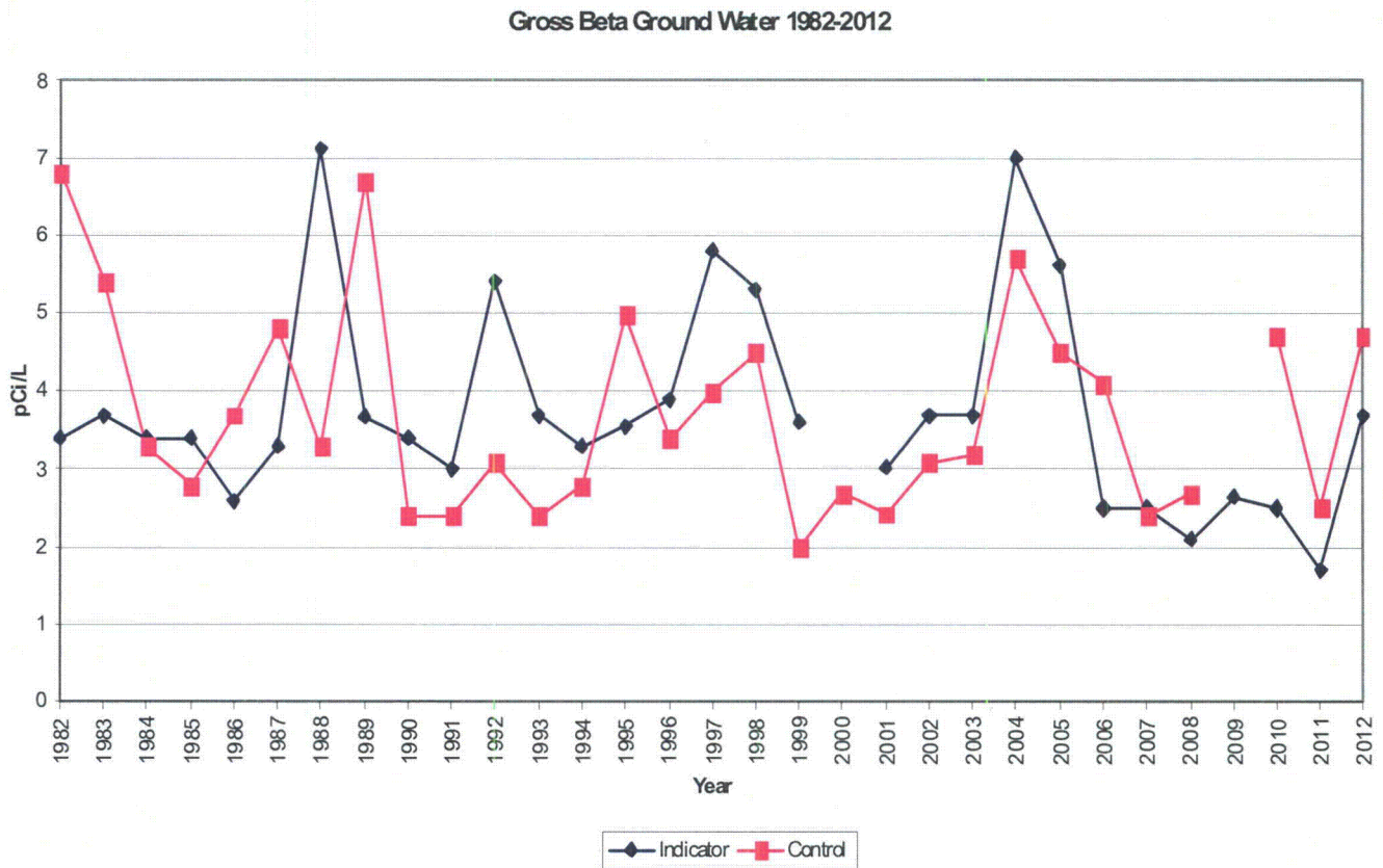
Figure 14: Shown above are the annual averages for gross beta in groundwater from 1982-2012. There were no indicator samples available in 2000 and no control samples available in 2009.
