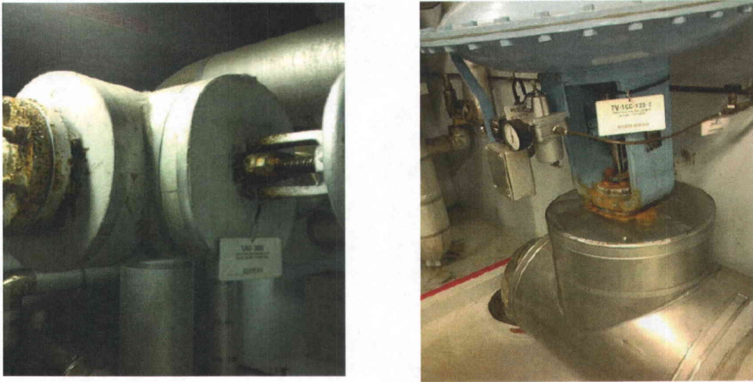
Figure 6-2: Corroded valves with old deficiency tags.
