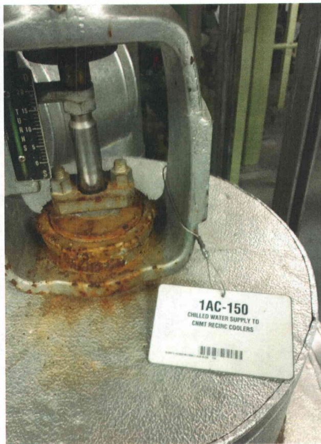
Figure 6-1: Surface corrosion for valve 1AC-150
