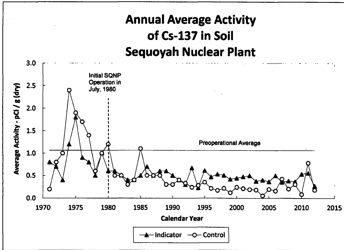
Figure H-3 Cs-137 in Soil
