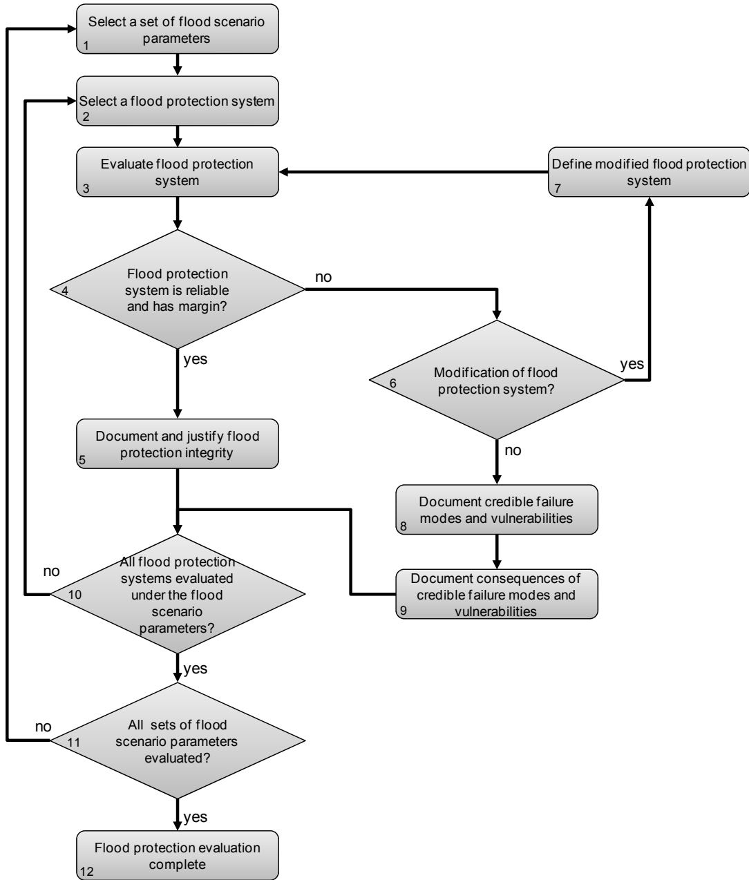
Figure 4: Flood protection evaluation procedure flowchart
