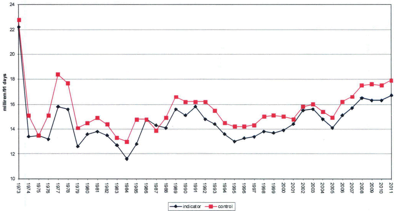
Figure 25: The similarity between indicator and control results demonstrates that the operation of Davis-Besse has not caused any abnormal gamma dose.
