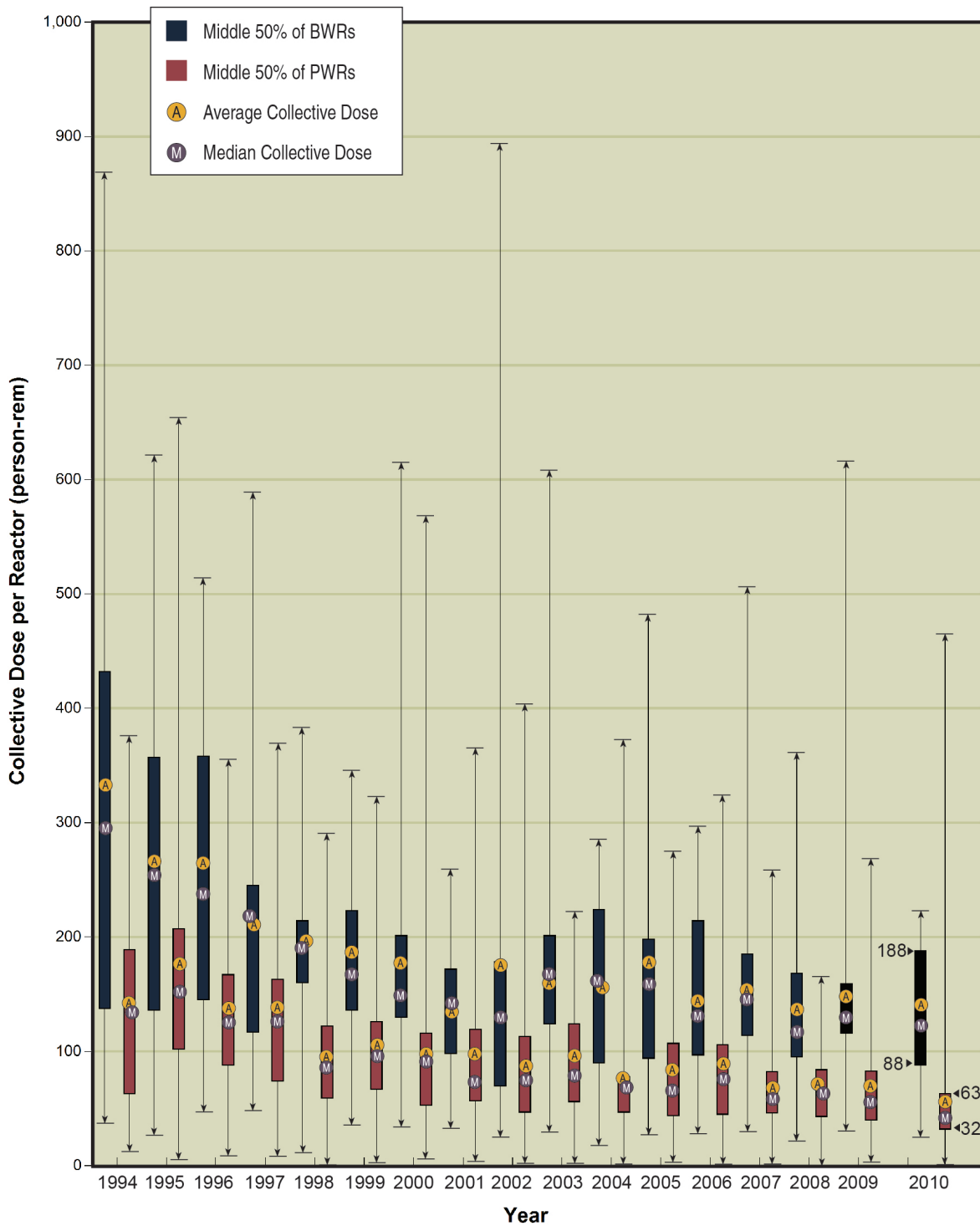
FIGURE 4.4. Average, Median, and Extreme Values of the Collective Dose per Reactor 1994–2010
