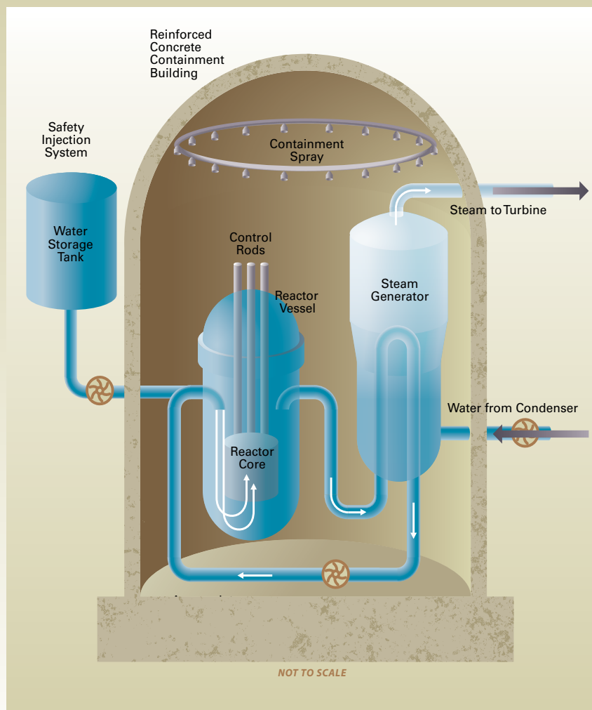
Figure 2.3 Typical U.S. Pressurized-Water Reactor.
