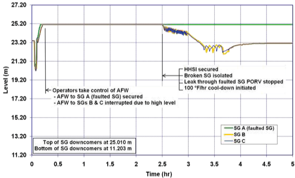
Figure 5-90 SGTR with Operator Action- Steam Generator Level
