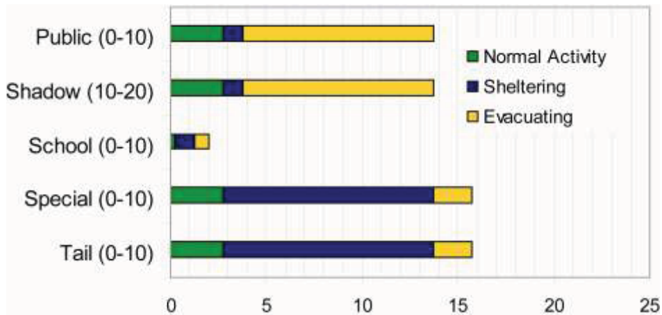
Figure 6-5 Duration of Protective Actions - Unmitigated STSBO
