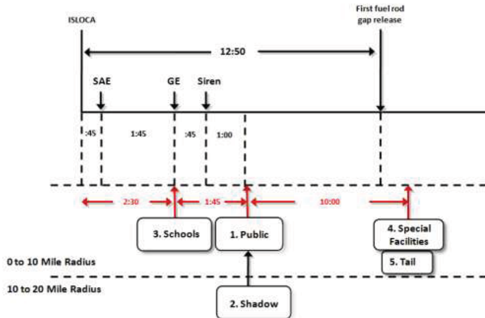
Figure 6-17 Unmitigated ISLOCA Timing for Sensitivity 3
