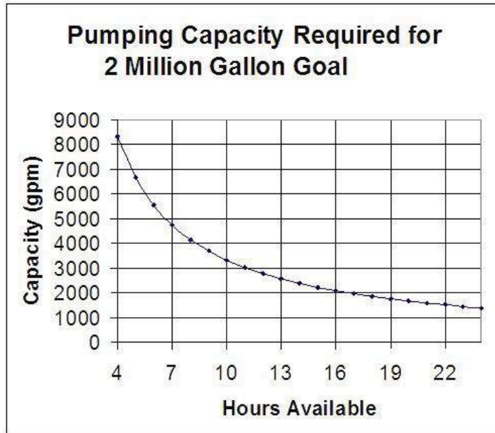
Figure 6-27 Pumping Capacity
