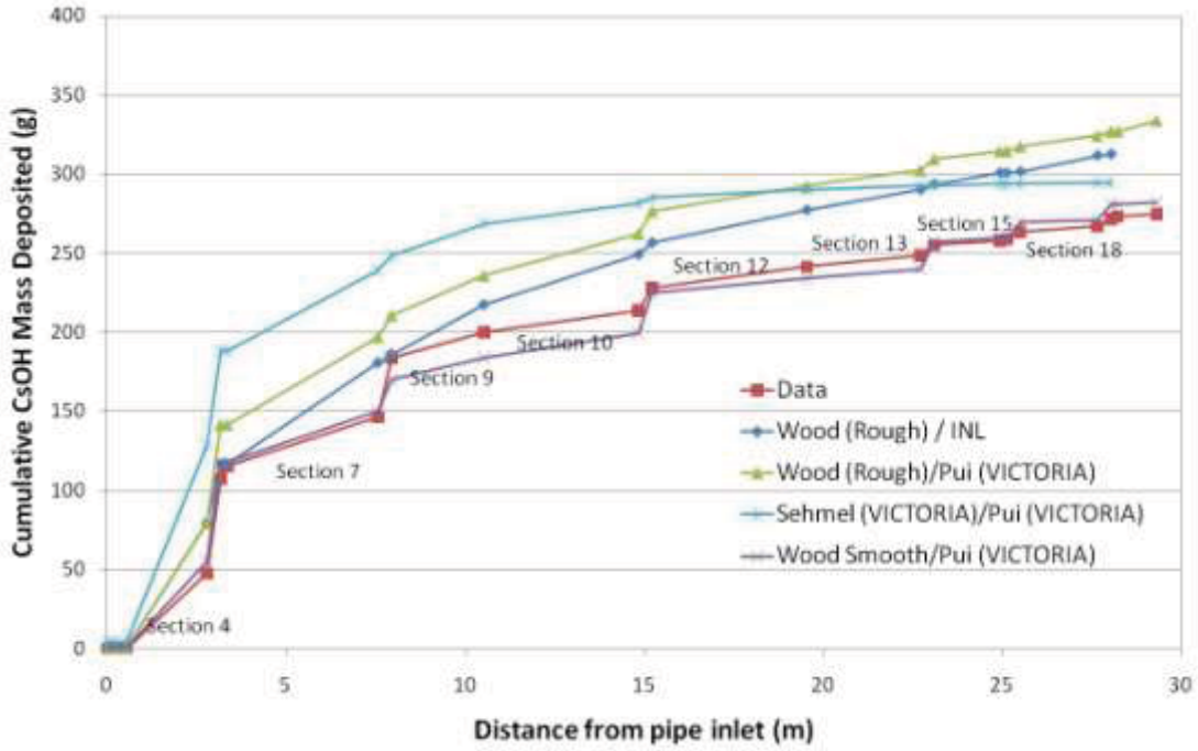
Figure D-42 Deposition profile along LA3A test section (20 aerosol size bins)
