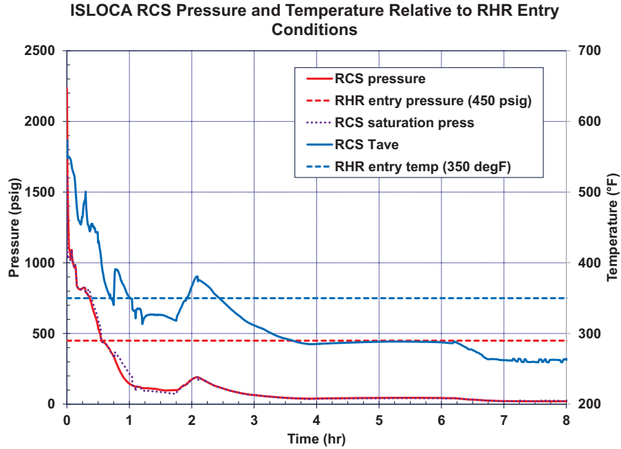
Figure 5-140 ISLOCA RCS Pressure and Temperature Relative to the RHR Entry Pressure and Temperature Criteria for the Unmitigated ISLOCA
