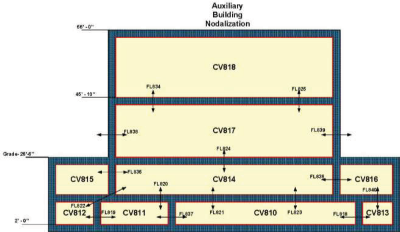
Figure 4-12 Auxiliary Building Hydrodynamic Nodalization
