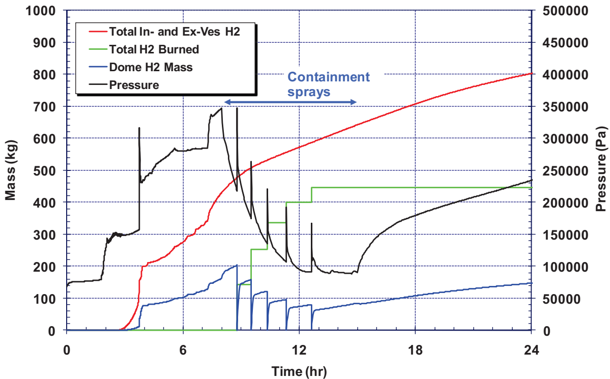
Figure 5-45 Comparison of the mitigated short-term station blackout containment pressure history versus the dome hydrogen mass and total hydrogen production
