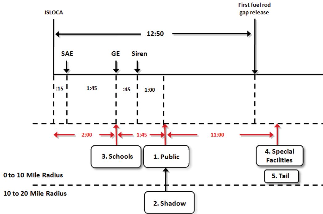
Figure 6-13 Unmitigated ISLOCA Timeline for Sensitivity 1
