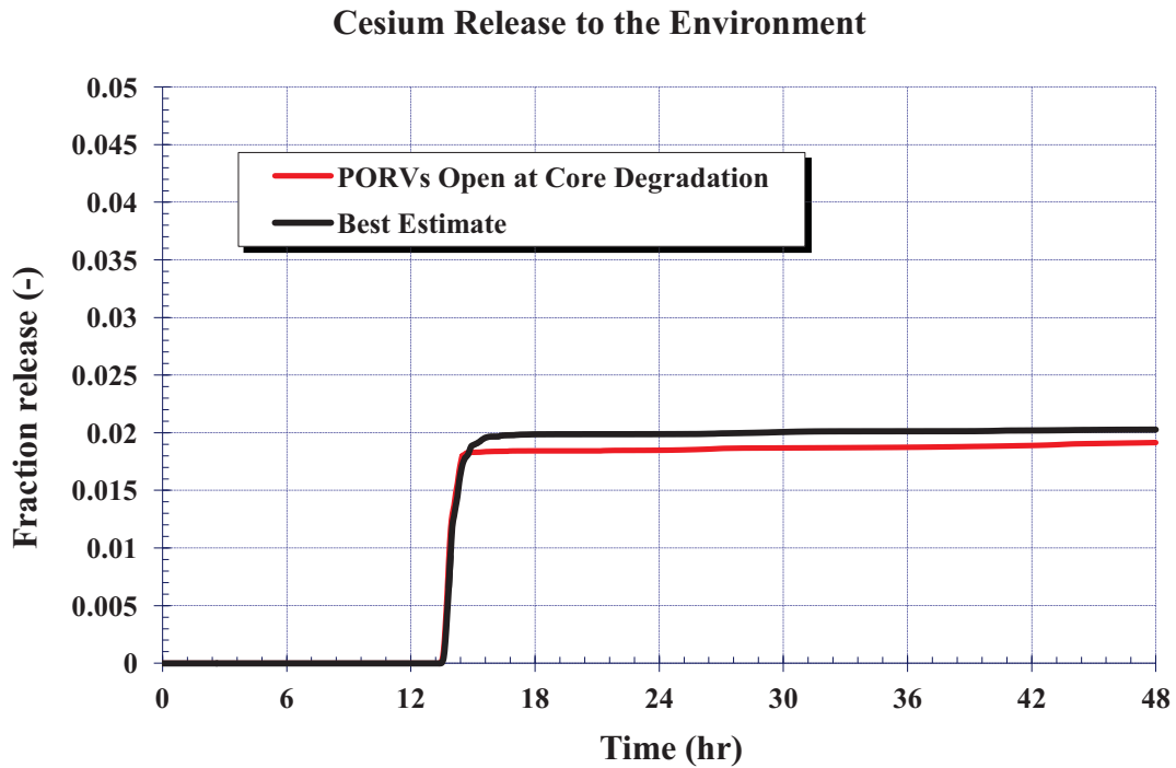
Figure 5-153 Cesium Release to the Environment – PORVs Open at Core Degradation
