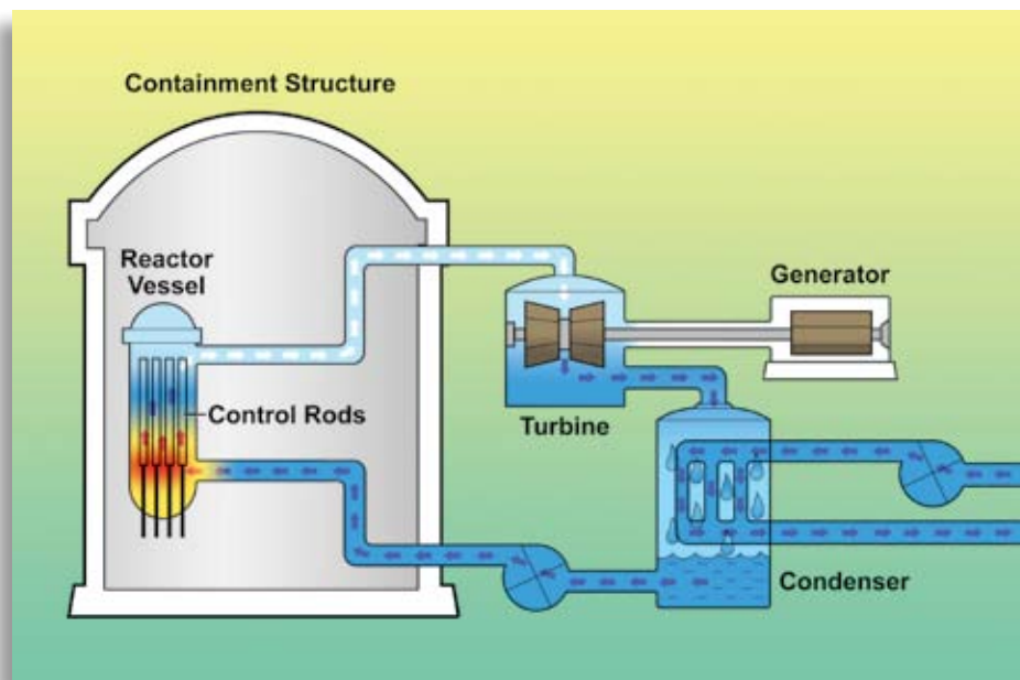
Boiling Water Reactor (BWR)
