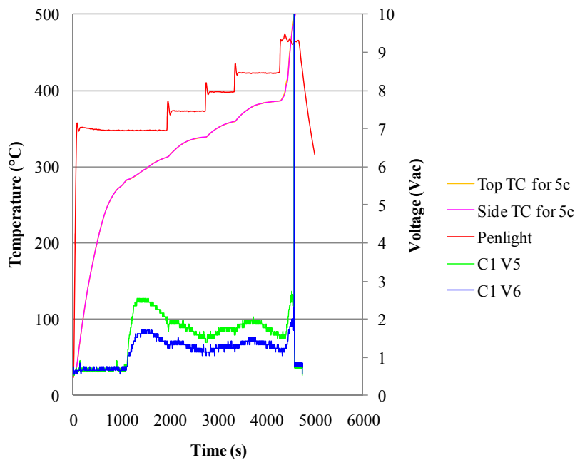
Figure 7.10: Item D target voltage increase during Test D13.
