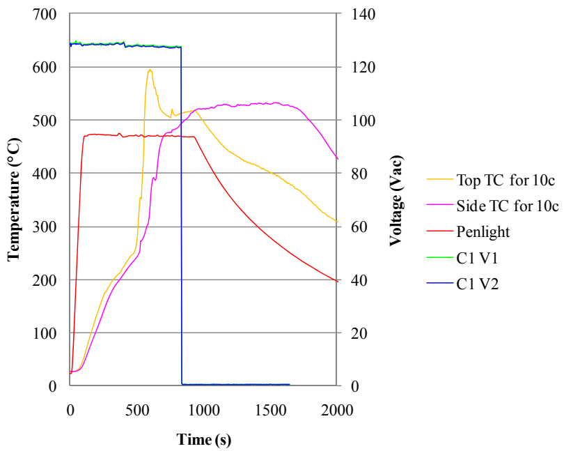
Figure B.115: Penlight shroud temperature and conductor voltages for Test D16.
