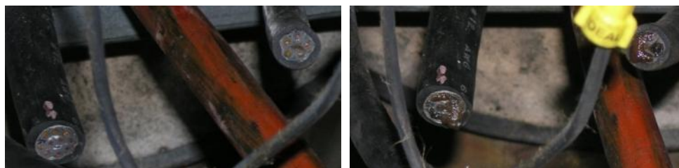
Figure 7.11: A pre-test view of the test cables (left) and a photo taken during the Test 15 (right) showing liquid leaking from the cut ends of the both of the thermal response cables (the 10/C and 5/C cables).
