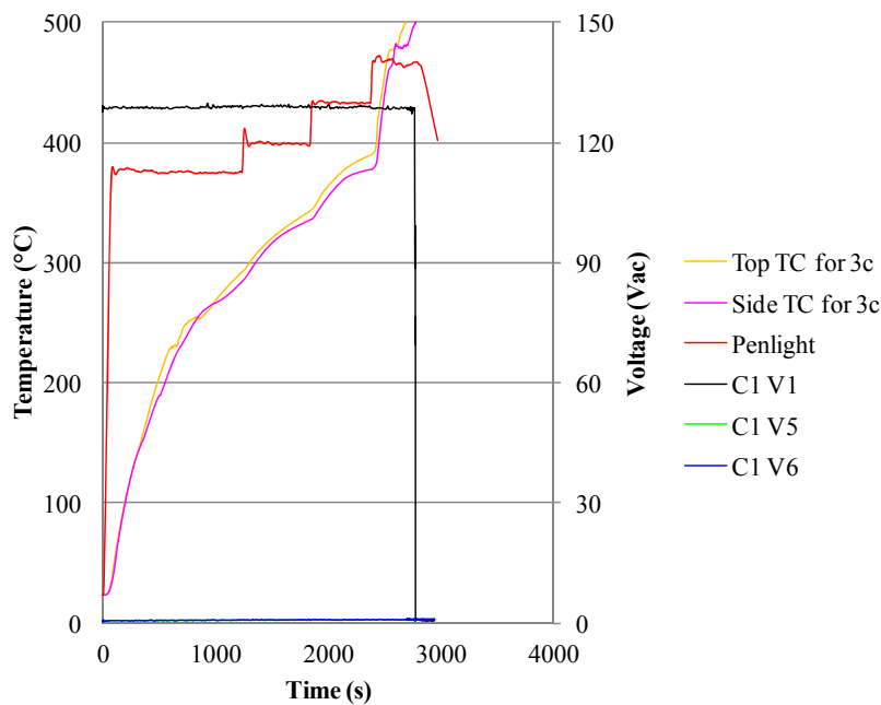
Figure 7.61: Test results for the HT insulated cable in Test 17-qual.
