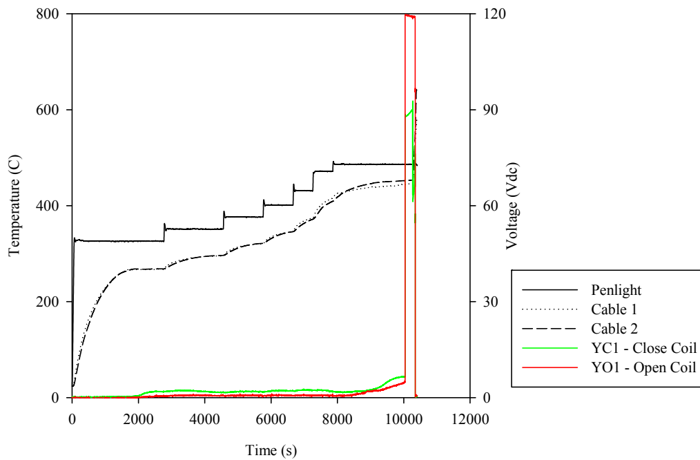
Figure B.56: Temperature profile and electrical response for Test D44, Circuit 2.
