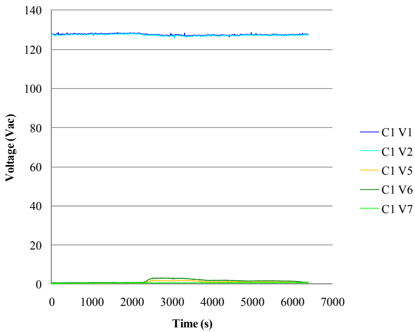
Figure B.27: All source and target conductor voltages for Test D15 displaying early degradation.
