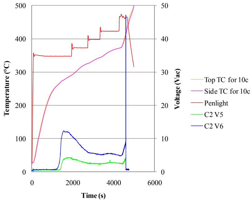
Figure B.106: Penlight shroud temperature and target conductor voltages for Test D13.
