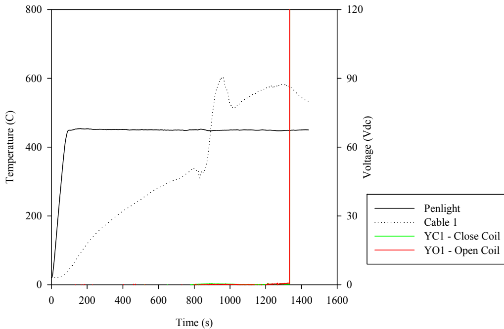
Figure B.67: Temperature profile and electrical response for Test D50, Circuit 1.
