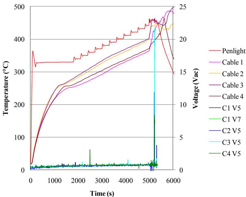
Figure 7.50: Temperature and target voltage response of Item I during Test K19.
