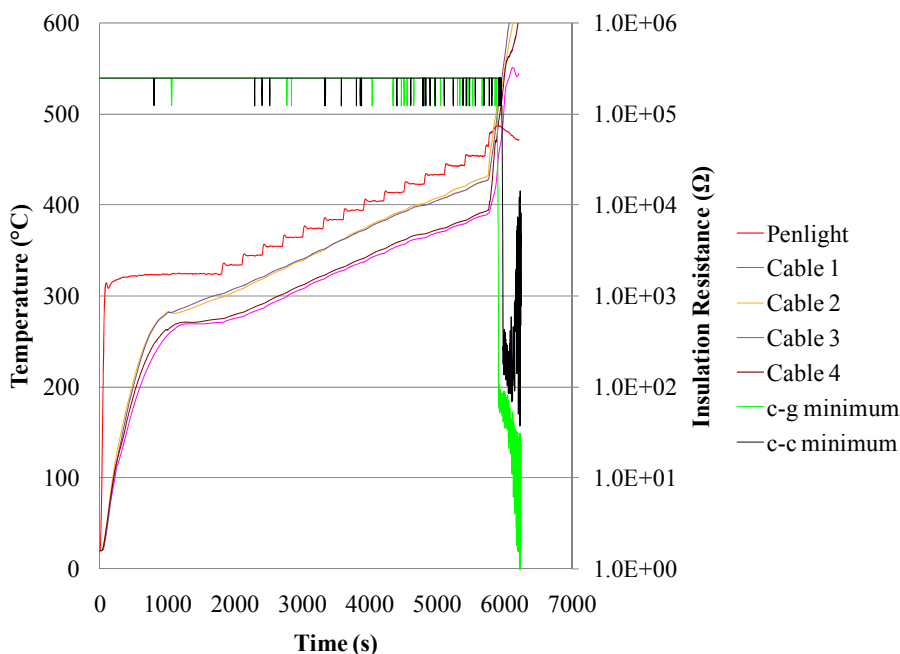
Figure 7.4: IRMS data for Item A during test K16.
