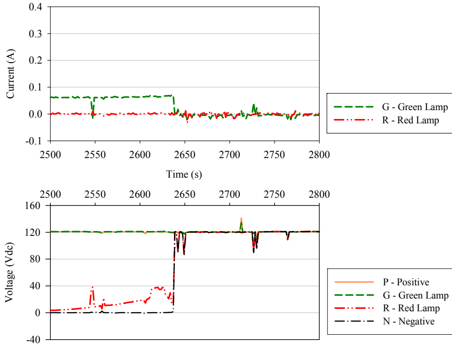
Figure B.88: Voltage and current response for the lamps in Test IS9, MOV1.
