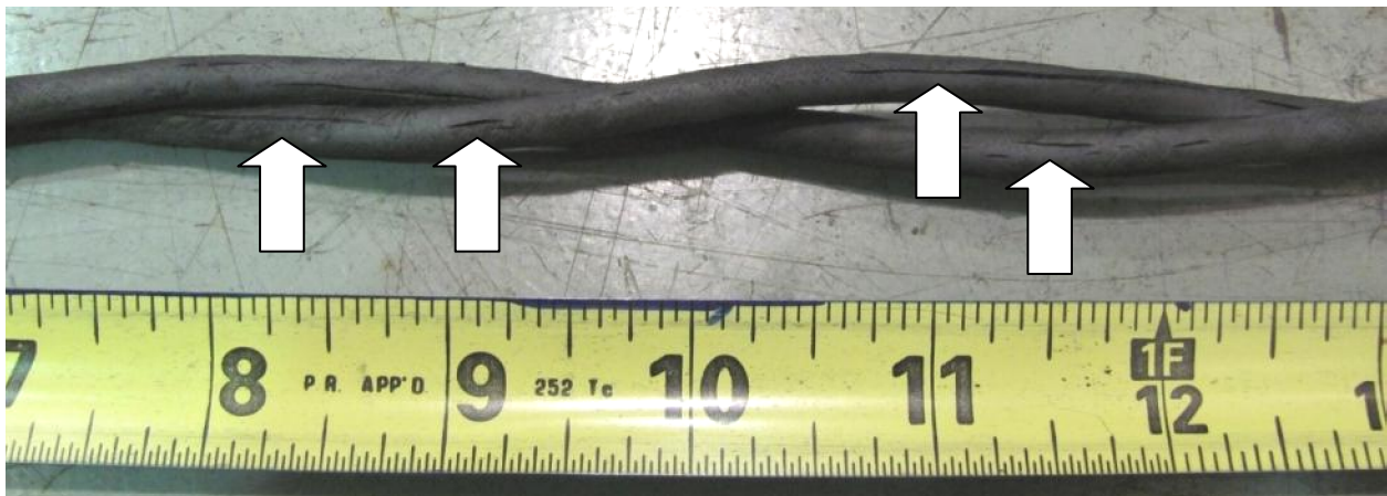
Figure 7.2: Longitudinal cracking along the conductors of Item A.
