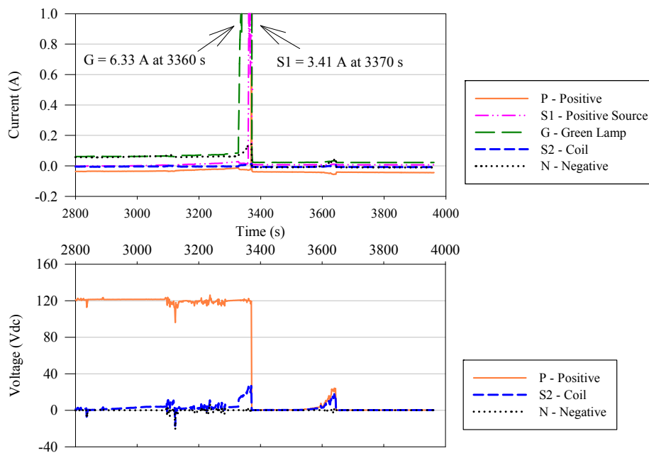
Figure B.128: Voltage and current response for the active target in Test IS10, SOV1.
