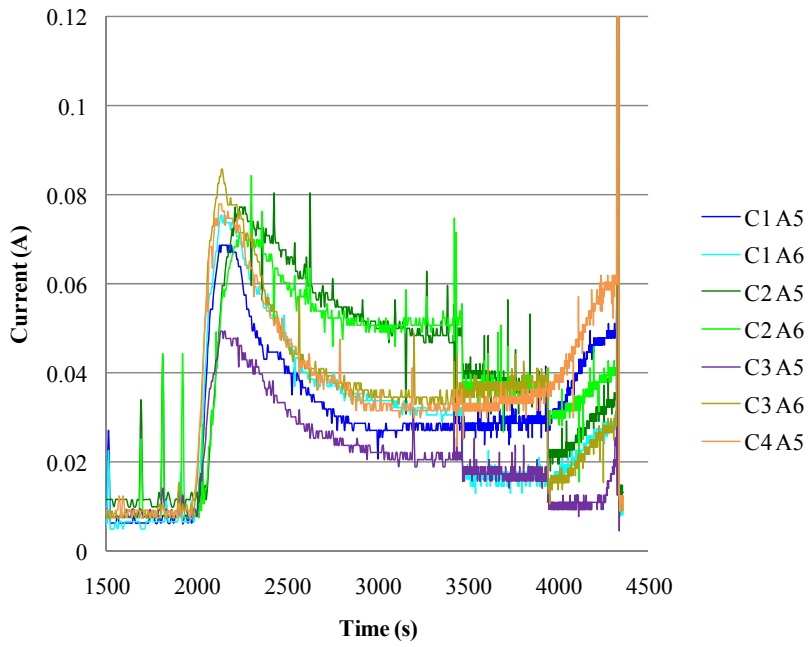
Figure 7.57: Modified target currents for Item J during Test K20.
