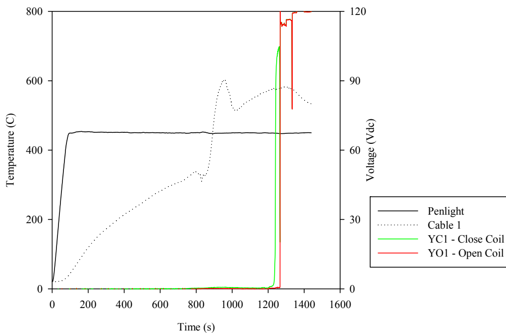
Figure B.70: Temperature profile and electrical response for Test D50, Circuit 2.
