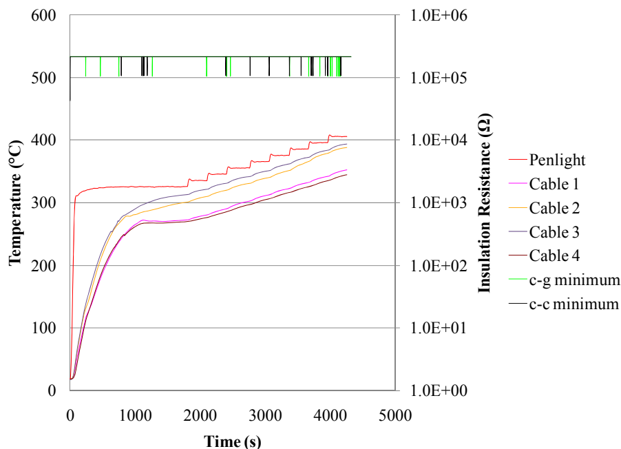
Figure B.8: Penlight shroud temperature, cable temperatures, and electrical performance data for Test K14.
