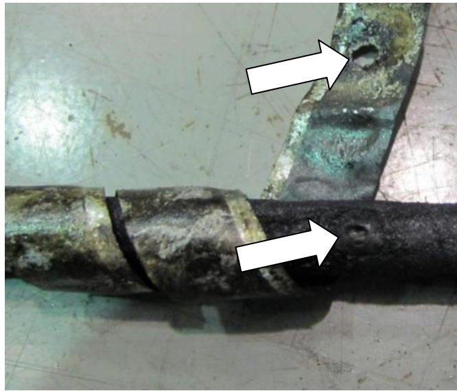
Figure 7.16: Hole in the conductor insulation corresponding to the hole found in the zinc wrap.
