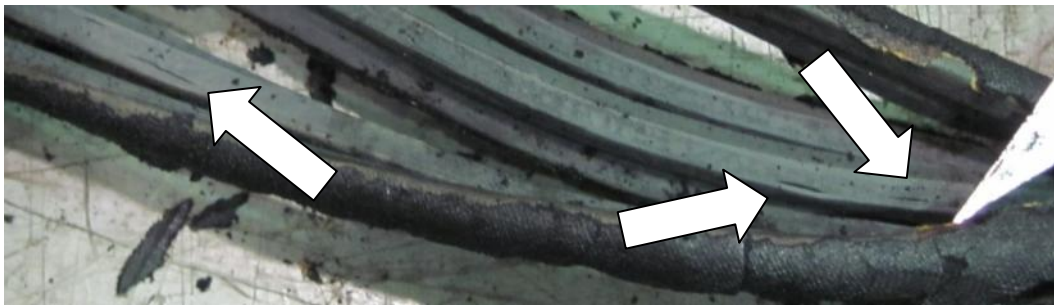
Figure 7.21: Longitudinal cracking found along the conductors of Item E
